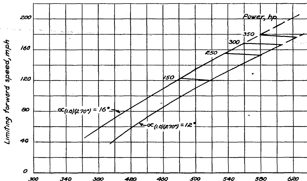
(a) Limiting forward speed and power required at altitude of 5000 feet.
