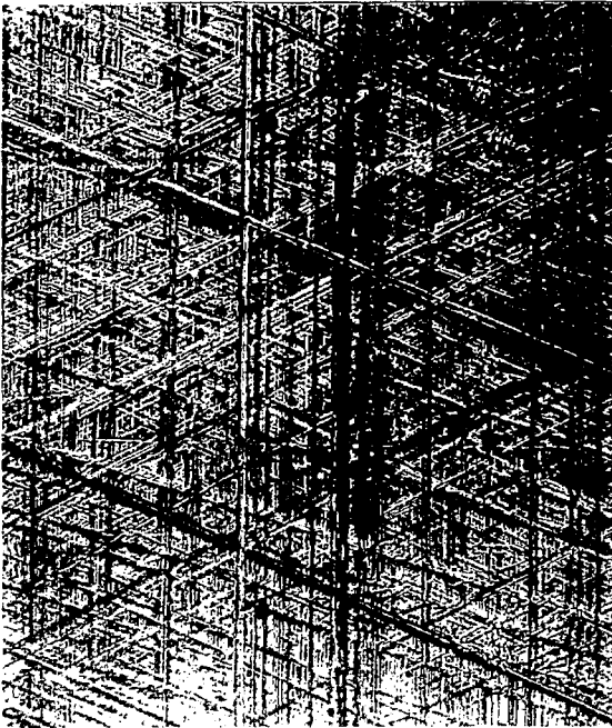
Figure 11. - A positive replica of the general surface area in an Allison V-1710 cylinder barrel after 33 hours of test running. X112.
