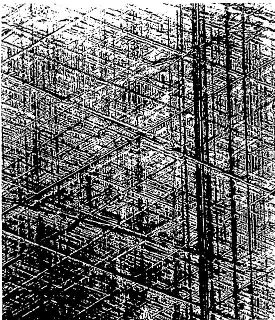
Figure 13. - A positive replica of the area at the bottom of ring travel of the top ring in an Allison V-1710 cylinder after 33 hours of test running. X112.
