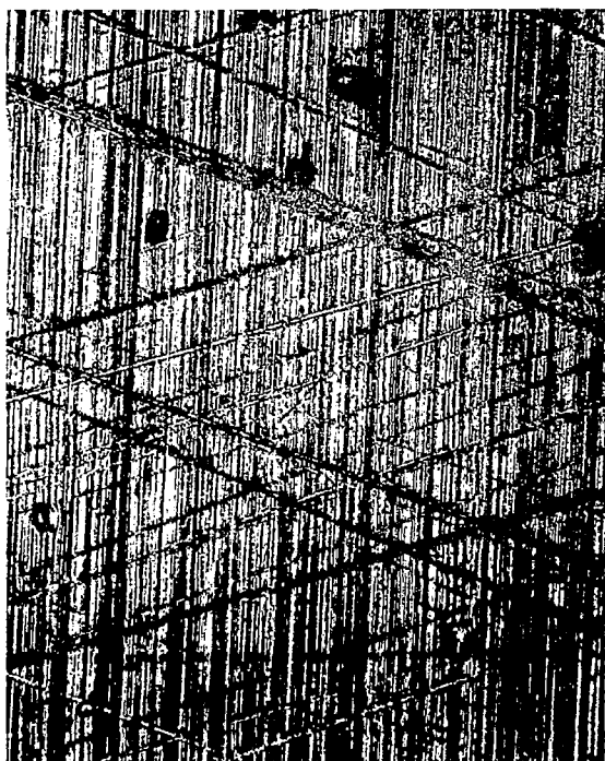
Figure 5. - A positive replica of the coarsely honed Allison V-1710 cylinder barrel after 48 hours of test running. X112.
