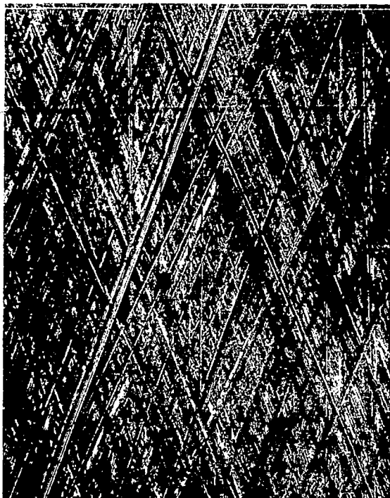
Figure 3. - A positive replica of a new coarsely honed Allison V-1710 cylinder barrel. X112.
