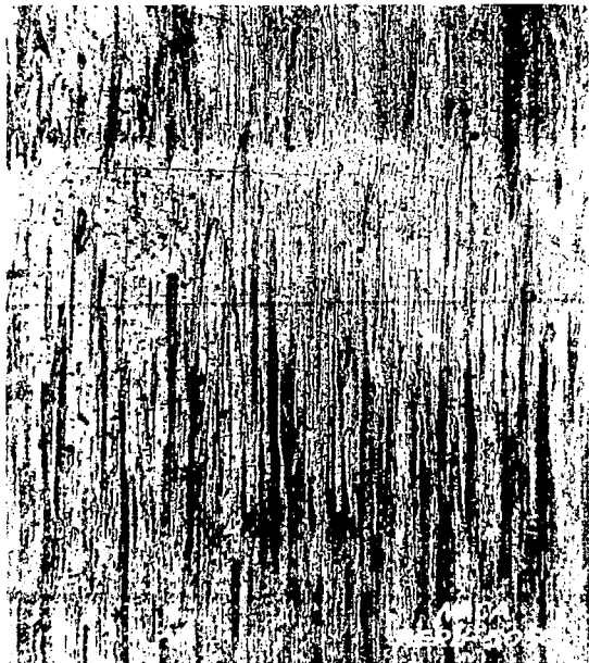
Figure 10. - A positive replica of the area at the top of ring travel in an Allison V-1710 cylinder barrel after 225 hours of test running. The top ring was stuck. X112.
