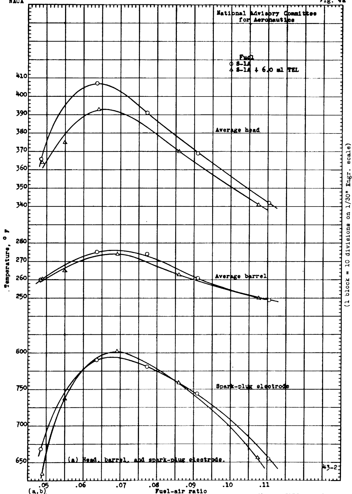
Figure 4. - Effect of tetraethyl lead on cylinder temperatures. Wright C90C cylinder; engine speed, 2000 rpm; compressure ratio, 7.0; inlet-air temperature, 250° F; cooling-air pressure drop, 2.7 inches of water; indicated mean effective pressure, 93 pounds per square inch.
