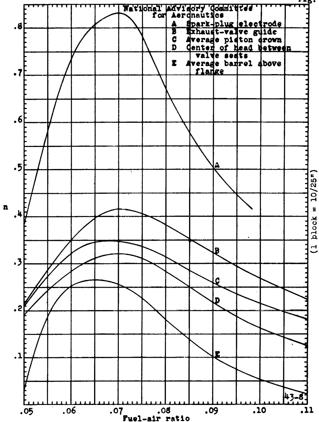
Figure 9. - Variation of the exponent n of the expression \bar{T} = c_1 \bar{T}^n with mixture ratio for an inlet-air temperature of 150^\circ\text{F} . Lycoming O-1230 cylinder; engine speed, 2000 rpm; compression ratio, 7.0; coolant-outlet temperature, 250^\circ\text{F} .
