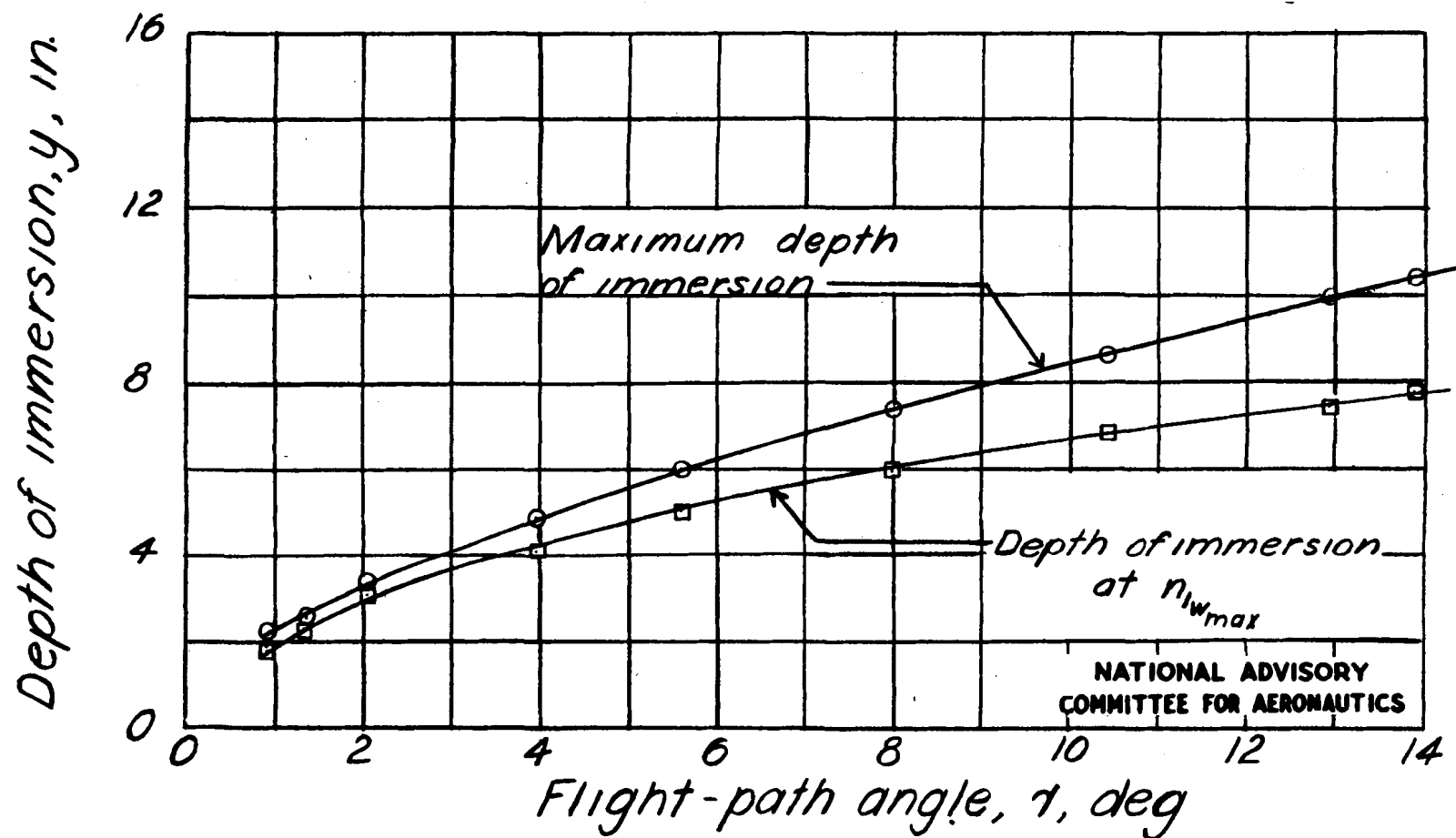
Figure 3.- Variation of maximum depth of immersion and immersion at time of maximum acceleration with flight-path angle. \tau = 6^\circ ; W = 1100 pounds.
