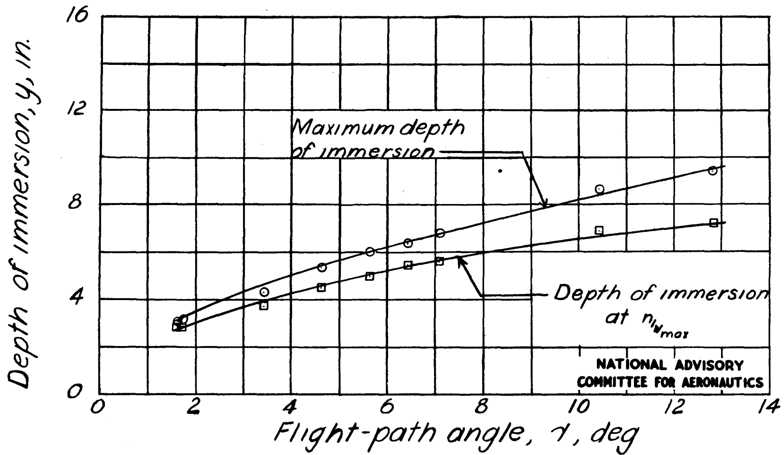
Figure 4.- Variation of maximum depth of immersion and immersion at time of maximum acceleration with flight-path angle. \tau = 9^\circ ; W = 1100 pounds.
