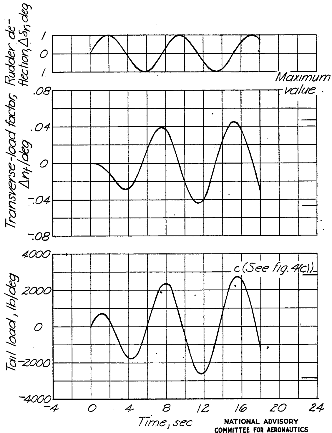
Figure 3.- Calculated tail load and transverse-load factor during fishtail maneuver on large flying boat.
