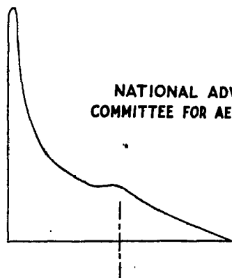
Figure 4.- Chordwise load distribution over typical section of vertical tail of flying boat.
