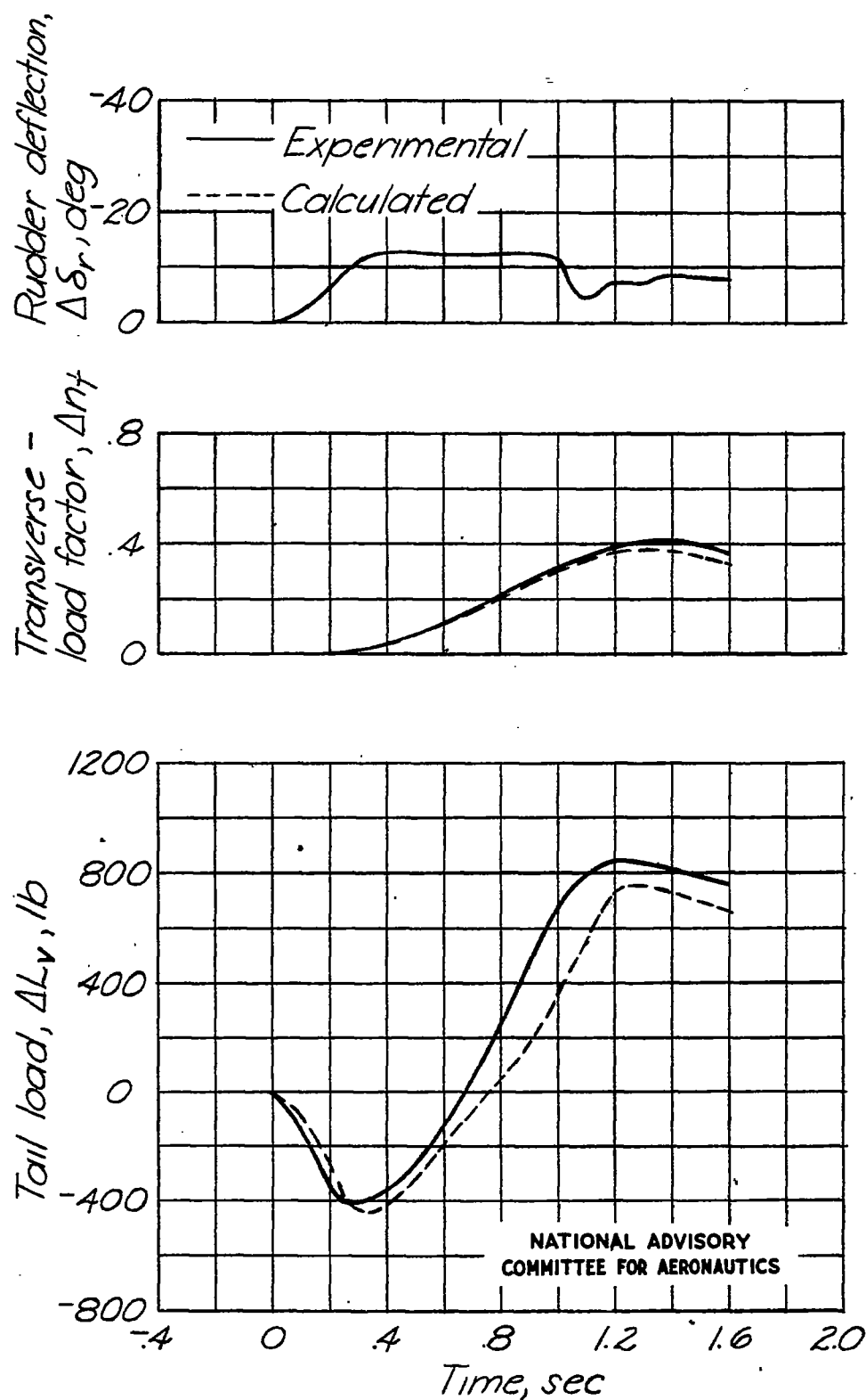
Figure 1.- Comparison of calculated and measured tail loads during rudder deflection on fighter airplane.
