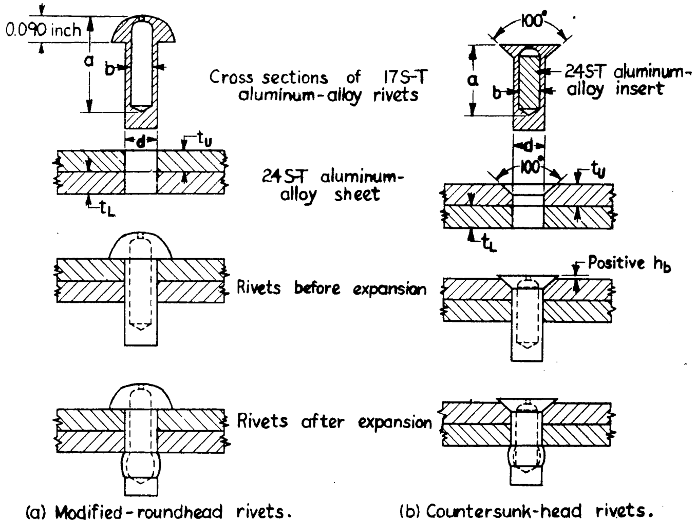
Figure 1.-Riveting procedure.
