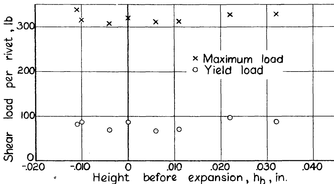
(c) Variation of yield and maximum load with h_b of countersunk-head-rivet specimens, t=0.081 in.
