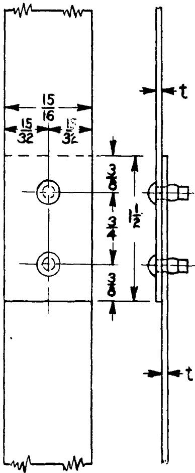
(a) Shear specimen
