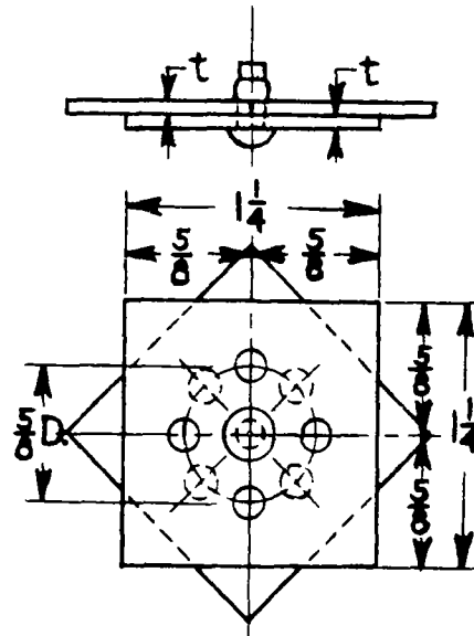
(b) Tension specimen
