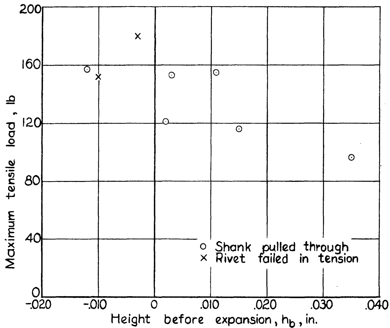
Figure 7.~ Variation of maximum tensile load with h_b ; t=0.081 in.
