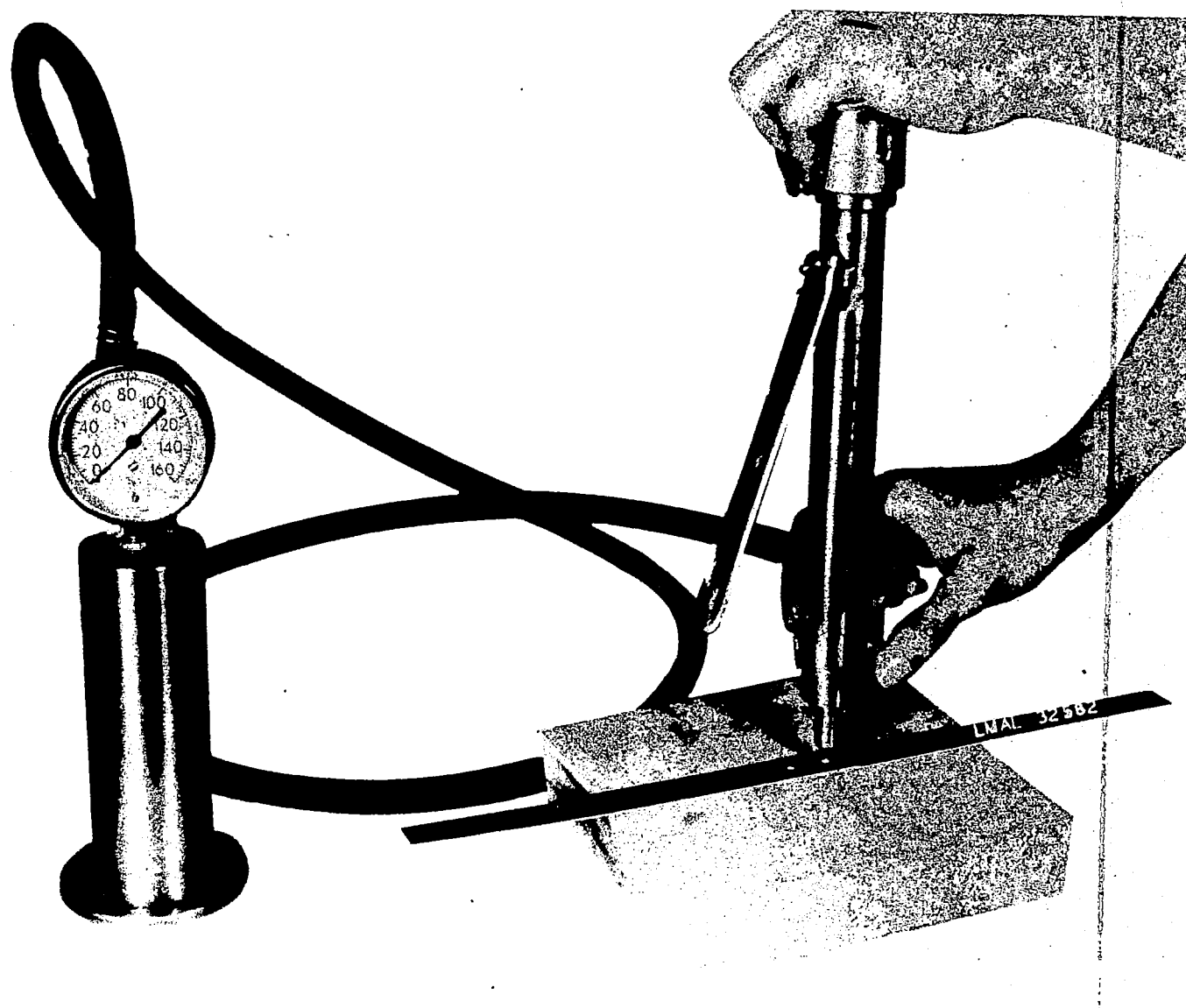
(a) Injection of oil into cavity of rivet.
