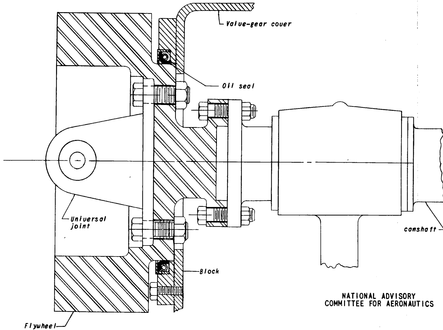
Figure 6. - Camshaft oil seal for Allison V-1710 block.
