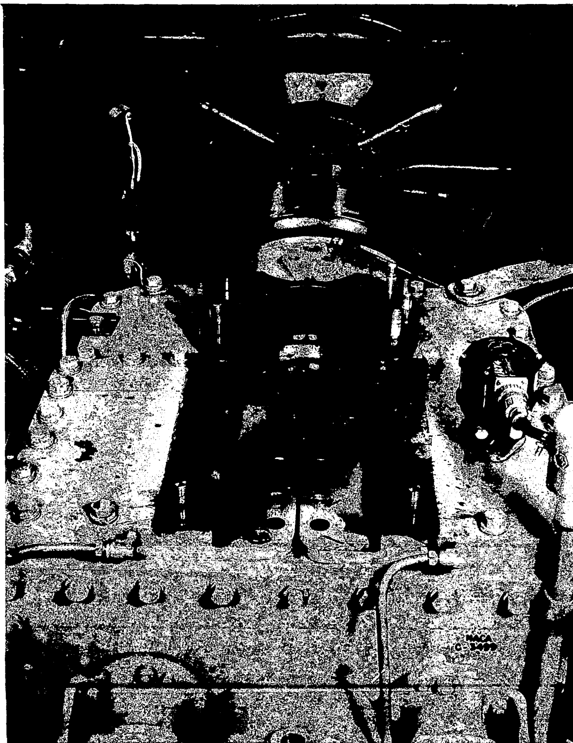
Figure 1. - CUE crankcase showing alterations to top plate.
