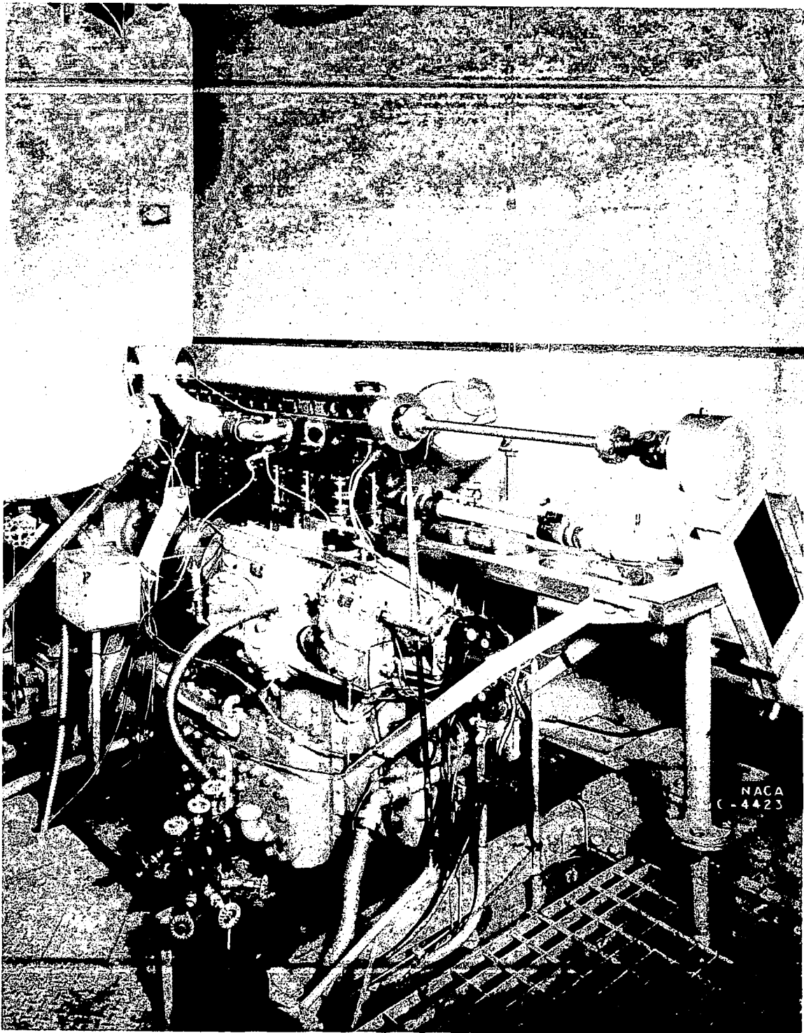
Figure 2. - CUE crankcase with Allison V-1710 block.
