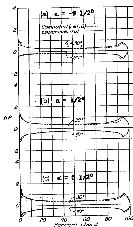
Figure 5.- Increments of resultant pressures for various angles of attack and various deflections of a 0.20cf tab on a 0.30c plain flap deflected 0^\circ .
