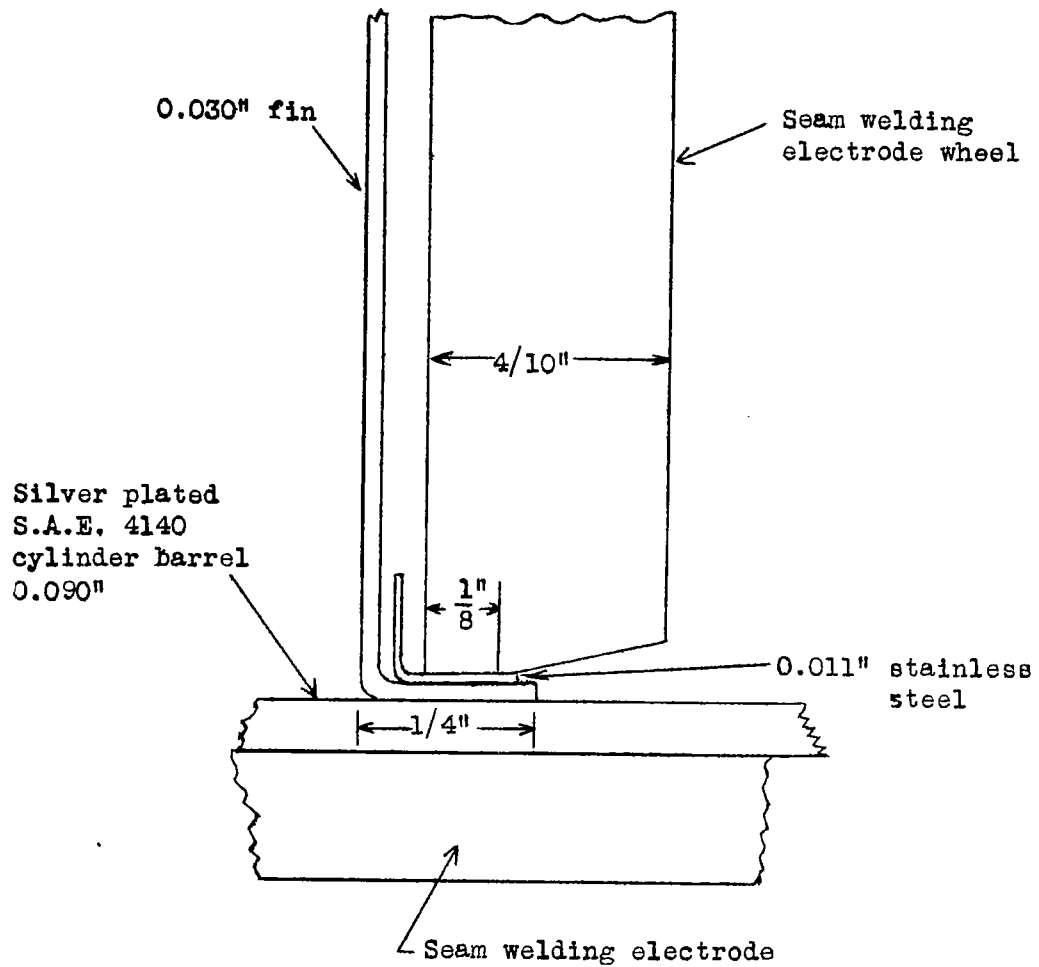
Figure 28.- Seam welding of fins to S.A.E. 4140 cylinder barrel.
