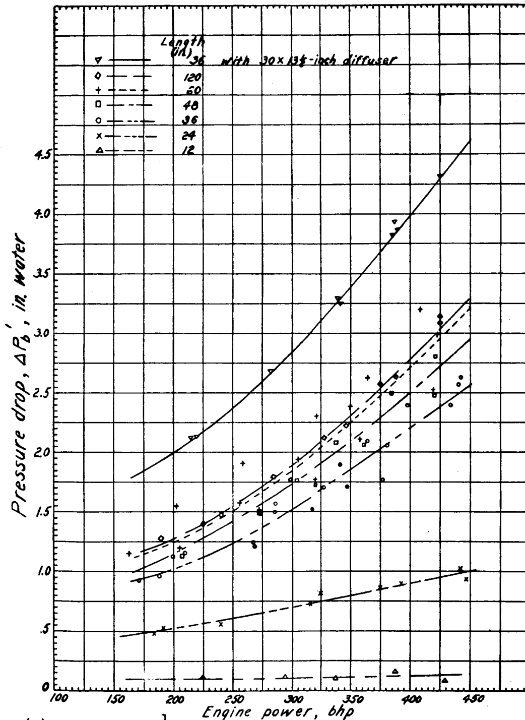
Figure 6. - Concluded. The effect of ejector length and diameter and engine power on cooling-air pressure drop for the grouped-ejector system.
