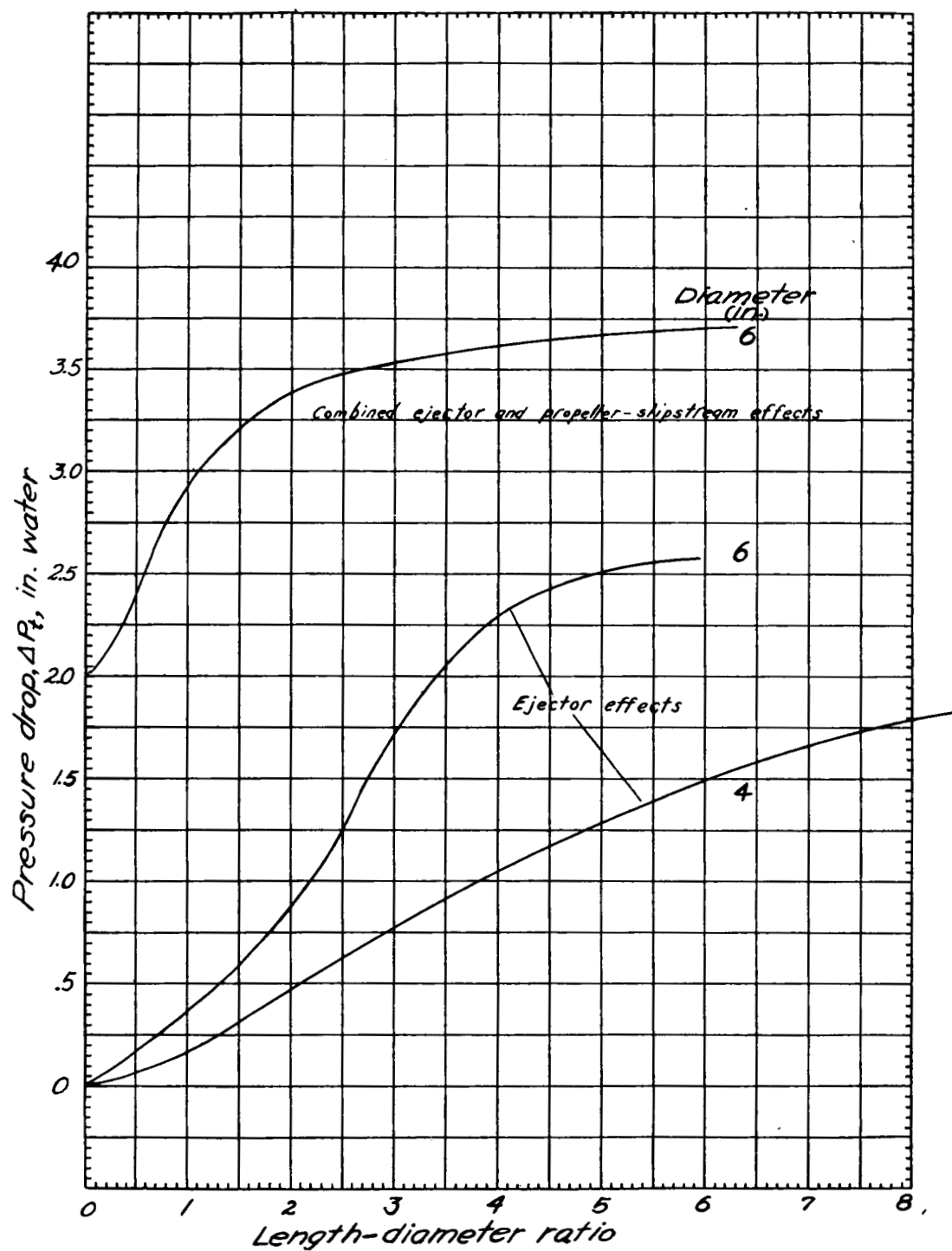
Figure 5. - The effect of length-diameter ratio on cooling-air pressure drop for individual-ejector system at 450 brake horsepower.
