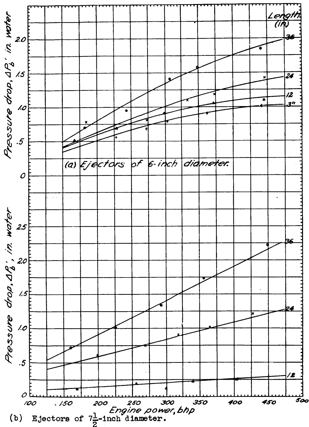
Figure 6. - The effect of ejector length and diameter and engine power on cooling-air pressure drop for the grouped-ejector system.
