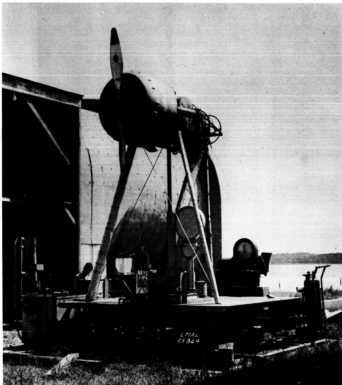
Figure 1. - The engine and outdoor test stand.
