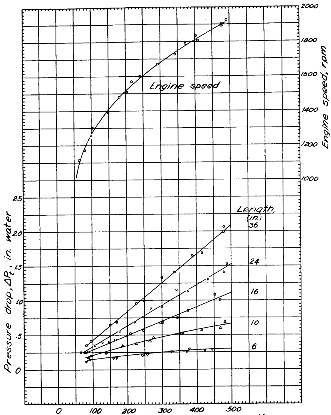
(a) Ejectors of 4-inch diameter. Engine power, bhp Figure 4. - The effect of ejector length and diameter and engine power on cooling-air pressure drop for the individual-ejector system.
