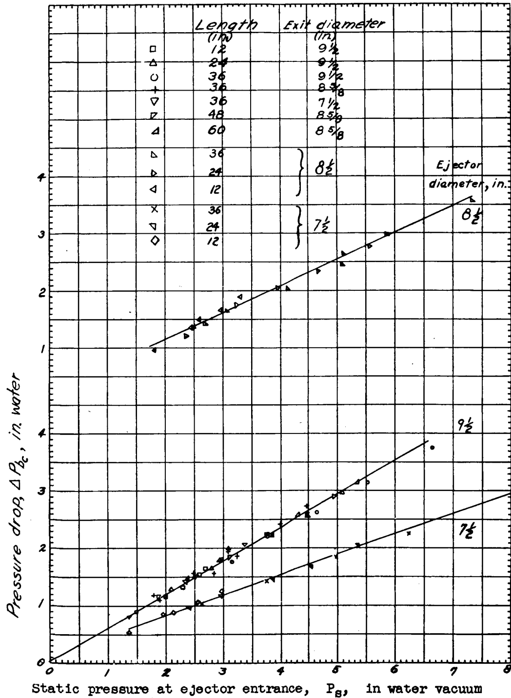
Figure 8. - The variation of pressure drop \Delta P_{b,c} with static pressure at ejector entrance P_s for the grouped ejectors. c
