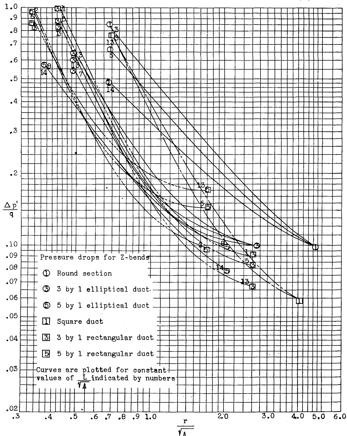
Figure 31.—Net pressure drop against radius of curvature for Z-bends.
