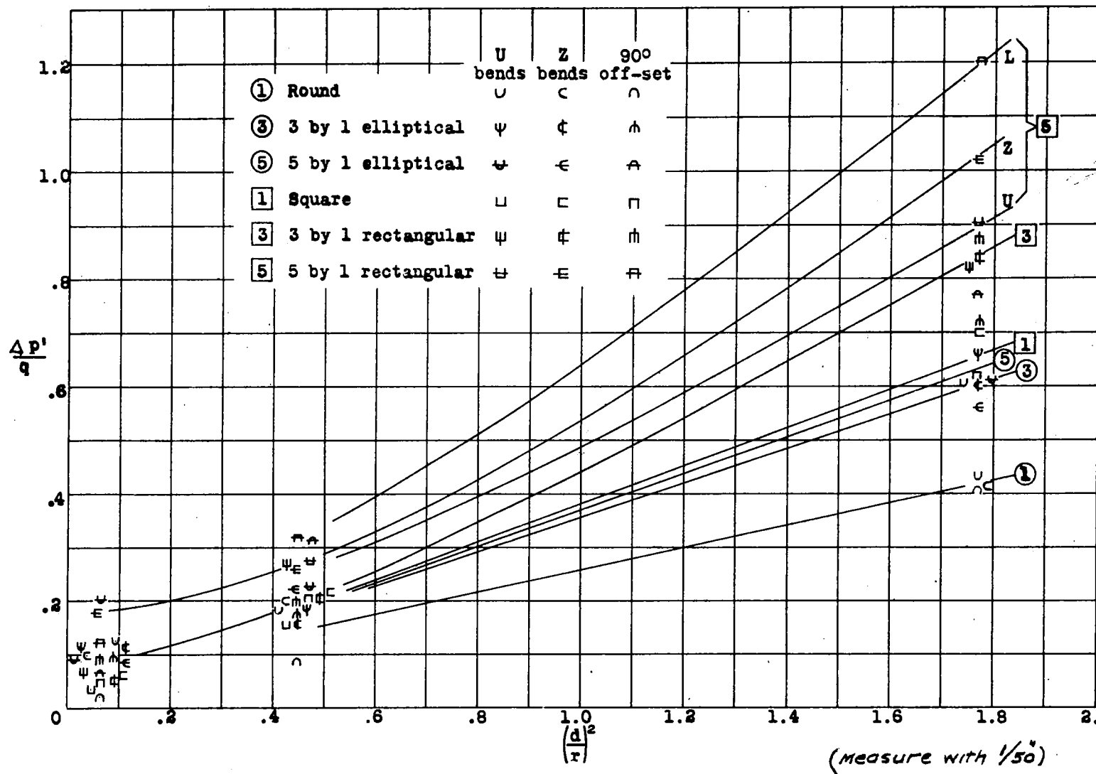
Figure 29.- Variation of net pressure drop with radius of curvature for compound bends with maximum spacer.
