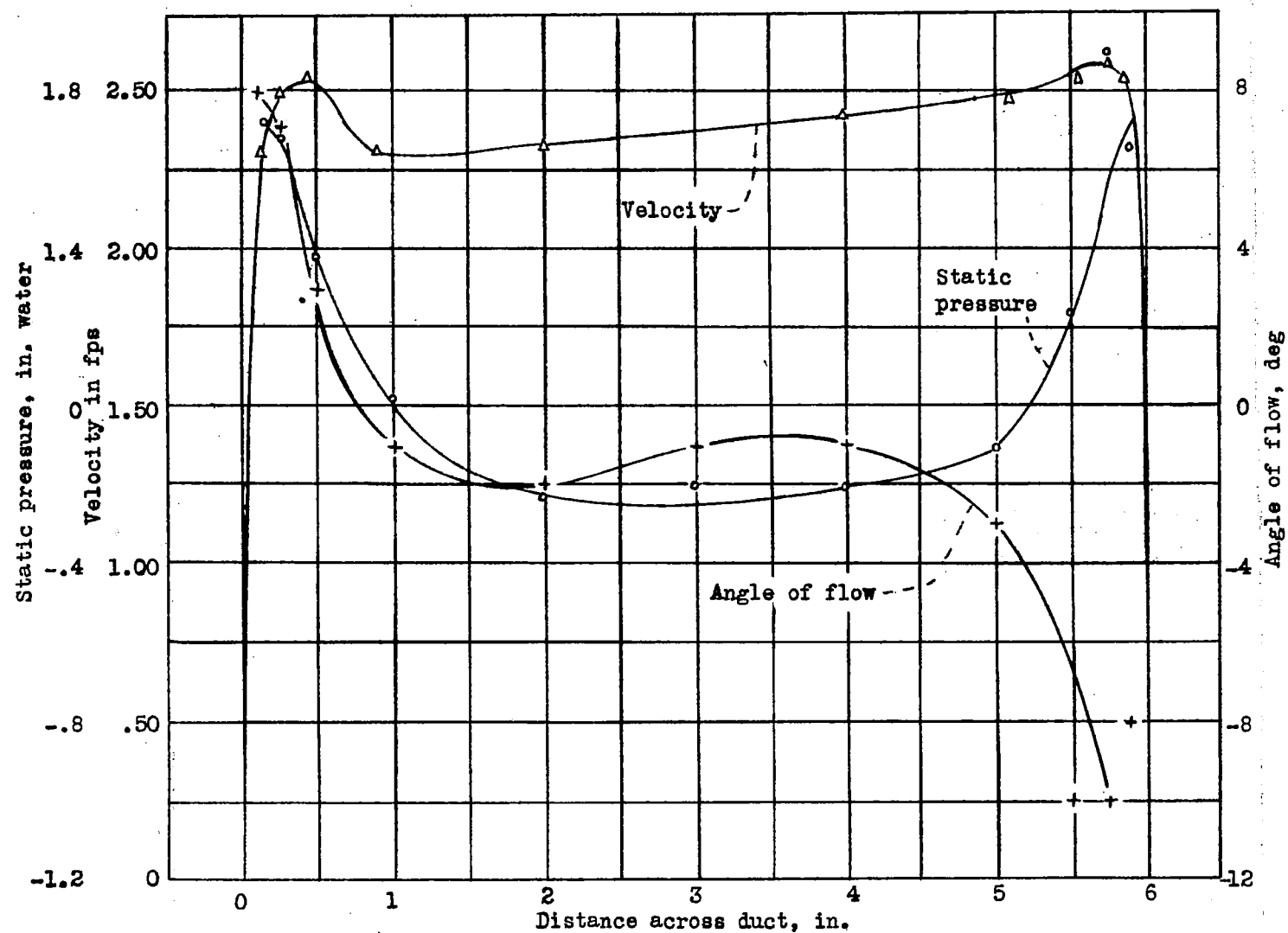
Figure 37.- Surveys at outlet of 90°-offset bend; r = 9 inches; line of survey normal to plane of second elbow.
