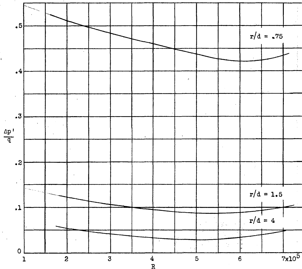
Figure 22.- Variation of net pressure drop with Reynolds number for single bends in 3 by 1 rectangular ducts.
