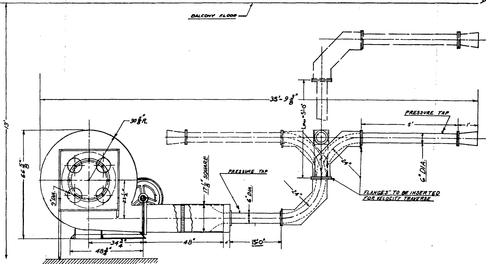
Figure 1(a,b):-Drawing of test set-up.
