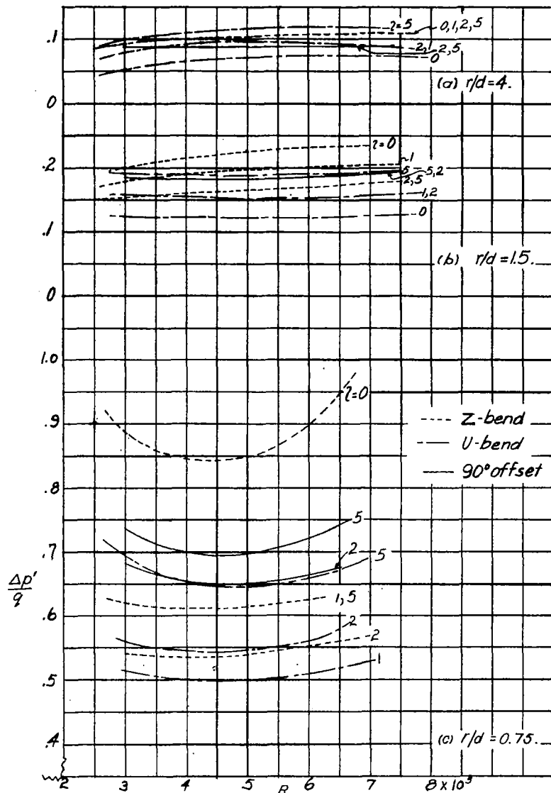
Figure 17.—Variation of net pressure drop with Reynolds number for compound bends in 3 by 1 elliptical ducts.
