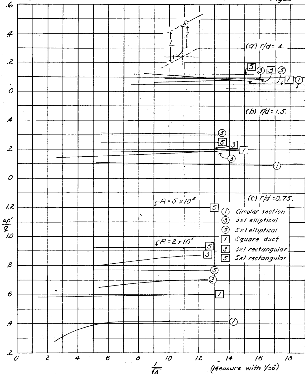
Figure 28.— Variation of net pressure drop with length of spacer for compound 90°-offset bends.
