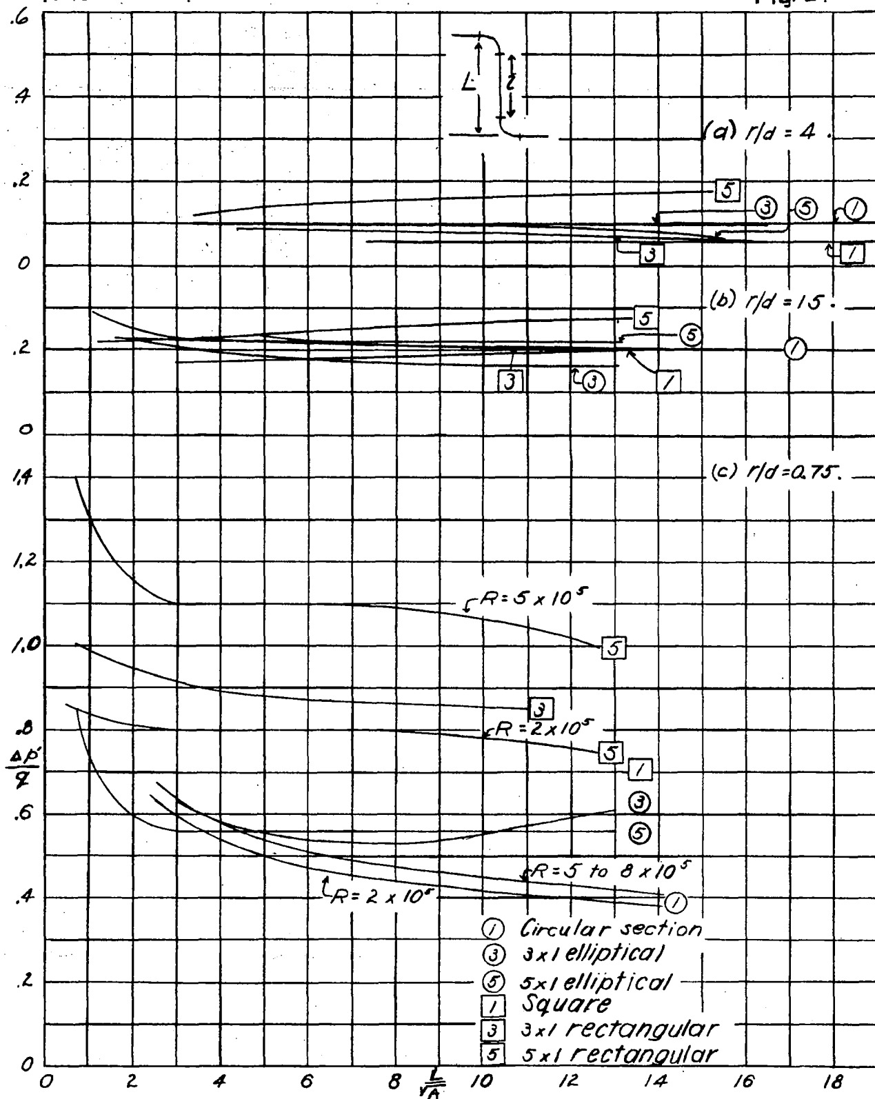
Figure 27.- Variation of net pressure drop with length of spacer for compound Z-bends. (Measure with 1/30^\circ )
