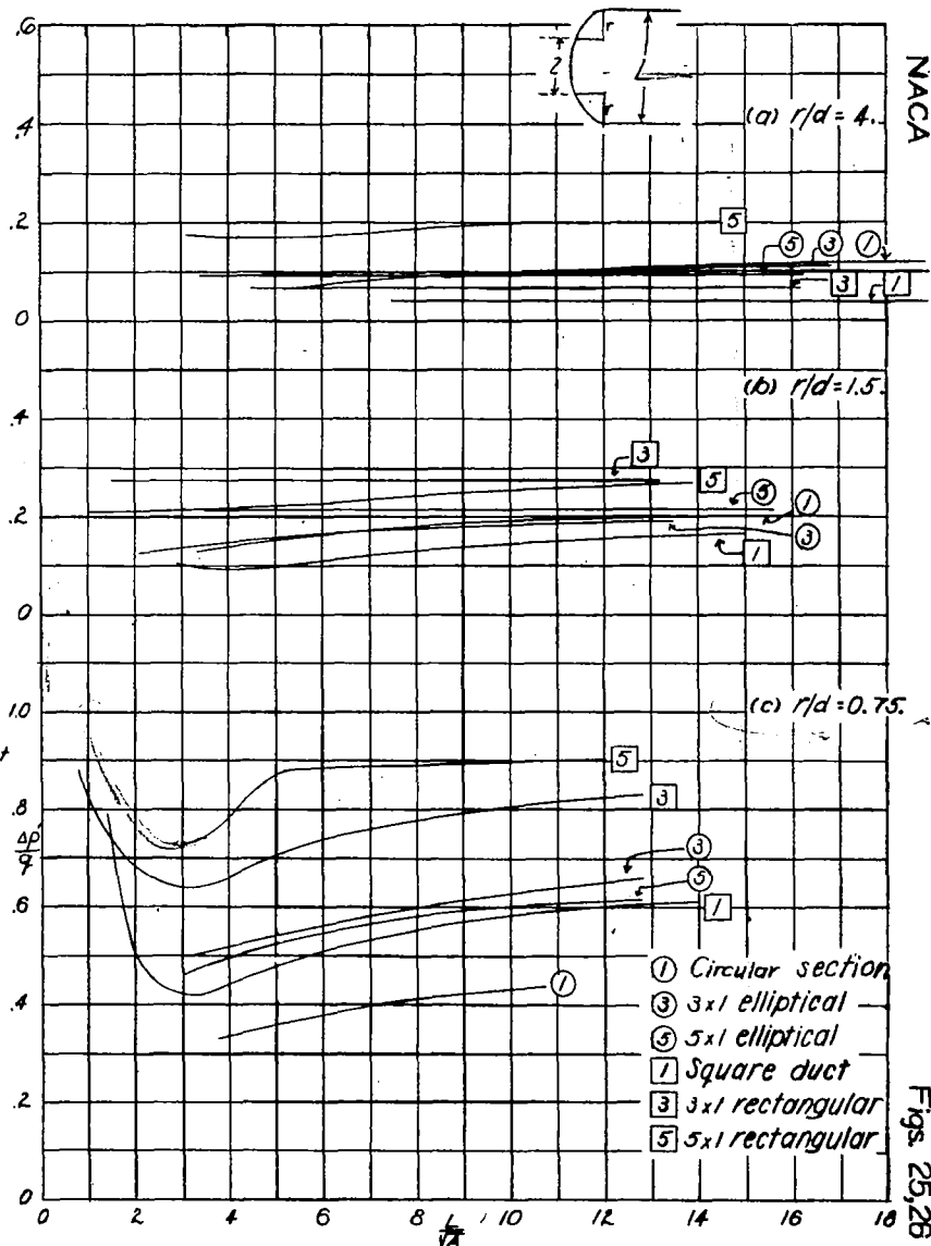
Figure 26.—Variation of net pressure drop with length of spacer for compound U-bends.
