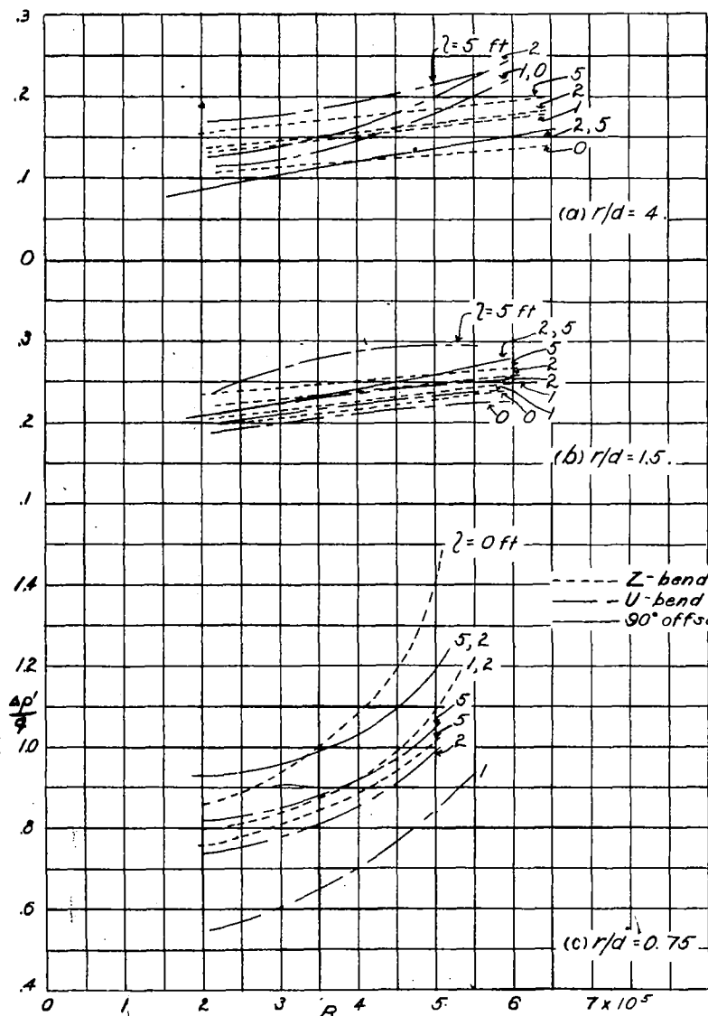
Figure 25.—Variation of net pressure drop with Reynolds number for compound bends in 5 by 1 rectangular ducts. (Measure with K_{90} )
