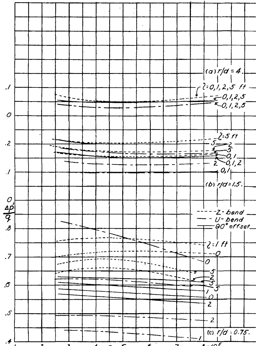
Figure 21.—Variation of net pressure drop with Reynolds number for compound bends in square ducts. (Measure with 1/20 )
