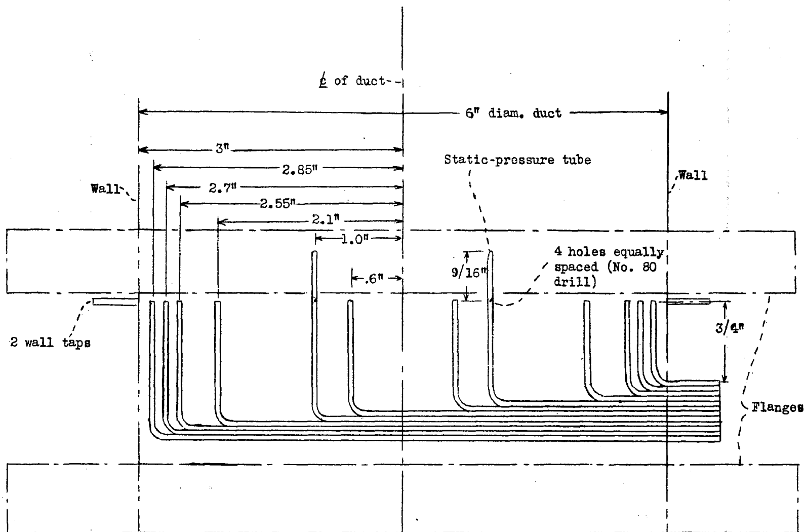
Figure 6.- Location of total- and static-pressure tubes of traversing head.
