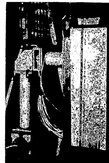
Figure 5.- Duct install- ation for test of 90° offset bend show- ing traversing head and multiple tube manometer.
