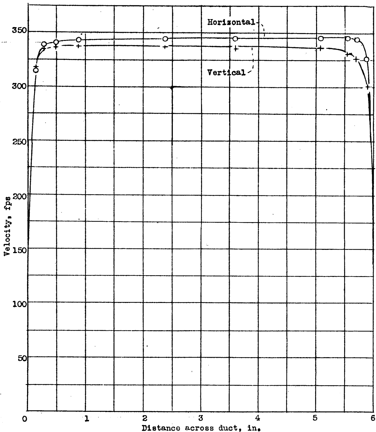
Figure 11.- Velocity traverse at the outlet of the 6-inch-diameter nozzle.
