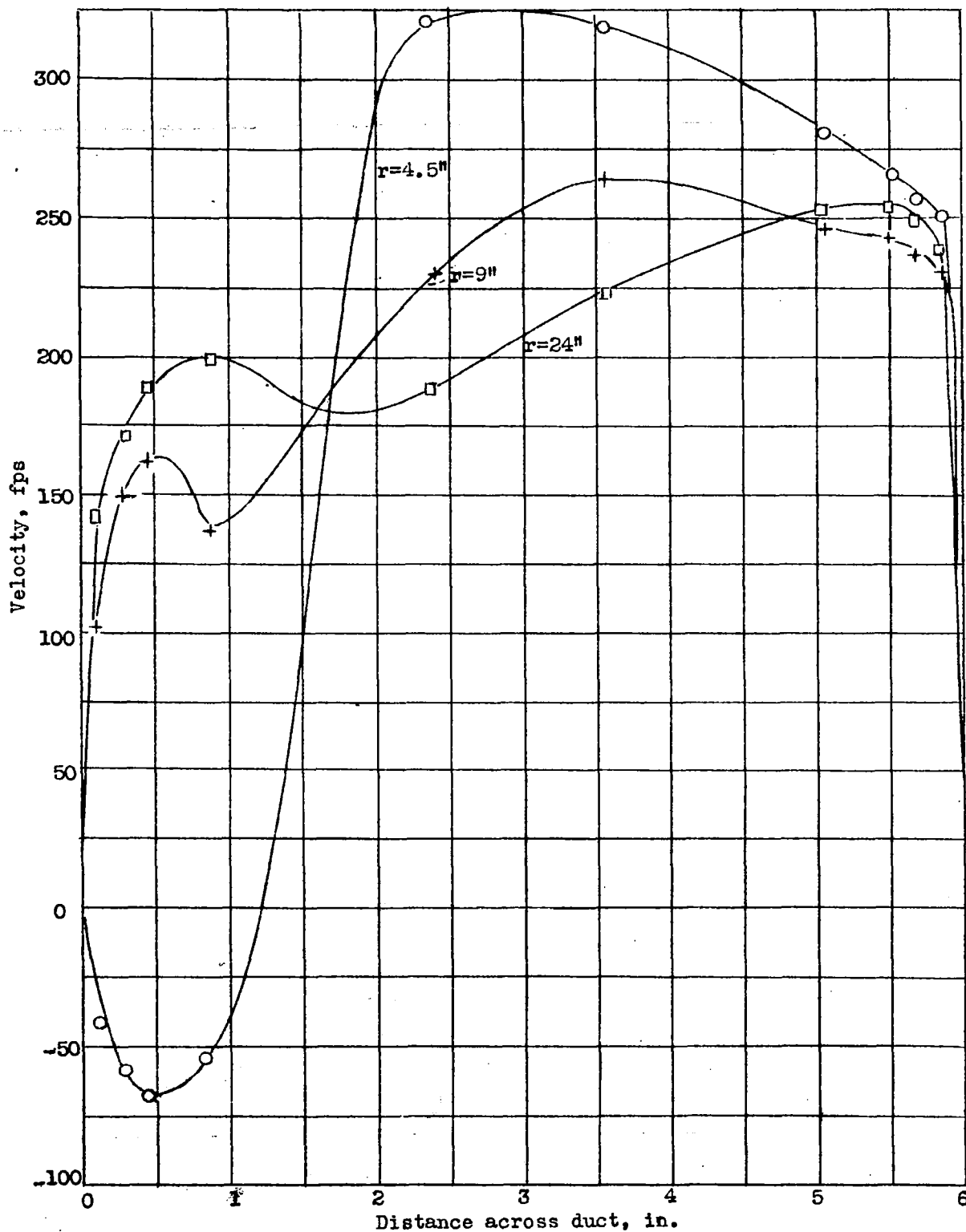
Figure 33.- Velocity distribution downstream of single elbow in plane of curvature.
