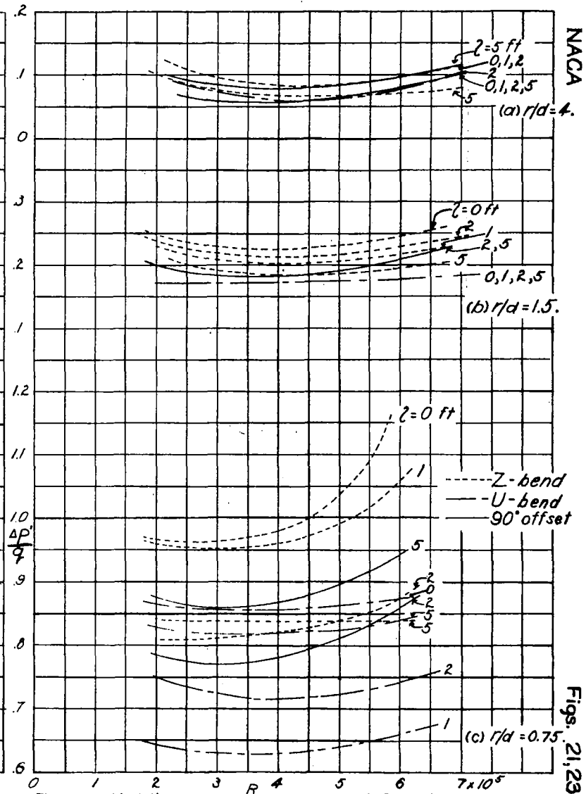
Figure 23.—Variation of net pressure drop with Reynolds number for compound bends in 3 by 1 rectangular ducts. (Measure with 1/20 )
