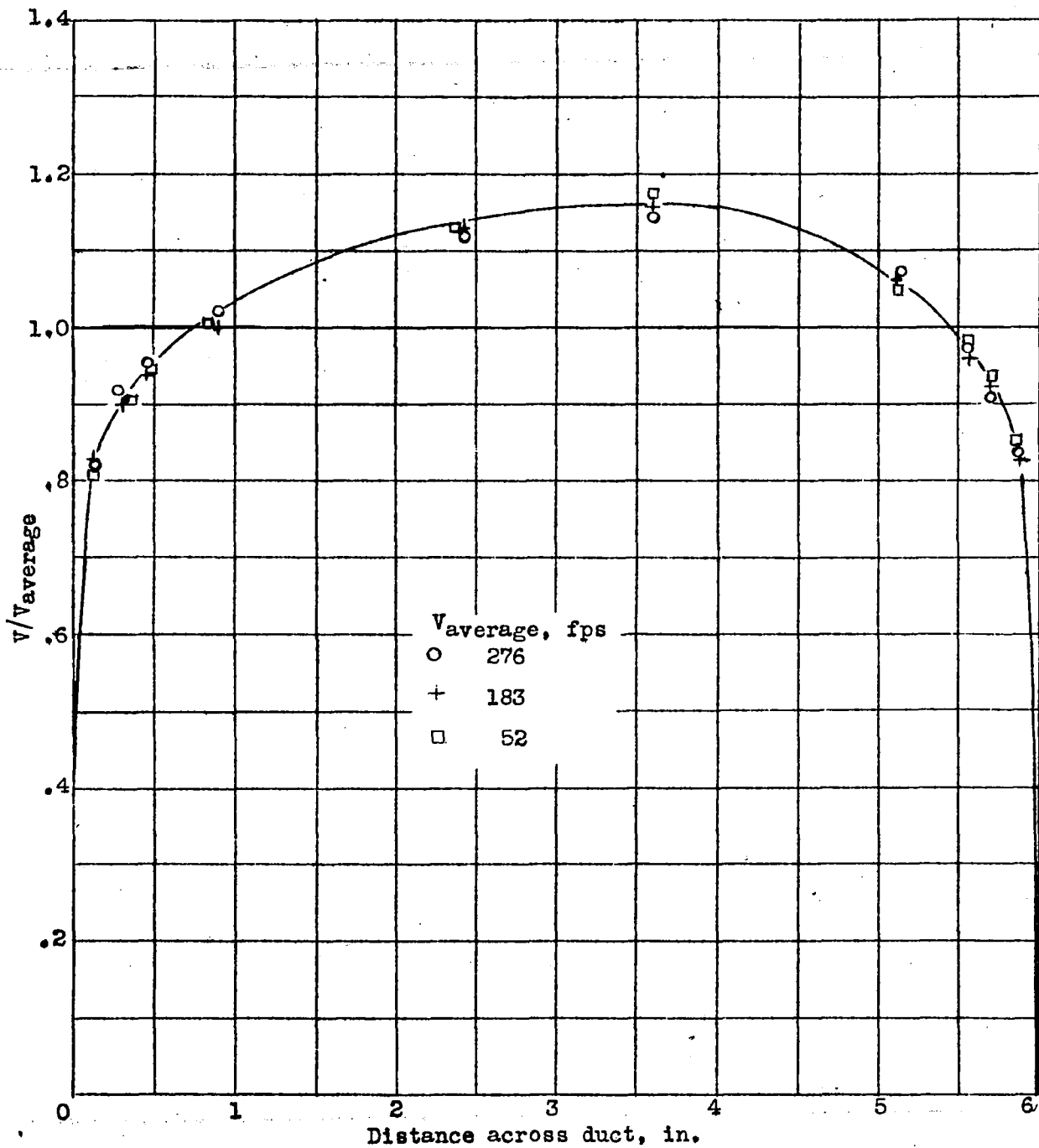
Figure 12.- Velocity traverses at inlet of the first elbow.
