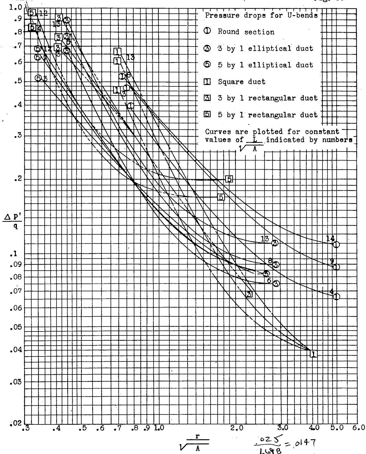
Figure 30.- Net pressure drop against radius of curvature for U-bends.
