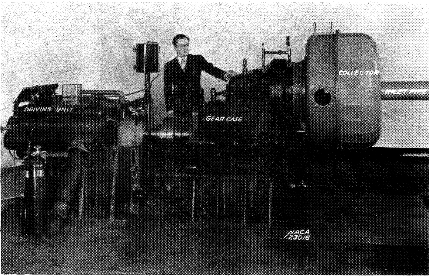
Figure 5 - Side view of variable-component supercharger test rig.
