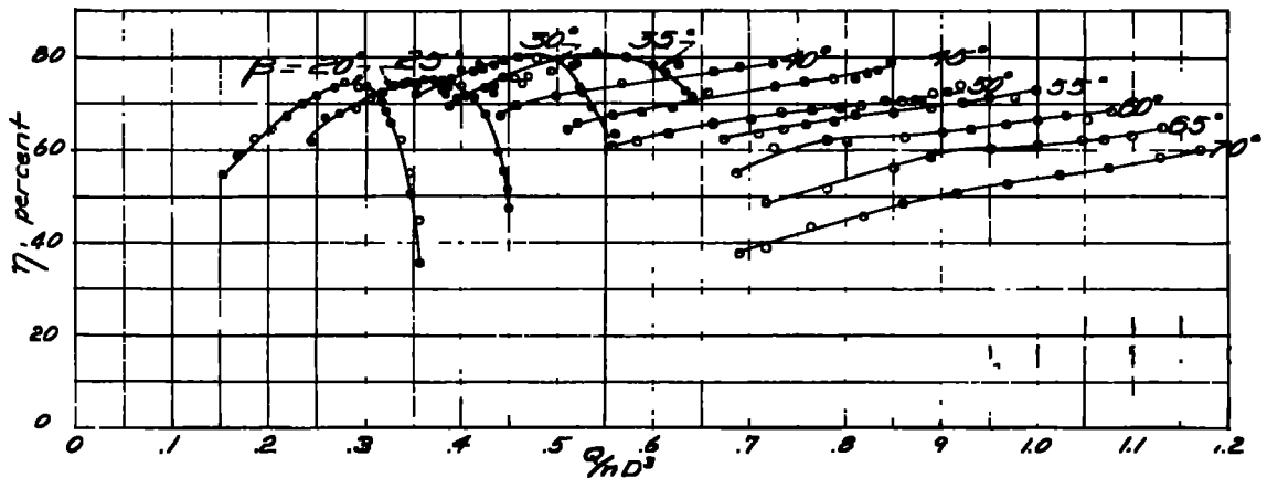
Figure 42.—Axial-fan efficiencies. B, 24 ; no contravanes; R.A.F. 6 blade section.
