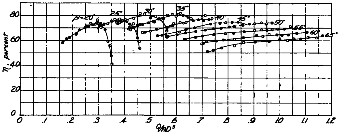
Figure 45.—Axial-fan efficiencies; No contravanes; B, 24 ; NACA 6412 blade section.
