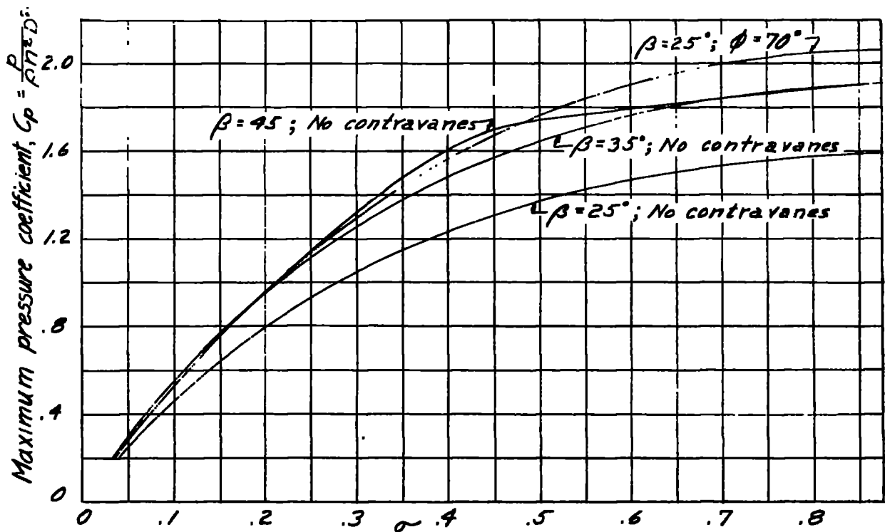
Figure 32.- Maximum pressure coefficients.
