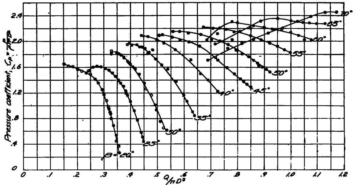
Figure 40.—Pressure coefficients. B, 24 ; no contravanes; R.A.F. 6 blade section.
