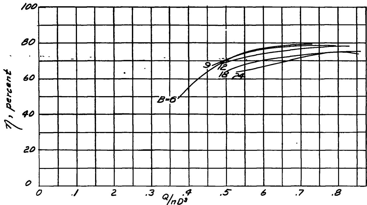
Figure 31.- Efficiencies at various solidities.
