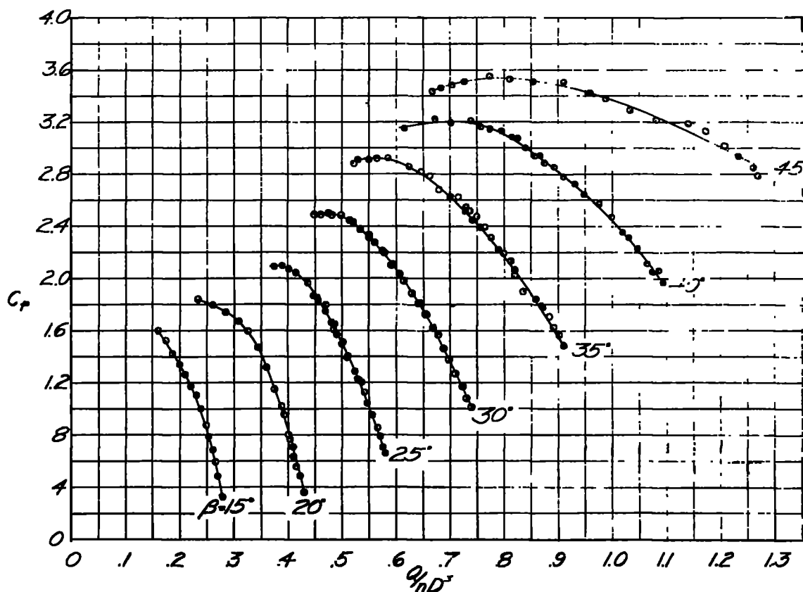
Figure 46.- Pressure coefficients. \phi, 70; B, 24 ; NACA 6912 blade section.
