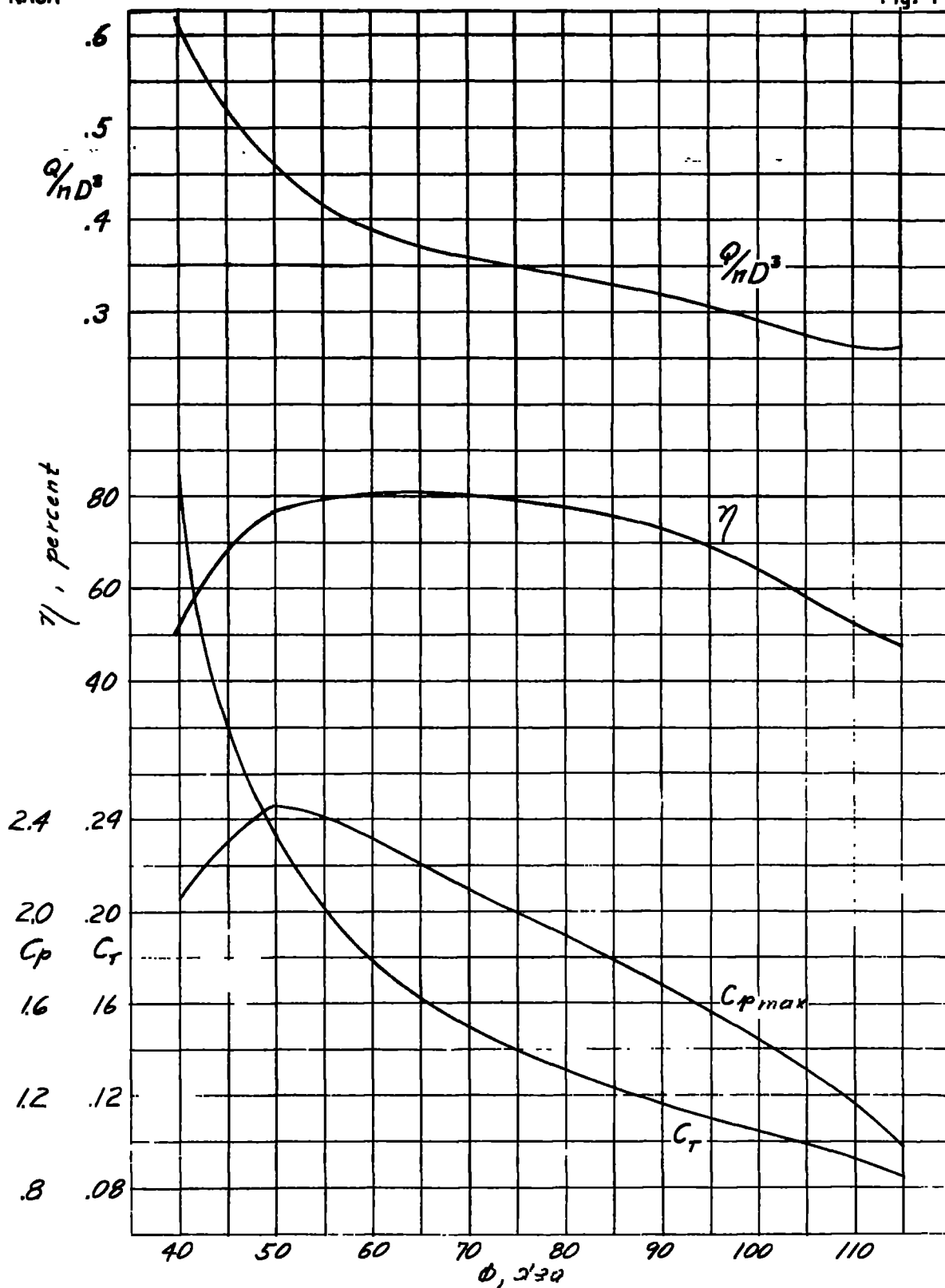
Figure 7.-- Fan characteristics for maximum pressure coefficient. \beta, 25^\circ ; \beta, 24^\circ ; R.A.F. 6 blade section.
