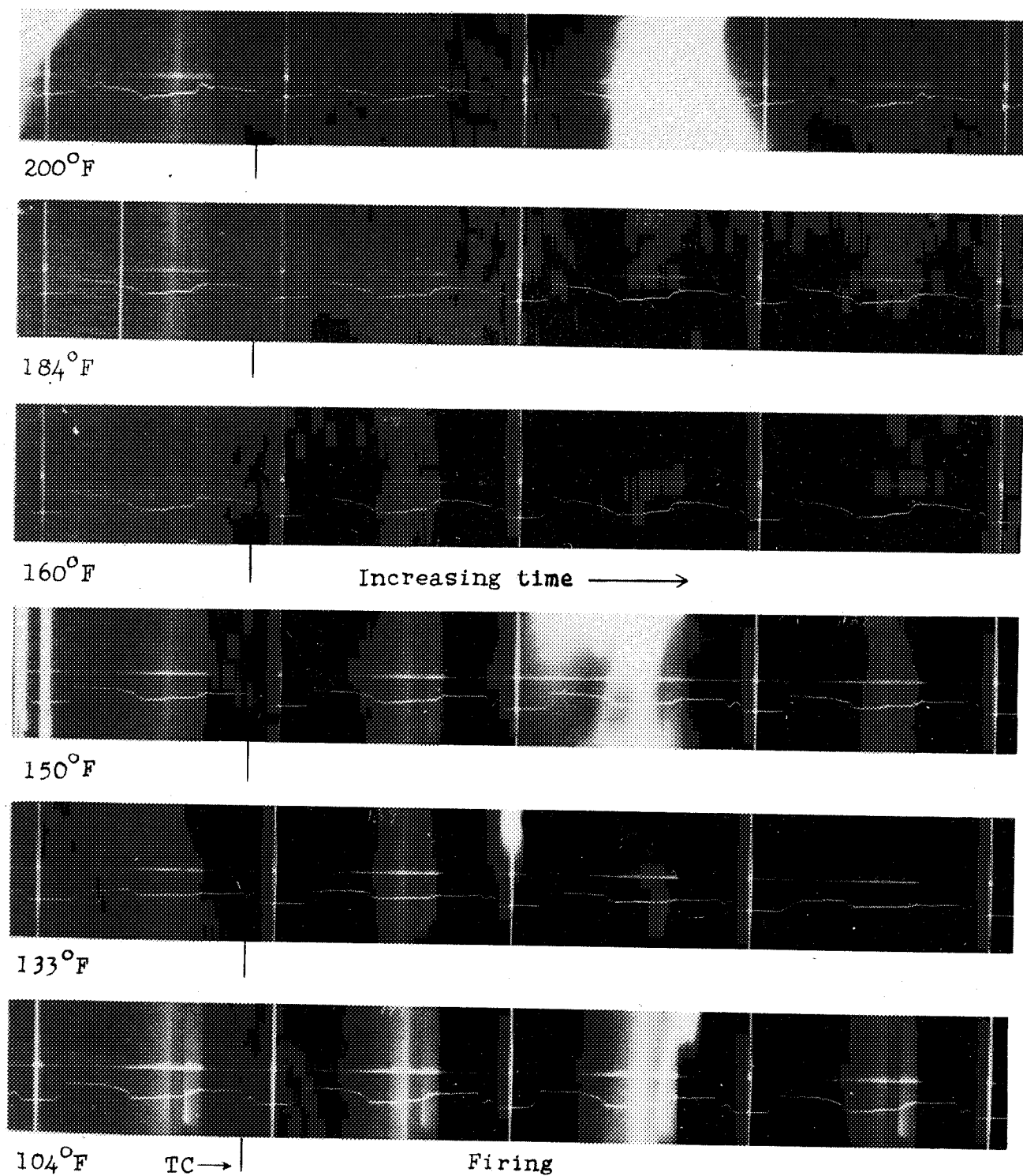
Figure 18b.- Cylinder sleeve displacement as a function of common oil and cylinder sleeve cooling water temperatures. SAE 20 oil. Speed 1800 rpm.
