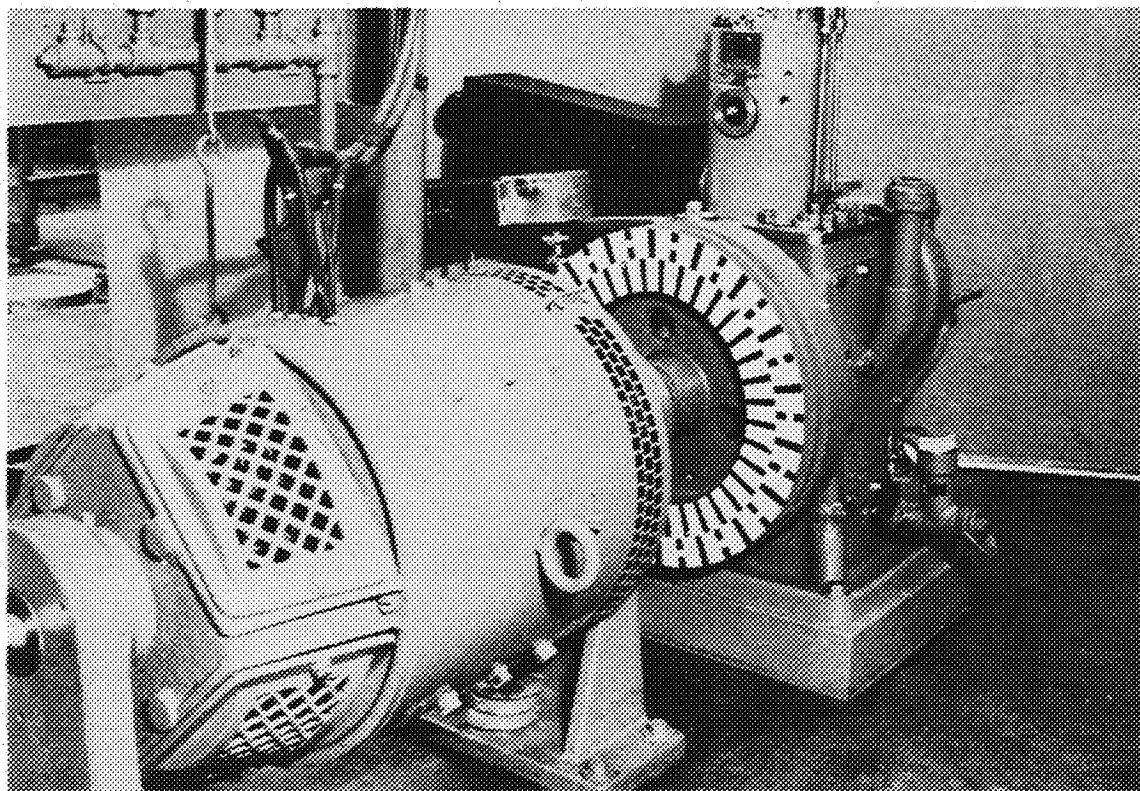
Figure 3.- Dynamometer end of friction engine.
