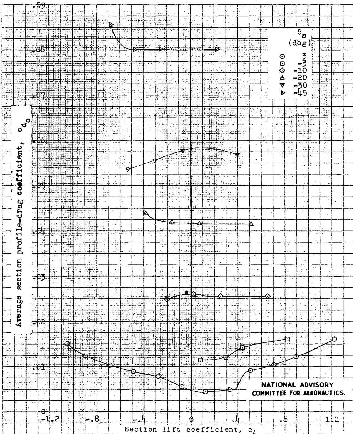
Figure 18.- Average section profile-drag characteristics over a 20-inch-span section of the spoiler aileron flap model for the Hughes XF-11 airplane. Configuration number 9; \delta_f = 0^\circ ; R = 6.0 \times 10^6 ; TDT test 799.
