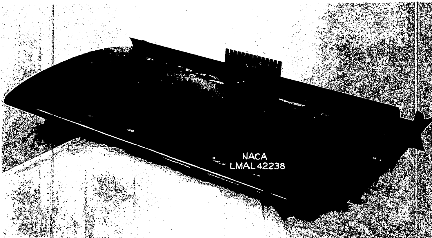
(a) Three-quarter front view of model showing the spoiler webs.
