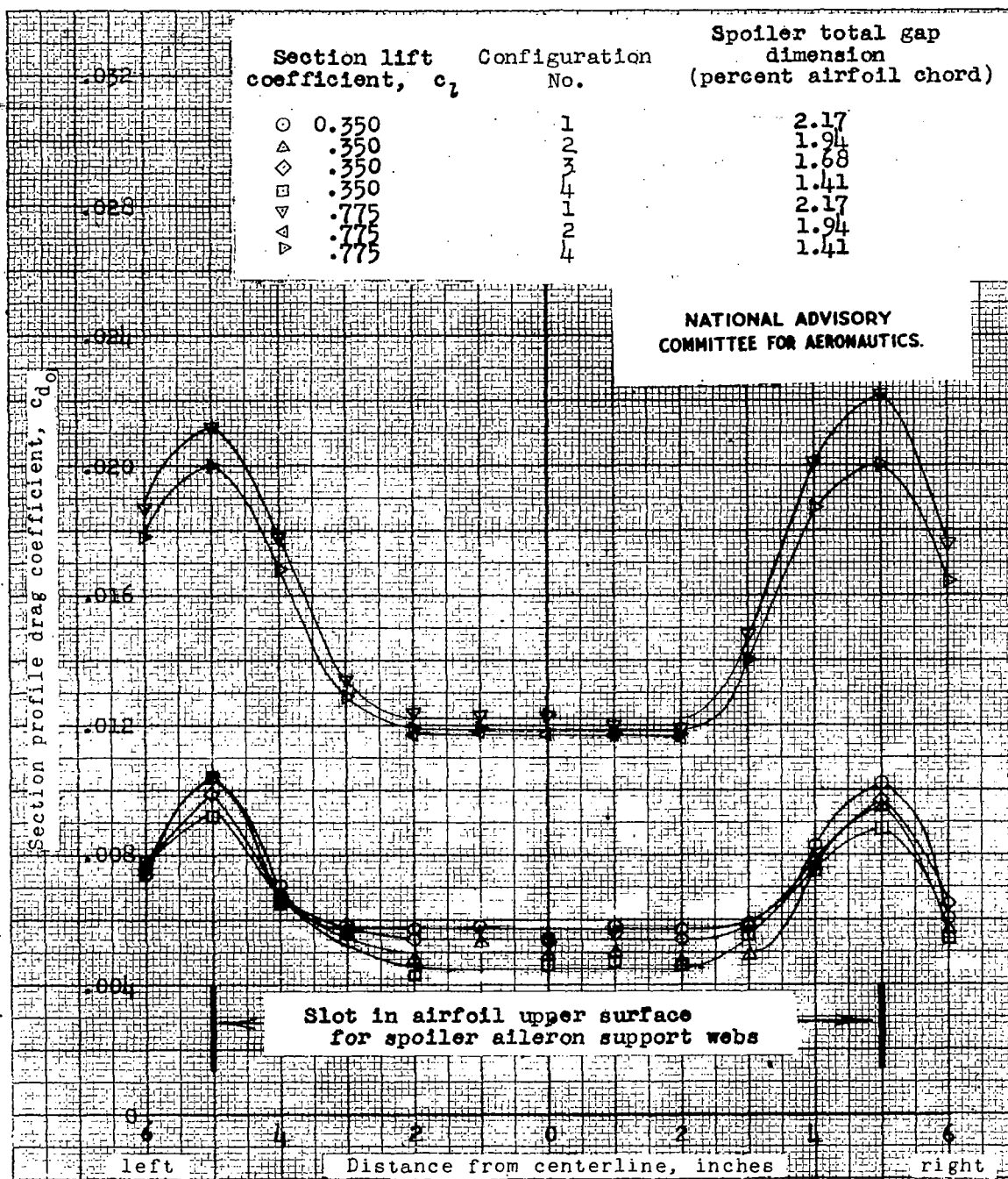
Figure 16.- Spanwise variation of the profile drag coefficient with spoiler rear-gap dimension for the spoiler aileron flap model for the Hughes XF-11 airplane. \delta_s = \delta_f = 0^\circ ; R = 2.5 \times 10^6 ; LTT test 392.
