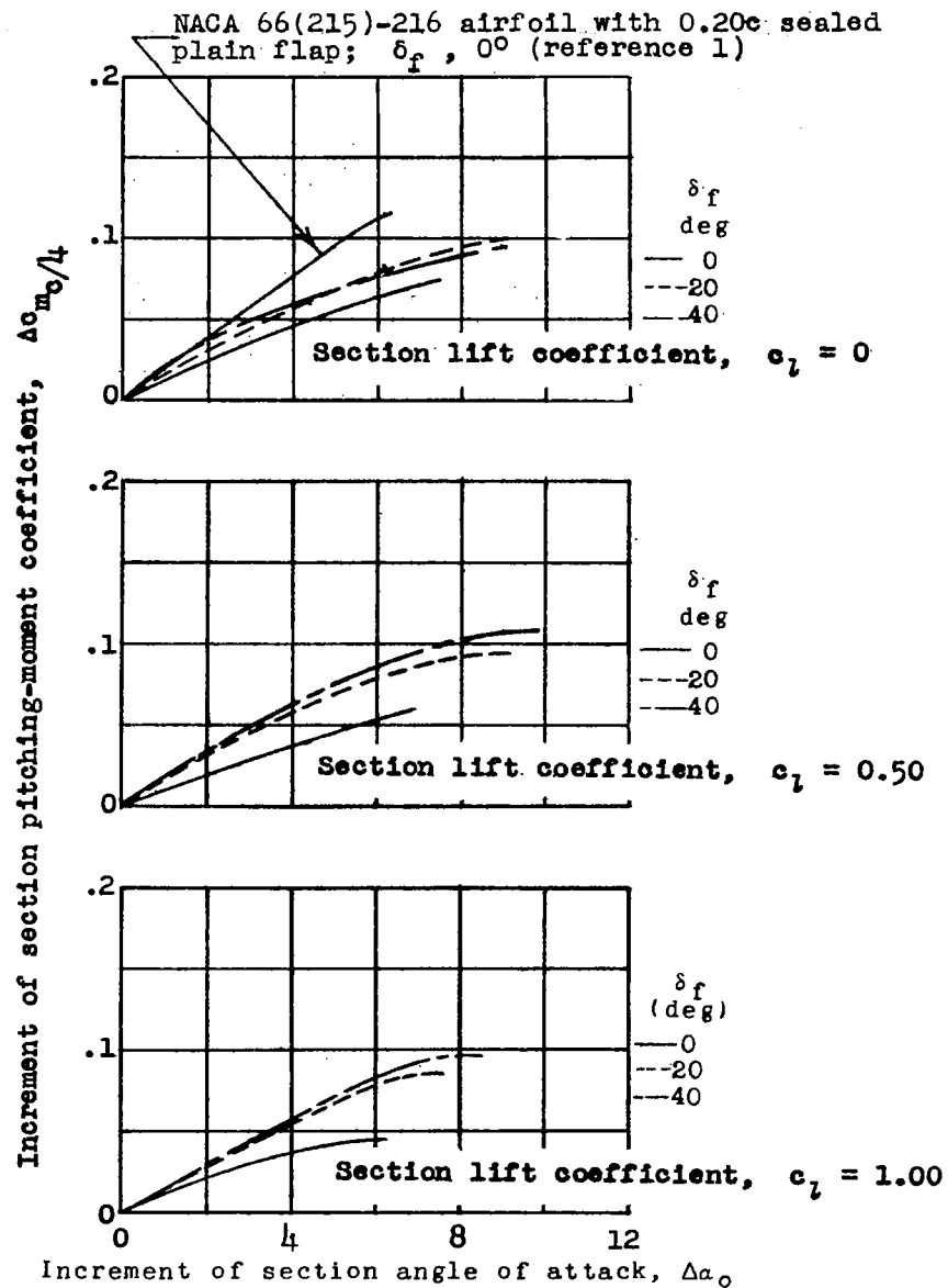
Figure 20.- Variation of the increment of section pitching-moment coefficient with the increment of section angle of attack for the spoiler aileron flap model for the Hughes XF-11 airplane. Configuration number 9.
