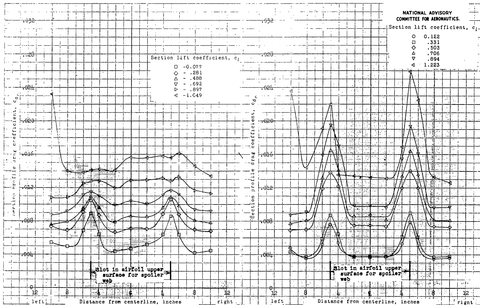
Figure 17.- Spanwise variation of the section profile-drag coefficient for the spoiler aileron flap model for the Hughes XF-11 airplane. Configuration number 9; \delta_s = 3^\circ ; \delta_f = 0^\circ ; R = 6.0 \times 10^6 ; TDT test 799.
