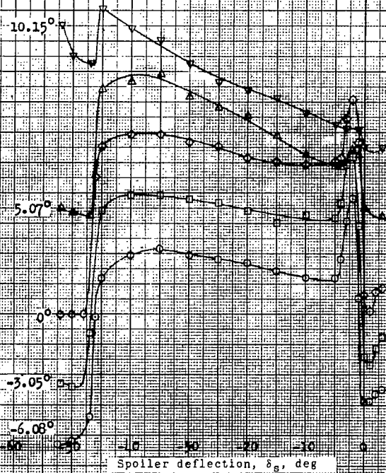
(b) \delta_f = 20^\circ . Figure 10.- Continued.
