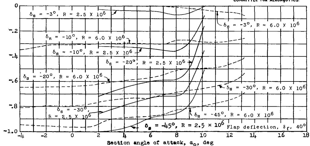
Figure 12.- Variation of the increment of section lift coefficient with section angle of attack for the spoiler flap model for the Hughes XF-11 airplane. Configuration number 9.
