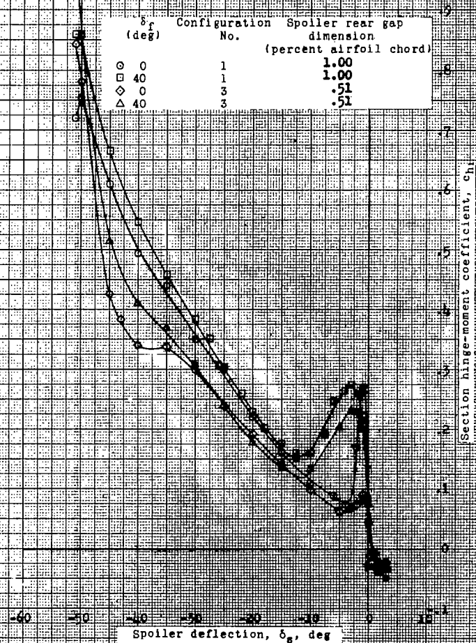
(b) \alpha_0 = 7.11^\circ . Figure 7.- Concluded.
