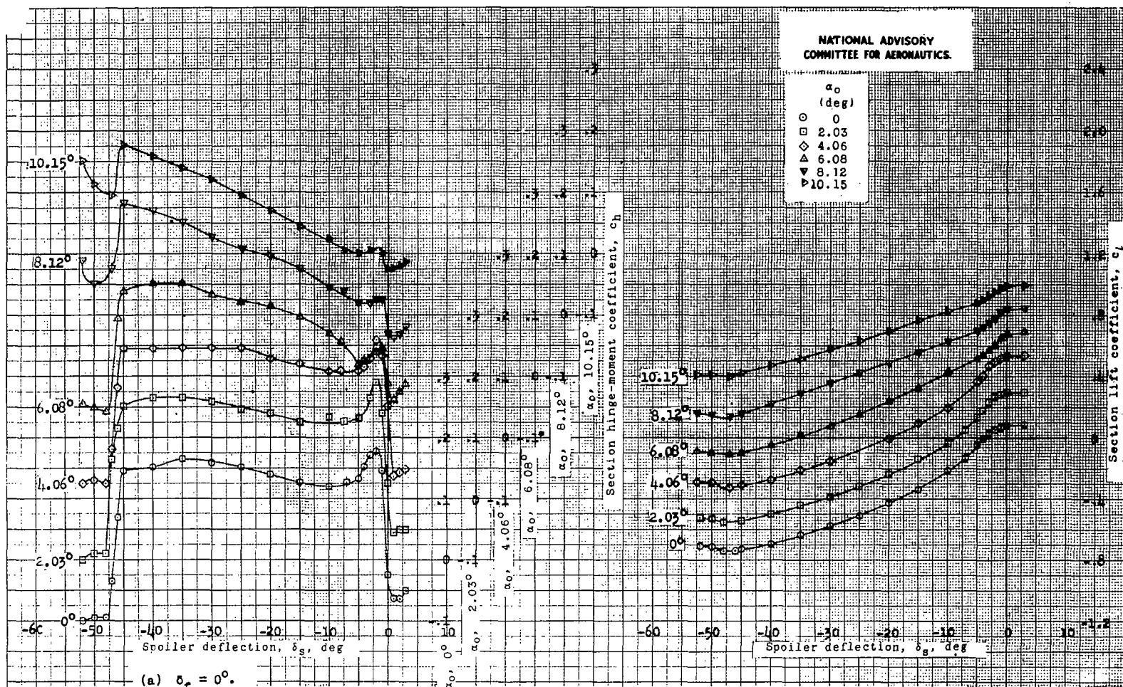
Figure 10.- Section hinge-moment and lift characteristics for the spoiler aileron flap model for the Hughes XF-11 airplane. Configuration number 9; R = 2.5 \times 10^6 ; LTT test 393.
