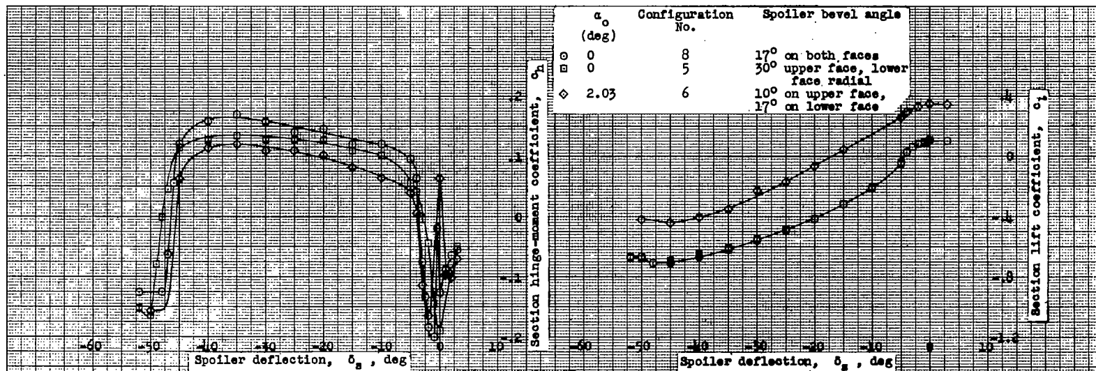
Figure 8.- The effect of spoiler bevel angle on the section hinge-moment and lift characteristics of the spoiler aileron flap model for the Hughes XF-11 airplane. Spoiler upper face smooth; \delta_p = 0^\circ ; R = 2.5 \times 10^6 ; LTT test 392.
