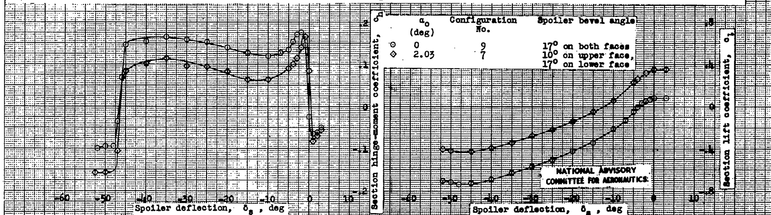
Figure 9.- Section hinge-moment and lift characteristics for the spoiler aileron flap model for the Hughes XF-11 airplane. Spoiler upper face rough; \delta_p = 0^\circ ; R = 2.5 \times 10^6 ; LTT test 392.
