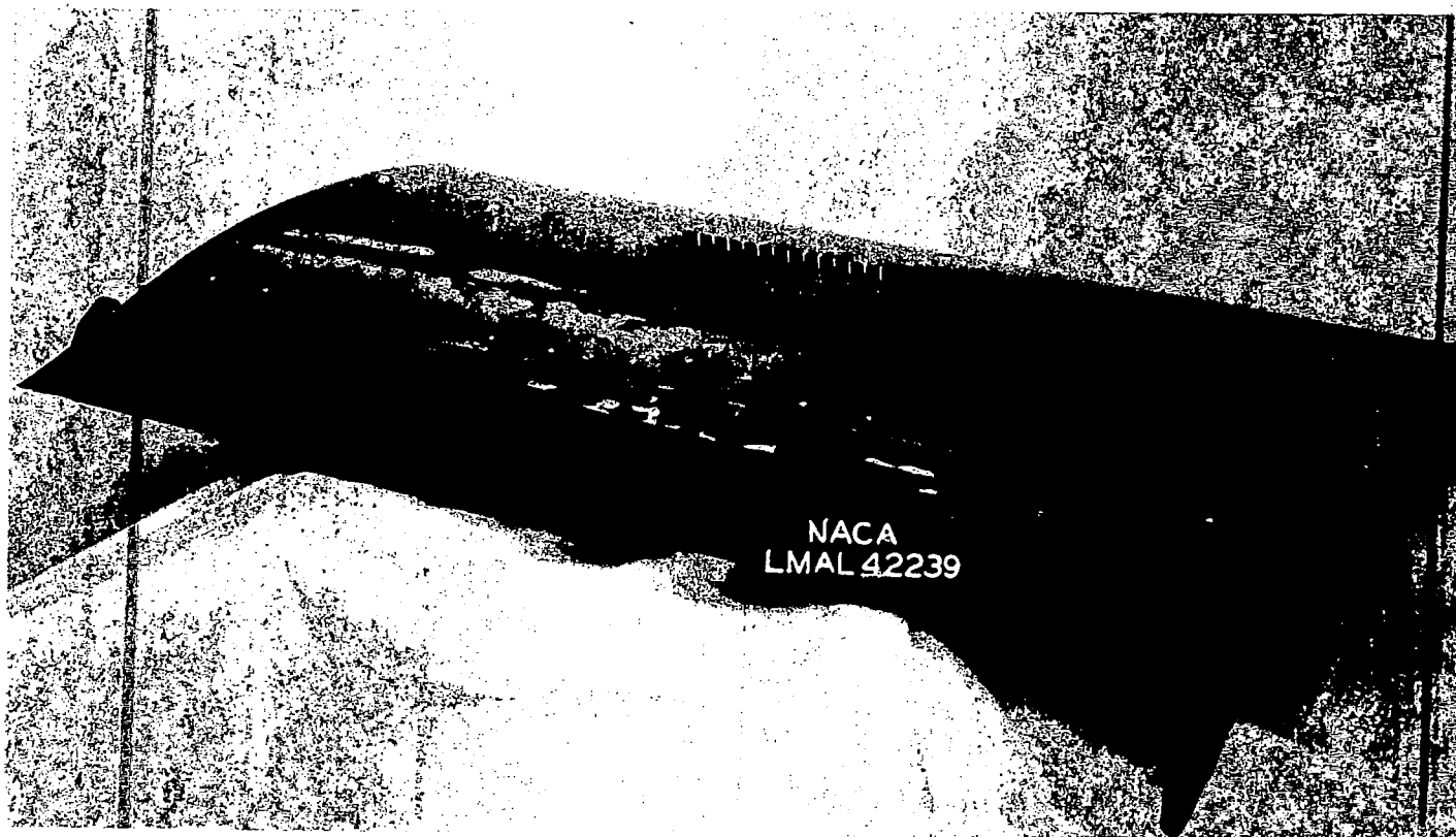
(c) Three-quarter top view of model showing the spoiler aileron slots in the airfoil upper surface.
