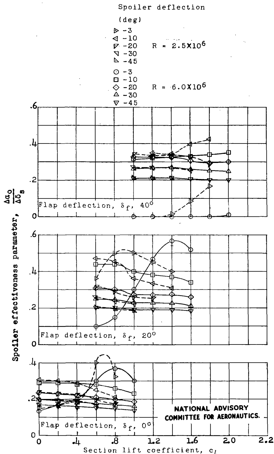
Figure 15.- Variation of spoiler effectiveness parameter, \frac{\Delta \alpha_o}{\Delta \delta_s} , with section lift coefficient for the spoiler aileron flap model for the Hughes XF-11 airplane. Configuration number 9.
