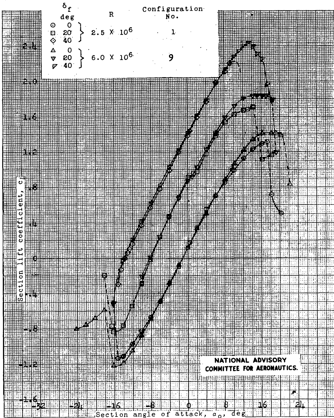
Figure 14.- Variation of section lift coefficient with Reynolds number for flap deflections of 0^\circ , 20^\circ , and 40^\circ . Spoiler aileron flap model for the Hughes XF-11 airplane. \delta_s = 3^\circ .
