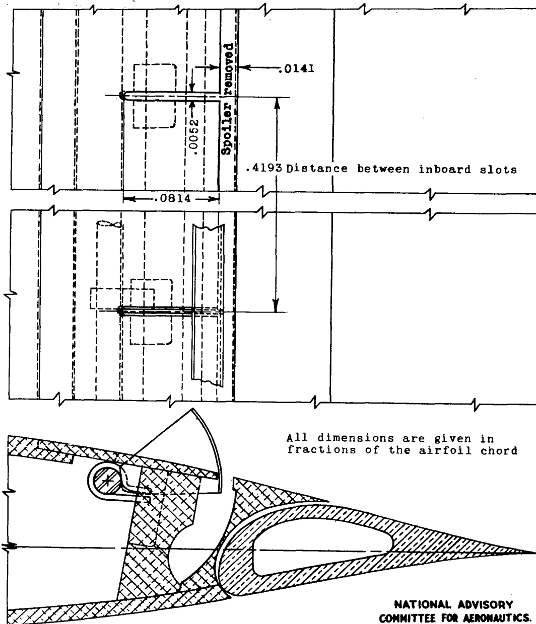
Figure 4.- Sketch showing the chordwise slots in the airfoil upper surface for the spoiler webs for the 0.28-percent airfoil chord spoiler. Spoiler aileron flap model for the Hughes XF-11 airplane.
