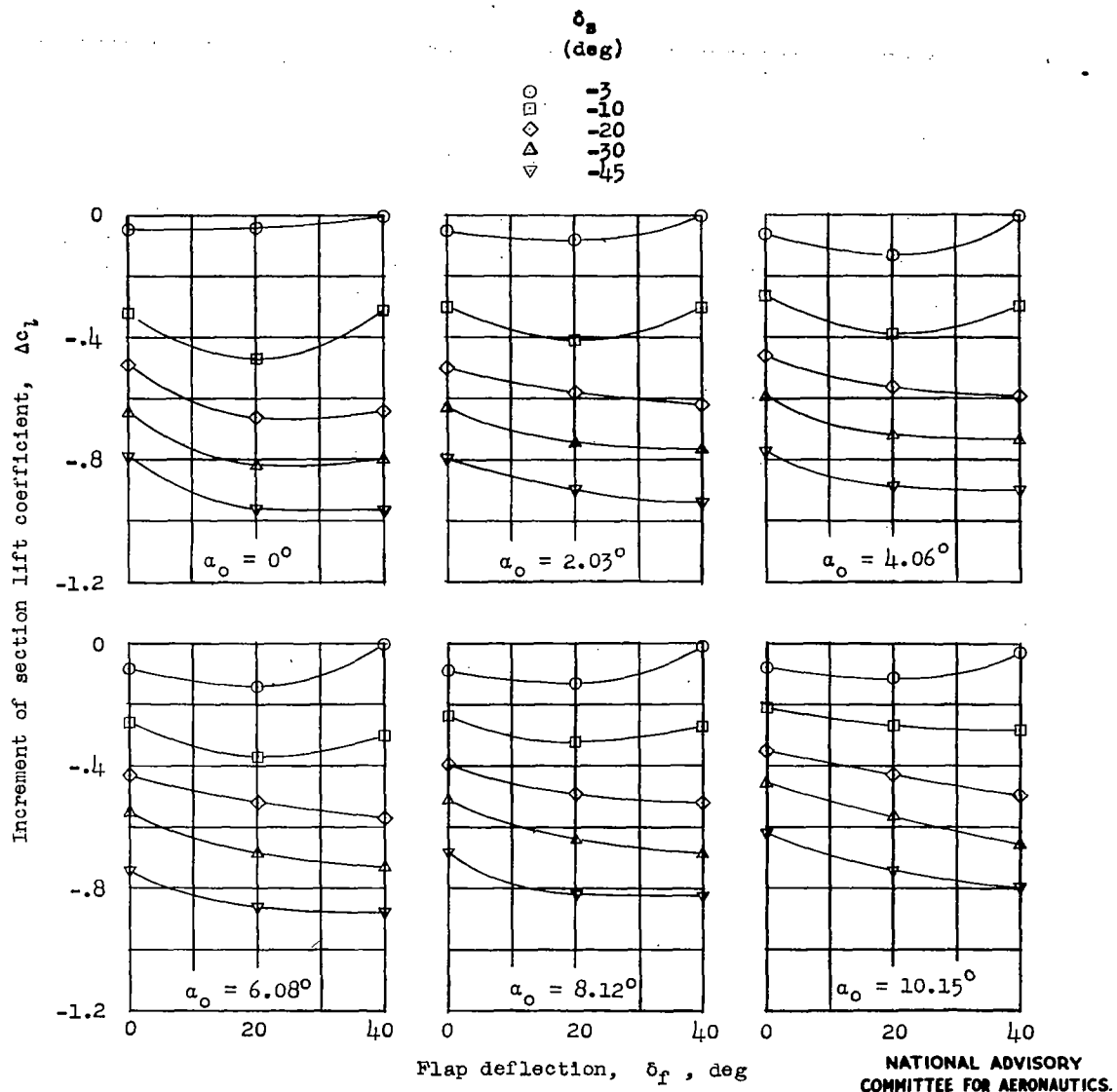
Figure 13.- Variation of the increment of section lift coefficient with flap deflection for the spoiler aileron flap model for the Hughes XF-11 airplane. Configuration number 9; R = 6.0 \times 10^6 .
