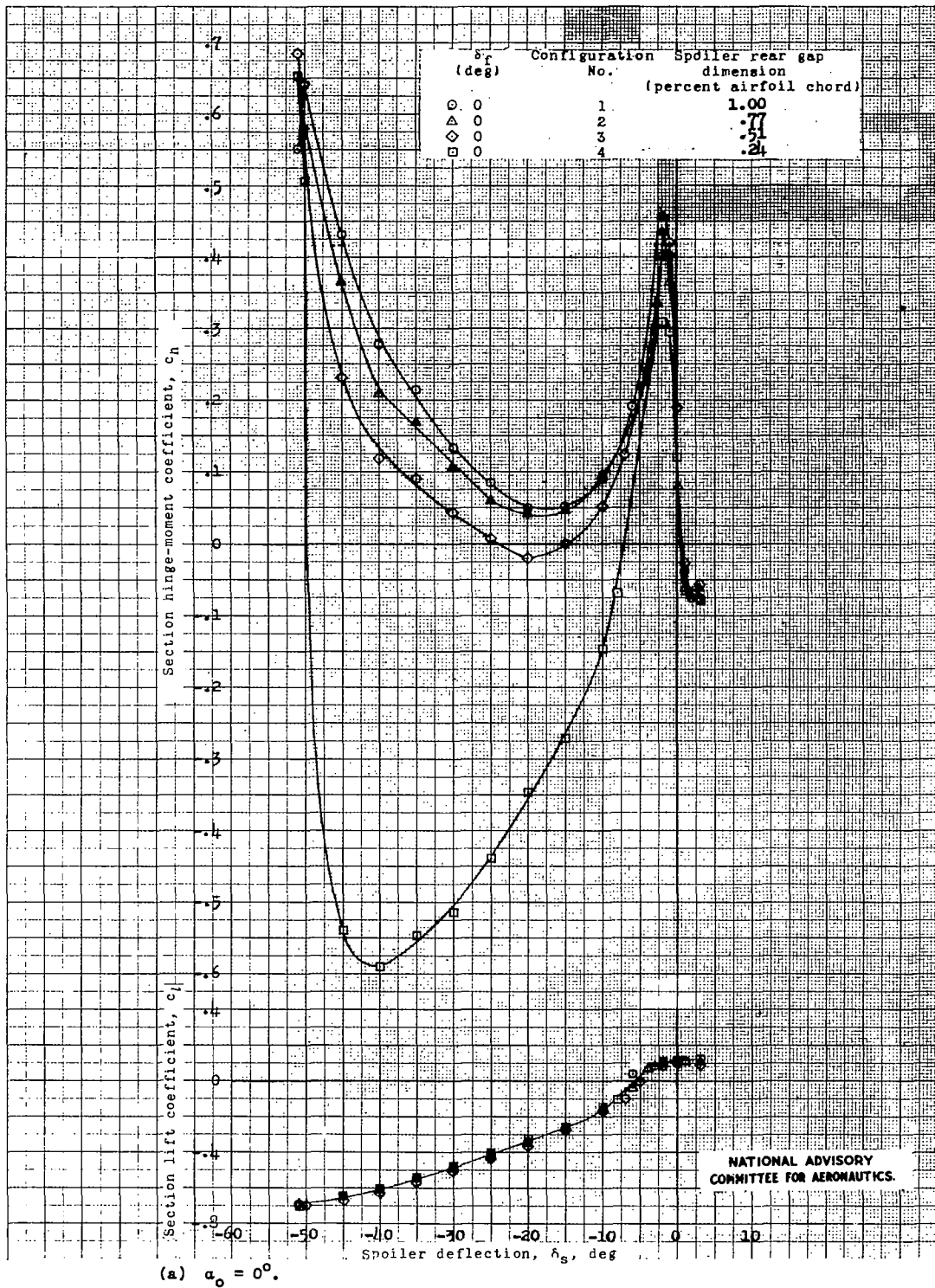
Figure 7.- Variation of section hinge-moment and lift coefficient with spoiler rear gap dimension for the spoiler aileron flap model for the Hughes XF-11 airplane. R = 2.5 \times 10^6 ; LTT test 392.
