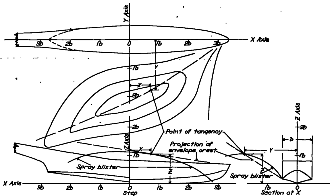
Figure 1.- Schematic sketch to show location on main spray blister of point of tangency to spray envelope.
