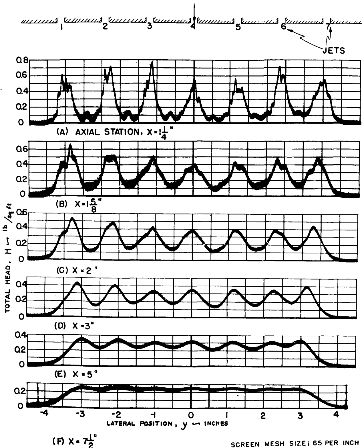
Figure 14.— Stabilizing effect of damping screen placed 1\frac{1}{16} " downstream from slots. Lateral total-head distributions.
