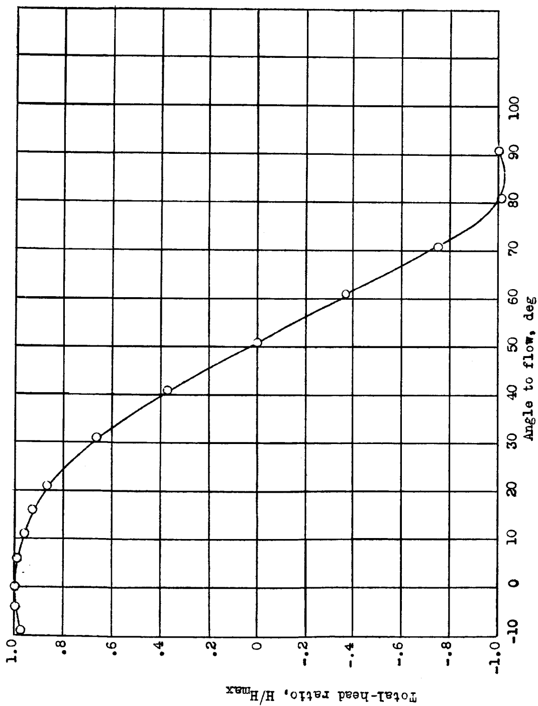
Figure 6.-- Total-head tube; directional sensitivity.
