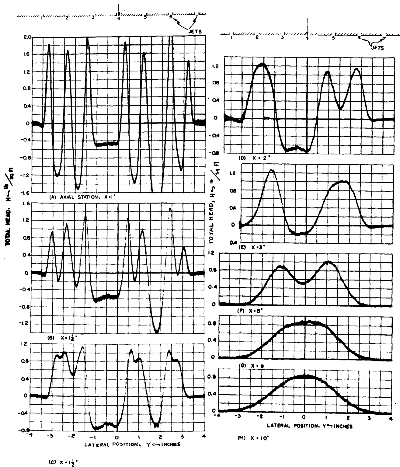
Figure 9.— Free jets. Lateral total-head distributions.
