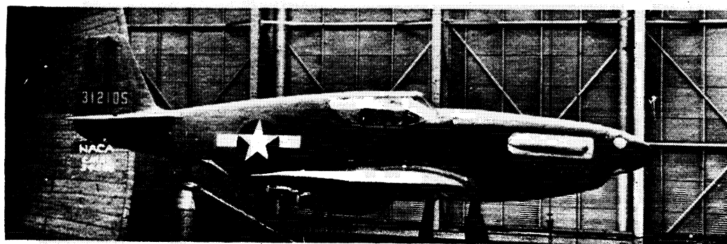
(l) Airplane 12. Sealed and faired condition; propeller removed.
