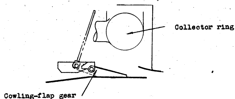
Section at original cowling outlet
