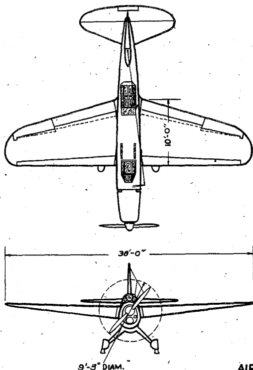
Figure 2.- Basic dimensions and general airplane characteristics of twelve airplanes tested.
