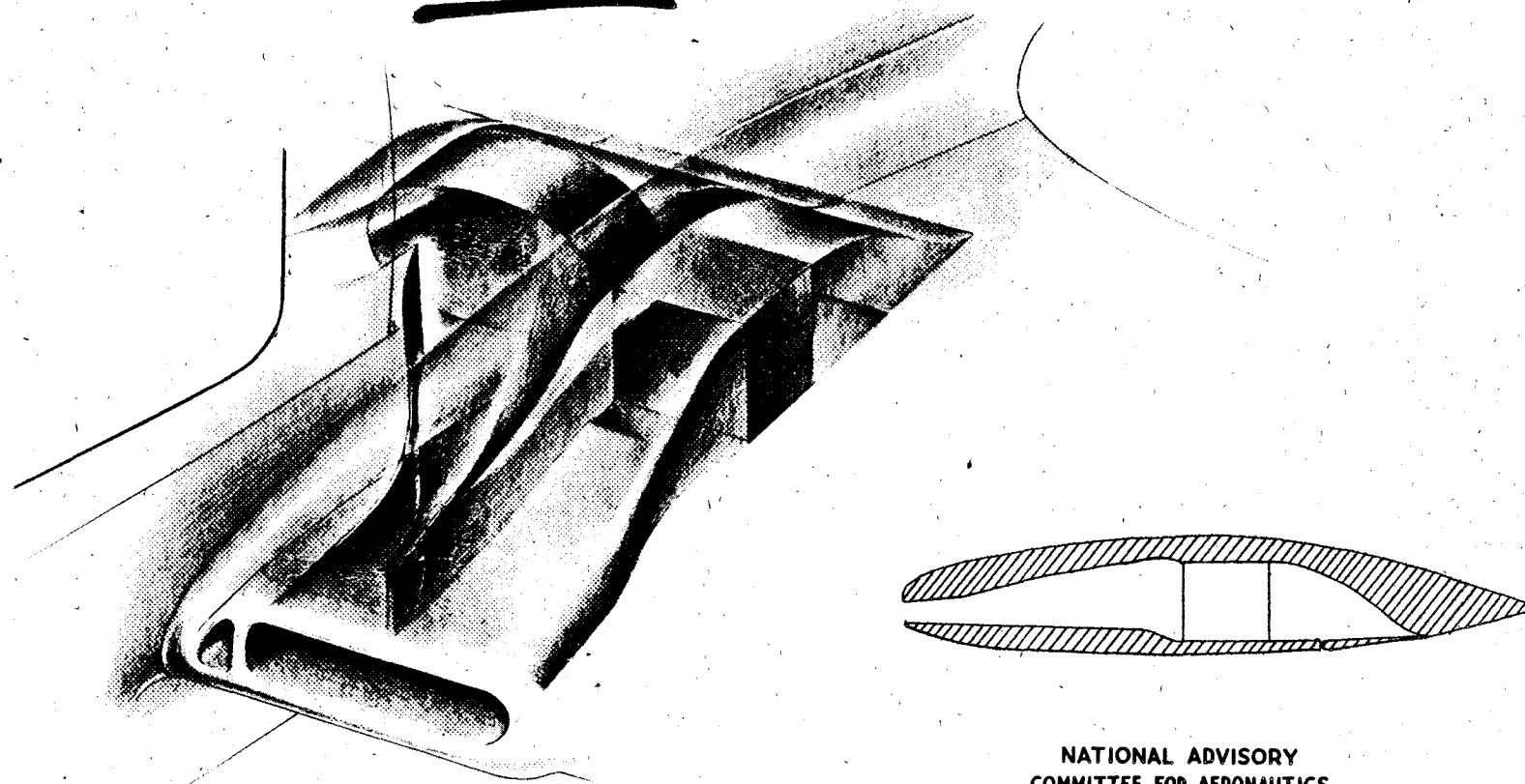
Figure 10.- Wing-duct inlet on airplane 11.
