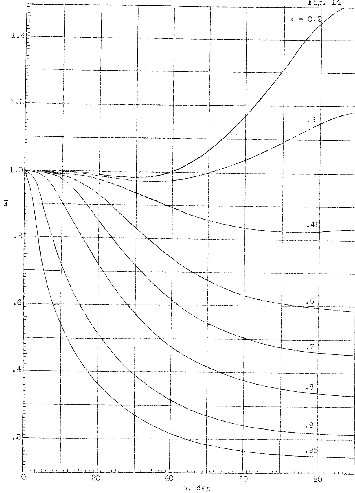
Figure 14.- Values of F for three-blade propeller. (Taken from reference 7.)
