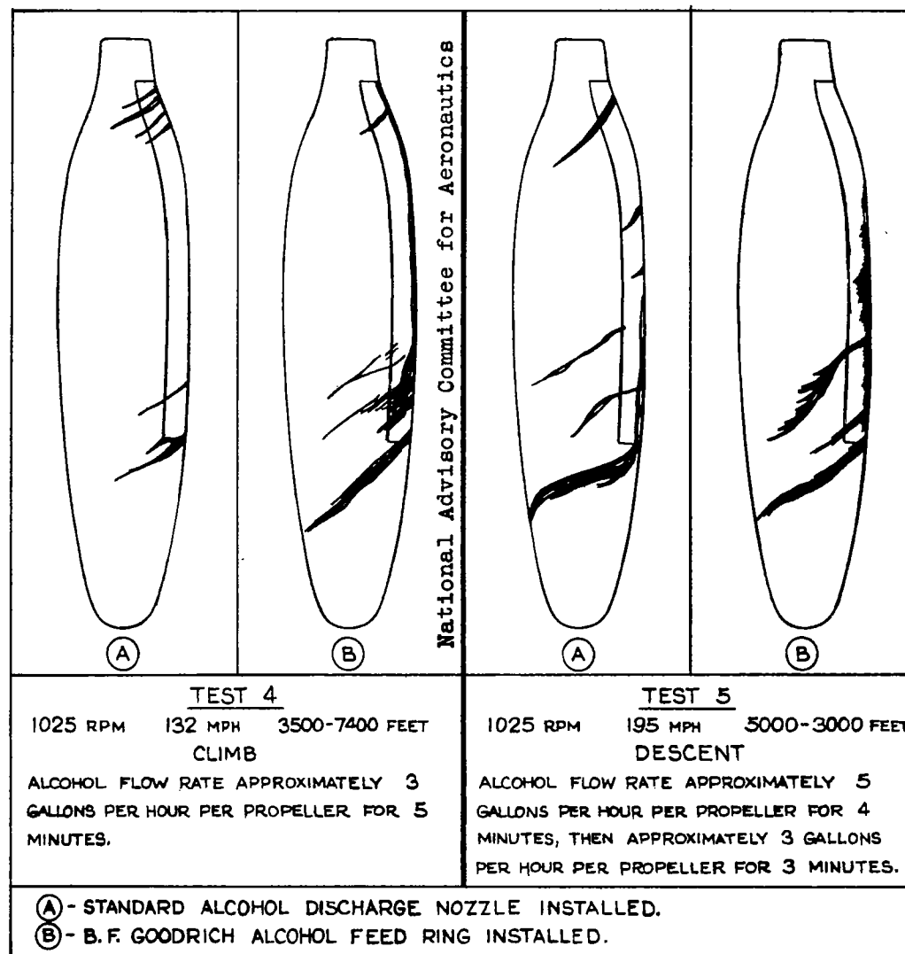
FIGURE 4 (CONCLUDED) - COMPARISON OF ALCOHOL FLOW DISTRIBUTION DURING CLIMB AND DESCENT CONDITIONS (b)
