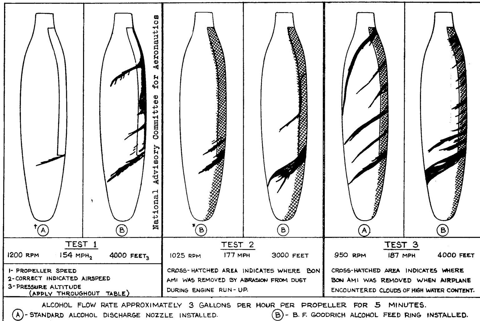
FIGURE 4 - COMPARISON OF ALCOHOL FLOW DISTRIBUTION ON CAMBER FACE OF PROPELLERS OF C-46 AIRPLANE EQUIPPED WITH B. F. GOODRICH ALCOHOL FEED RINGS ON LEFT PROPELLER AND STANDARD ALCOHOL DISCHARGE NOZZLES ON RIGHT PROPELLER DURING LEVEL FLIGHT.
