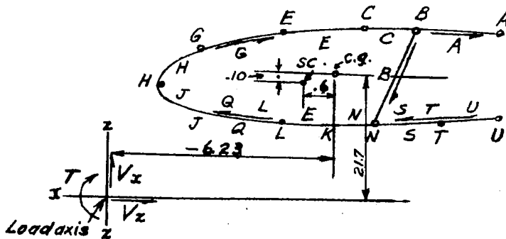
Figure 23.— Sign convention. All loads and dimensions shown are positive.
