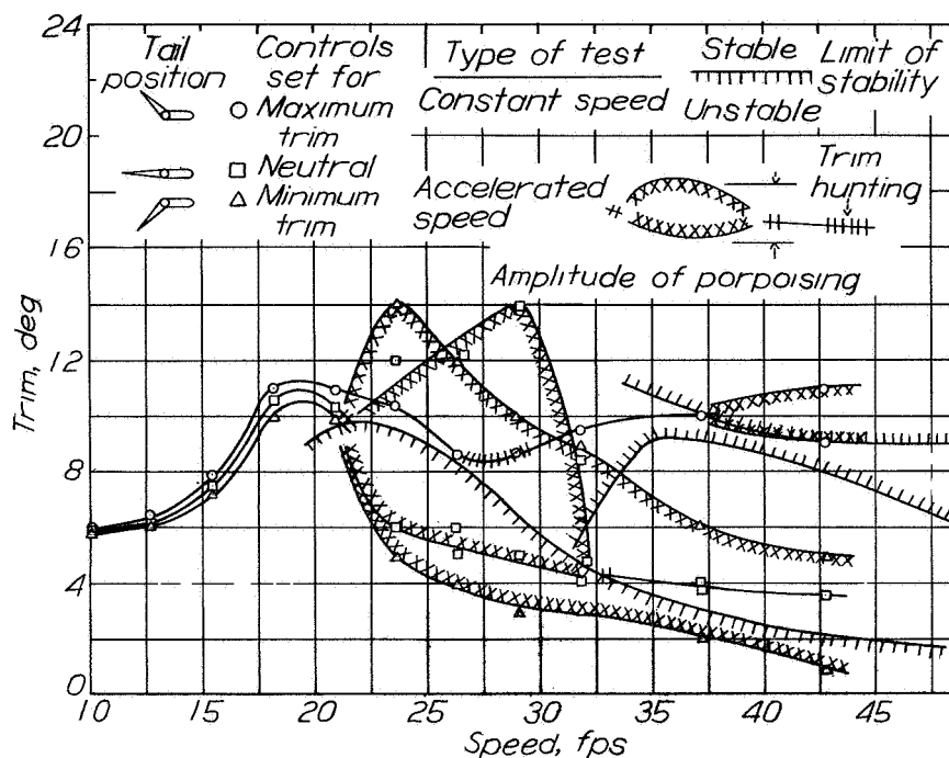
Figure 12.- Model 101BC. Stability characteristics obtained during accelerated and constant-speed runs. Load at rest, \Delta_0 = 76.5 lb; mass moving vertically, 76.5 lb.
