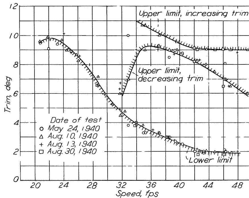
Figure 9.- Model 101BC. Scatter of points obtained during tests of 101BC.
