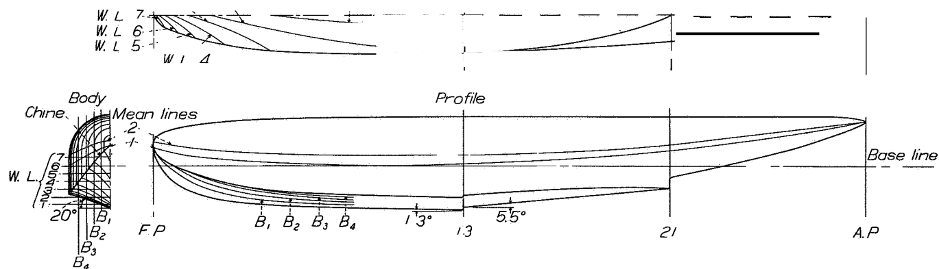
Figure 2.- Lines of model 101BA
