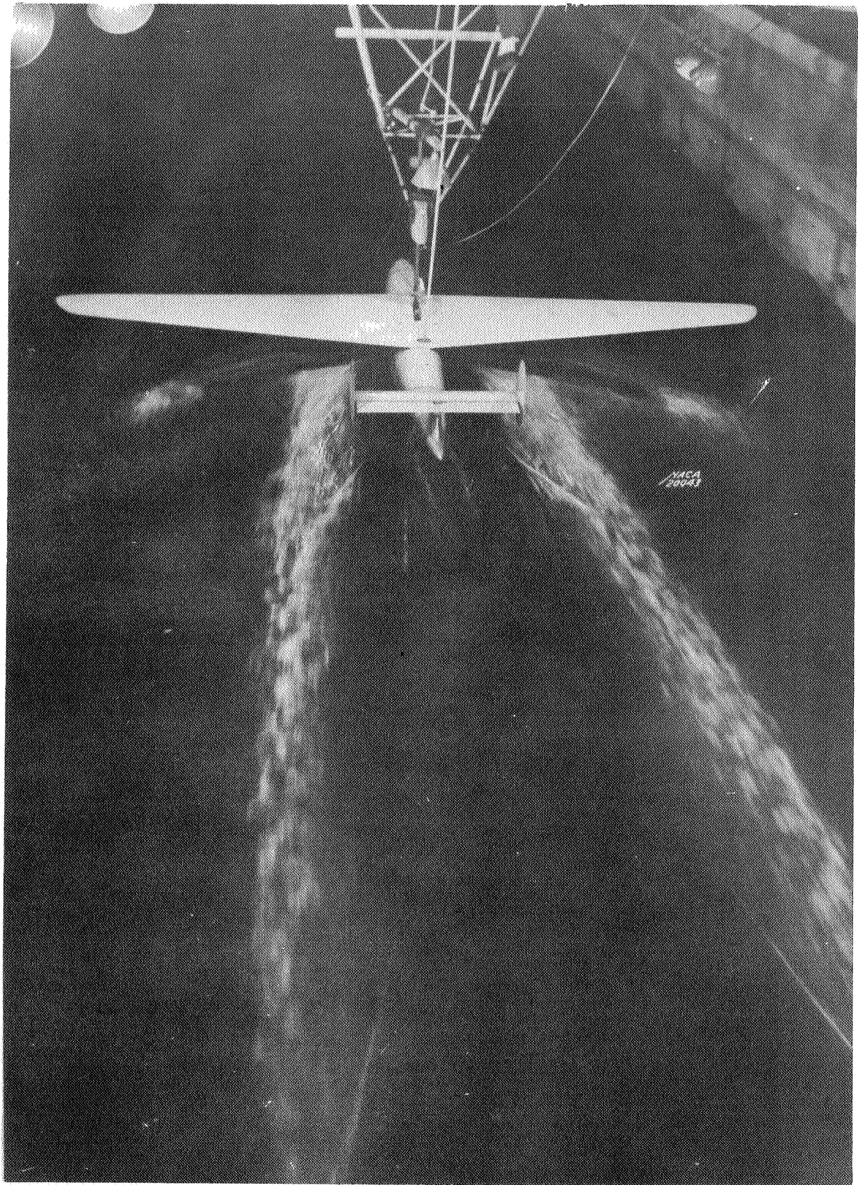
Figure 8. - Model 101 being towed under auxiliary carriage.
