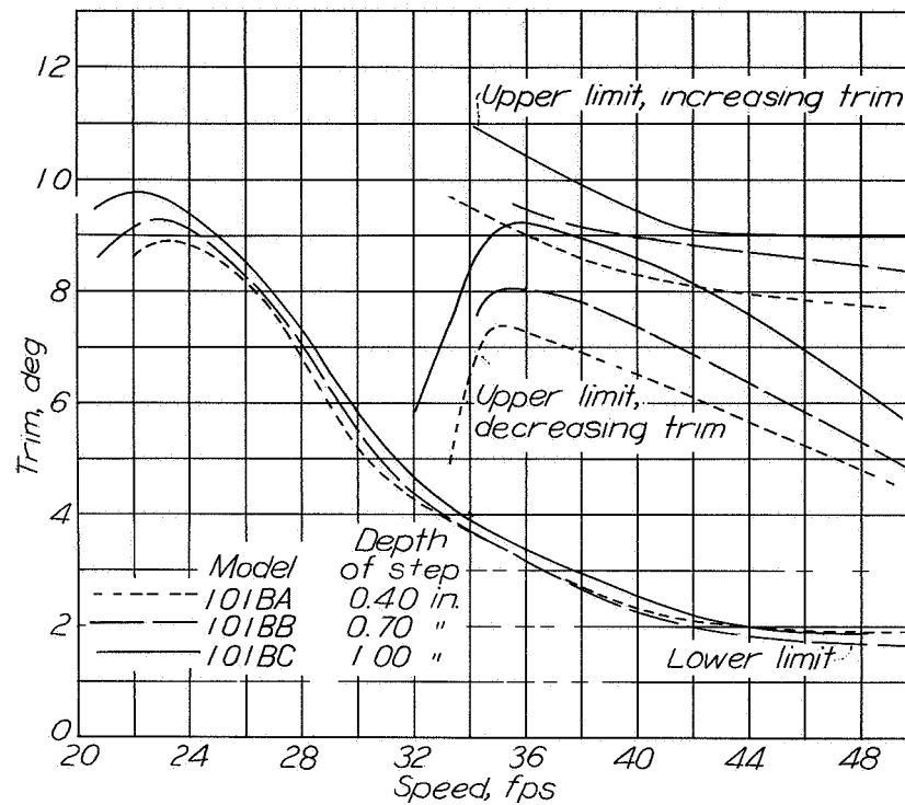
Figure 16.- Model 101. Effect of depth of step on limits of stability.
