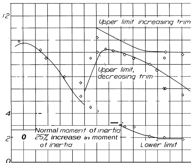
Figure 13.- Model 101BC. Effect of increasing moment of inertia, constant-speed runs.
