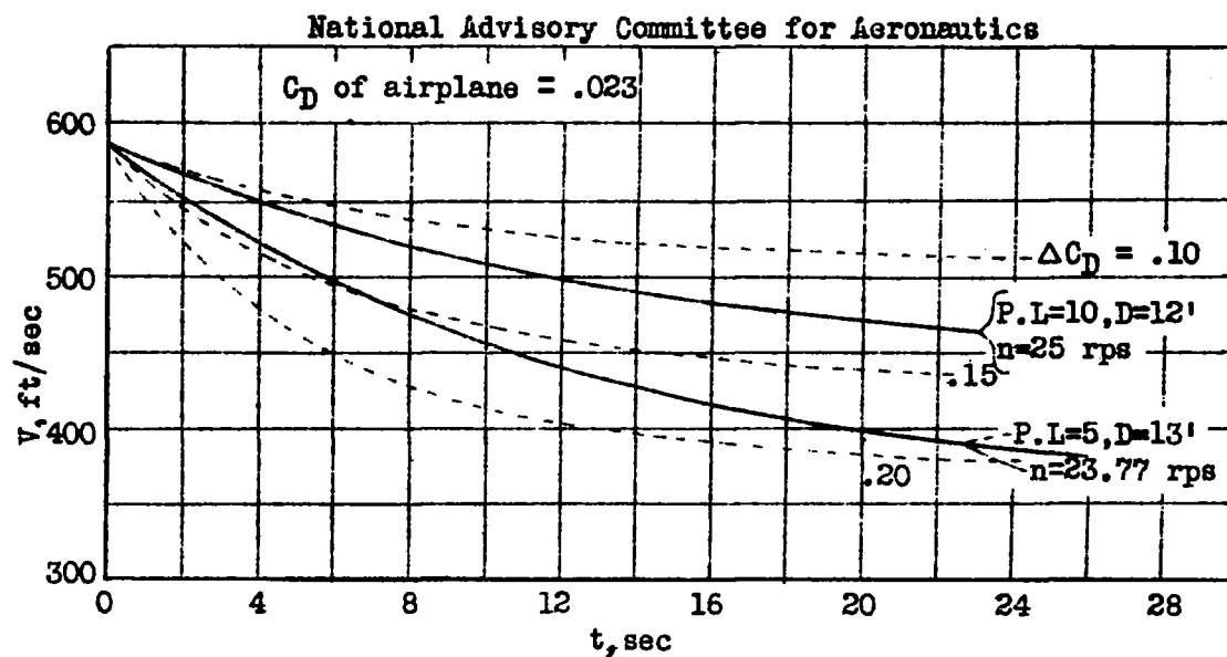
Figure 16.- The variation of velocity with time for a dive bomber utilizing constant-speed reversed-pitch propellers and aerodynamic dive flaps while in a 60^\circ dive.
