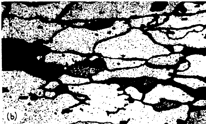
Figure 5a,b.- Inter- granular attack in 24S-T aluminum-alloy sheet, specimen 43879-5.
