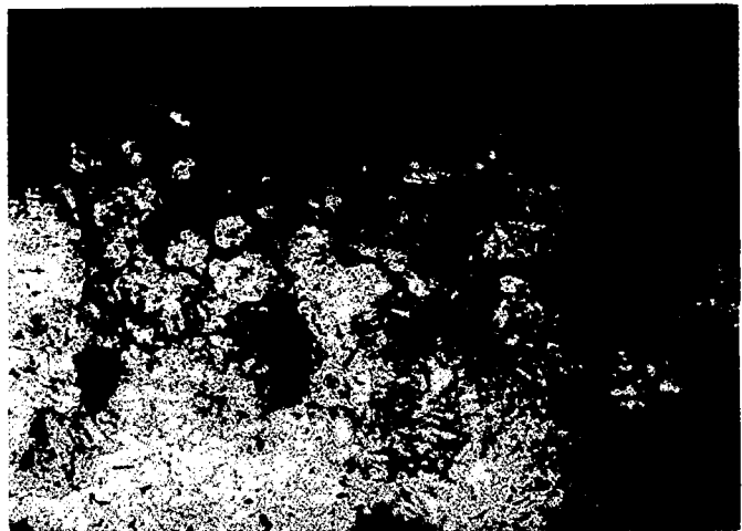
Figure 8.- Intergranular attack in a zone still exhibiting a dendritic structure in extruded 24S-T aluminum alloy, specimen 36990-4. Magnification, 100 diameters.
