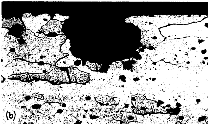
Figure 1a,b.- Pit- ting attack in 24S-T aluminum- alloy sheet, speci- men 43870-6.
