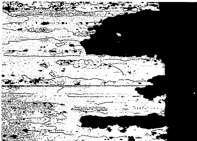
Figure 2.- Pitting type of edge at- tack in 24S-T alu- minum-alloy tubing, specimen 45974. Magnification, 100 diameters.
