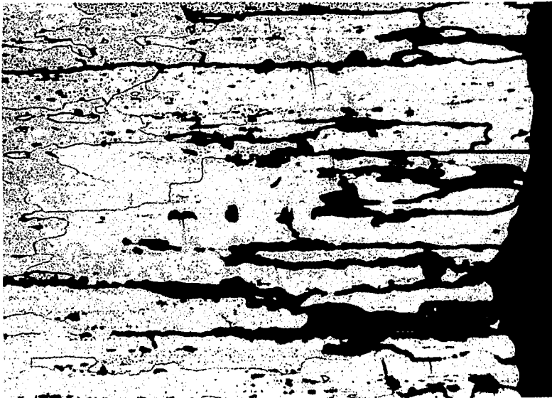
Figure 7.- Intergranular type of edge attack in 24S-T aluminum-alloy tubing, specimen 45973. Magnification, 100 diameters.
