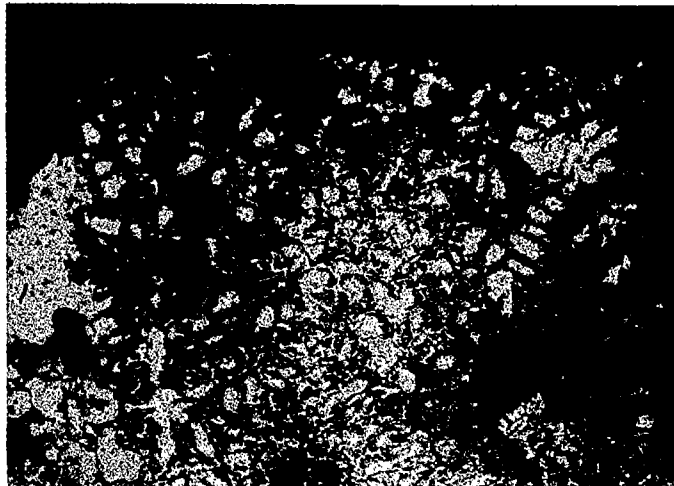
Figure 10.- Interdendritic attack in extruded 24S-T aluminum alloy, specimen 36989-1. Magnification, 100 diameters.
