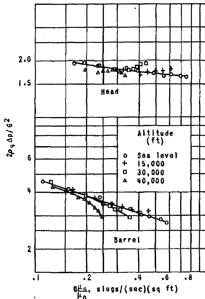
Figure 10. - Variation of pressure-loss coefficient based on downstream density with corrected mass flow of cooling air; data with heat transfer.
