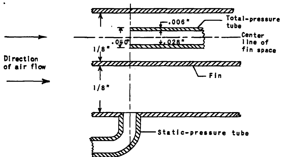
Section A-A showing fin space and pressure-tube proportions
