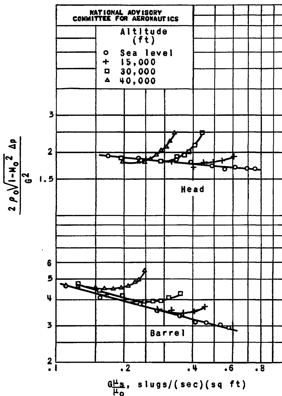
Figure 11. - Variation of pressure-loss coefficient based on characteristic Mach number with corrected mass flow of cooling air; data without heat transfer.
