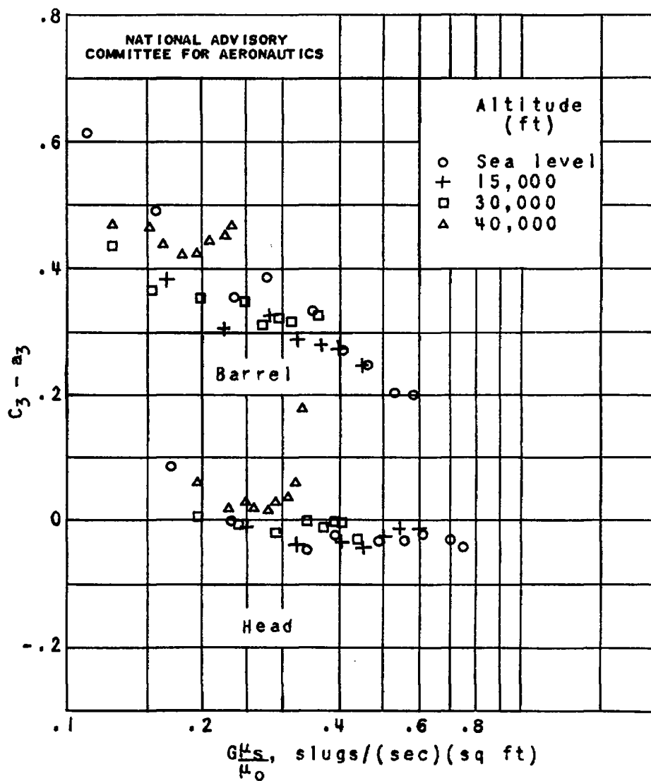
Figure 5. - Variation of baffle-exit pressure-loss coefficient with corrected mass flow of cooling air; data without heat transfer.
