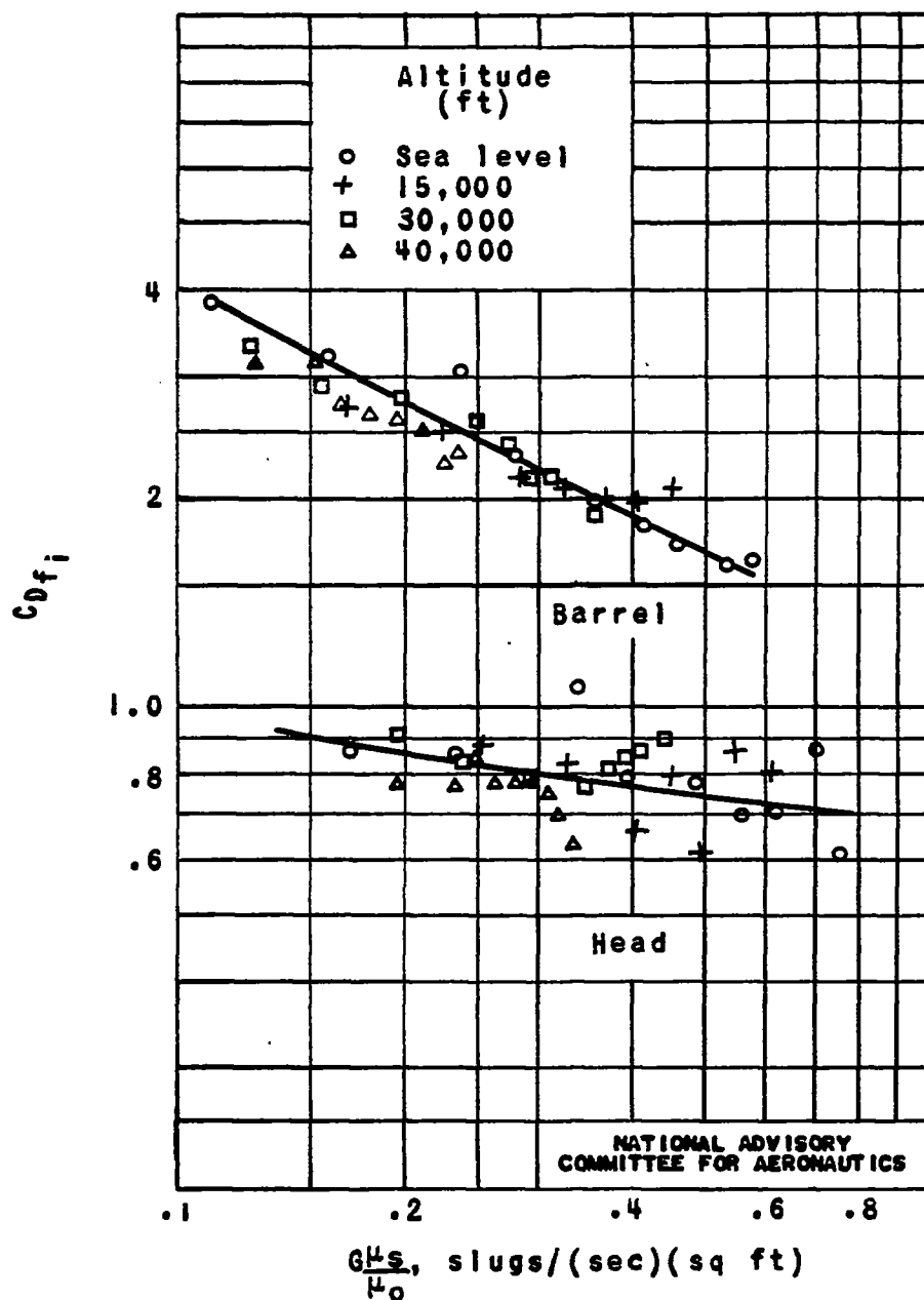
Figure 4. - Variation of friction-drag coefficient C_{Df_i} with corrected mass flow of cooling air; data without heat transfer.
