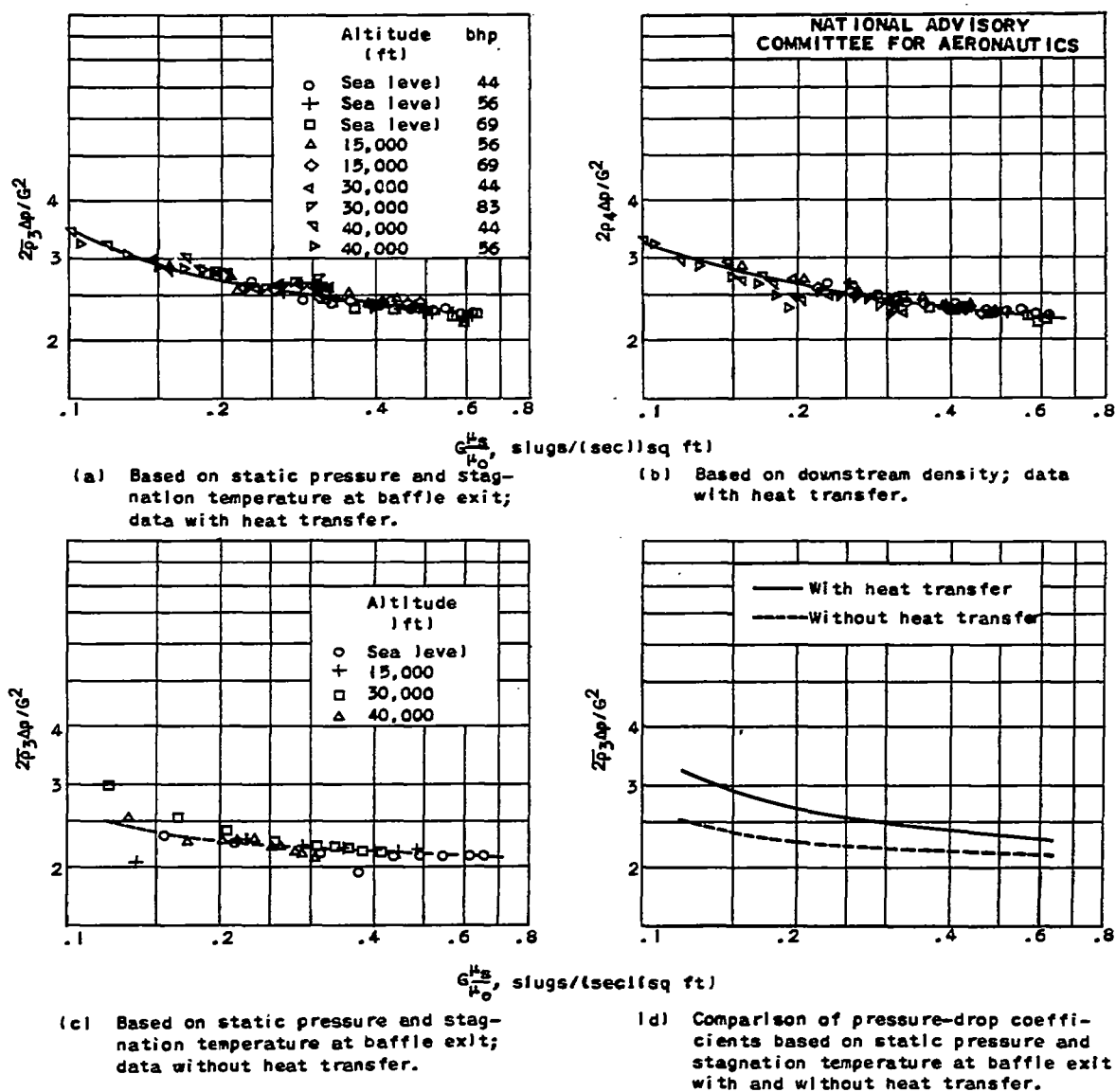
Figure 12. - Pressure-drop coefficients for combined head and barrel determined with and without heat transfer.
