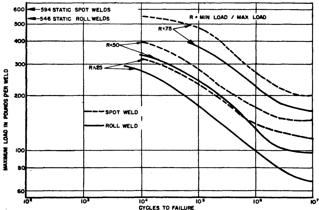
FIG. 21.-FATIGUE CURVES FOR ROLL-WELDED AND SPOT-WELDED SAMPLES. (SAMPLES 5" X 0.040" WELDS \frac{3}{8} " APART.)
