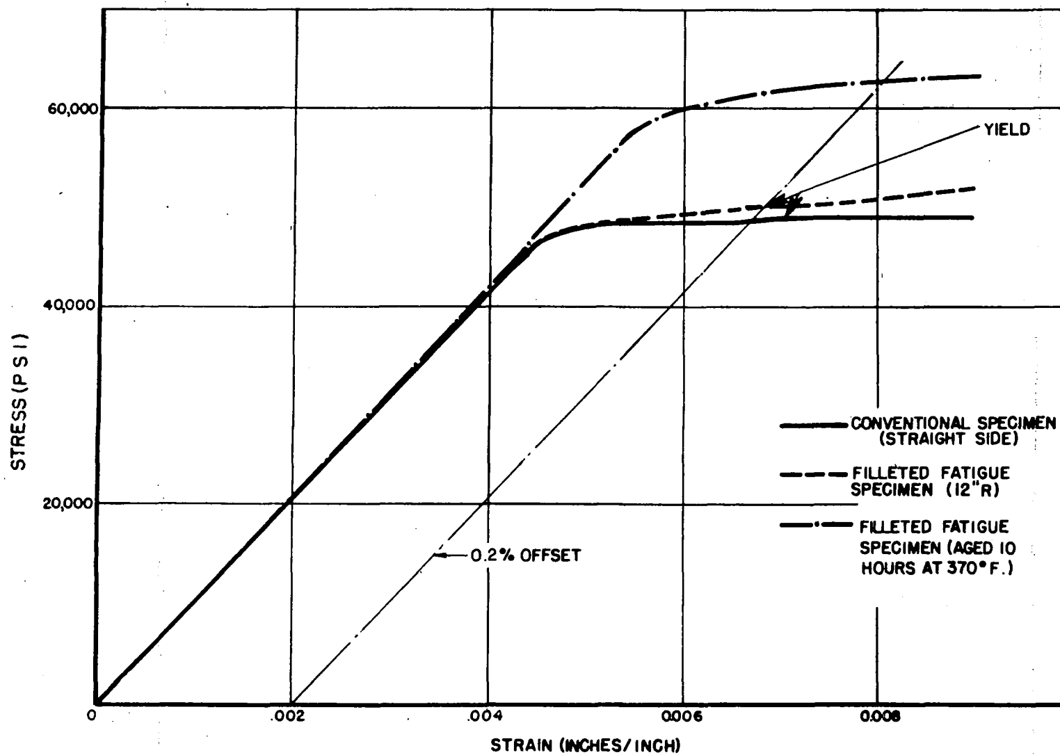
FIG. 2: STATIC STRESS-STRAIN CURVE FOR ALCLAD 24 S-T SHEET 1.000" X 0.40".
