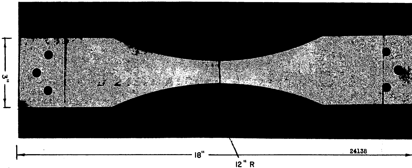
Figure 1. Photograph of a Typical (failed) Test Piece Used in Fatigue Tests. (0.040" Alclad 24S-T Sheet)
