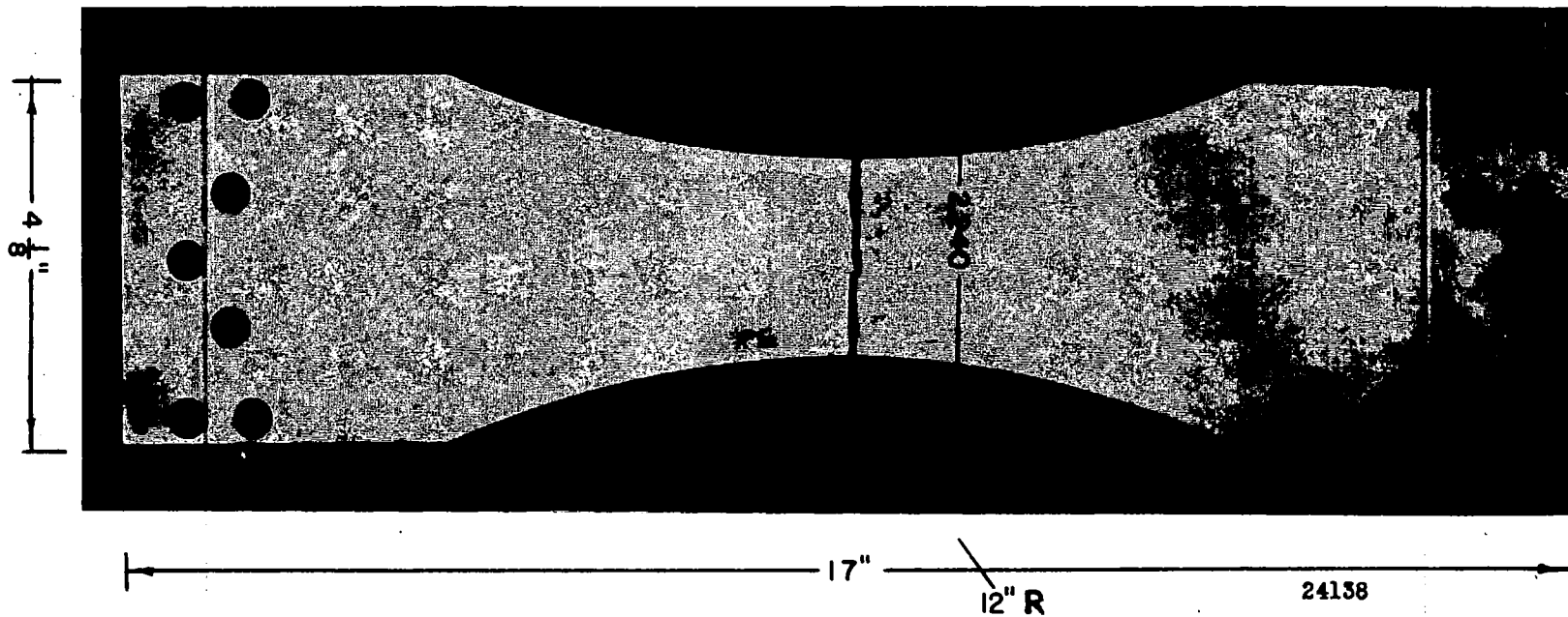
Figure 6. Photograph of a Typical (failed) Sheet Efficiency Test Piece Used in Fatigue Tests. (0.040" Alclad 24S-T, \frac{3}{4}" Spot Spacing.)
