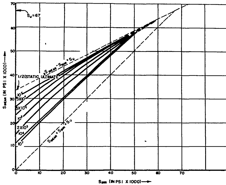
FIG 42-CONSTANT LIFETIME CURVES MEAN LOAD VS. MINIMUM LOAD.
