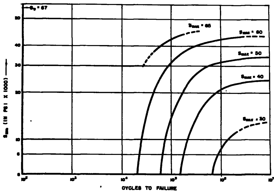
FIG. 31.-CONSTANT MAXIMUM-LOAD CURVES, MINIMUM LOAD VS. LIFETIME.
