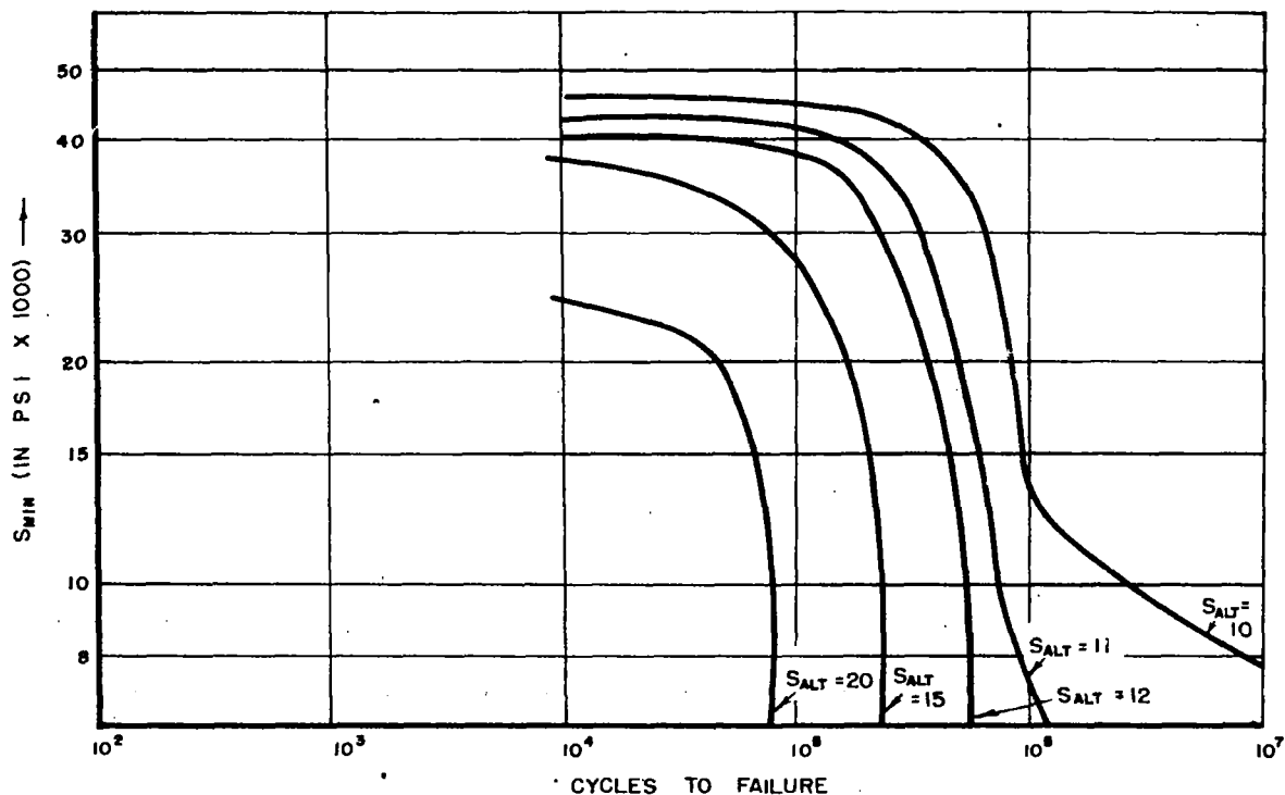
FIG. 37.- CONSTANT ALTERNATING LOAD CURVES, MINIMUM LOAD VS. LIFETIME.
