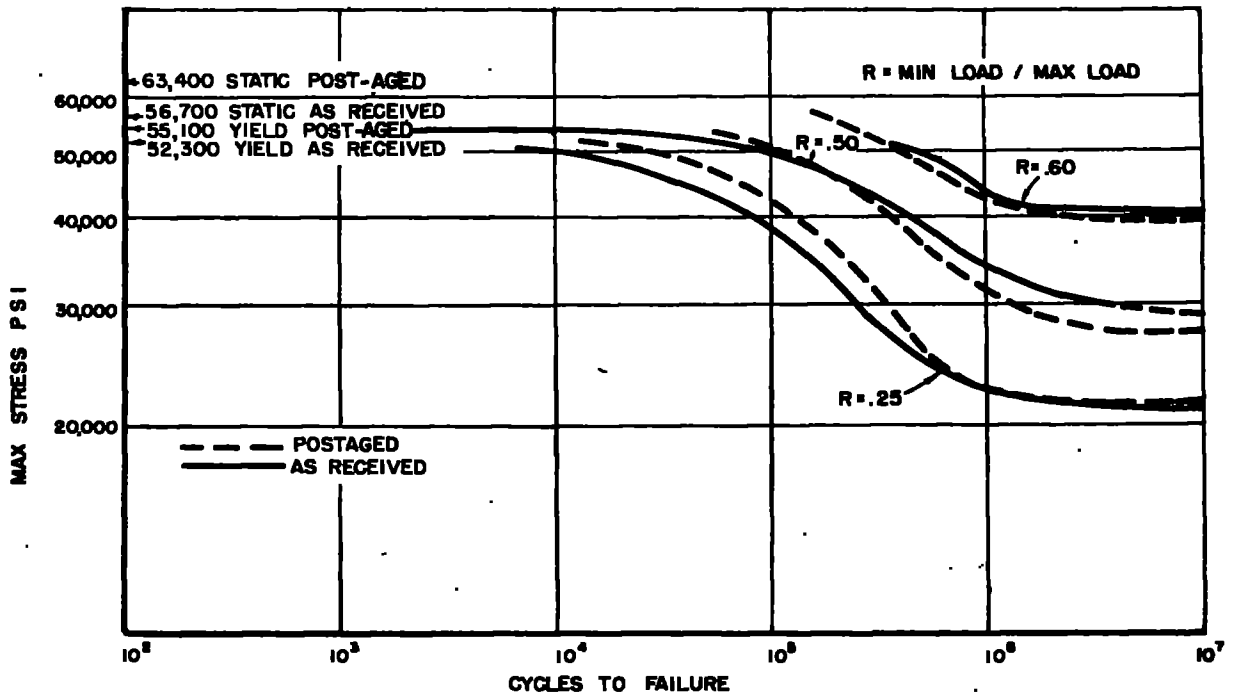
FIG. 9.- FATIGUE CURVES FOR SHEET EFFICIENCY SAMPLES 0.040" AS RECEIVED AND POST-AGED.
