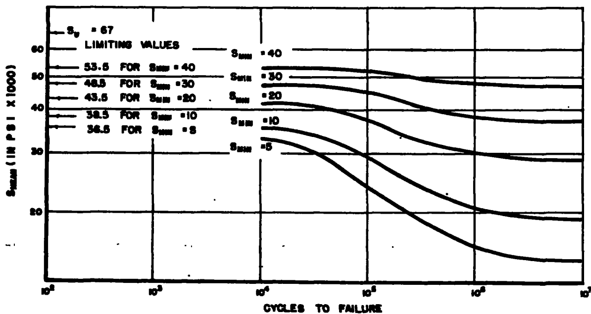
FIG. 29.-CONSTANT MINIMUM LOAD CURVES, MEAN LOAD VS. LIFETIME.
