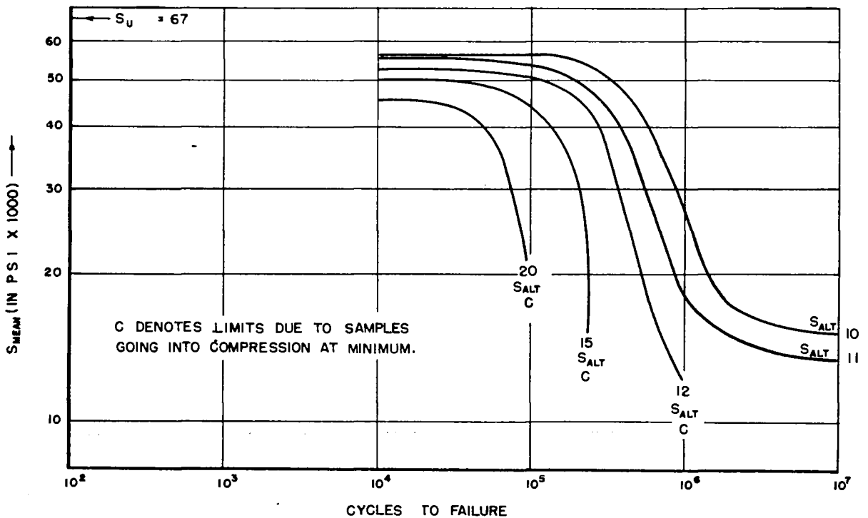
FIG. 39.-CONSTANT ALTERNATING LOAD CURVES, MEAN LOAD VS. LIFETIME.
