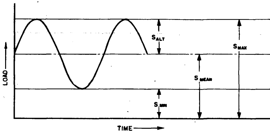
FIG. 26.-LOAD COMPONENTS OF TENSION-TENSION FATIGUE TESTING.
