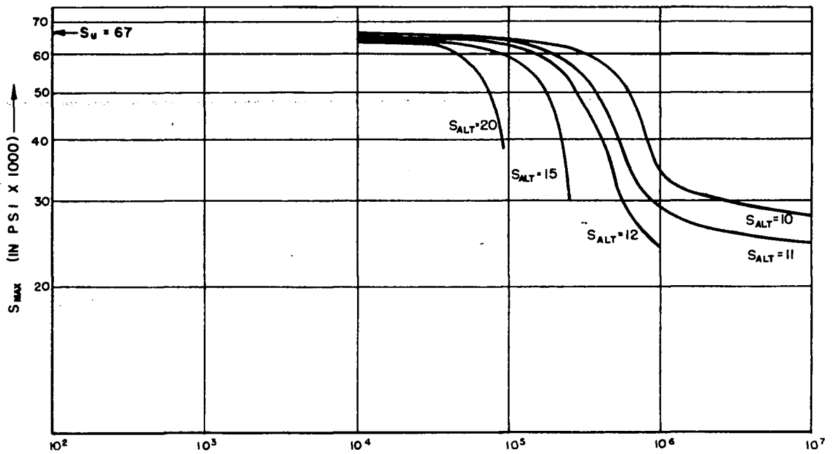
FIG. 38.-CONSTANT ALTERNATING LOAD CURVES, MAXIMUM LOAD VS. LIFETIME
