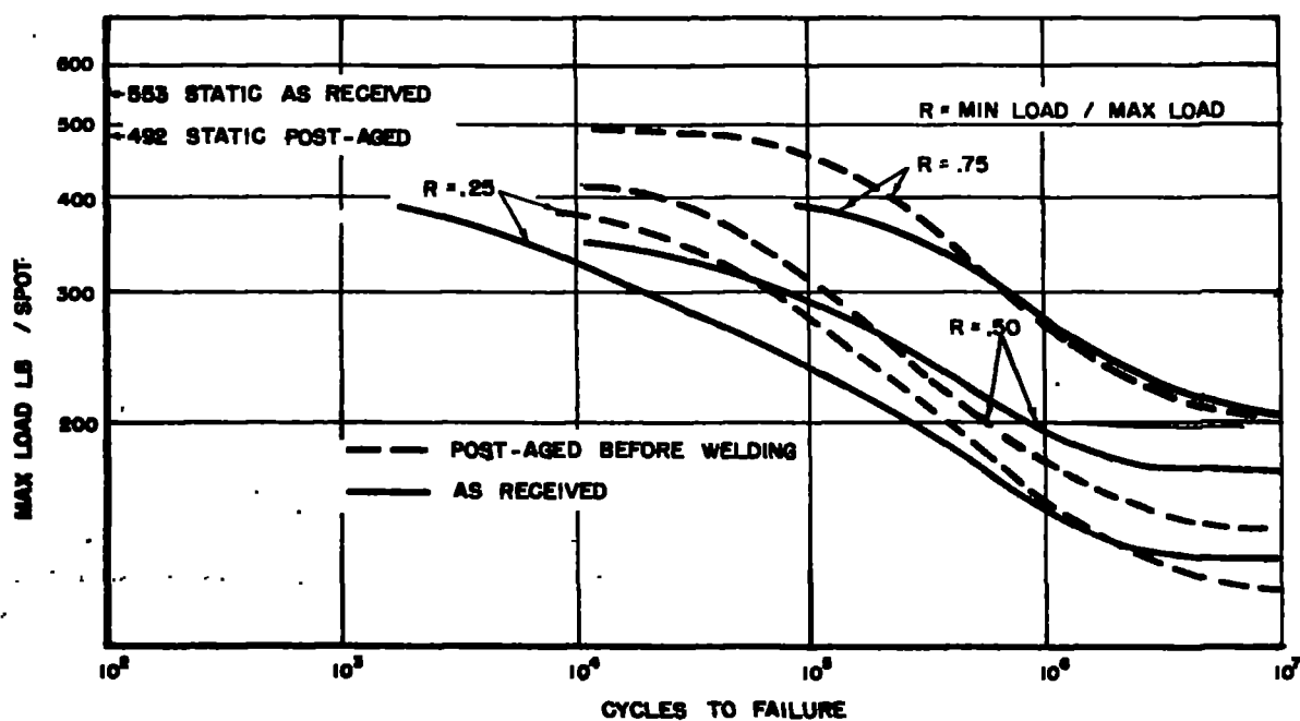
FIG. 15.- FATIGUE CURVES FOR LAP JOINT SAMPLES AS RECEIVED AND POST-AGED BEFORE WELDING (SAMPLES 5" X 0.040" SPOTS 3/4" APART.)
