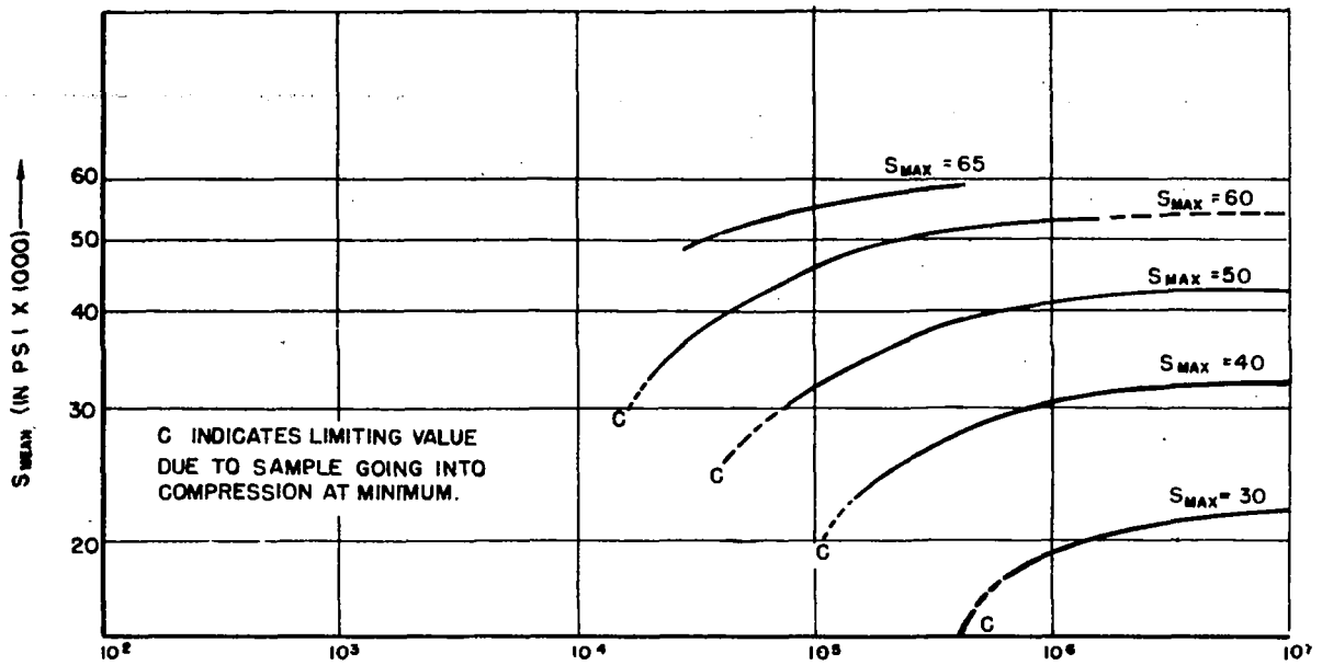
FIG. 32. CONSTANT MAXIMUM LOAD CURVES, MEAN LOAD VS. LIFETIME
