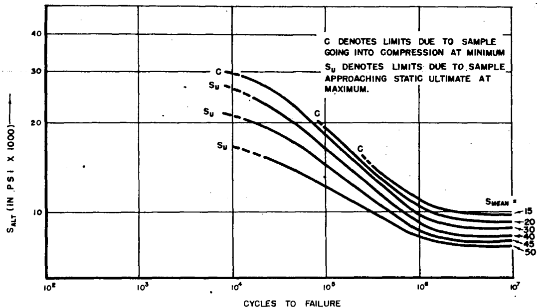
FIG. 36.-CONSTANT MEAN LOAD CURVES, ALTERNATING LOAD VS. LIFETIME.
