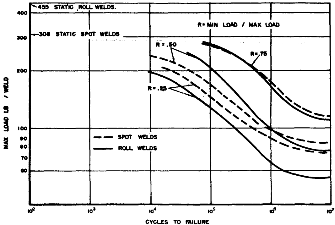
FIG. 20.-FATIGUE CURVES FOR ROLL-WELDED AND SPOT-WELDED SAMPLES. (SAMPLES 5" X 0.040" WELDS 3/8" APART.)
