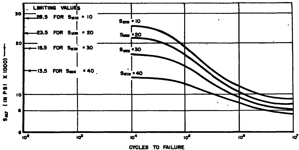
FIG. 30.-CONSTANT MINIMUM LOAD CURVES, ALTERNATING LOAD VS. LIFETIME.
