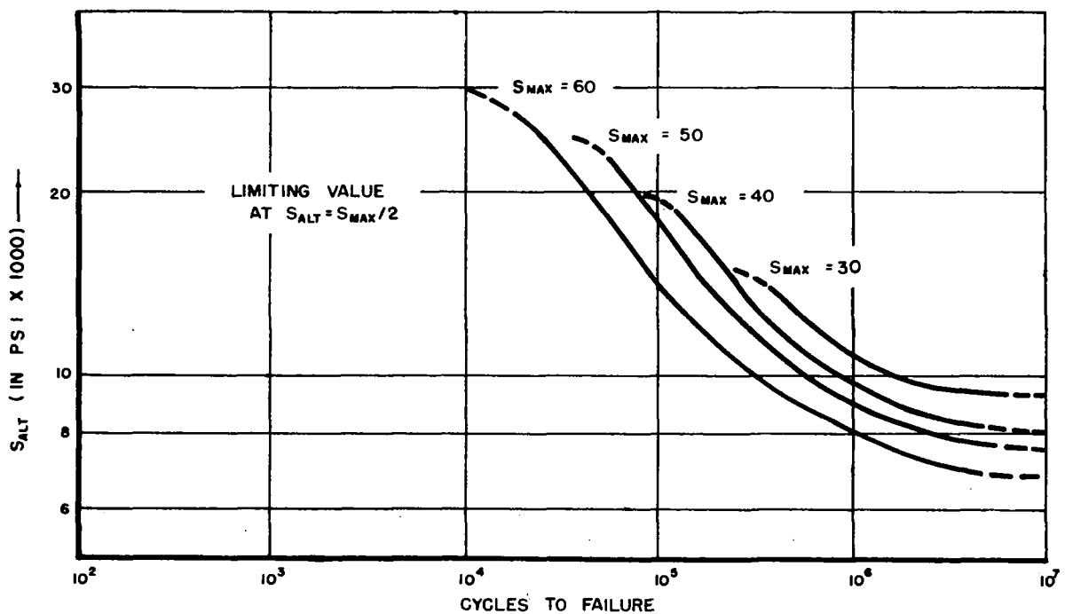
FIG. 33.-CONSTANT MAXIMUM LOAD CURVES, ALTERNATING LOAD VS. LIFETIME
