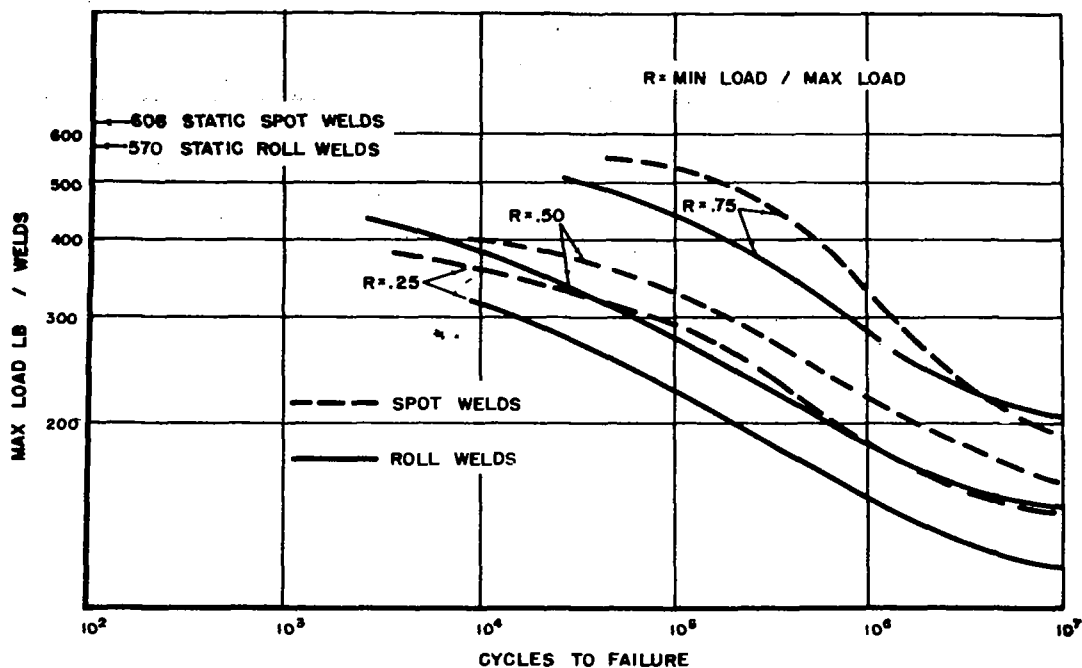
FIG. 22.-FATIGUE CURVES FOR ROLL-WELDED AND SPOT-WELDED SAMPLES. (SAMPLES 5" X 0.040", SPOTS 1-1/4" APART.)
