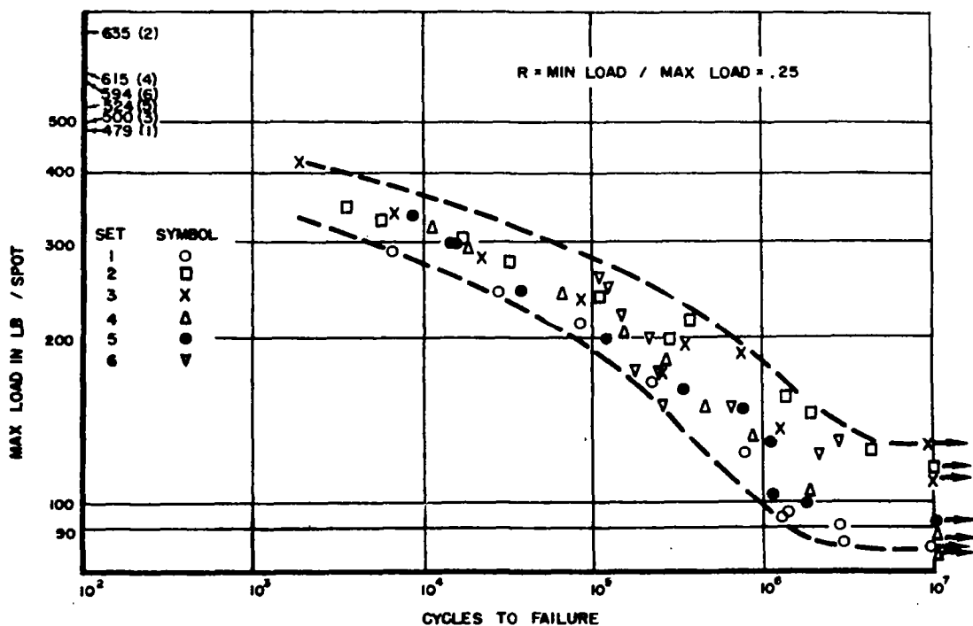
FIG. 23.-FATIGUE CURVES FOR LAP JOINT SAMPLES MADE WITH VARIOUS WELDING CONDITIONS FROM SHEET OF DIFFERENT HEATS (SAMPLES 5" X 0.040", 6 SPOT WELDS SPACED 3/4" APART.)
