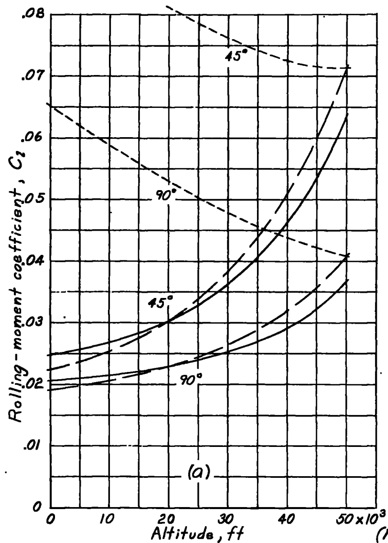
(a) The rolling moment necessary to bank to 45° at the end of the first half second and 90° at the end of the first second.
