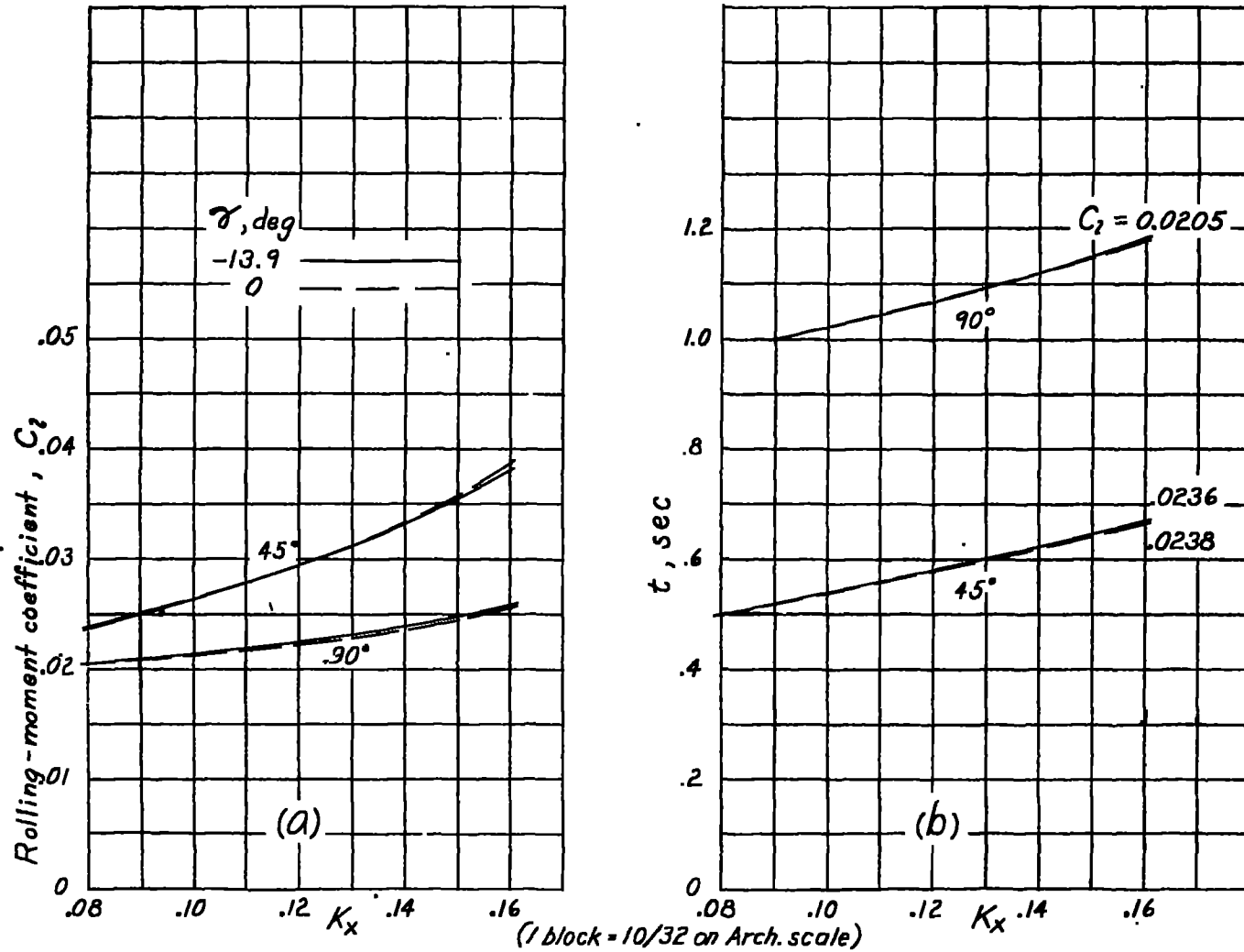
(a) The rolling moment necessary to bank to 45^\circ at the end of the first half second and 90^\circ at the end of the first second.
