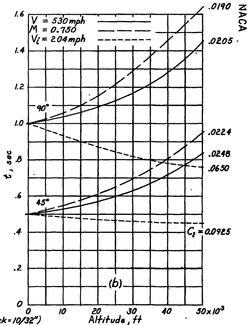
(b) The time to bank to 45° and 90°.
