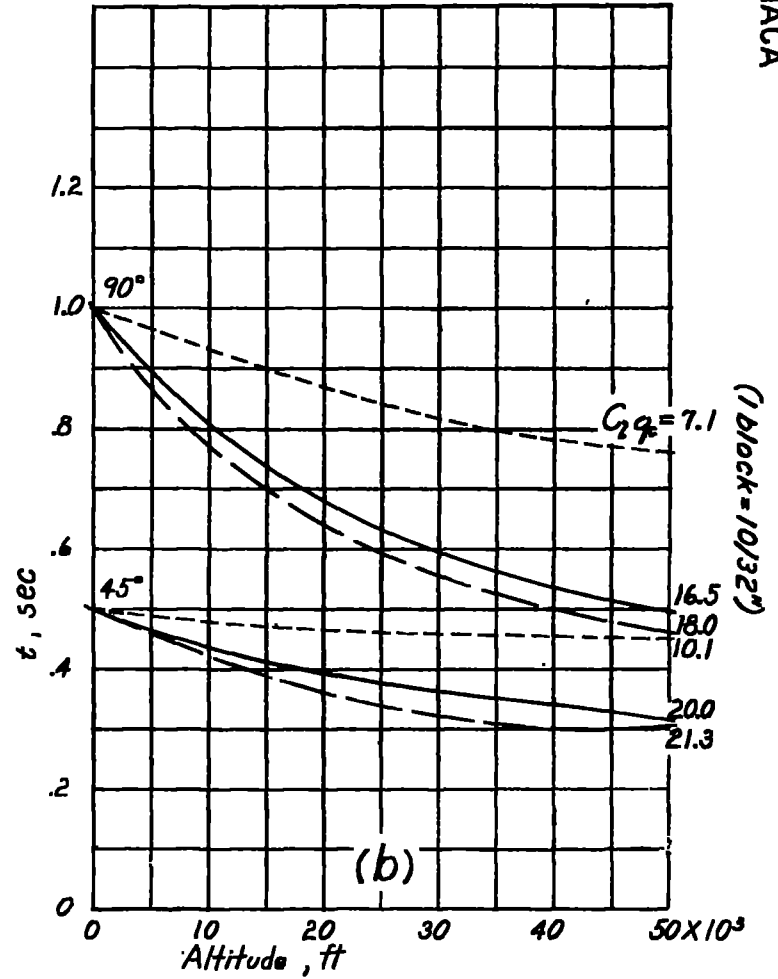
(b) The time to bank to 45^\circ and 90^\circ .
