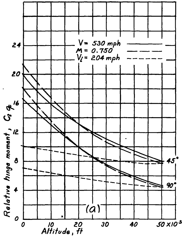
(a) The relative hinge moment necessary to bank to 45^\circ at the end of the first half second and 90^\circ at the end of the first second.
