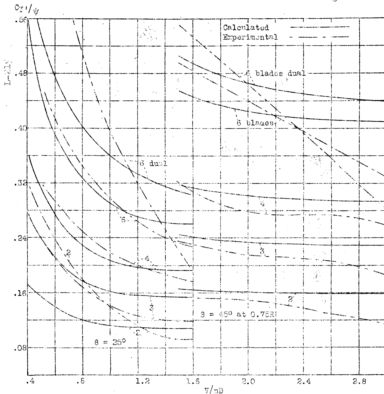
Figure 14.- Comparison of calculated curves of C_T/\psi with the faired experimental curves from reference 17 for 10° yaw. The original data with respect to pitch, with wind axes, have been converted to data with respect to yaw, with body axes.
