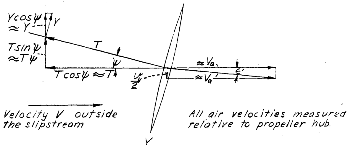
Figure 3.- Vector relations pertaining to the sidewash of a propeller in yaw.
