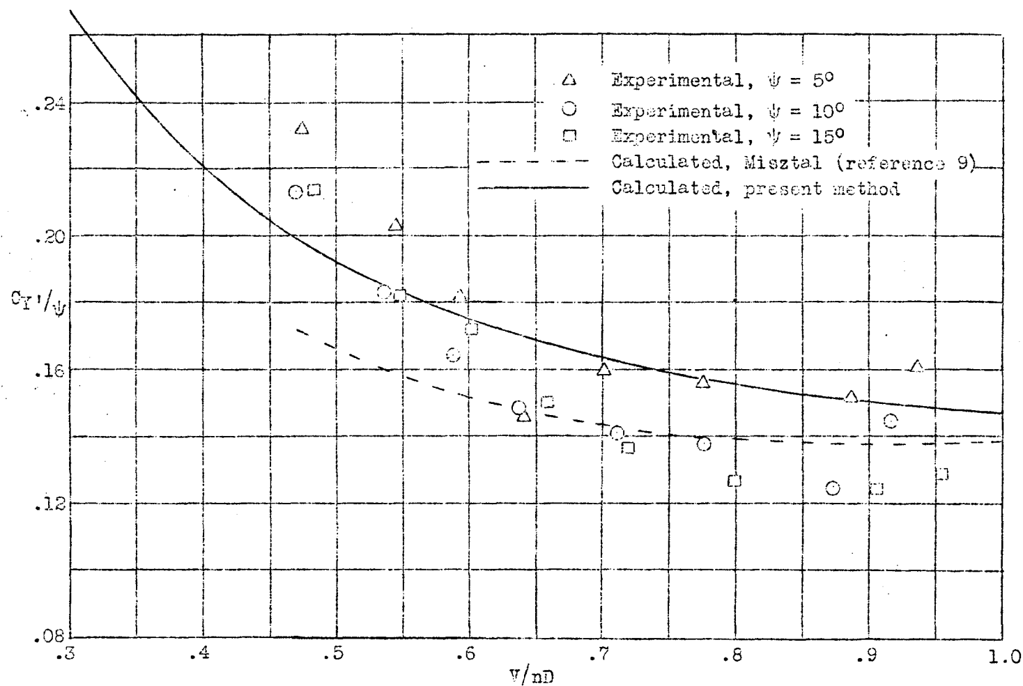
Figure 12.- Comparison of calculated curves of C_Y' / \psi with the experimental values of reference 15.
