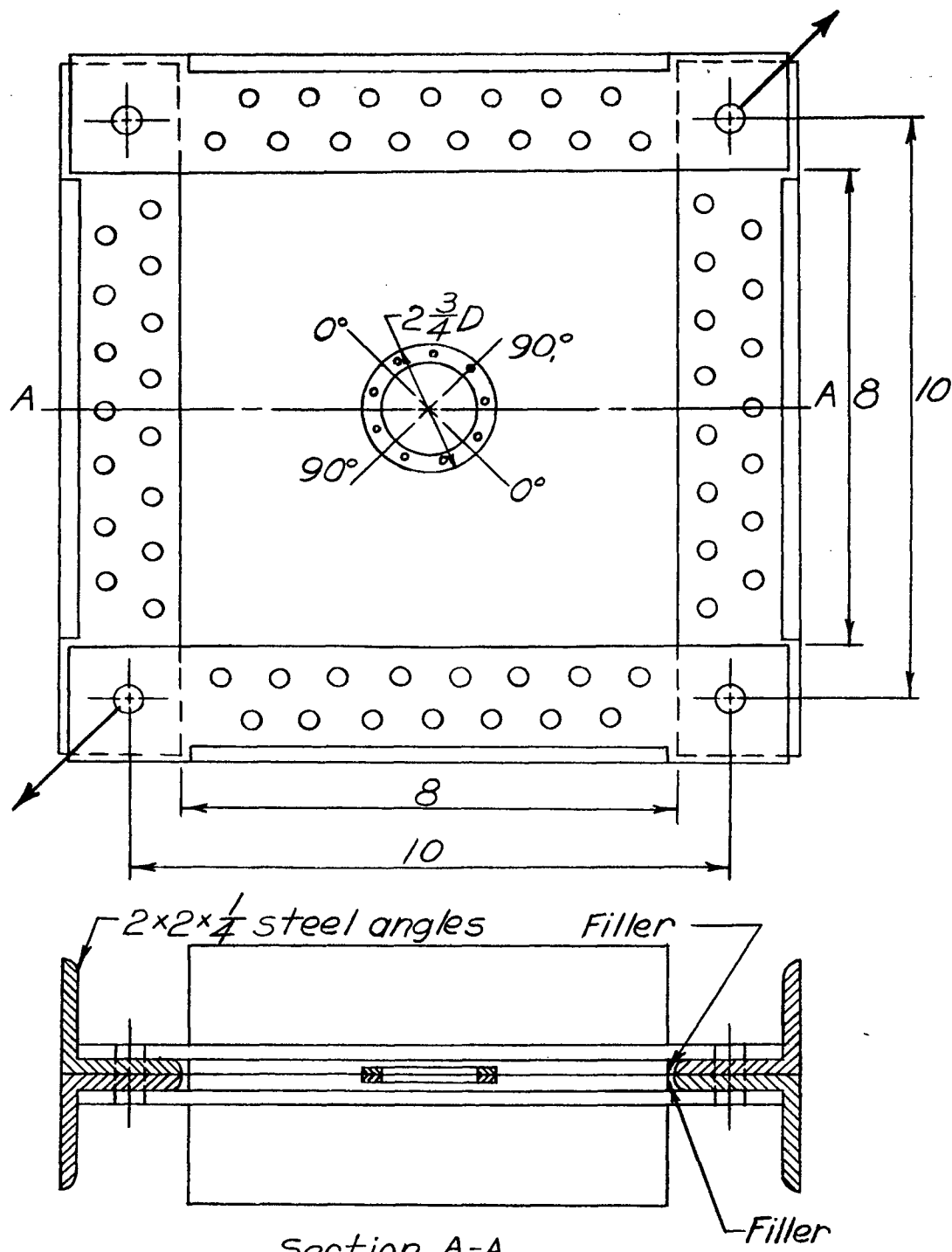
Figure 1.- Shear frame and specimen with reinforcing ring.
