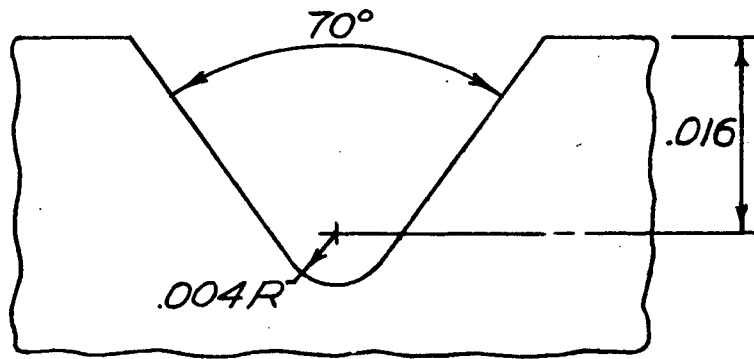
Figure 2.- File notch on edge of hole.
