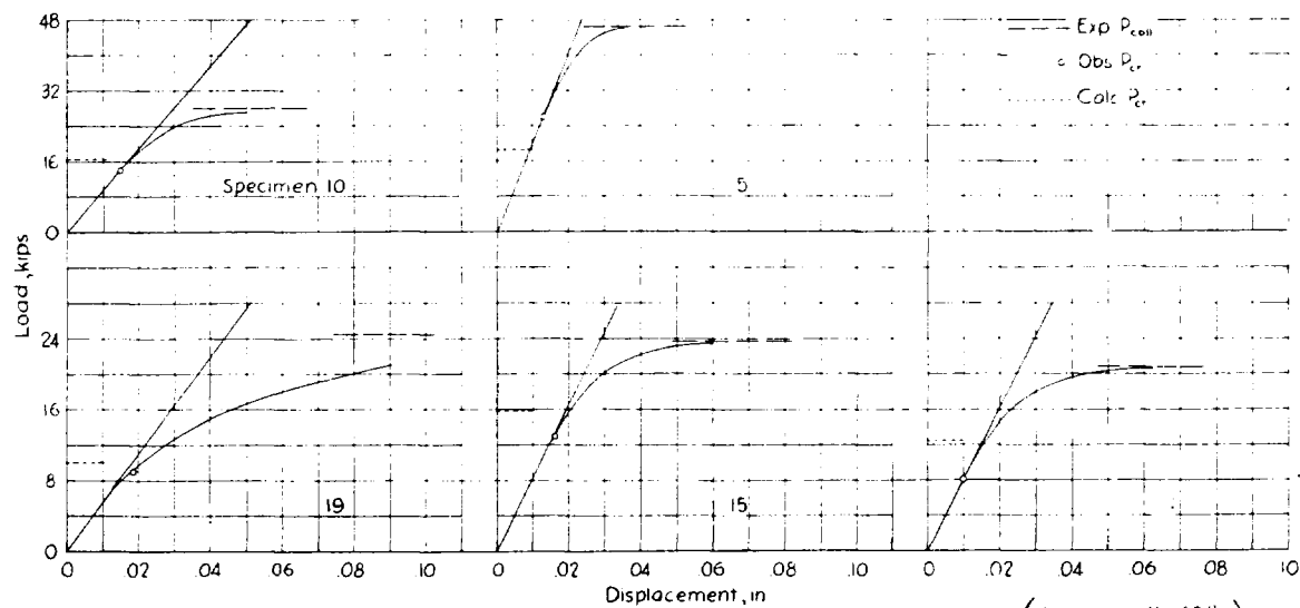
Figure 5.- Load-displacement curves for perforated webs.
