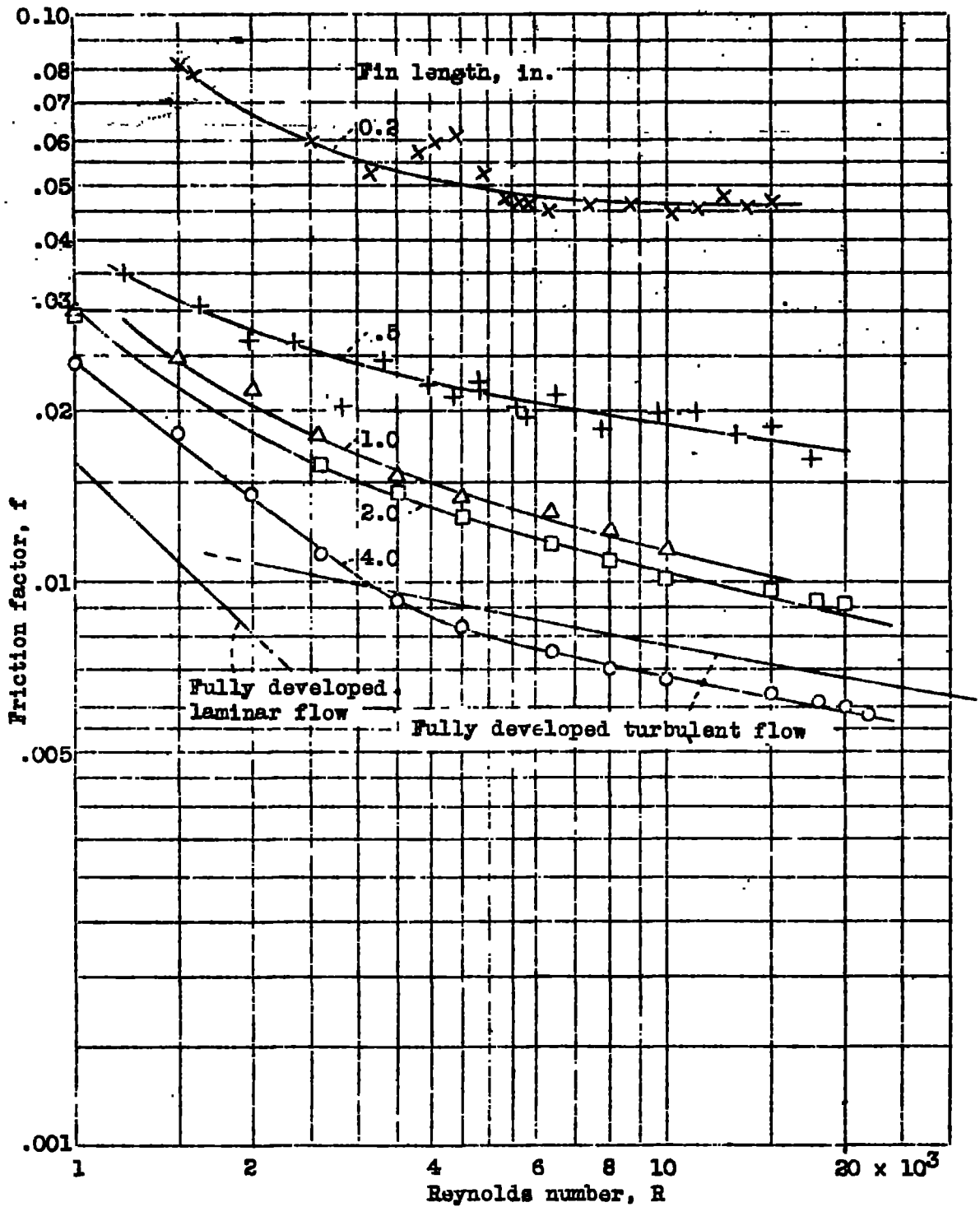
Figure 3.- Variation of friction factor with Reynolds number for the fin arrangements tested.
