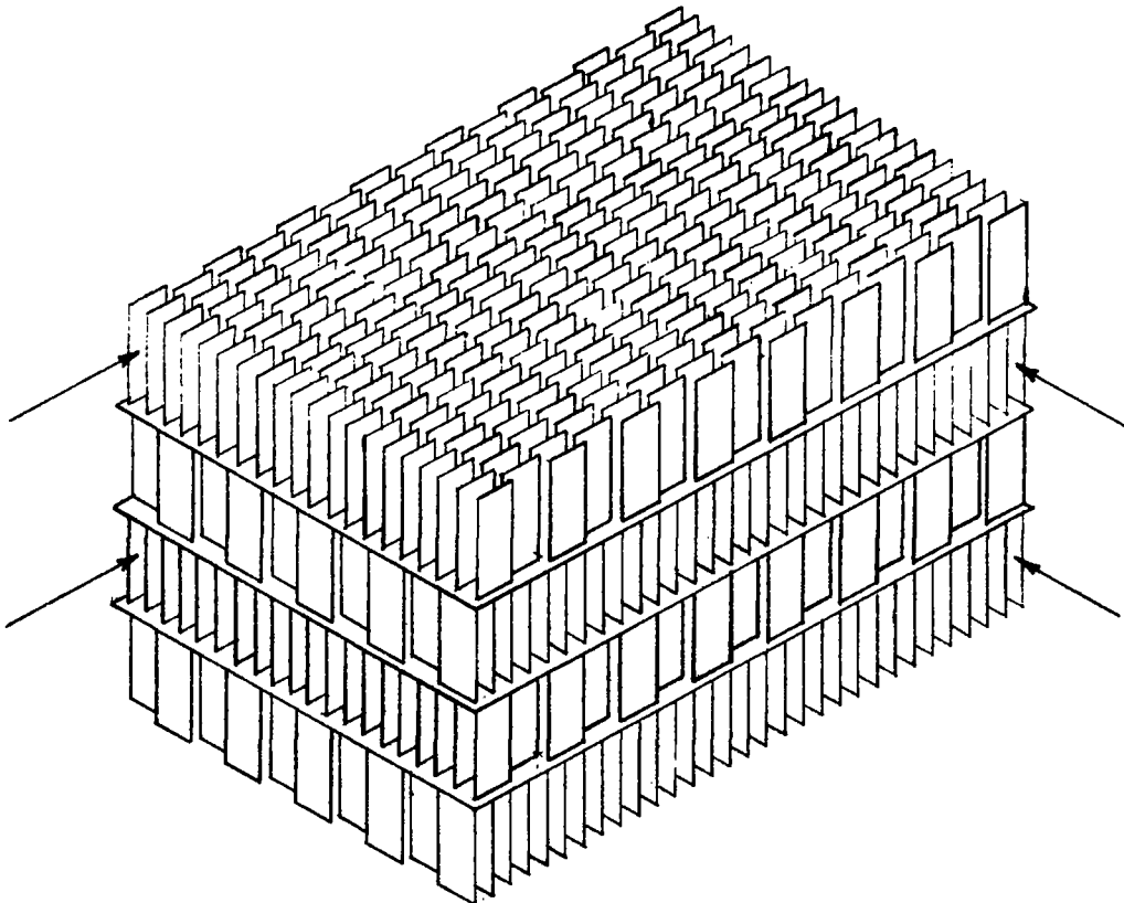
Figure 5.- Method of using staggered heat-transfer surfaces in a cross-flow heat exchanger.
