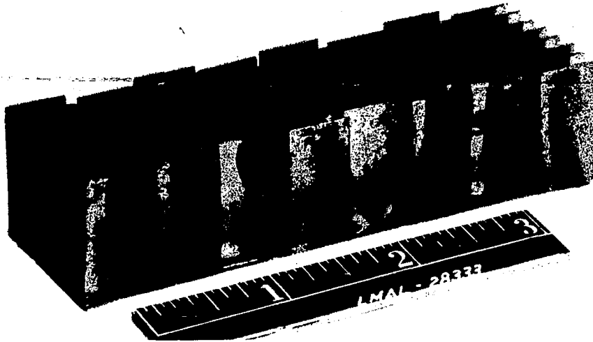
Figure 1.- Multiple-entrance heat-transfer system with 0.5 inch fins.
