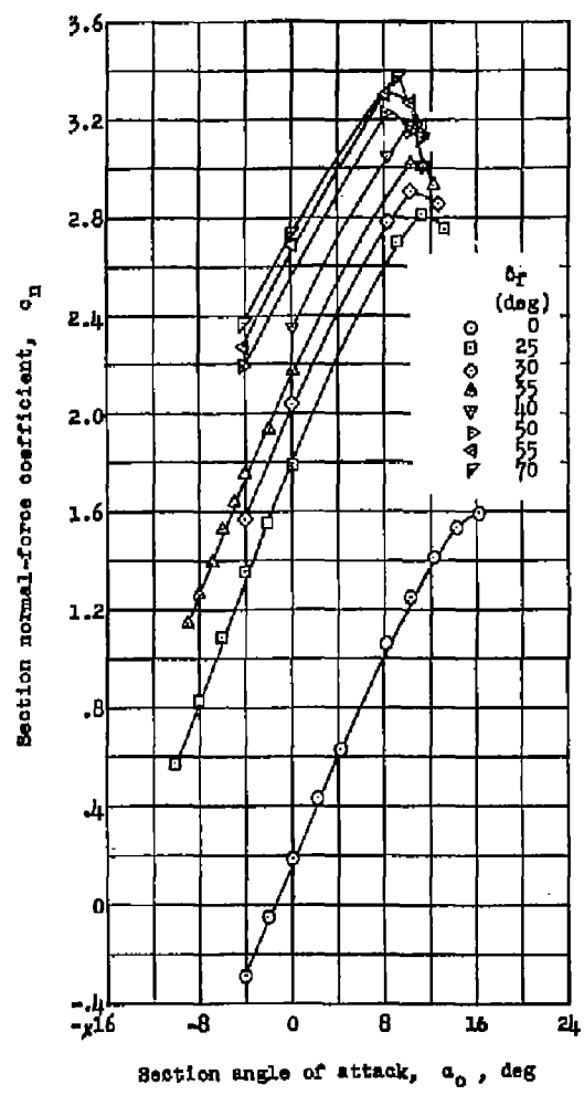
Figure 3.- Section normal-force and pitching-moment characteristics of an NACA 65(216)-215, \alpha = 0.8 airfoil section equipped with a double slotted flap. R = 6.3 \times 10^6 .
