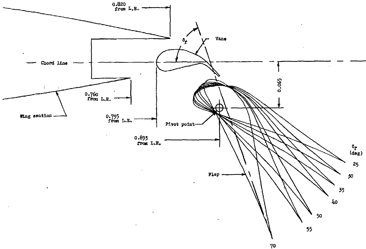
Figure 2.- Double slotted flap configurations on an NACA 65(216)-215, \alpha = 0.8 airfoil section.
