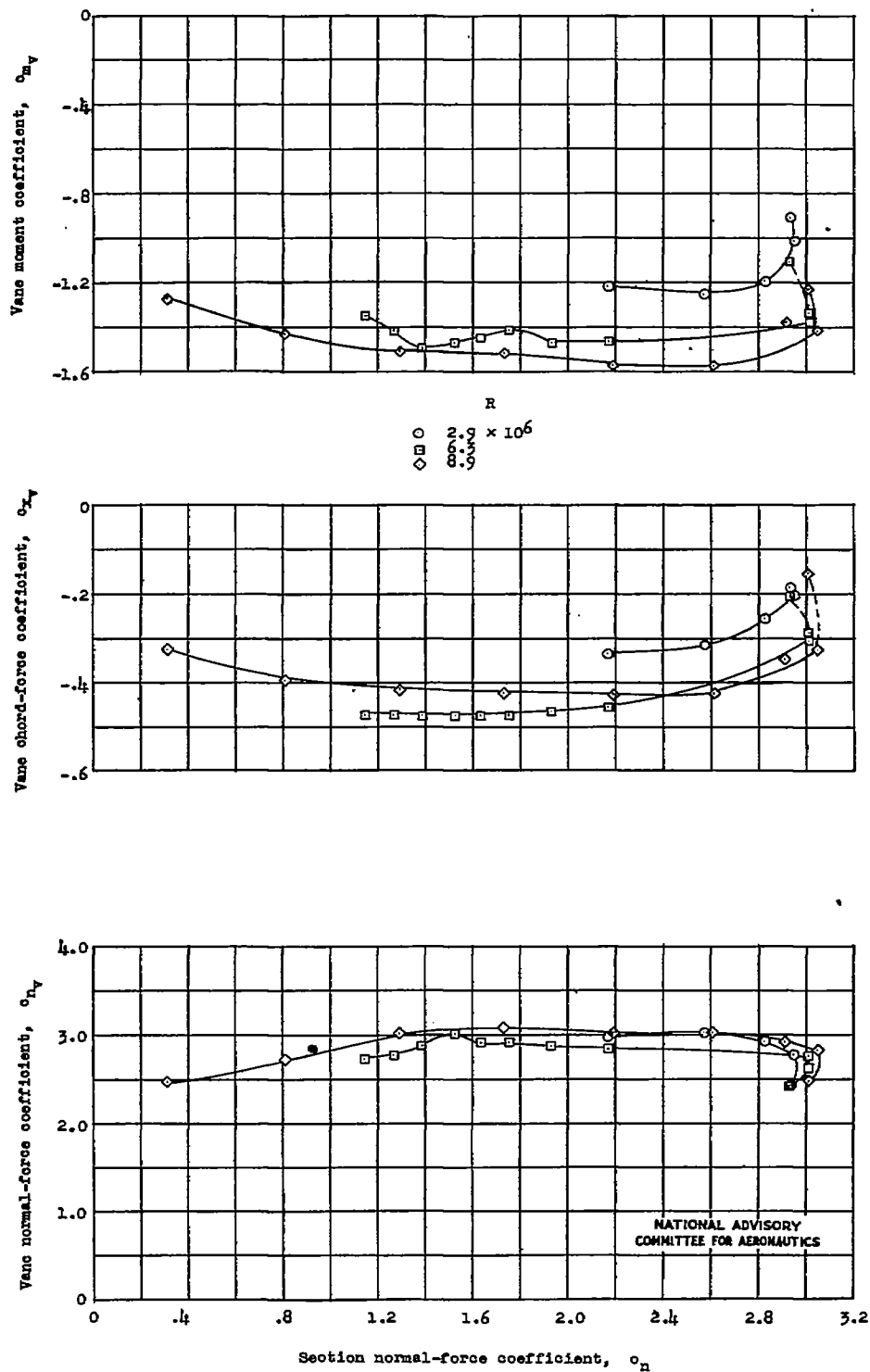
Figure 9.- Scale effect on vane characteristics of the NACA 65(216)-215, \alpha = 0.8^\circ airfoil section equipped with a double slotted flap. \delta_f = 35^\circ .
