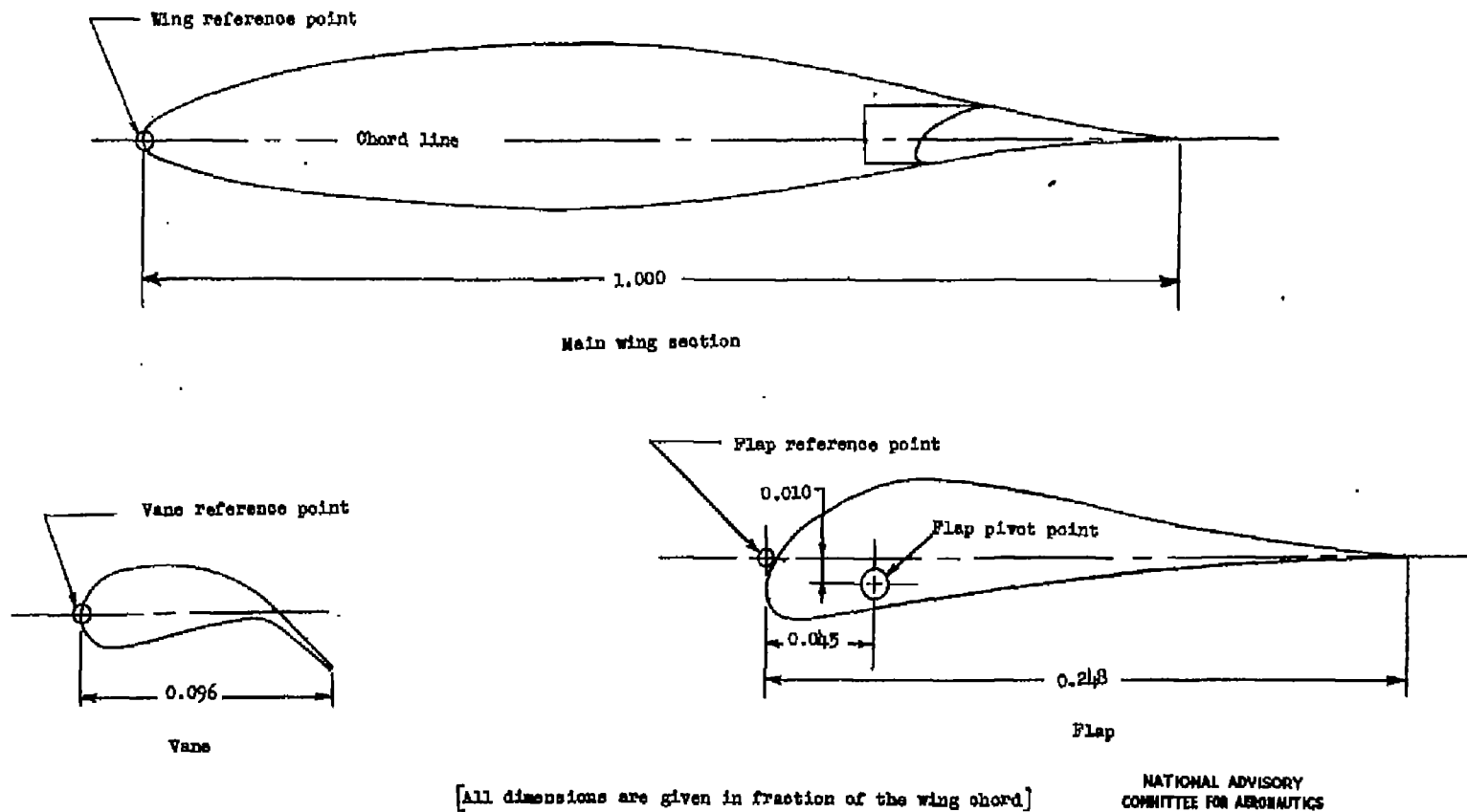
Figure 1.- Wing, vane, and flap of the NACA 65(216)-215, \alpha = 0.8 airfoil section.
