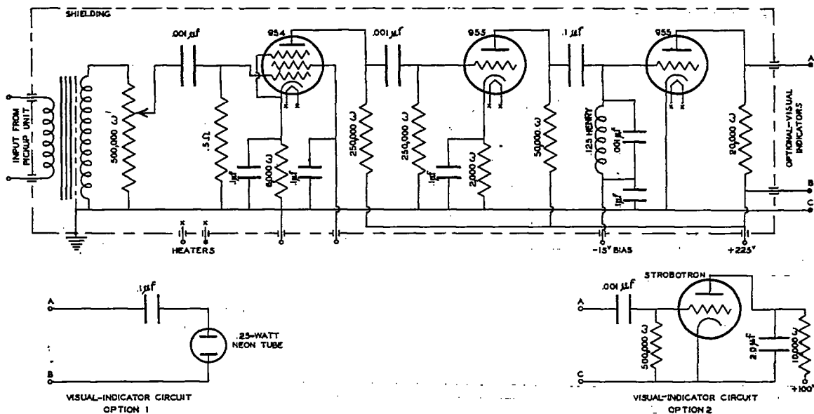
CIRCUIT DIAGRAM OF DETONATION-DETECTOR AMPLIFIER.
