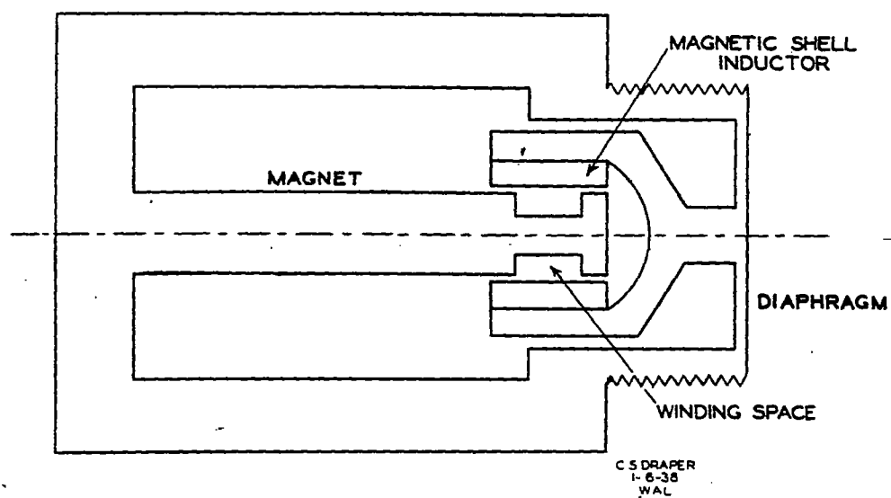
ELEMENTS OF INDICATOR WITH SHELL INDUCTOR GENERATOR
