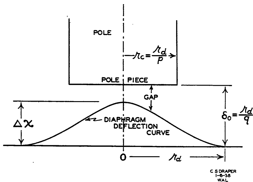
AIR GAP BETWEEN DIAPHRAGM AND FLAT POLE PIECE.
