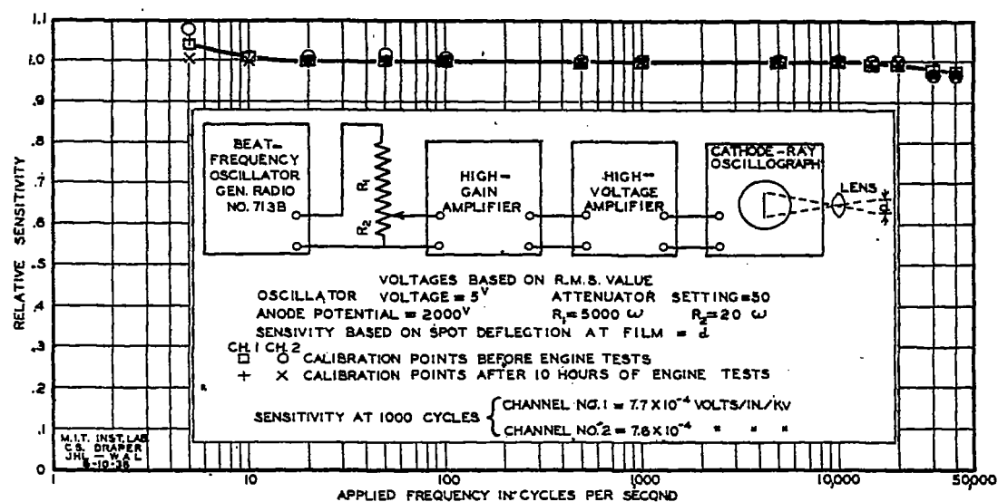
ELECTRICAL CALIBRATION OF AMPLIFIER-OSCILLOGRAPH SYSTEM. FIG. 26
