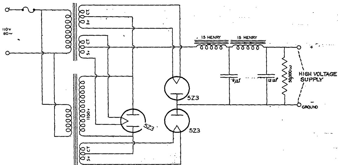
CIRCUIT DIAGRAM OF HIGH-VOLTAGE POWER SUPPLY.
