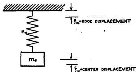
FIGURE 8.— EQUIVALENT SYSTEM FOR DIAPHRAGM.
