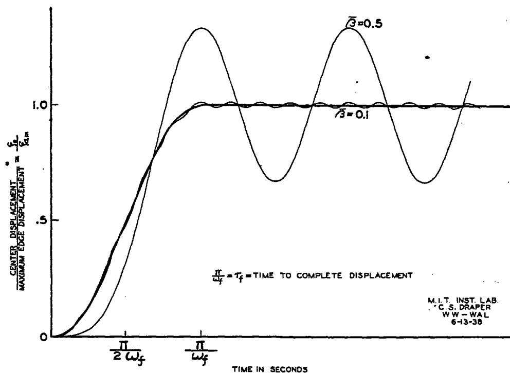
ABSOLUTE DISPLACEMENT OF DIAPHRAGM CENTER VS. TIME. FIG. 9
