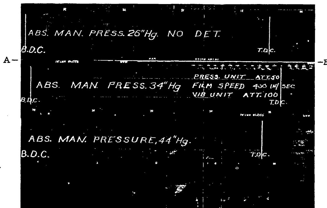
Fig. 35.- Effect of supercharging. (Continued on following page)
