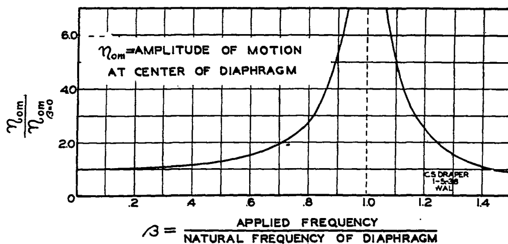
EFFECT OF FREQUENCY ON DIAPHRAGM DEFLECTION UNDER UNIFORM PRESSURE VARYING SINUSOIDALLY.
