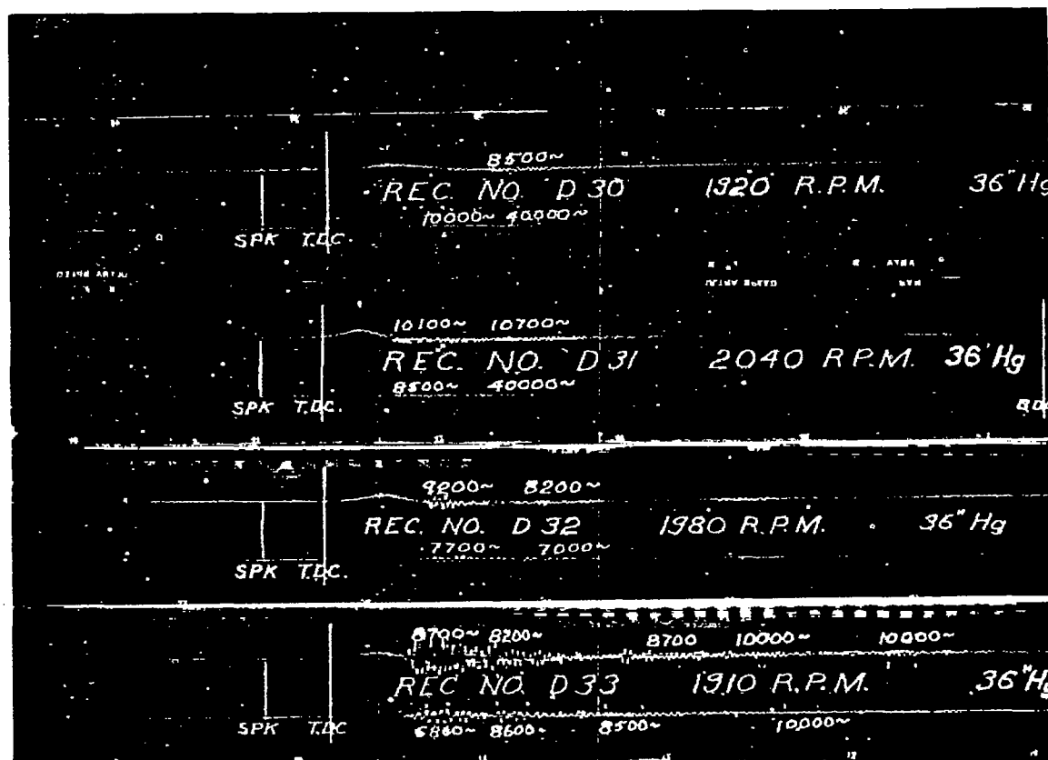
Fig. 36.- Effect of detonation.
