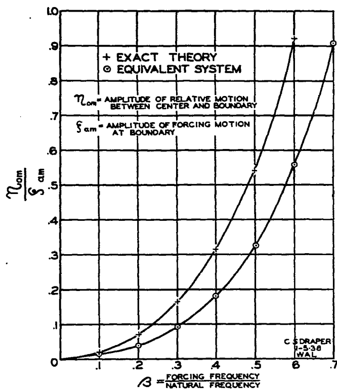
MOTION OF CLAMPED DIAPHRAGM DUE TO SIMPLE HARMONIC MOTION OF BOUNDARY
