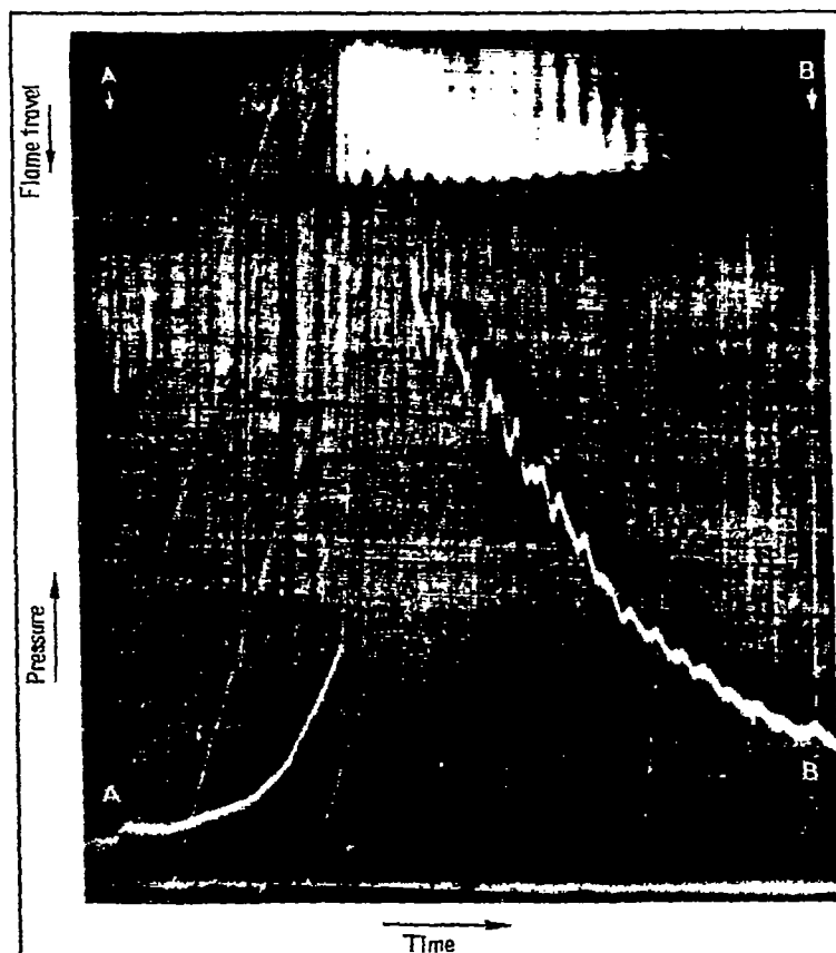
Figure 1.- The relationship between the frequencies of the shock waves on the flame photographs and the vibrations recorded on the pressure cards at an engine speed of 1,500 r.p.m. Knock induced with isopropyl nitrite. Fuel, petrol; Full throttle; Spark advance, 30 deg.; A, ignition; B, 61 deg. after ignition.
