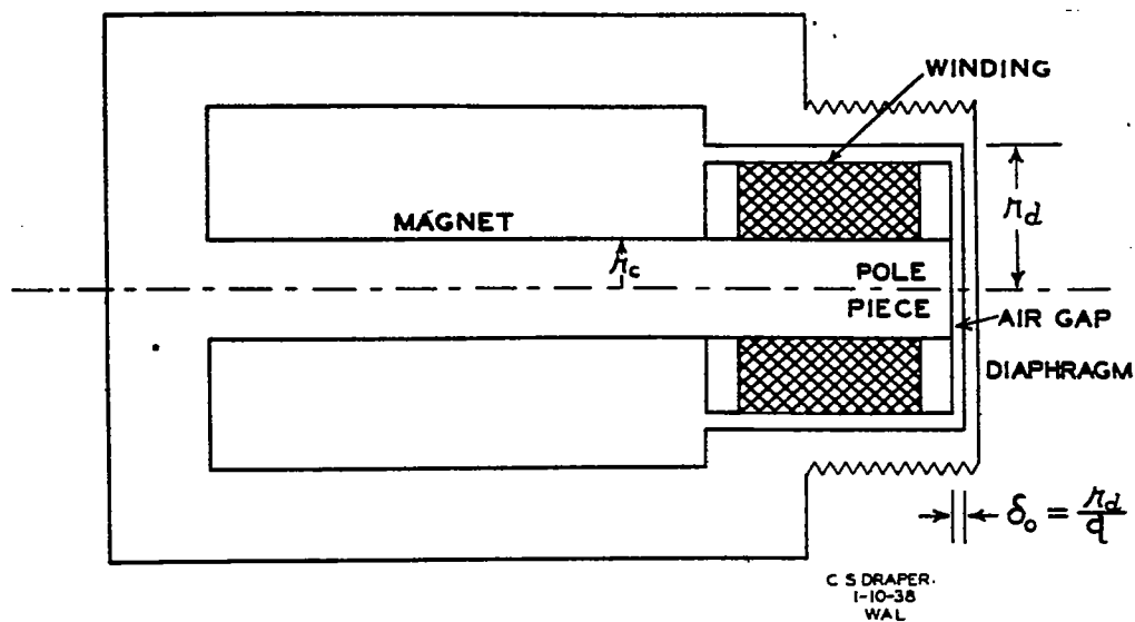
ELEMENTS OF INDICATOR WITH FLAT-DIAPHRAGM GENERATOR.
