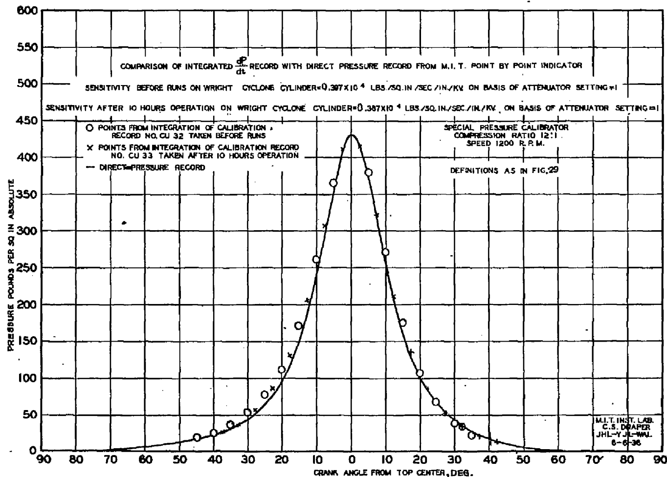
OVERALL CALIBRATION OF VIBRATION UNIT CONNECTED TO AMPLIFIER CHANNEL NO. 2 FIG. 30
