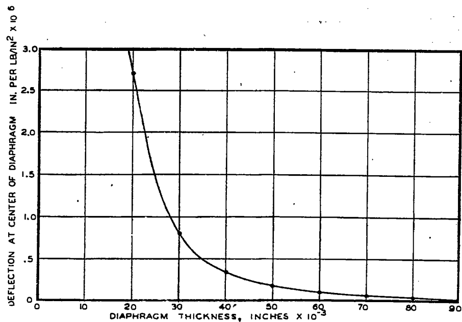
ELASTIC COEFFICIENT OF CIRCULAR STEEL DIAPHRAGMS.
