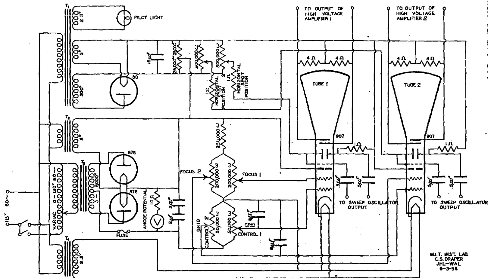
CIRCUIT DIAGRAM OF TWO-ELEMENT CATHODE-RAY OSCILLOGRAPH AND POWER SUPPLY.
