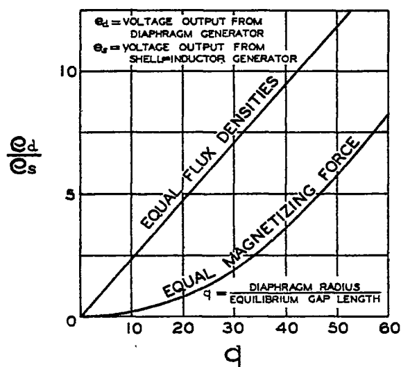
FIGURE 6.— RATIO BETWEEN GENERATED VOLTAGE FROM DIAPHRAGM AND SHELL INDUCTOR GENERATORS FOR EQUAL VELOCITIES.
