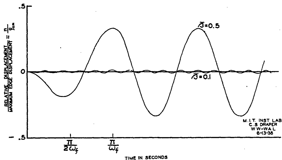
DISPLACEMENT OF DIAPHRAGM CENTER RELATIVE TO ITS EDGES VS. TIME.
