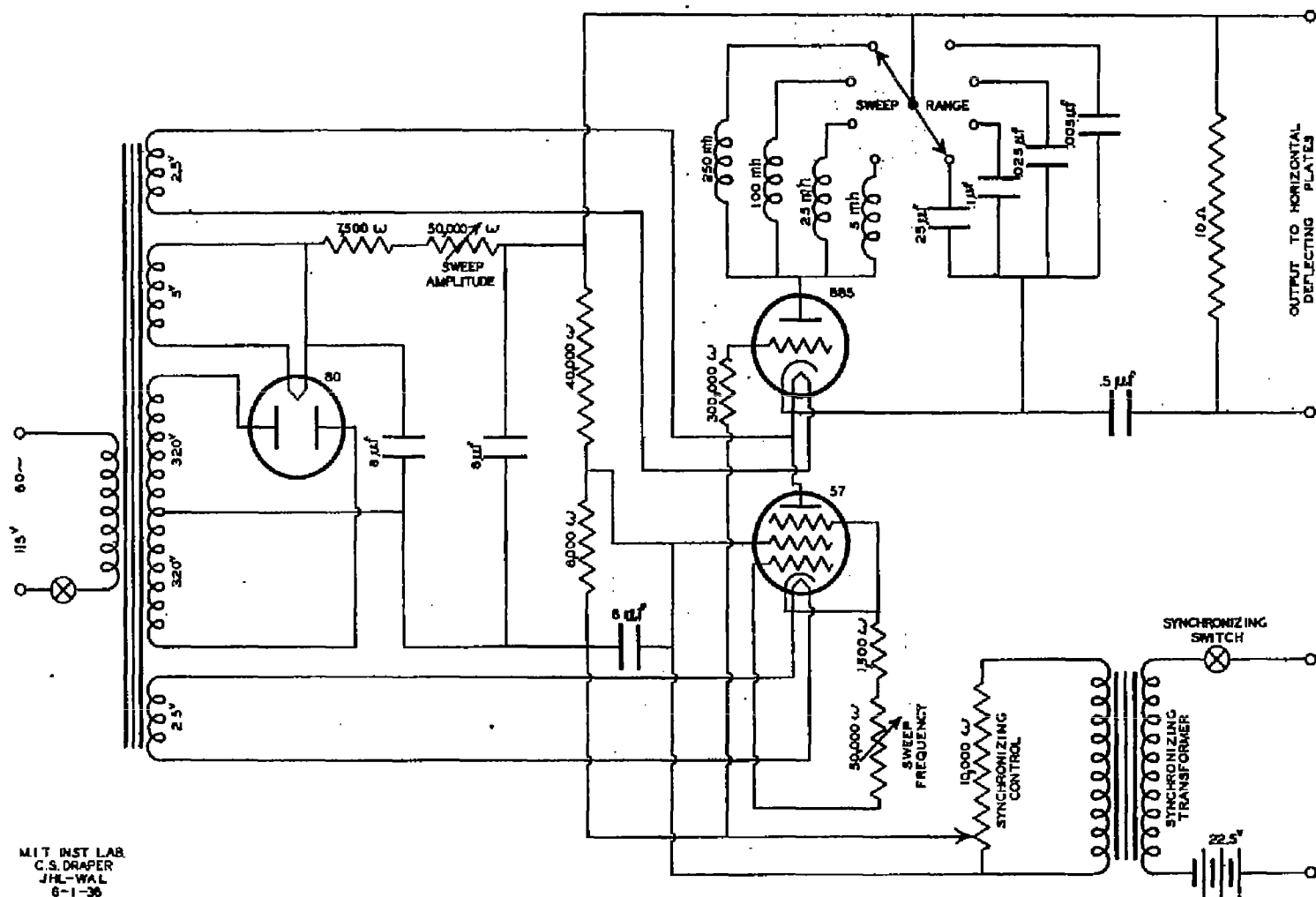
CIRCUIT DIAGRAM OF SWEEP OSCILLATOR.
