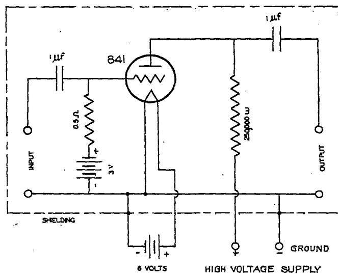
CIRCUIT DIAGRAM OF HIGH VOLTAGE AMPLIFIER.
