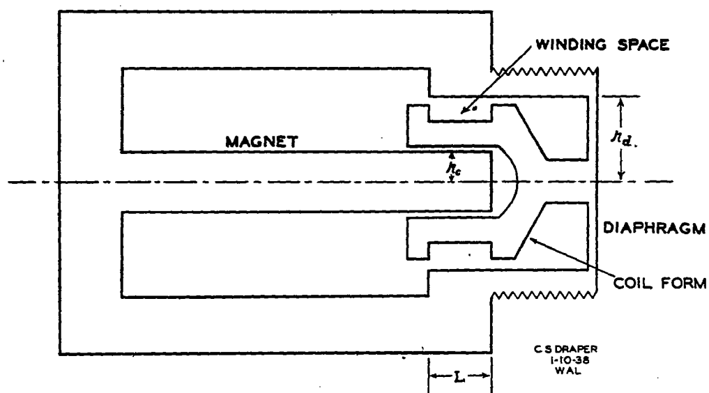
ELEMENTS OF INDICATOR WITH MOVING-COIL GENERATOR
