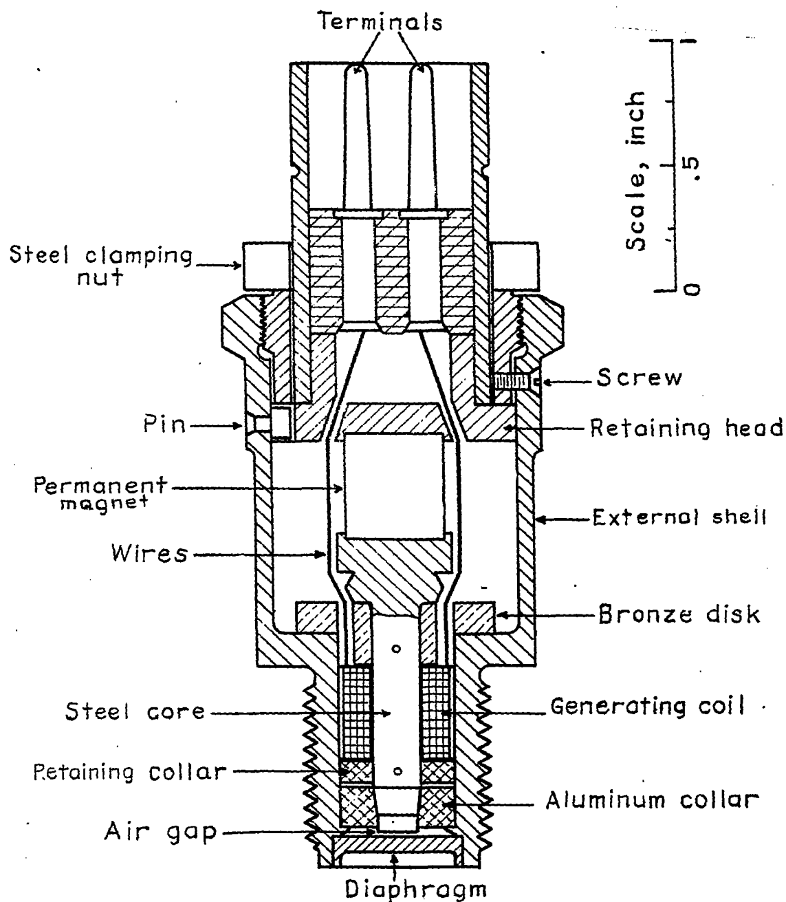
PICK UP UNIT FOR RATE OF CHANGE OF PRESSURE
