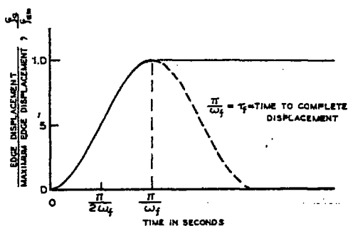
FIGURE 7.— TYPICAL FORCING DISPLACEMENT VS. TIME.
