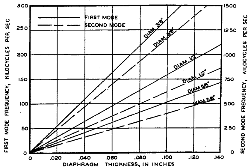
NATURAL FREQUENCY vs. THICKNESS FOR CIRCULAR STEEL DIAPHRAGMS.
