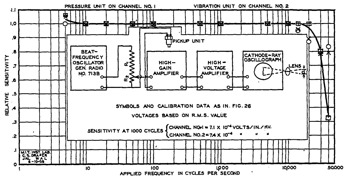
ELECTRICAL CALIBRATION OF AMPLIFIER-OSCILLOGRAPH SYSTEM WITH PICKUP UNITS. FIG. 27
