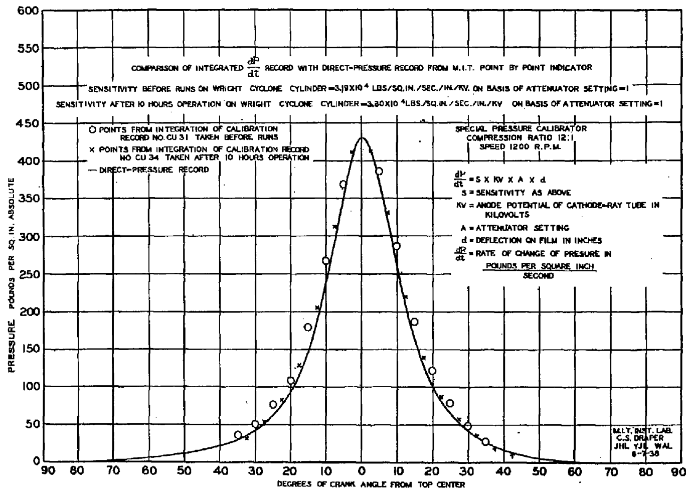
OVERALL CALIBRATION OF PRESSURE UNIT CONNECTED TO AMPLIFIER CHANNEL NO. 1.
