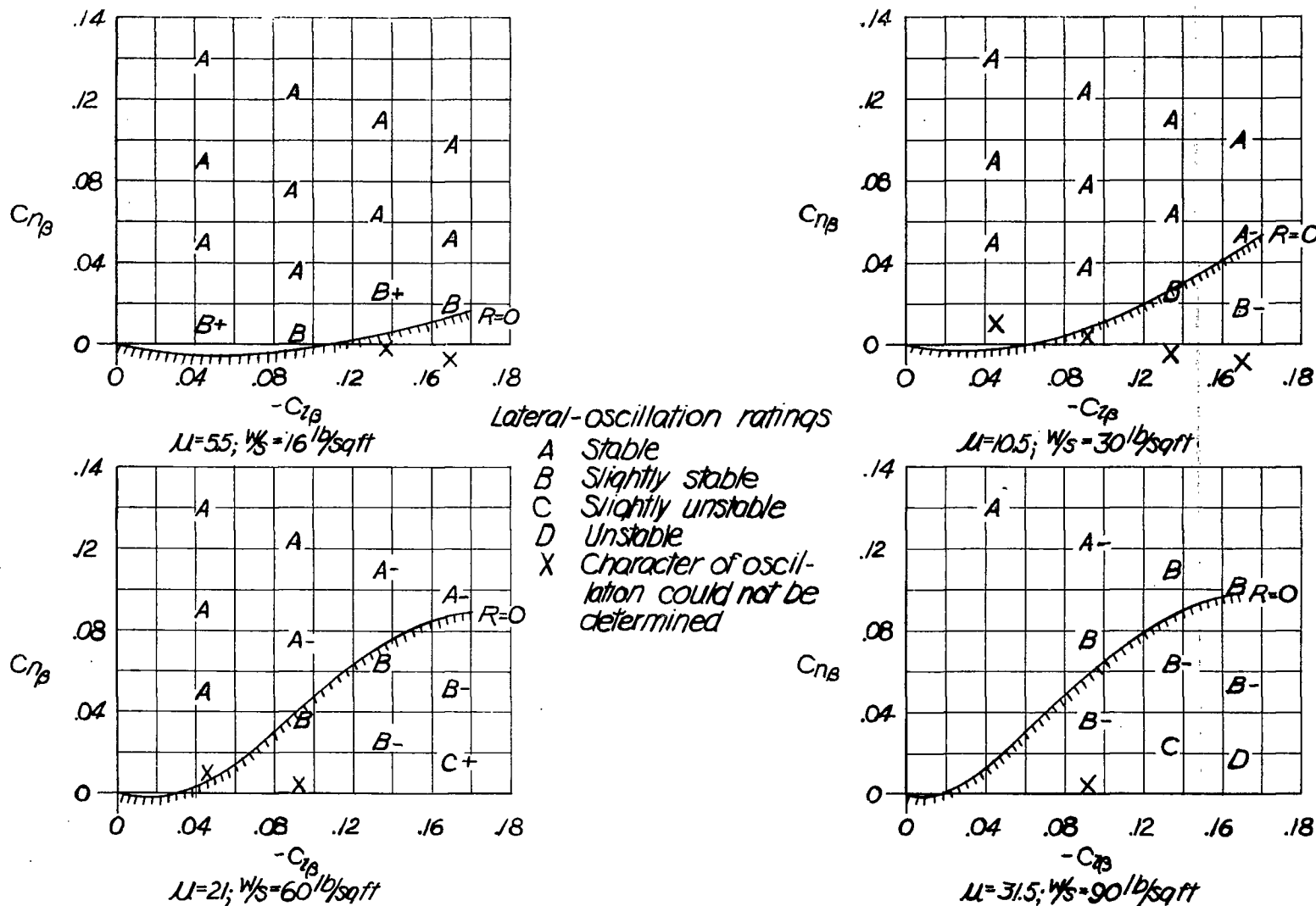
FIGURE 6.- Ratings for damping of lateral oscillation for various wing loadings and model configurations.
