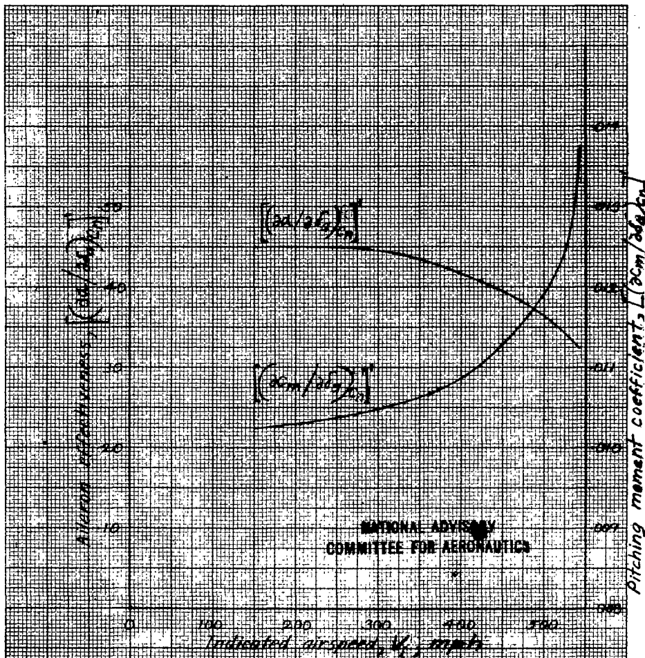
Figure 2. Variation with indicated airspeed of parameters \left(\frac{da}{d\delta}\right)_{in} and \left(\frac{\delta c_m}{\delta \delta}\right)_{in} for section at mid-aileron span. From wind-tunnel results. Modified Frise aileron, \delta = 34^\circ , lift coefficient and Mach number appropriate for P-47G-1 RE airplane at 4000 feet altitude. Data from NACA 8-foot high-speed tunnel.
