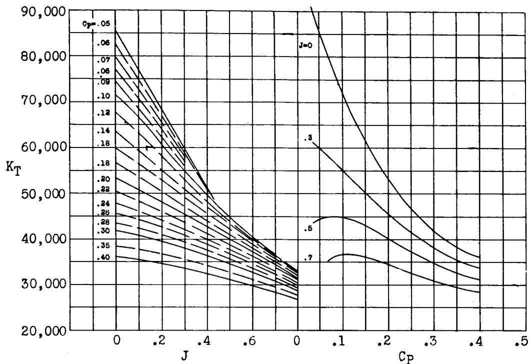
Figure 19.- 3155 propeller III dual rotation. AF \times \text{number of blades} = 650 .
