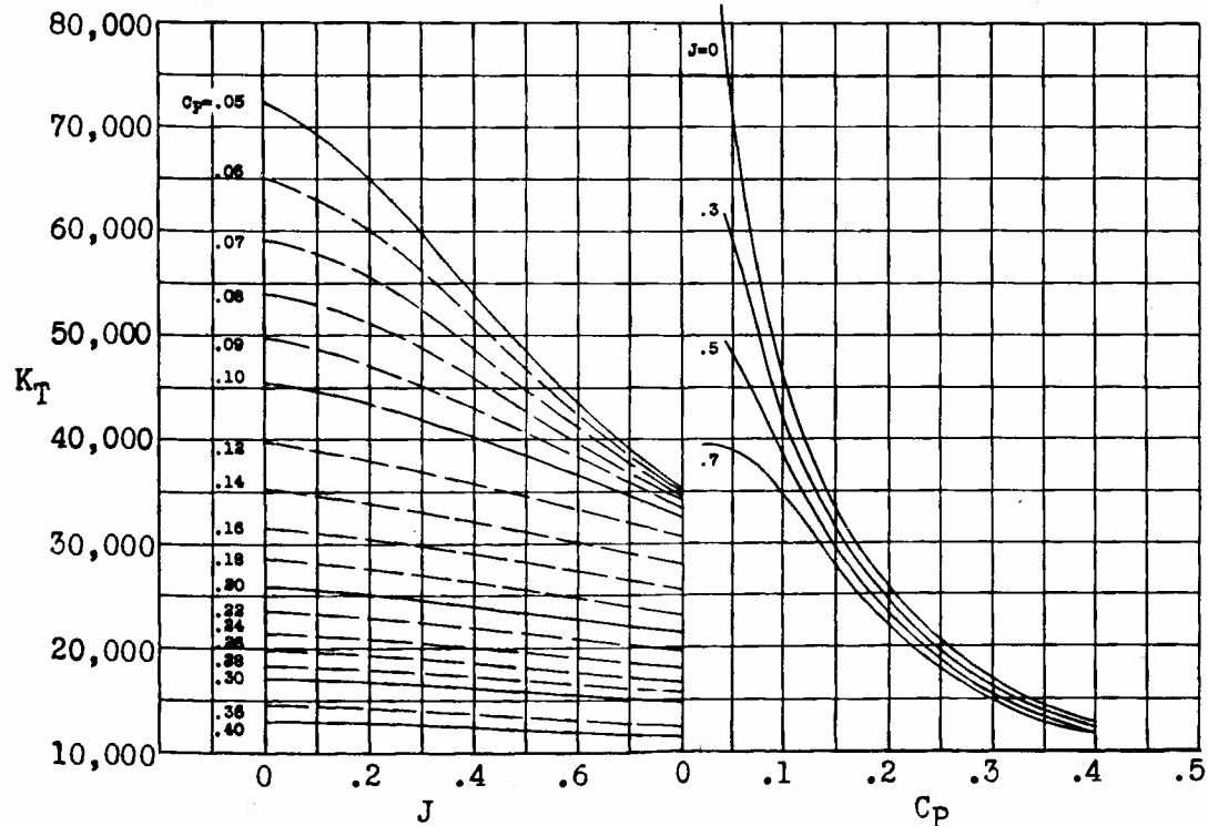
Figure 6.- 3155 propeller III single rotation. AF \times number of blades = 200.
