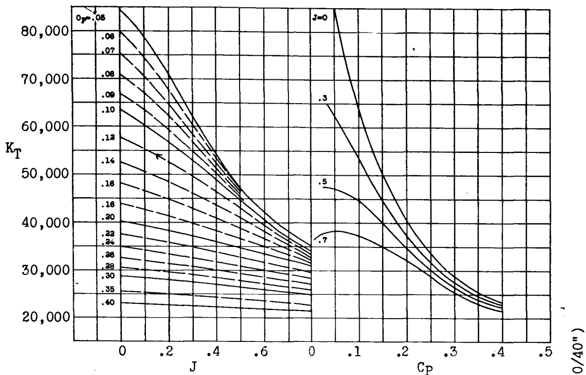
Figure 17.- 3155 propeller III dual rotation. AF \times \text{number of blades} = 350 .
