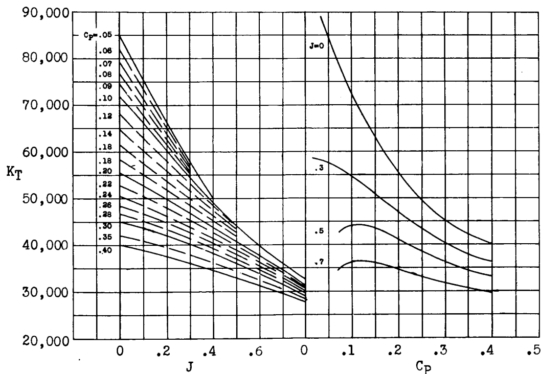
Figure 20.- 3155 propeller III dual rotation. AF \times \text{number of blades} = 800 .
