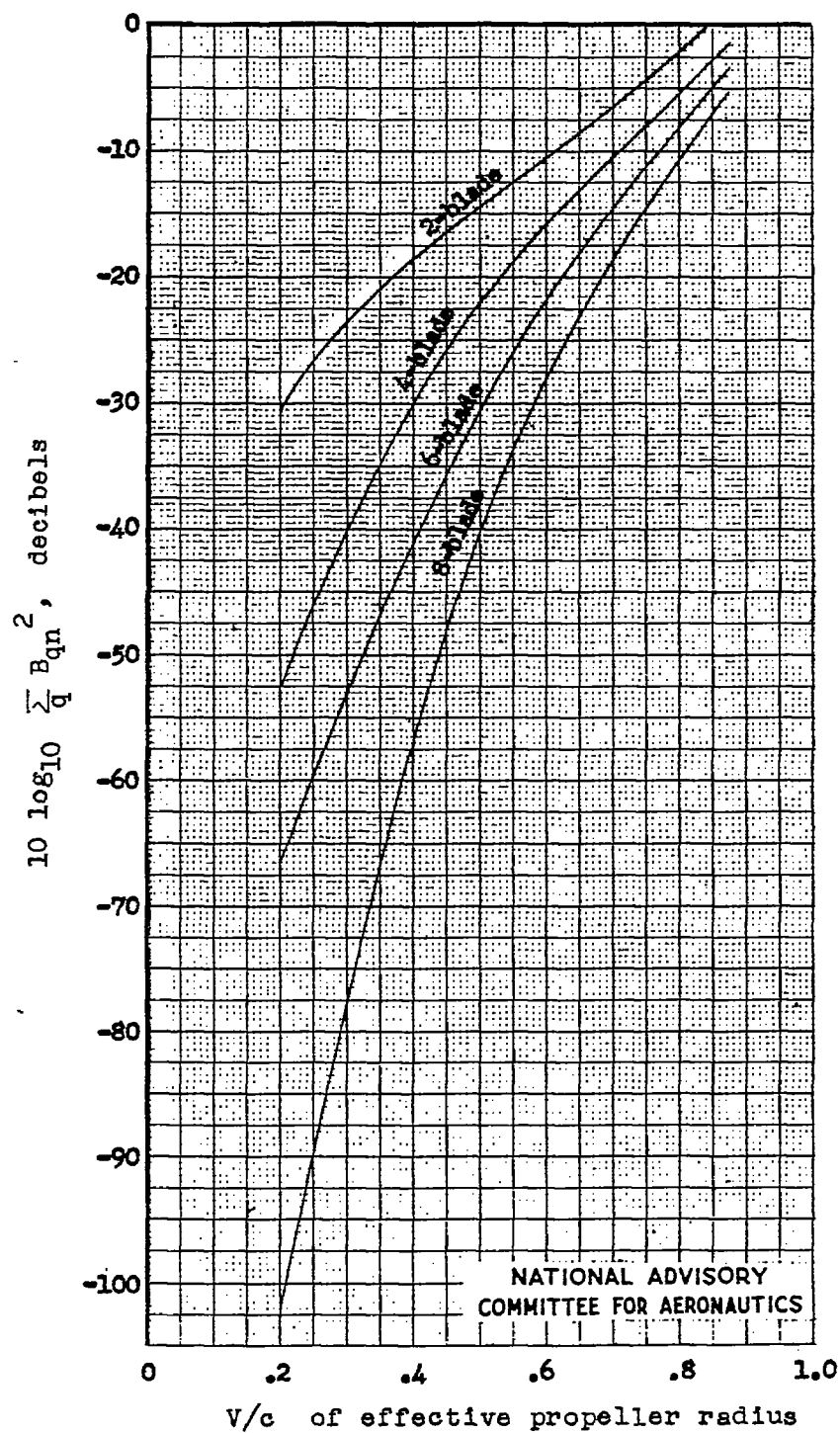
Figure 3.- Function 10 \log_{10} \sum B_{qn}^2 for various numbers of propeller blades.
