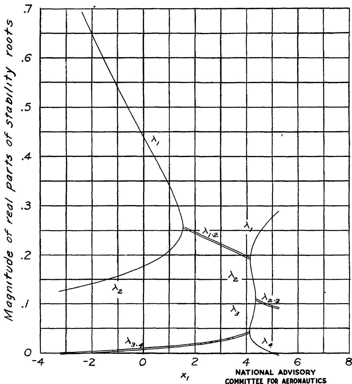
Figure 14.- Variation of real parts of stability roots with x_1 . \Gamma = 30^\circ ; S_2 = S_1 ; \epsilon = 0 ; l = 10.0 c_1 ; z_0 = 1.74 c_1 ; K_Y = 6.67 c_1 ; z_1 = 10.00 c_1 .
