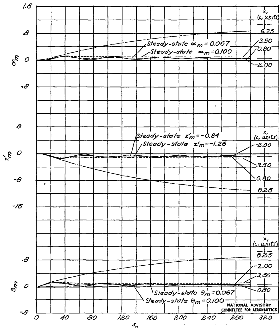
Figure 21.- Indicial responses for unit C_m disturbance.
