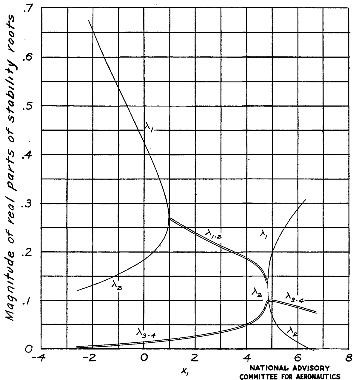
Figure 15.- Variation of real parts of stability roots with x_1 for increased vertical damping. S_2 = S_1 ; \epsilon = 0 ; l = 10.0c ; K_y = 6.67c ; z_1 = 5.00c .
