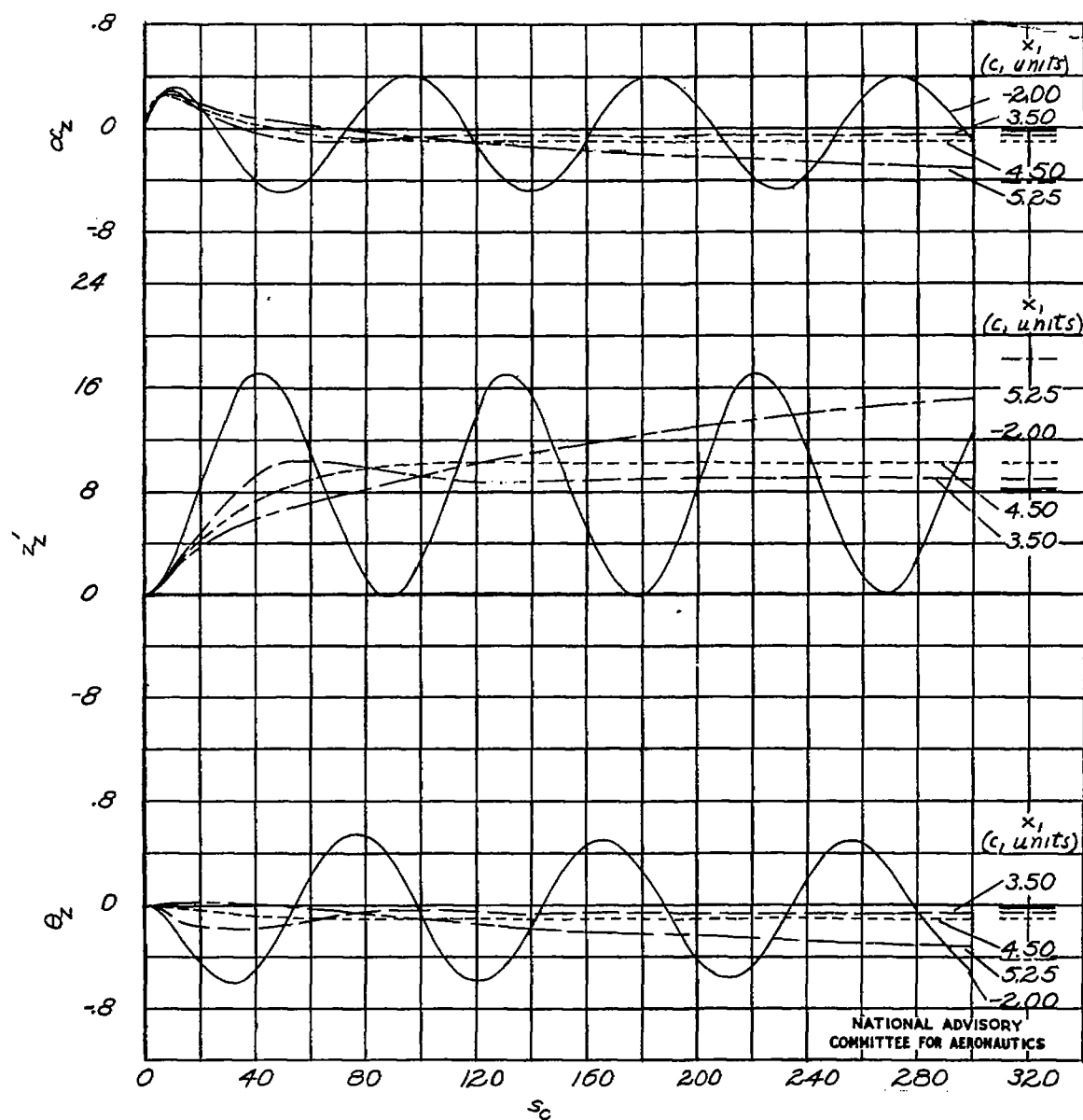
Figure 18.—Indicial responses for unit C_z disturbance. \Gamma=30^\circ ; S_2=S_1 ; \epsilon=0 ; \lambda=10.0c_1 ; z_0=1.74c_1 ; K_Y=0.67c_1 ; z_1=5.00c_1 ; x_1=-2.00c_1 , 3.50c_1 , 4.50c_1 , or 5.25c_1 .
