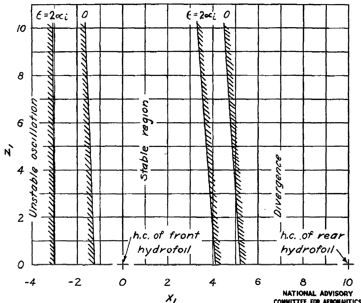
Figure 4.- Stable regions for two downwash angles. \Gamma = 0^\circ ; S_2 = S_1 ; \lambda = 10.0c ; Z_0 = 1.00c ; K_Y = 6.67c .
