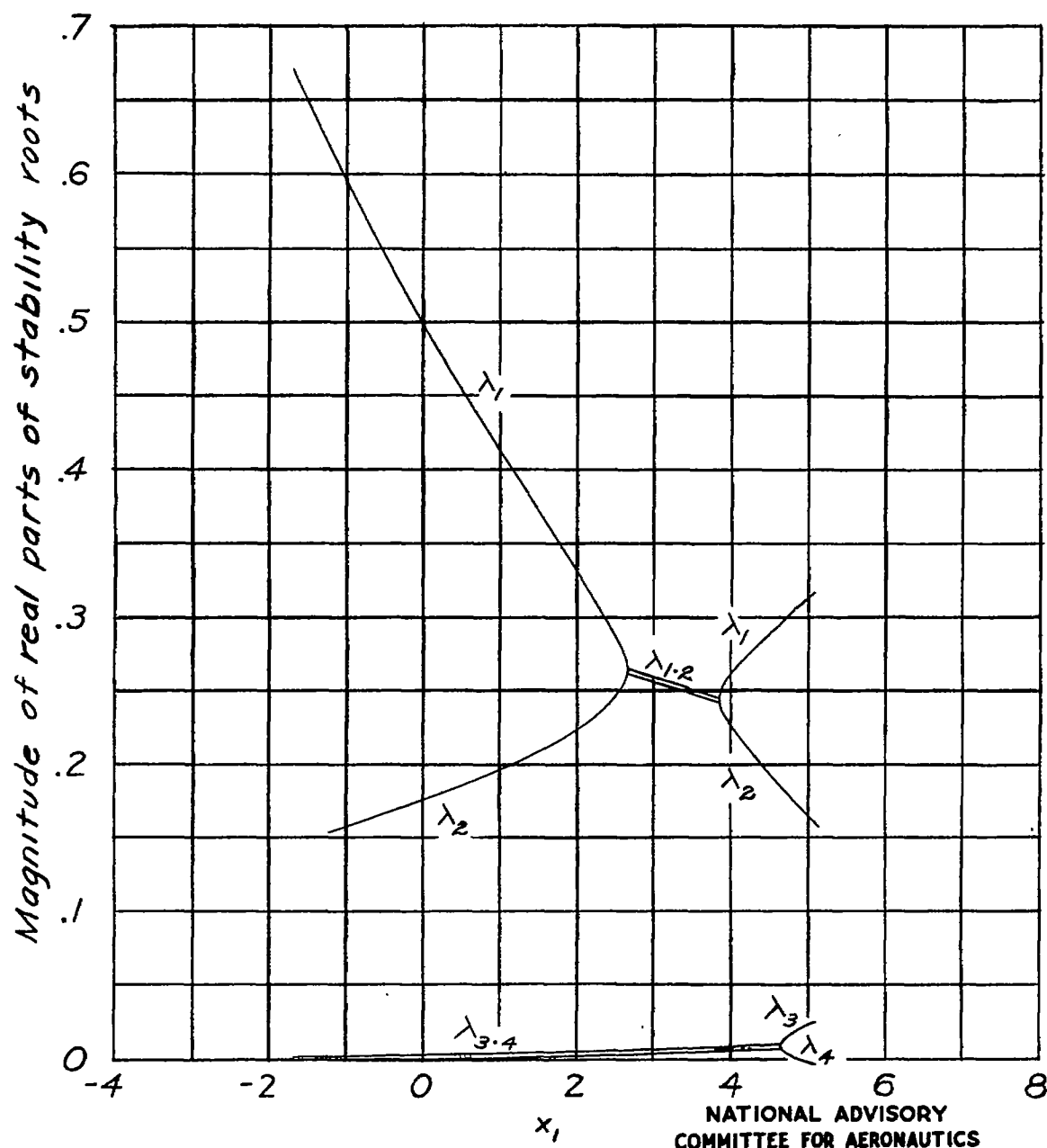
Figure 12.- Variation of real parts of stability roots with x_1 . \Gamma = 0^\circ ; S_2 = S_1 ; \epsilon = 0 ; l = 10.0 c_1 ; z_0 = 1.00 c_1 ; K_Y = 6.67 c_1 ; z_1 = 5.00 c_1 .
