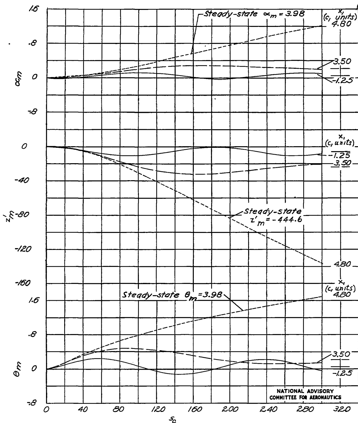
Figure 17.- Indicinal responses for unit C_m disturbance. \Gamma = 0^\circ ; S_2 = S_1 ; \epsilon = 0 ; \lambda = 10.0 c_i ; z_0 = 1.00 c_i ; K_Y = 6.67 c_i ; z_i = 5.00 c_i ; x_1 = -1.25 c_i , 3.50 c_i , or 4.80 c_i .
