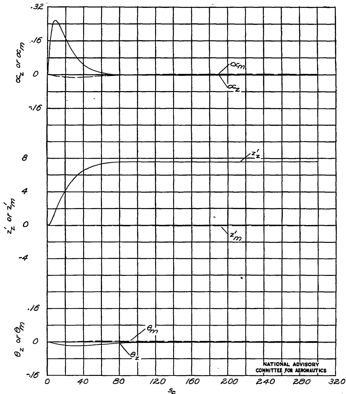
Figure 23.—Indicial responses for unit C_z and unit C_m disturbances. \Gamma=30^\circ ; S_2=S_1 ; \epsilon=0 ; l=100.0c_1 ; z_0=1.74c_1 ; K_Y=6.67c_1 ; z_1=5.00c_1 ; x_1=35.00c_1 .
