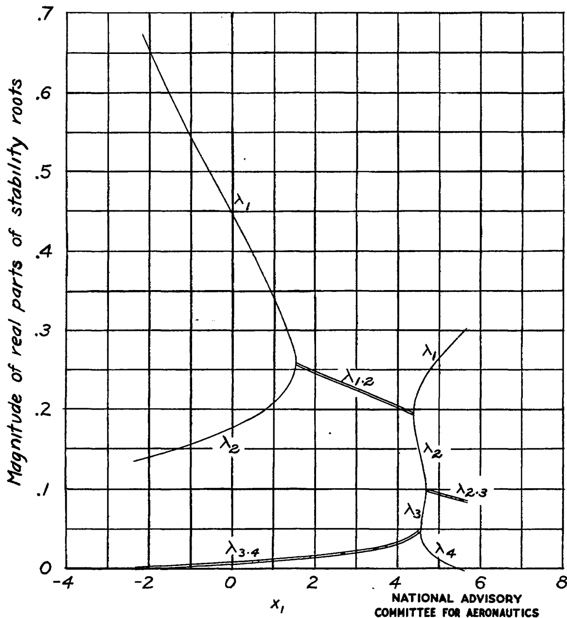
Figure 10.- Variation of real parts of stability roots with x_1 . \Gamma = 30^\circ ; S_2 = S_1 ; \epsilon = 0 ; l = 10.0 c_1 ; z_0 = 1.74 c_1 ; K_y = 6.67 c_1 ; z_1 = 5.00 c_1 .
