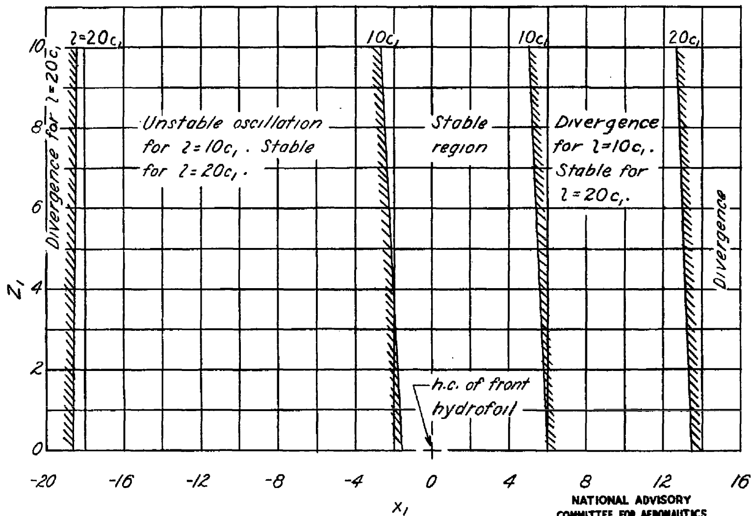
Figure 8.- Stable regions for two longitudinal spacings. \Gamma = 30^\circ ; S_2 = S_1 ; \epsilon = 0 ; z_0 = 1.74c_1 ; K_y = 6.67c_1 .
