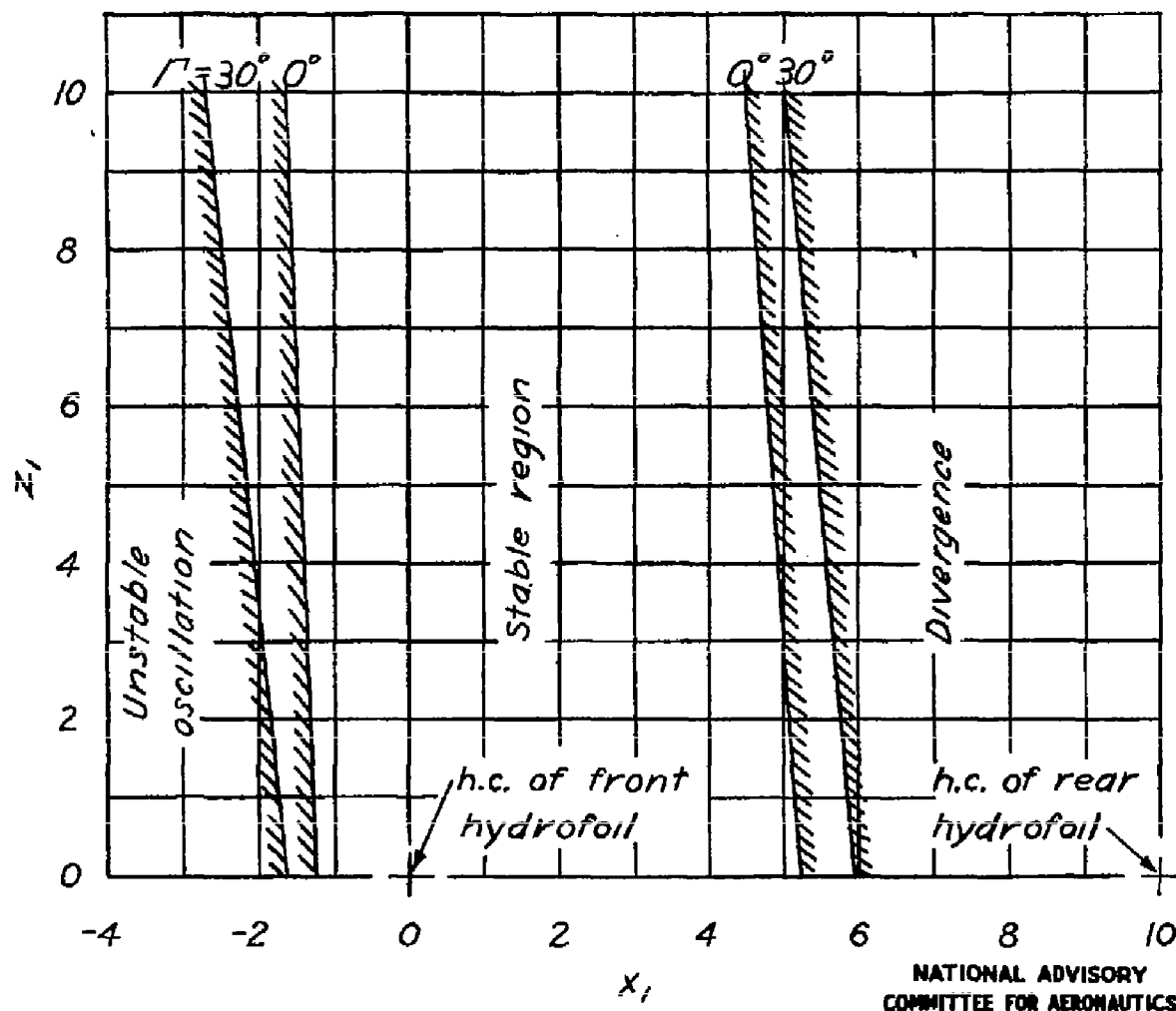
Figure 6.- Stable regions for two dihedral angles. S_x = S_1 ; \epsilon = 0 ; l = 10.0 c_1 ; z_0 = 1.00 c_1 for \Gamma = 0^\circ , and 1.74 c_1 for \Gamma = 30^\circ ; K_y = 6.67 c_1 .
