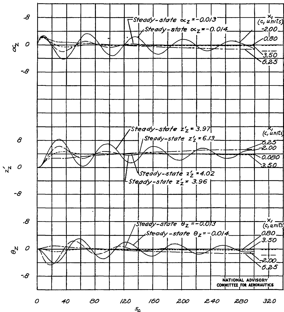
Figure 20.- Indicial responses for unit C_z disturbance.
