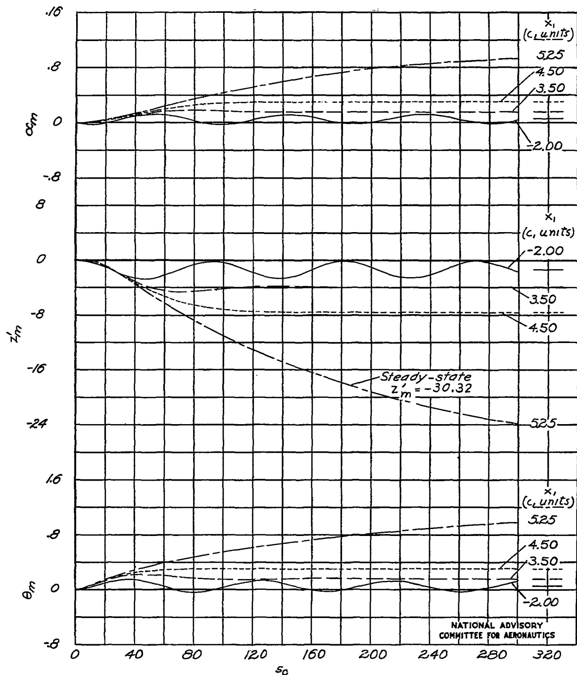
Figure 19.- Indicial responses for unit C_m disturbance. \Gamma = 30^\circ ; S_2 = 5 ; \epsilon = 0 ; l = 10.0c_1 ; z_0 = 1.74c_1 ; K_Y = 6.67c_1 ; z_1 = 5.00c_1 ; x_1 = -2.00c_1 , 3.50c_1 , 4.50c_1 , or 5.25c_1 .
