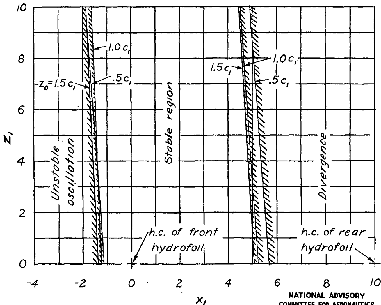
Figure 5.- Stable regions for three immersion depths. \Gamma = 0^\circ ; S_2 = S_1 ; \epsilon = 0 ; l = 10.0 c_l ; K_Y = 6.67 c_l .
