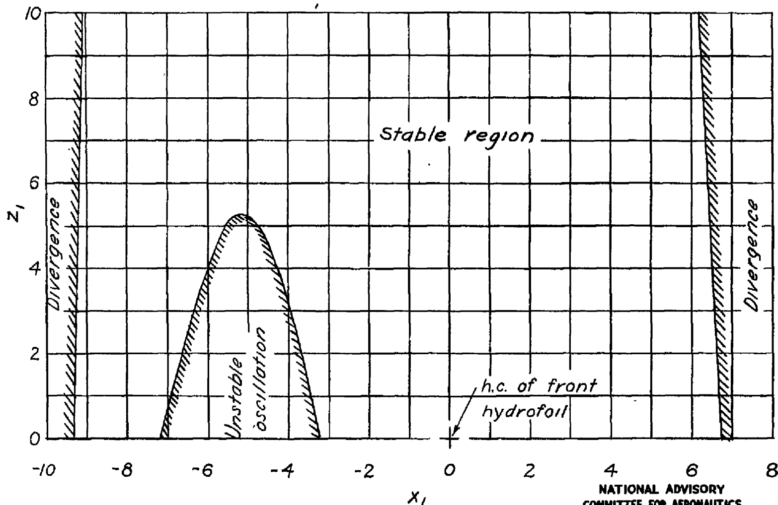
Figure 7.- Stable region with \partial C_L / \partial z' double that for \Gamma = 30^\circ
