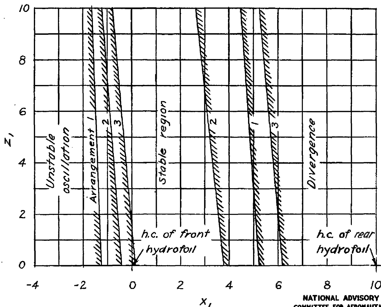
Figure 3.- Stable regions for three area distributions. \Gamma=0^\circ ; \epsilon=0 ; l=10.0c ; z_0=1.00c ; K_Y=6.67c . (For this figure c , is the chord for arrangement 1, in which the two hydrofoils are identical.)
