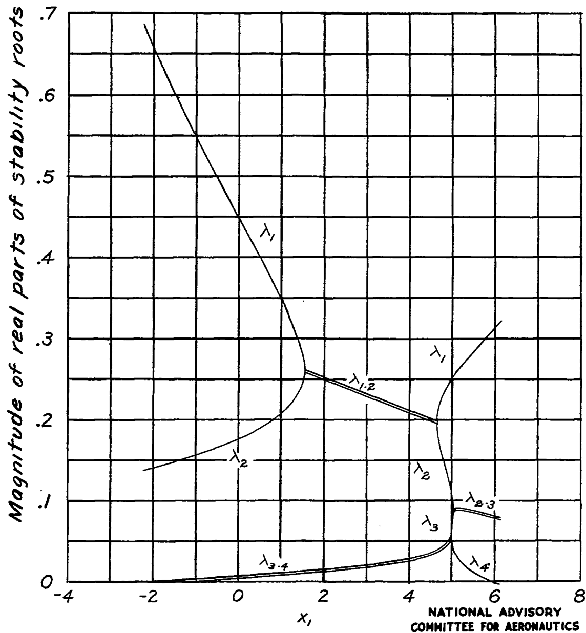
Figure 13.- Variation of real parts of stability roots with x_1 . \Gamma = 30^\circ ; S_2 = S_1 ; \epsilon = 0 ; l = 10.0 c_1 ; z_0 = 1.74 c_1 ; K_Y = 6.67 c_1 ; z_1 = 0 .
