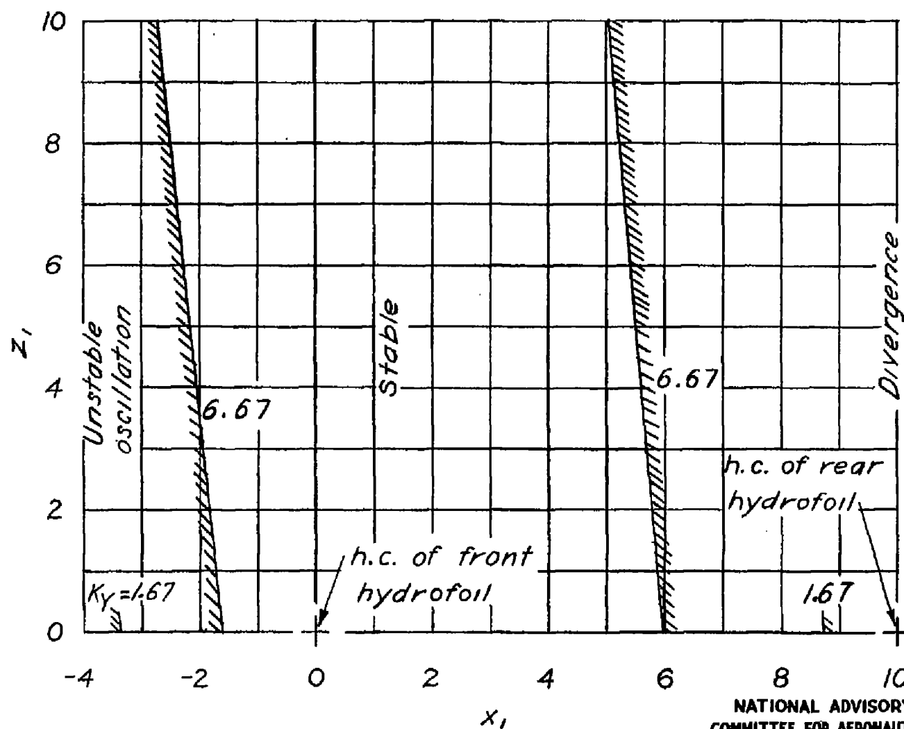
Figure 9.- Range of stable center-of-gravity location for two values of K_y . \Gamma = 30^\circ ; S_2 = S_1 ; \epsilon = 0 ; l = 10.0 c_1 ; z_0 = 1.74 c_1 .
