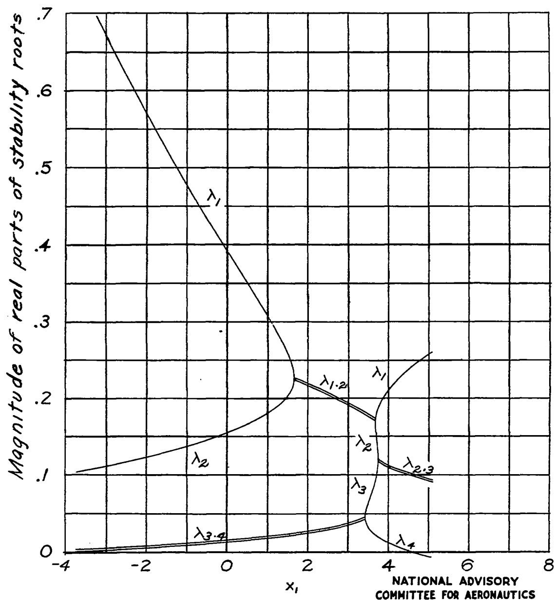
Figure 11.- Variation of real parts of stability roots with x_1 . \Gamma = 30^\circ ; S_2 = S_1 ; \epsilon = 2\alpha_c ; l = 10.0 c_1 ; z_0 = 1.74 c_1 ; K_Y = 6.67 c_1 ; z_1 = 5.00 c_1 .
