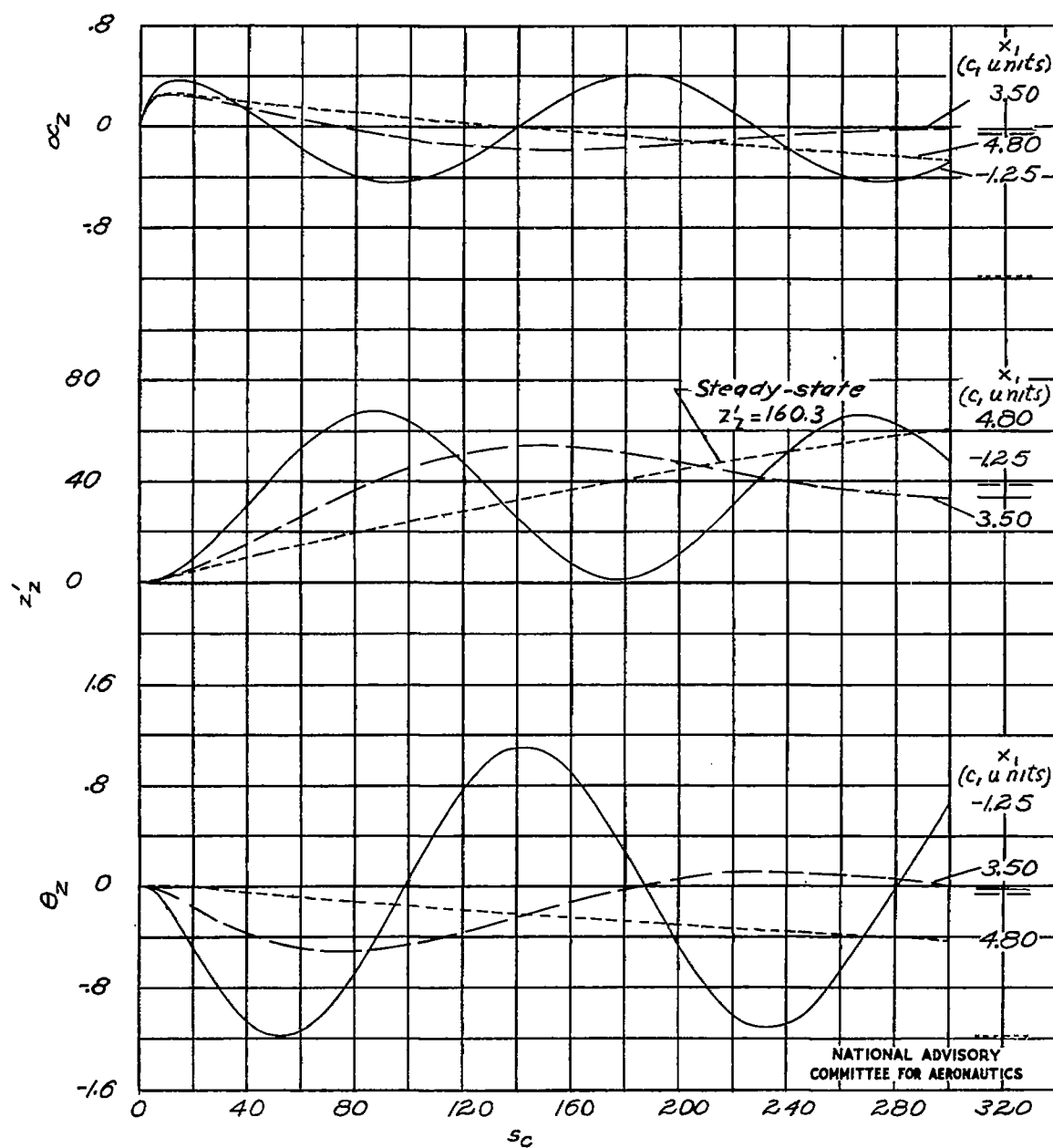
Figure 16.- Indicial responses for unit C_z disturbance. \Gamma=0^\circ ; S_2=S_1 ; e=0 ; l=10.0c_1 ; z_0=1.00c_1 ; K_Y=6.67c_1 ; z_1=5.00c_1 ; x_1 = -1.25c_1 , 3.50c_1 , or 4.80c_1 .
