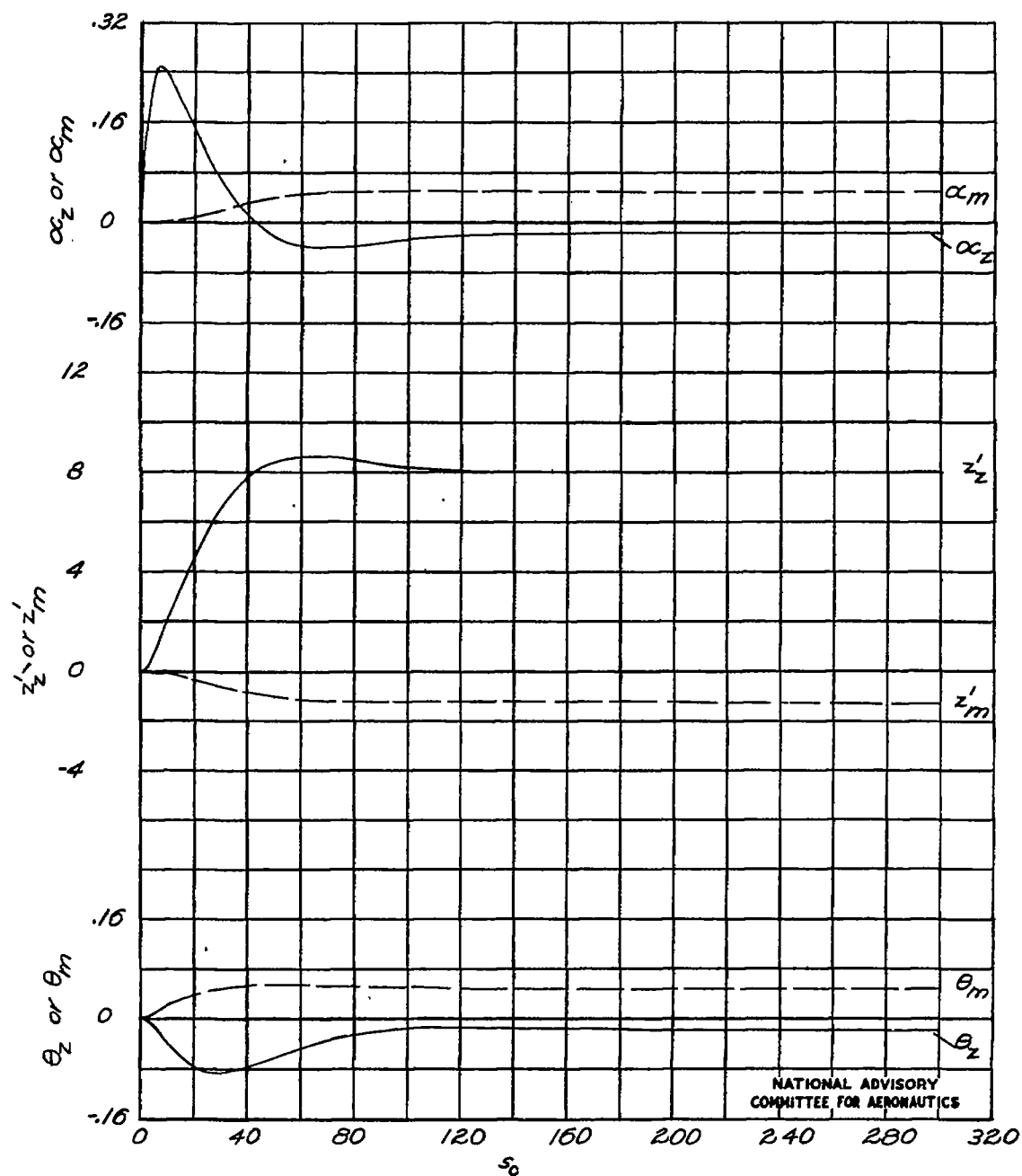
Figure 22.— Indicial responses for unit C_z and unit C_m disturbances. \Gamma = 30^\circ ; S_2 = S_1 ; \epsilon = 0 ; l = 20.0 c_1 ; z_0 = 1.74 c_1 ; K_Y = 0.67 c_1 ; z_1 = 5.00 c_1 ; x_1 = 7.00 c_1 .
