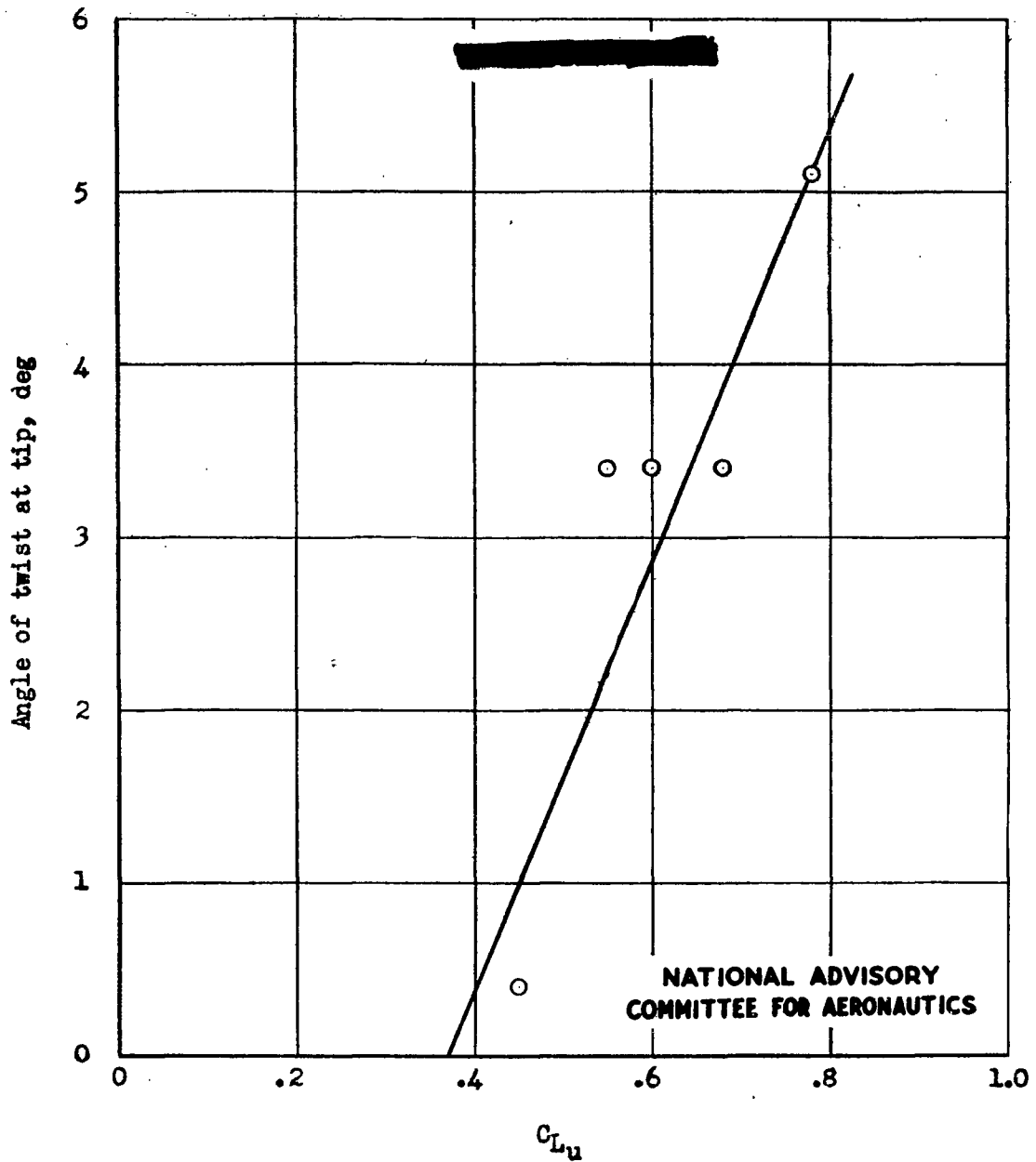
Figure 7.- Twist of propeller tip as function of C_{Lu} for propeller A. Tip speed constant at q/q_{cr} = 0.37 .
