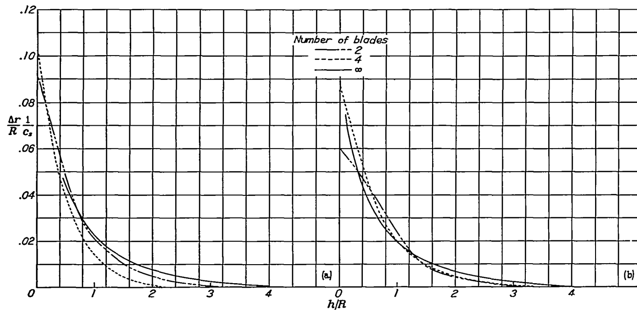
(a) \lambda = 1/4 .
