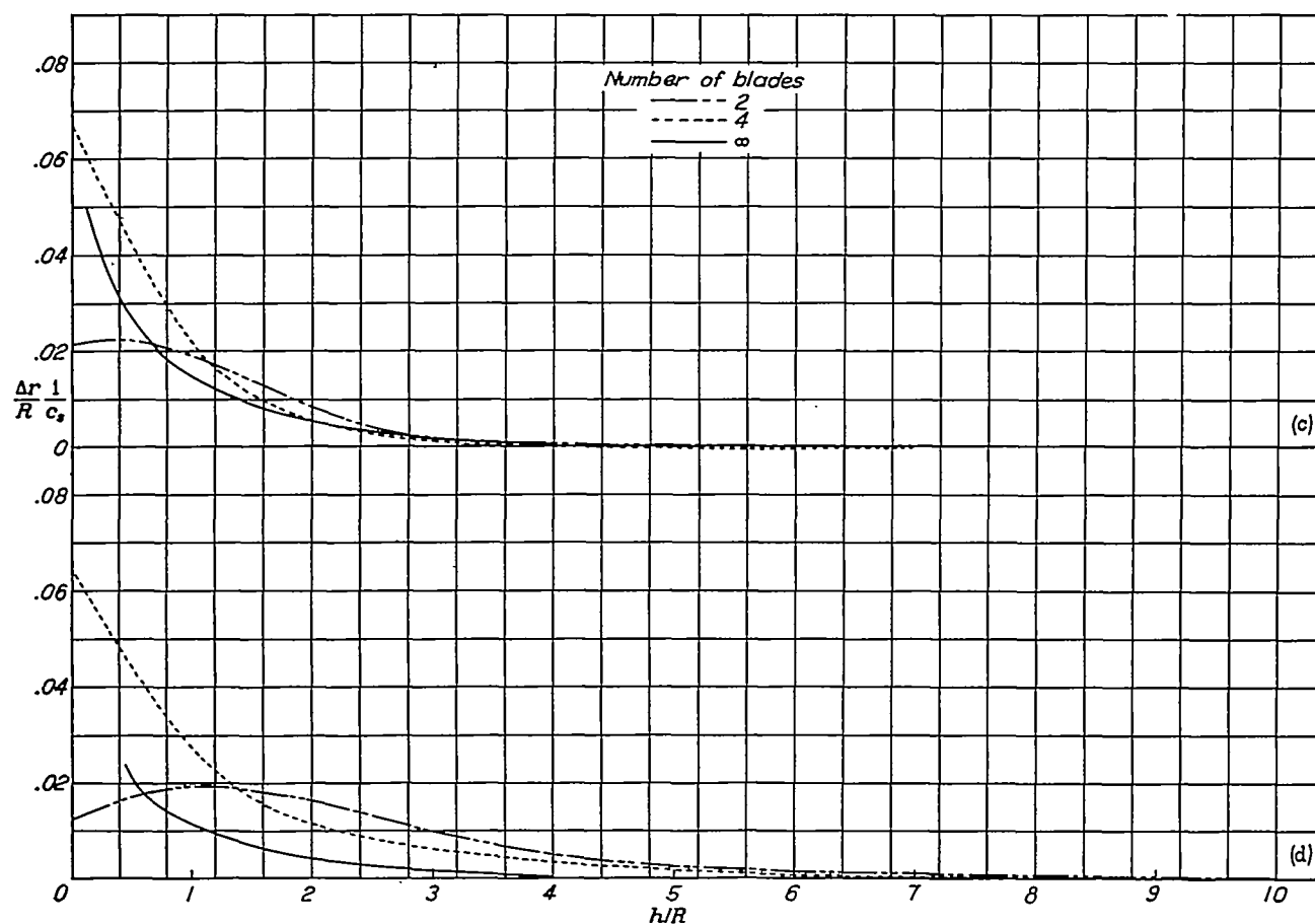
(c) \lambda = 1 .
