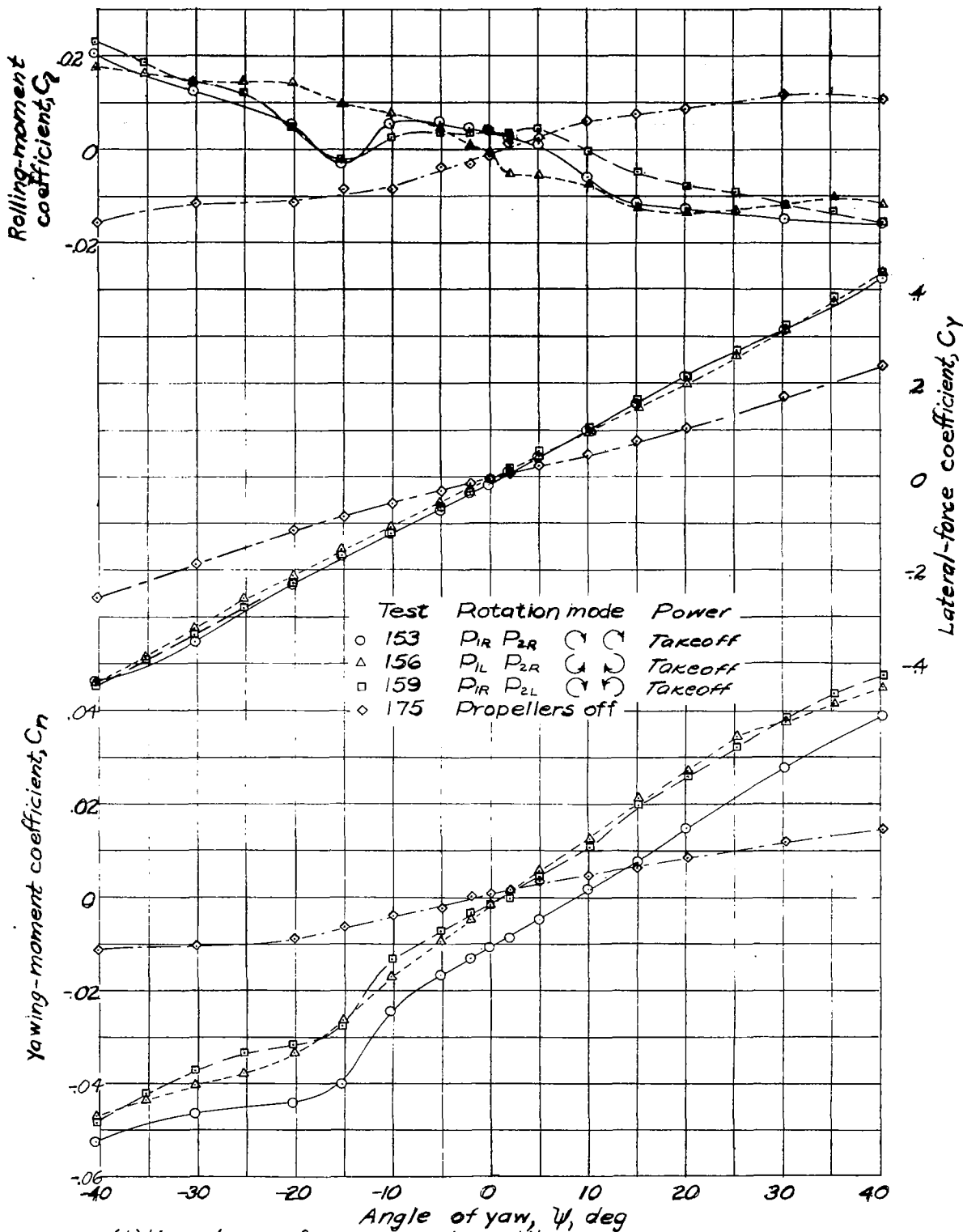
(b) Variation of C_n , C_2 , and C_y with \psi . Figure 12.- Concluded.
