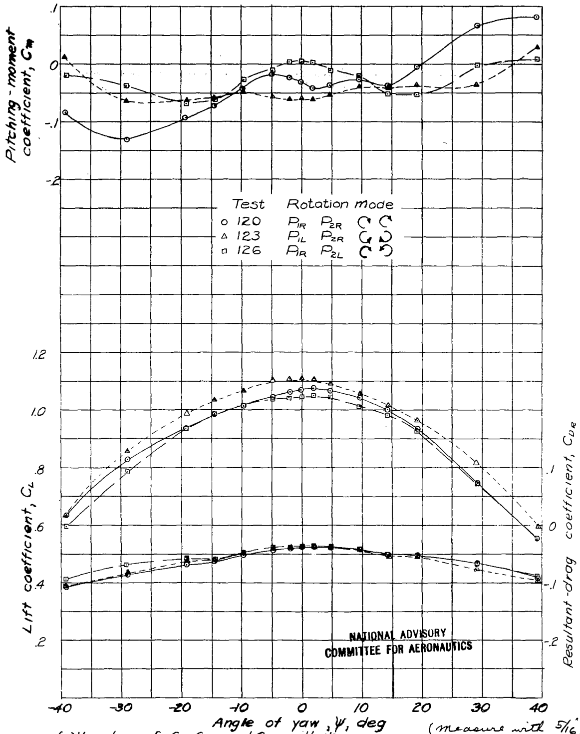
(a) Variation of C_L , C_m , and C_{DR} with \psi Figure 15.- Effect of propeller rotation on the aerodynamic characteristics in yaw of the 1/10-scale complete model of the North American XB-2B airplane. High-speed condition; landing gear up; cowl flaps closed; rated power; \alpha , 40.5^\circ ; \delta_a, \delta_f, \delta_r, \delta_e, 0^\circ ; q, 16.37 pounds per square foot.
