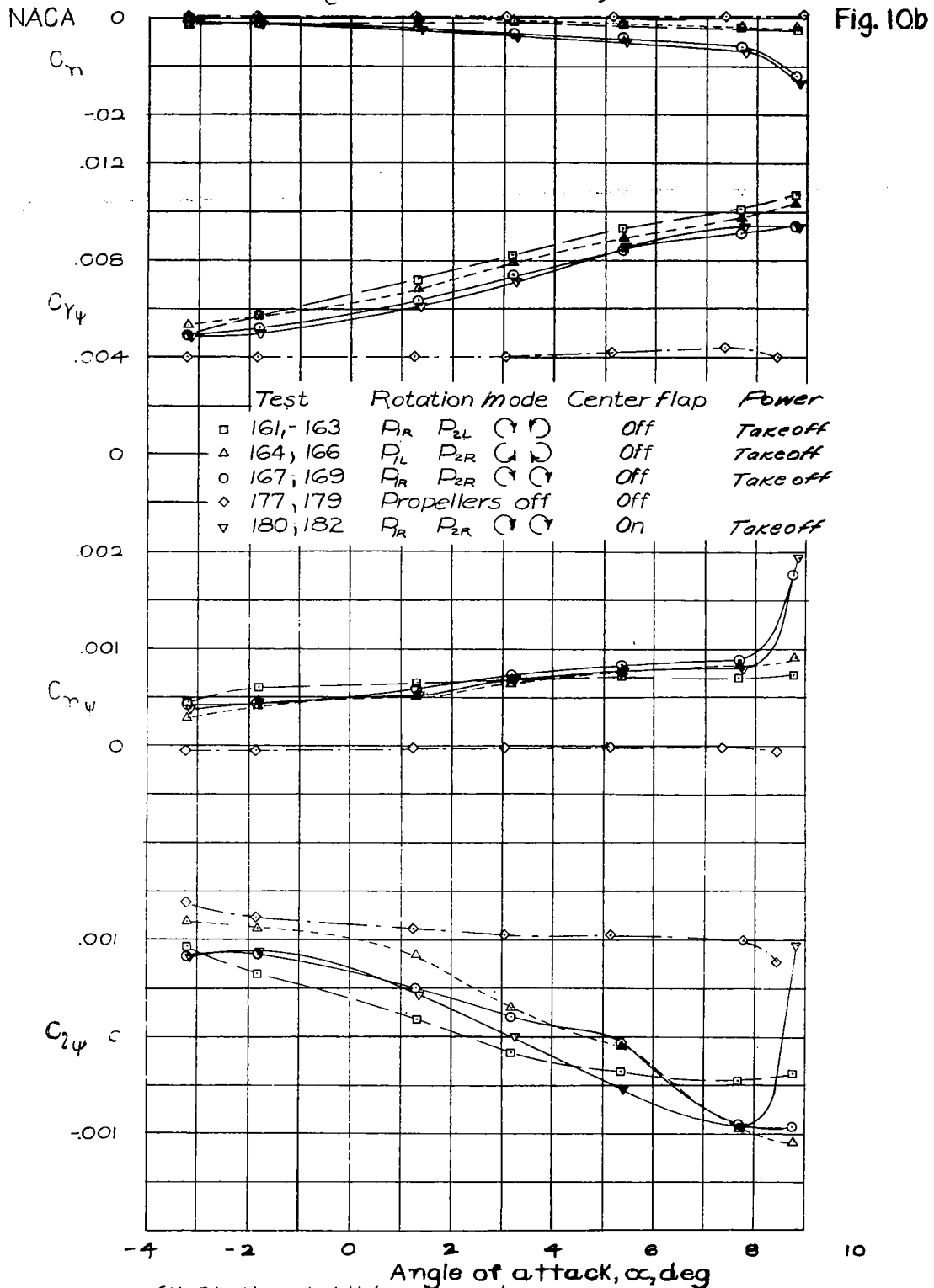
(b) Static-stability derivatives in yaw. Figure 10.- Concluded.
