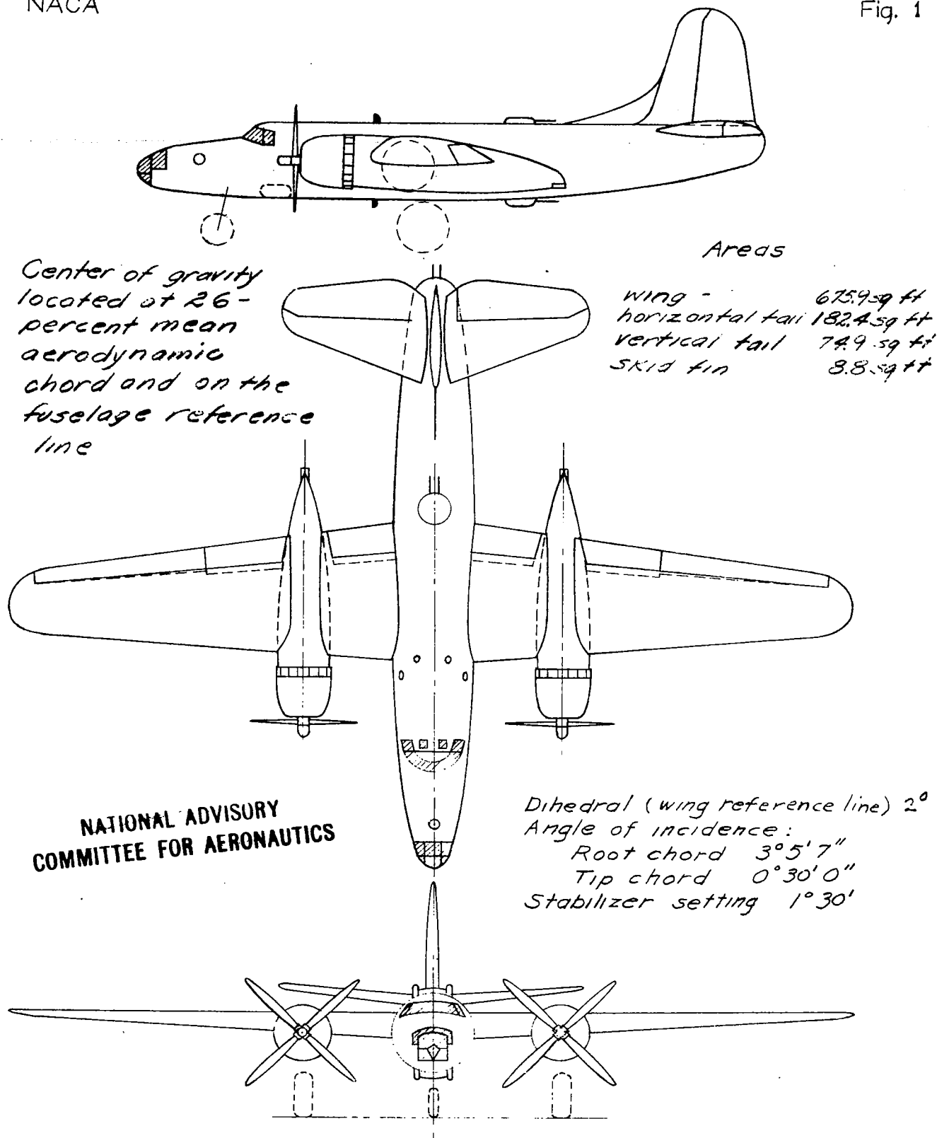
FIGURE 1. - Three-view drawing of the North American XB-28 airplane.
