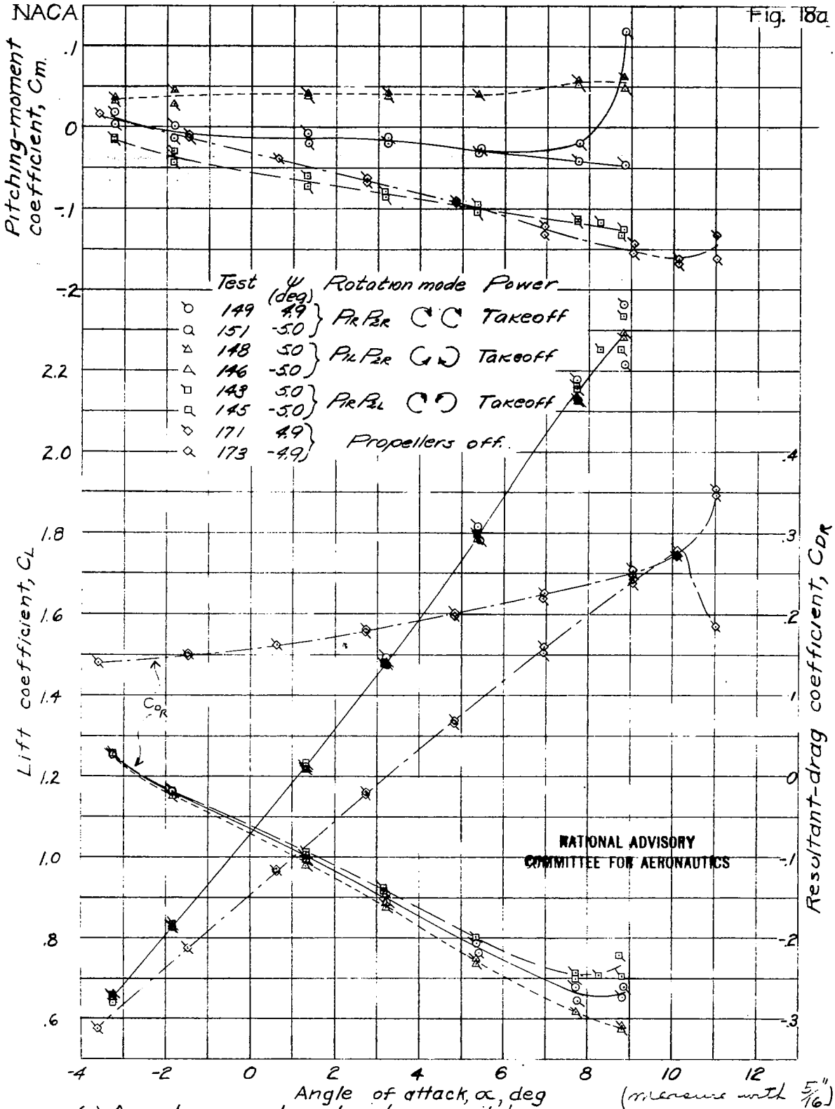
(a) Aerodynamic characteristics in pitch. Figure 18:- Effect of power and propeller rotation on the aerodynamic characteristics of the 1/10-scale complete model of the North American XB-28 airplane. Landing condition; landing gear down; cow/flaps closed; \beta, 27.1^\circ ; \delta_a, \delta_e, \delta_r, 0^\circ ; \delta_f, 45^\circ ; \delta_{f_2}, 40^\circ ; q, 4.09 pounds per square foot.
