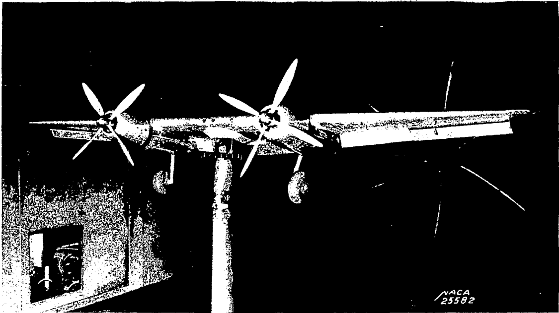
Figure 3a.- Three-quarter front view of the wing of the 1/10-scale model of the North American XB-28 airplane in the 7- by 10-foot wind tunnel. Wing with duplex flaps deflected (split flap over center section normally covered by fuselage), landing gear extended, and propellers on.
