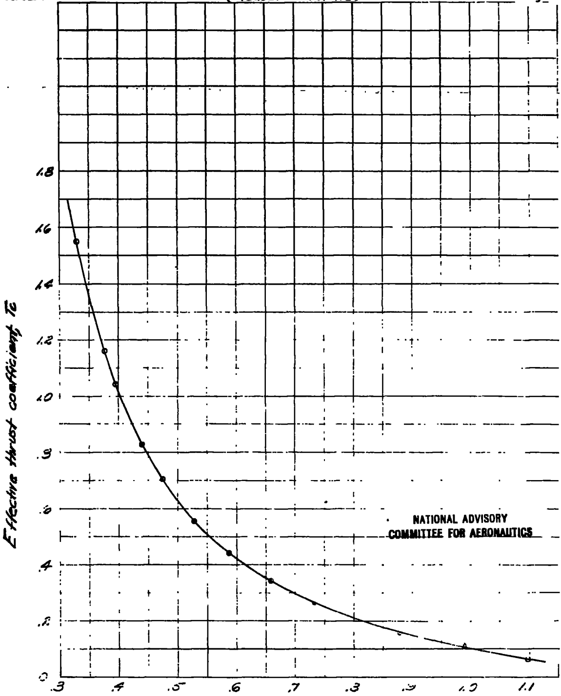
Advance-diameter ratio, V/nd (a) \beta, 27.1^\circ ; propeller rotation mode P_{12} P_{12} ; \alpha_w, 0.6^\circ ; \delta_6, \delta_7, \delta_8, \delta_9, 0^\circ ; tunnel velocity, 61.0 feet per second. Test 170. Figure 5.- Effective-thrust-coefficient calibration of propellers of \frac{1}{10} -scale model of North American XB-28 airplane.
