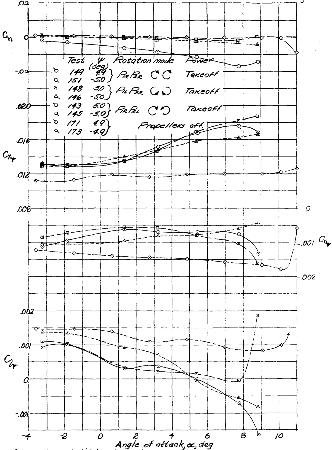
(b) Static-stability derivatives in yaw. Figure 18.- Concluded.
