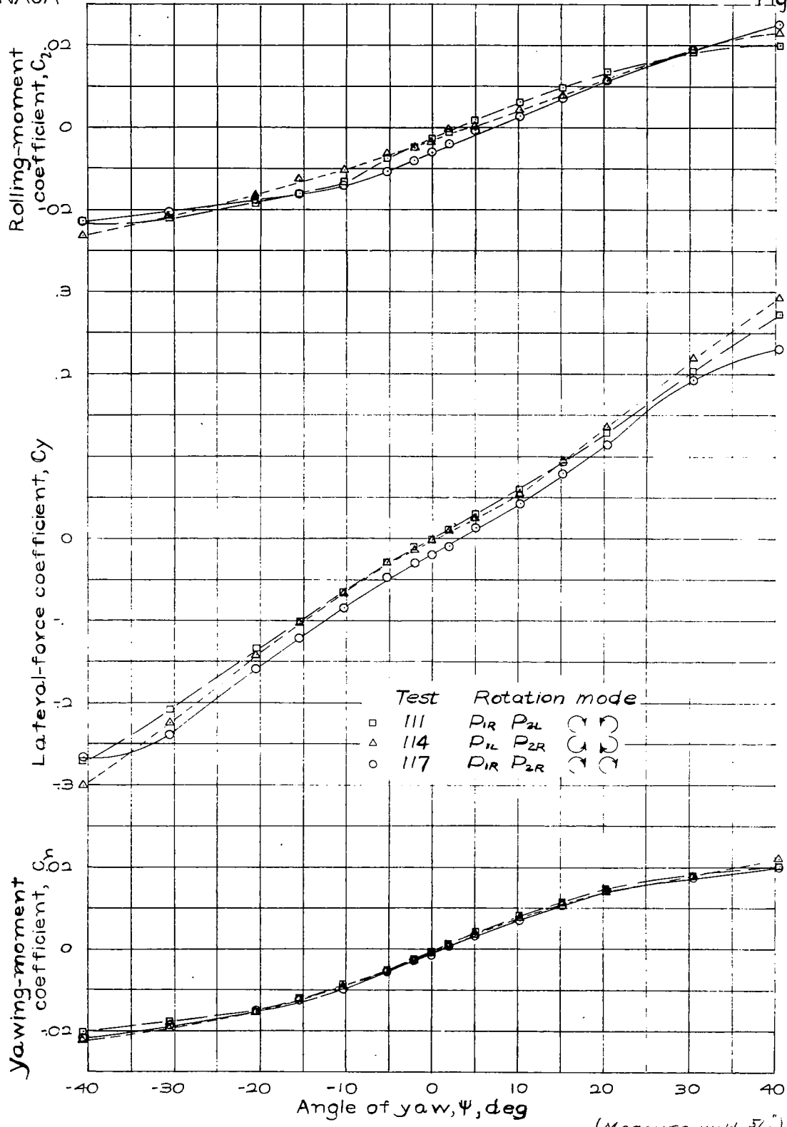
(b) Variation of C_n , C_l , and C_y with \psi . Figure 11.- Concluded.
