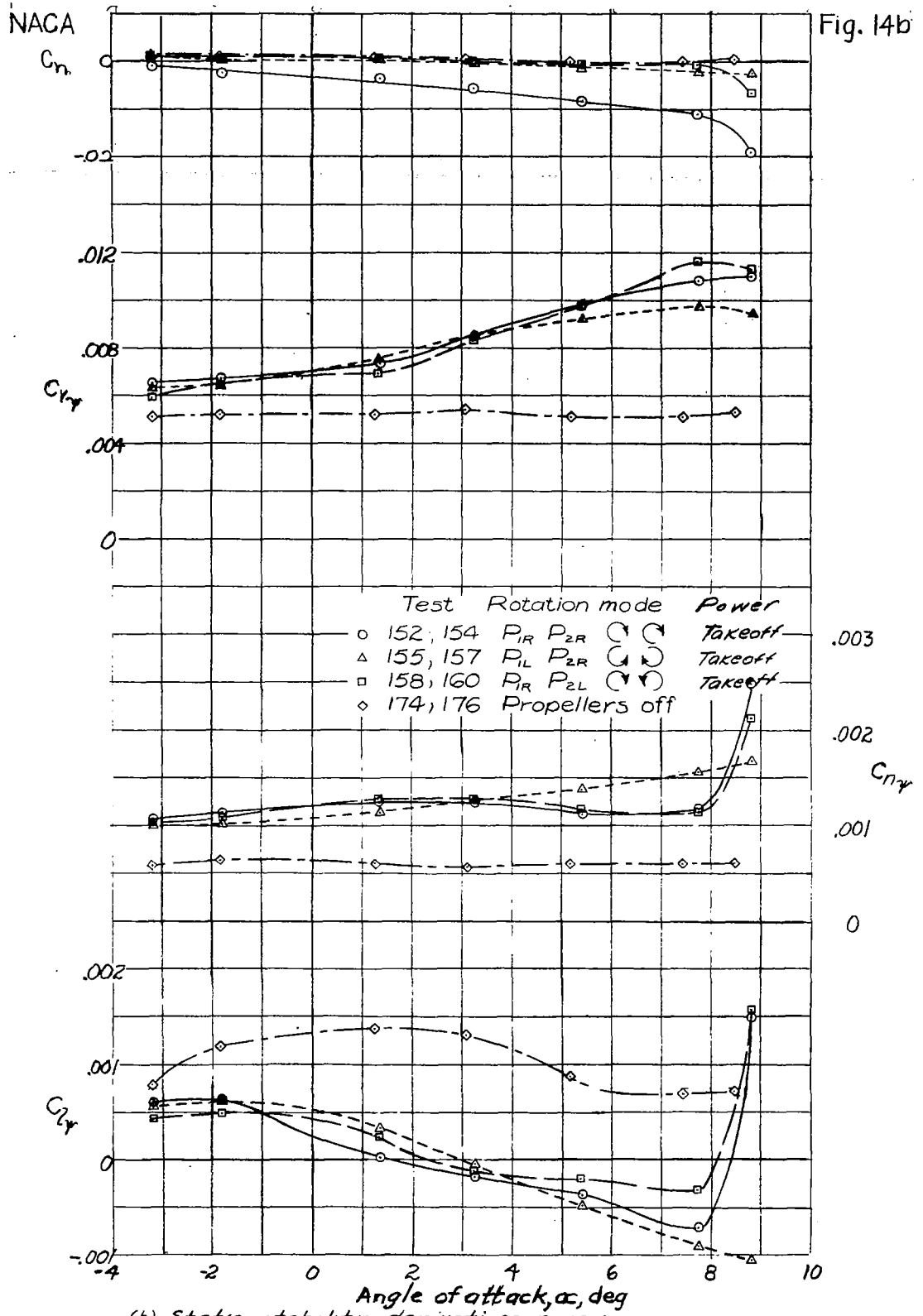
(b) Static-stability derivatives in yaw. Figure 14. - Concluded.
