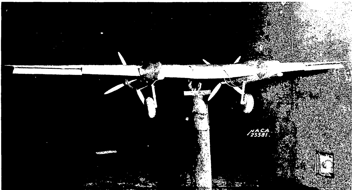
Figure 3b.- Three-quarter rear view of the wing of the 1/10-scale model of the North American XB-28 airplane in the 7- by 10-foot wind tunnel. Wing with duplex flaps extended (split flap over center section normally covered by fuselage), landing gear extended, and propellers on.
