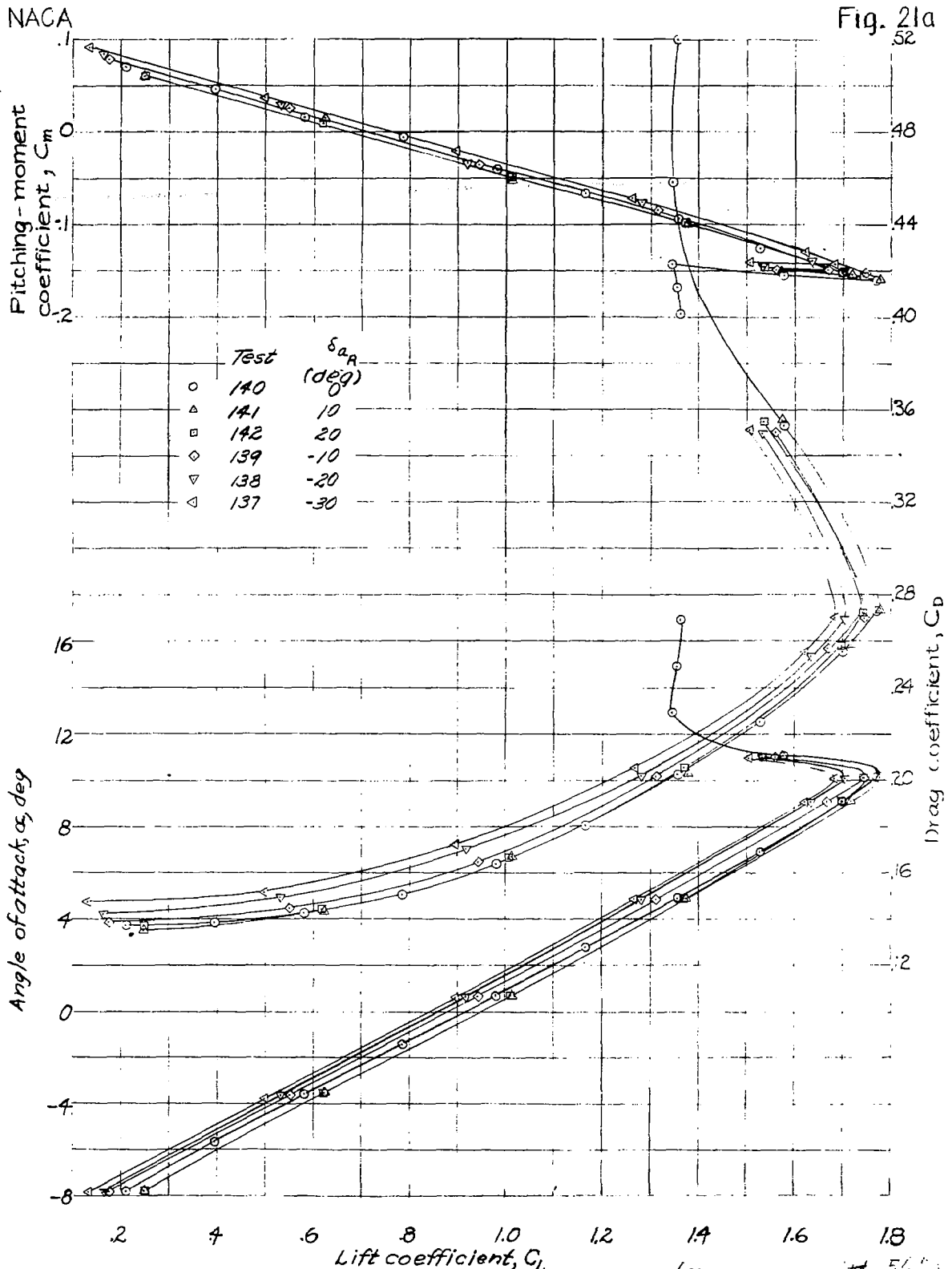
(a) Variation of \alpha , C_m and C_D with C_L . (m. curve with 5/16 ) FIGURE 21. - Effect of right aileron deflection on the power-off aerodynamic characteristics in pitch of the 1/10-scale model of the North American XB-2B airplane. Landing condition; landing gear down; \delta_e, \delta_r, 0^\circ ; \delta_f, 45^\circ ; \delta_{f_2}, 40^\circ ; q, 4.09 pounds per square foot.
