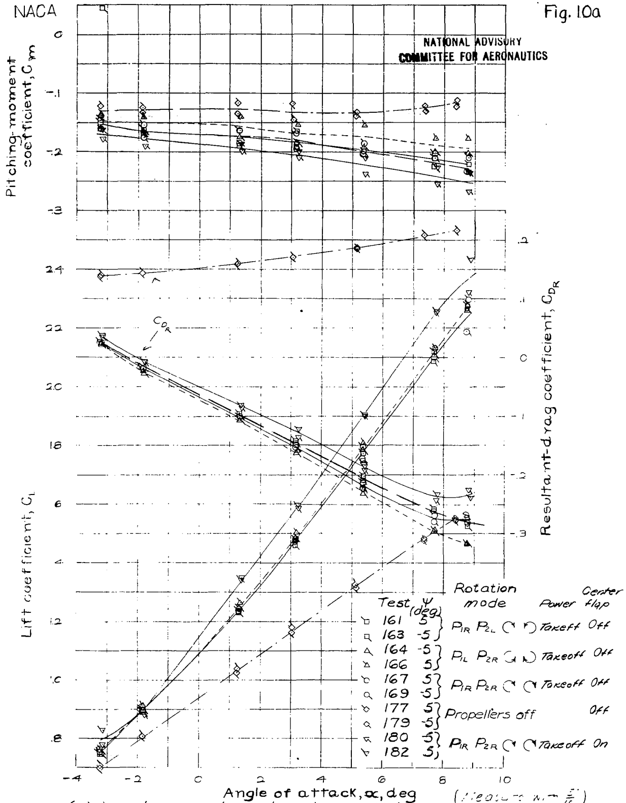
(a) Aerodynamic characteristics in pitch. (Measurements with \frac{c}{l} ) Figure 10.- Effect of propeller rotation, power, and center-section flap on the aerodynamic characteristics of the wing of the 1/10-scale model of the North American XB-28 airplane. Landing condition; landing gear down; cowl flap closed; \beta, 27.1^\circ ; \delta_{f1}, 45^\circ ; \delta_{f2}, 40^\circ ; q, 4.09 pounds per square foot.
