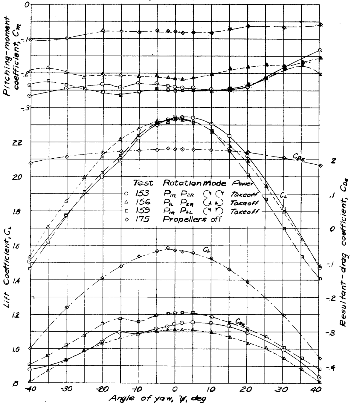
(a) Variation of C_L, C_m , and C_{DR} with \gamma . Figure 12.- Effect of power and propeller rotation on the aerodynamic characteristics in yaw of wing plus fuselage of the \frac{1}{10} -scale model of the North American XB-2B airplane. Landing condition; landing gear down; cowl flaps closed; \beta, 27.1^\circ ; \delta_1, 0^\circ ; \delta_{F1}, 45^\circ ; \delta_{F2}, 40^\circ ; q, 40.9 pounds per square foot.
