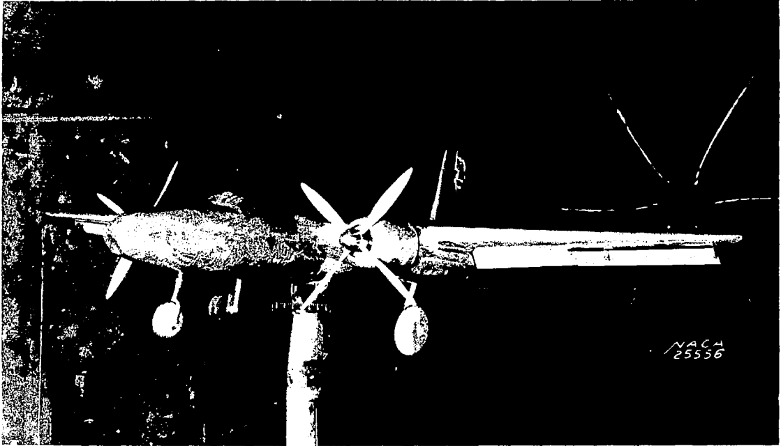
Figure 2a.- Three-quarter front view of the 1/10-scale model of the North American XB-28 airplane.
