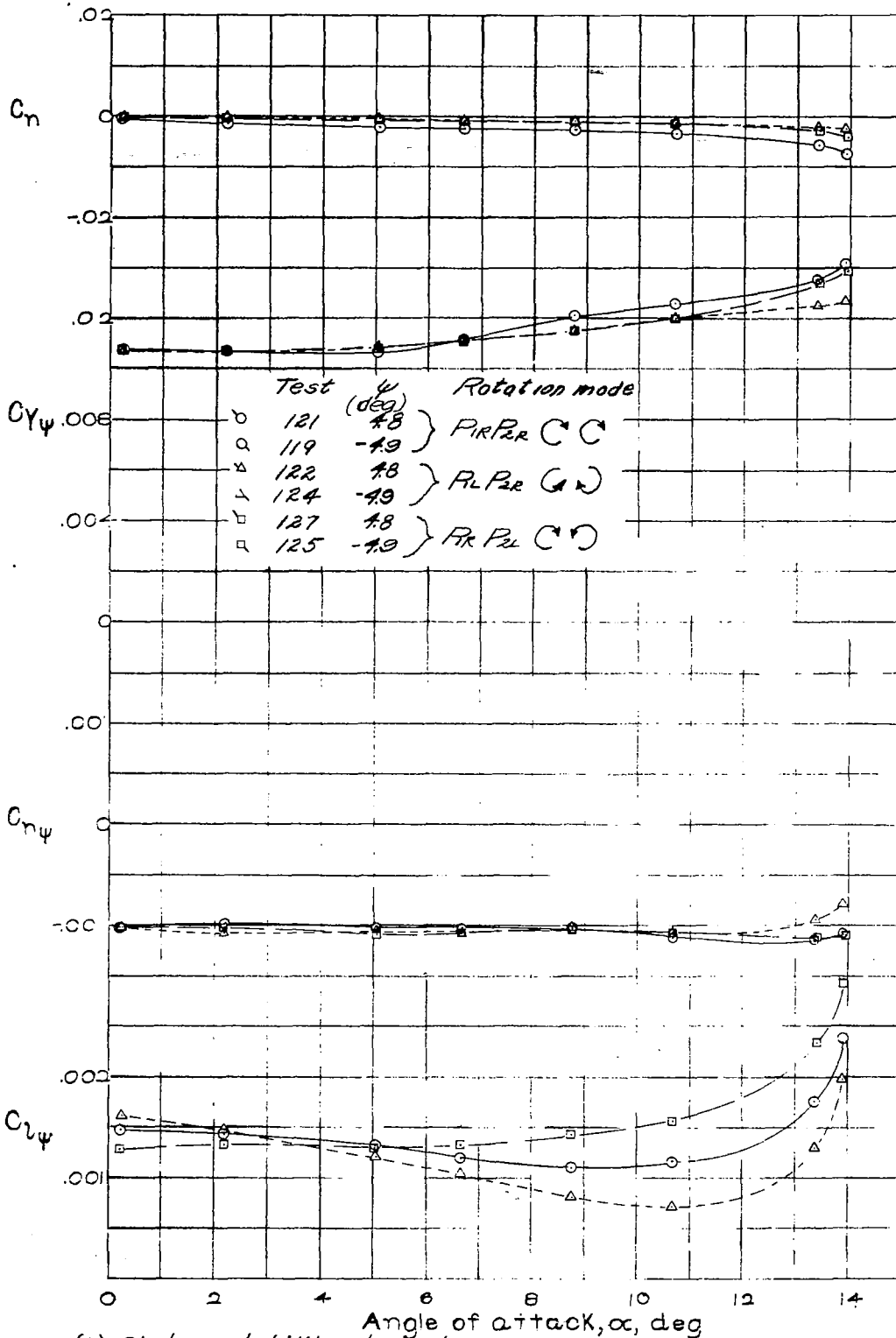
(b) Static-stability derivatives in yaw. Figure 17: Concluded.
