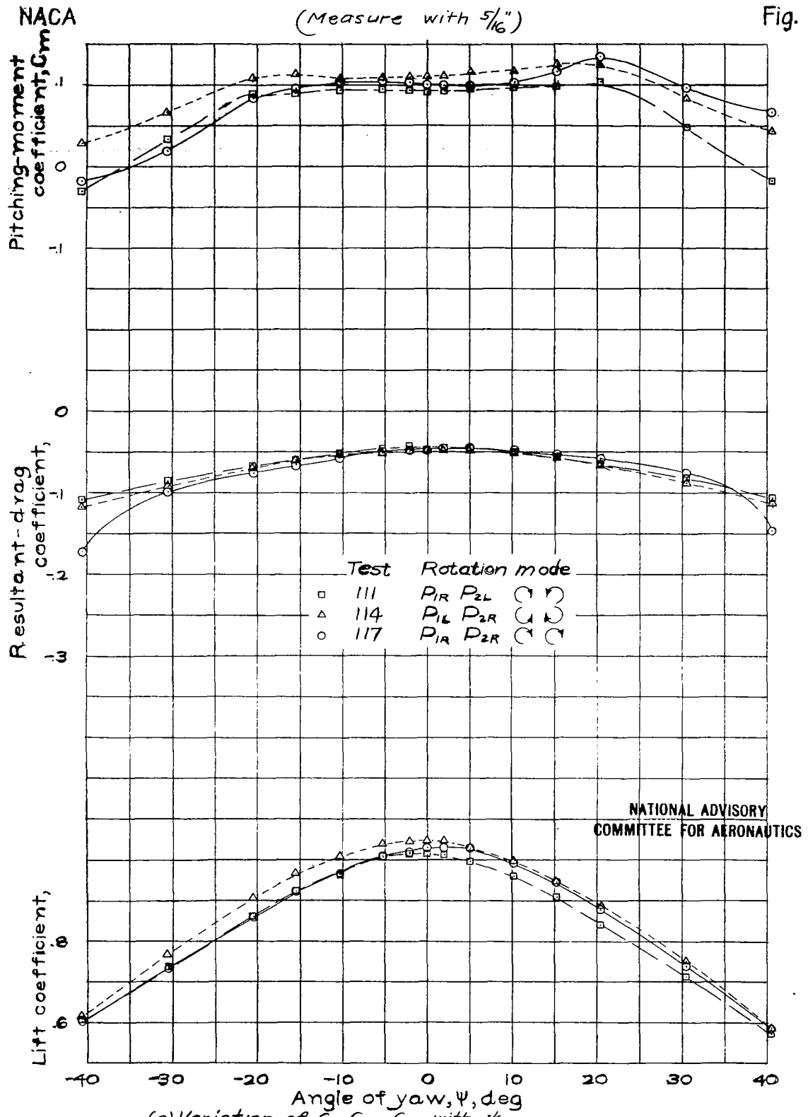
Figure 11.- Effect of propeller rotation on the aerodynamic characteristics in yaw of the wing plus fuselage of the 1/10-scale model of the North American XB-2B airplane. High-speed condition; landing gear up; cowl flaps closed; rated power; \beta, 40.5^\circ ; \delta_a, \delta_f, 0^\circ ; q, 76.37 pounds per square foot.
