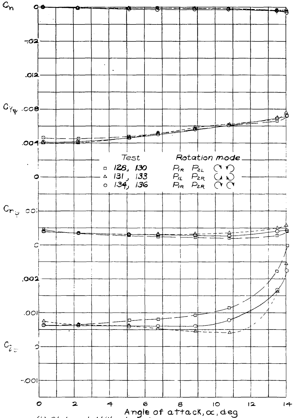
(b) Static-stability derivatives in yaw.
