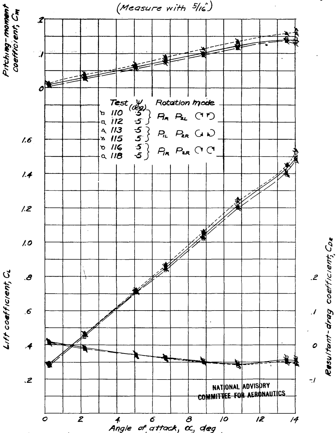
(a) Aerodynamic characteristics in pitch.
