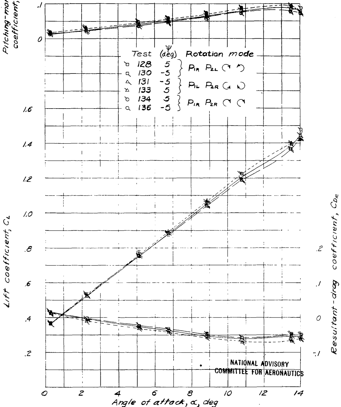
(a) Aerodynamic characteristics in pitch.
