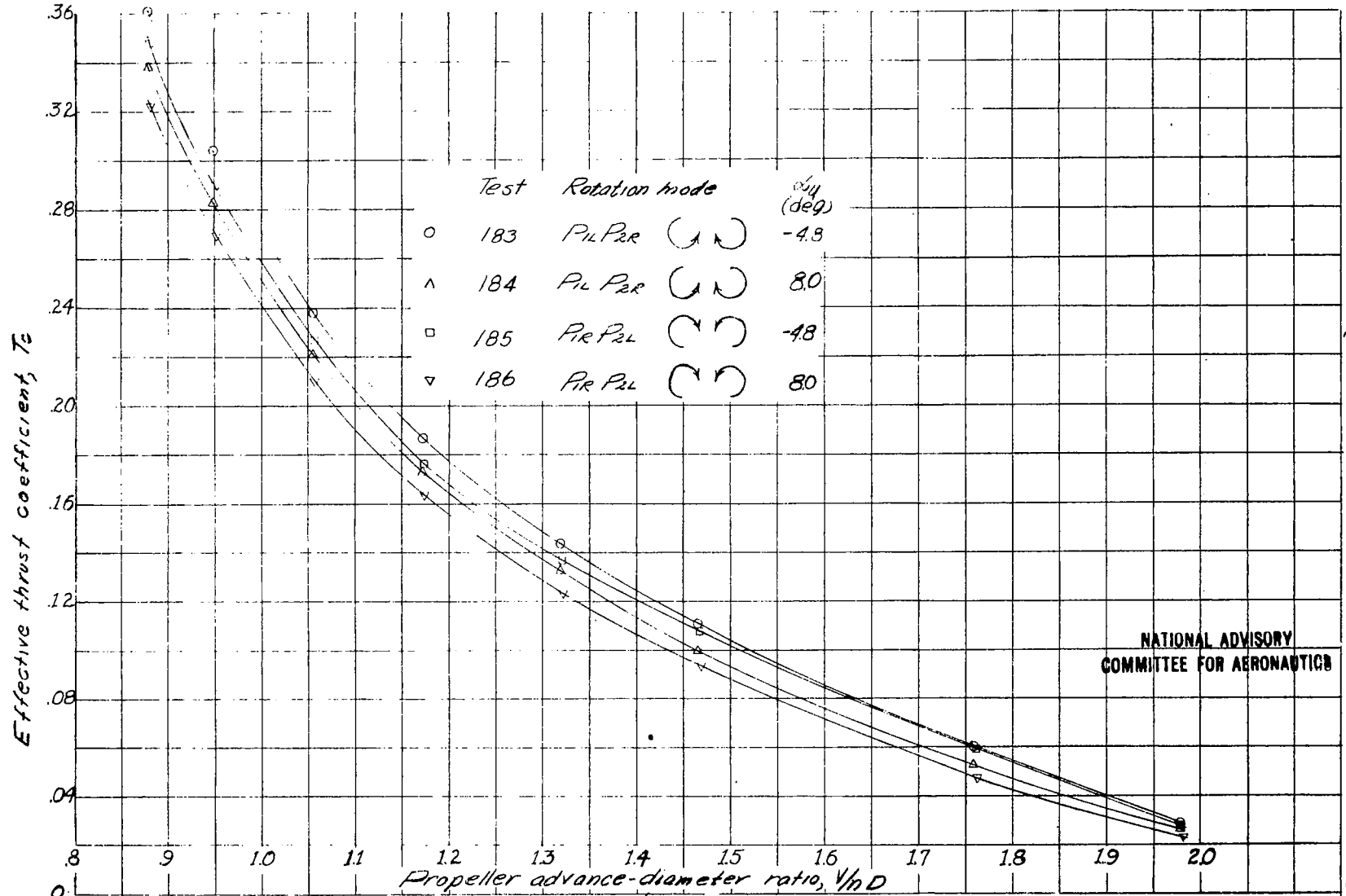
Figure 19—Effective thrust coefficient as a function of V/nD for the 1/10-scale model wing of the North American XB 2B airplane. High-speed condition; landing gear up; \beta, 9.05^\circ ; \delta_1, 0^\circ ; q, 16.37 pounds per square foot.
