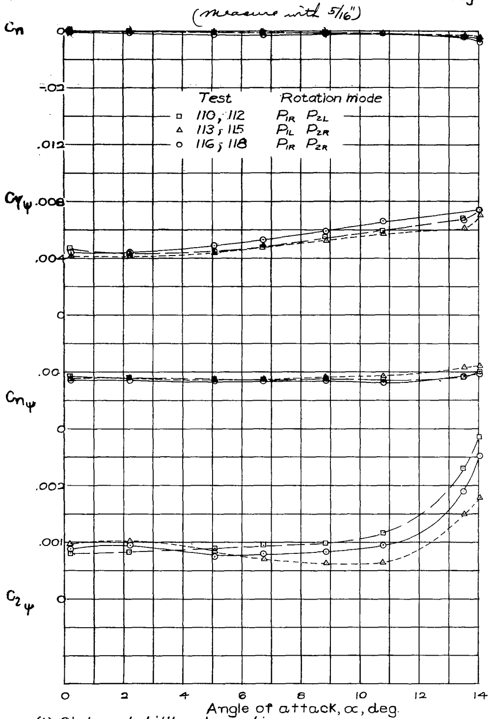
(b) Static-stability derivatives in yaw. Figure 13.-Concluded.
