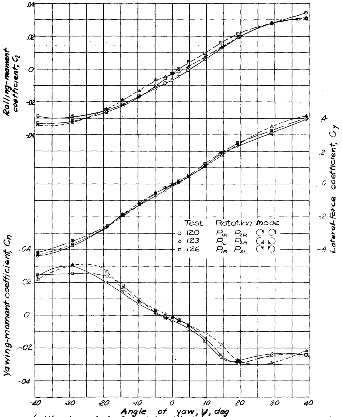
(b) Variation of C_n , C_r , and C_y with \psi . Figure 15.-Concluded.
