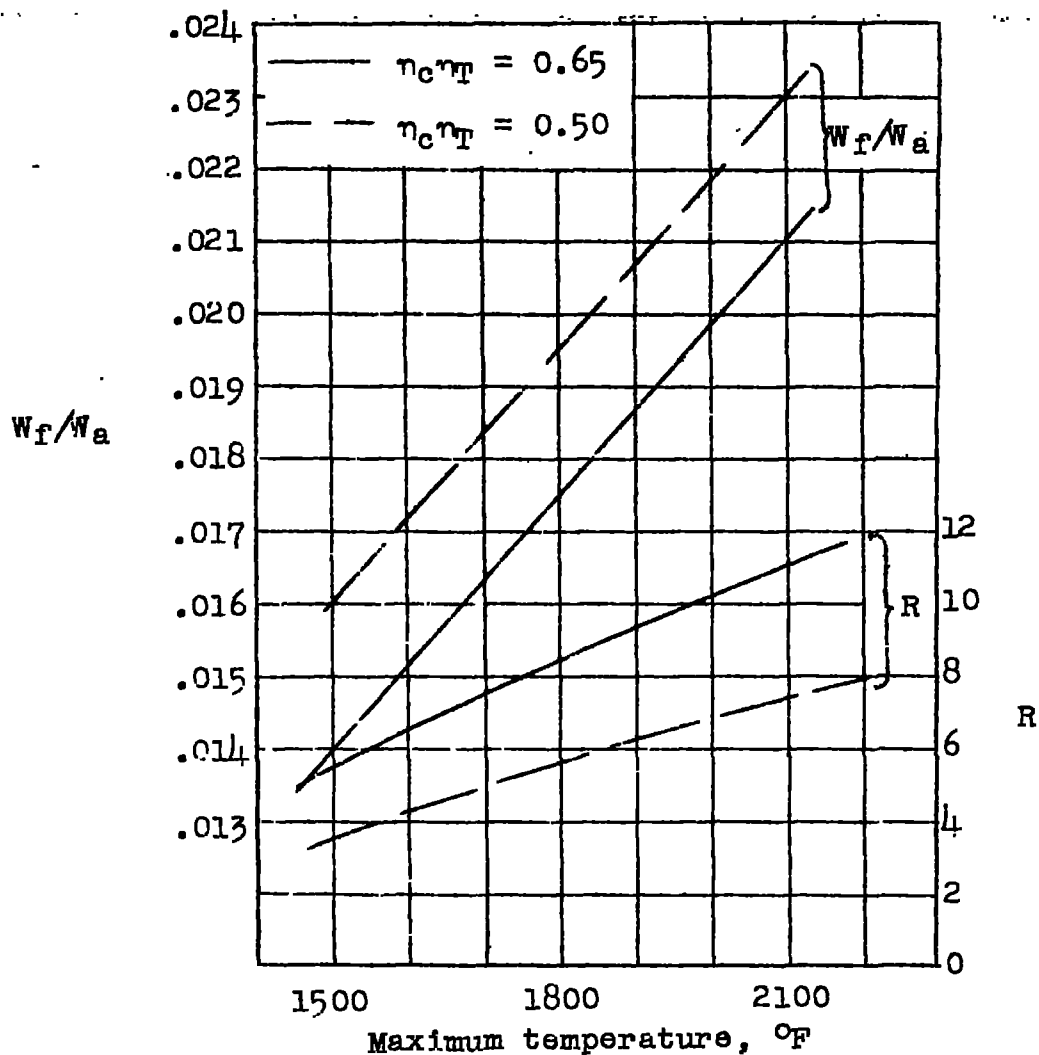
Figure 10.- Effect of engine temperature on fuel-air ratio and compression ratio. Maximum-power condition.
