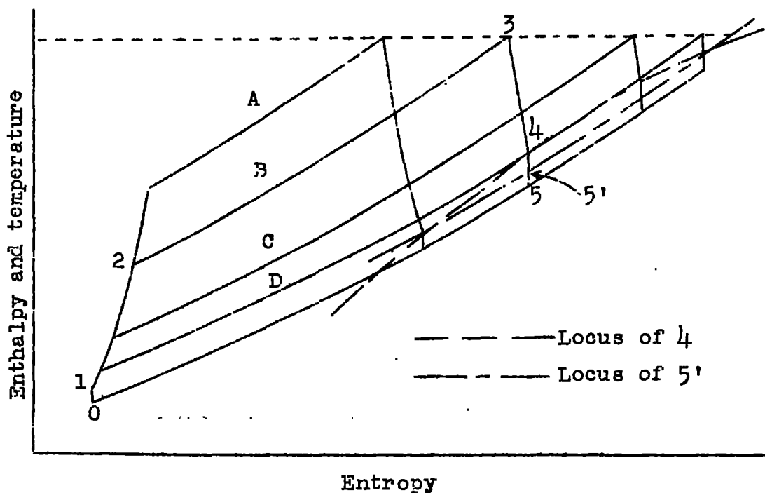
Figure 3.- Jet-engine cycles.
