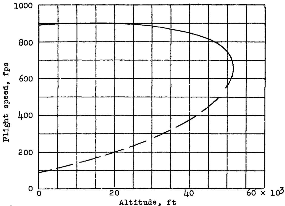
Figure 19.- Effect of altitude on level-flight speed of jet-propelled airplane. t_{\max} = 1500^{\circ} \text{ F} ; \eta_c = \eta_T = 85 percent; W = 5400 pounds; S = 108 square feet.
