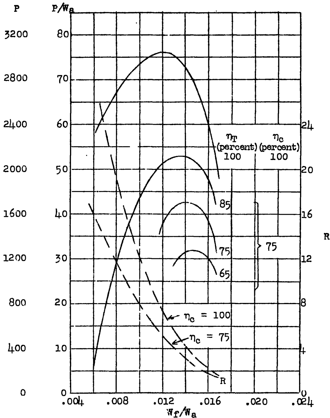
Figure 5.- Effect of fuel-air ratio on thrust power and pressure ratio. At sea level; V_o = 800 feet per second; t_{max} = 1500^\circ F.
