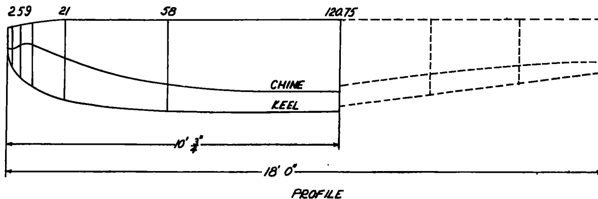
FIGURE 1.-LANGLEY IMPACT BASIN FLOAT MODEL M-1. OFFSETS GIVEN IN TABLE I.
