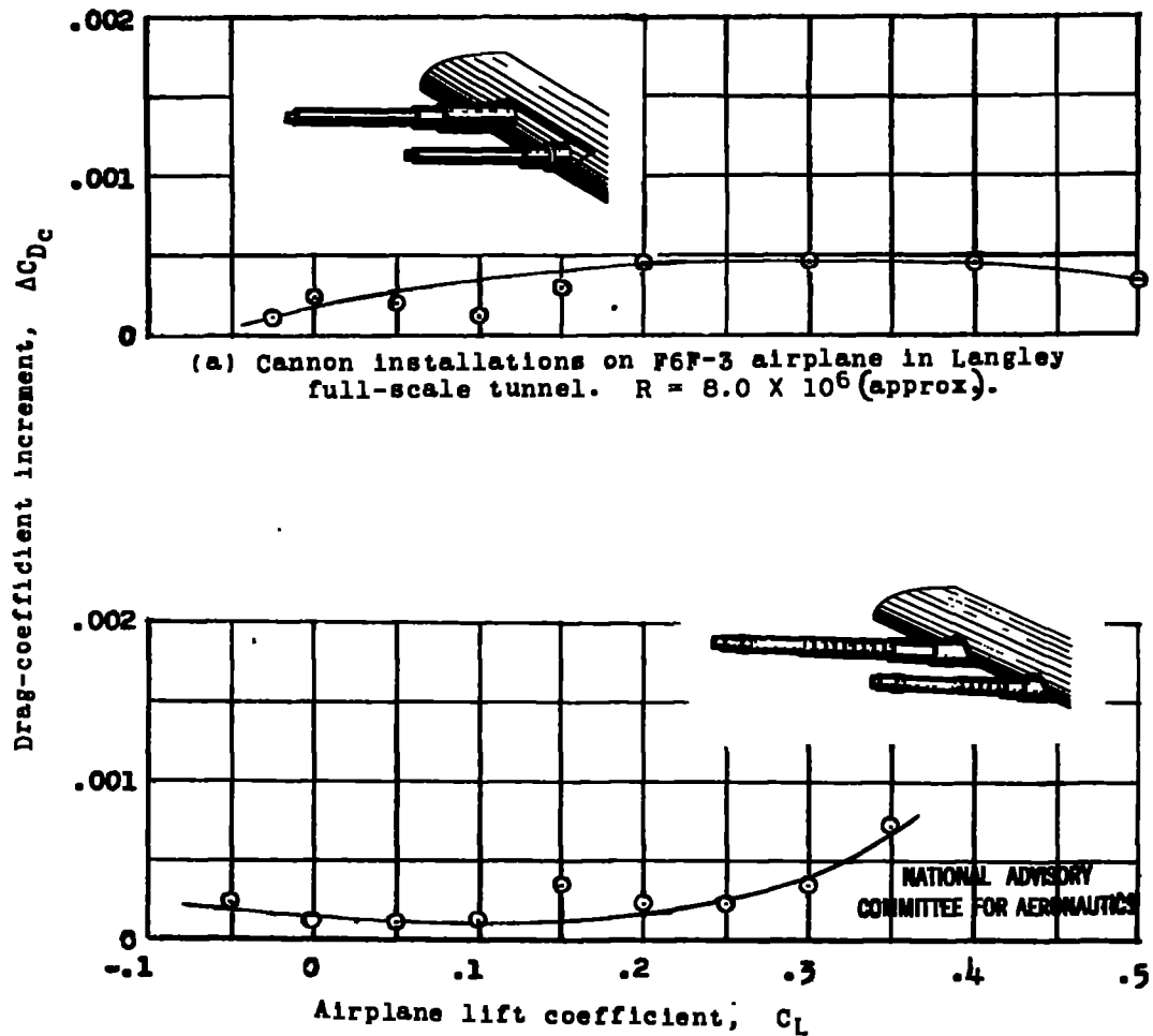
(b) Cannon on F4U-1 airplane in Langley full-scale tunnel. R = 7.6 \times 10^6 .
