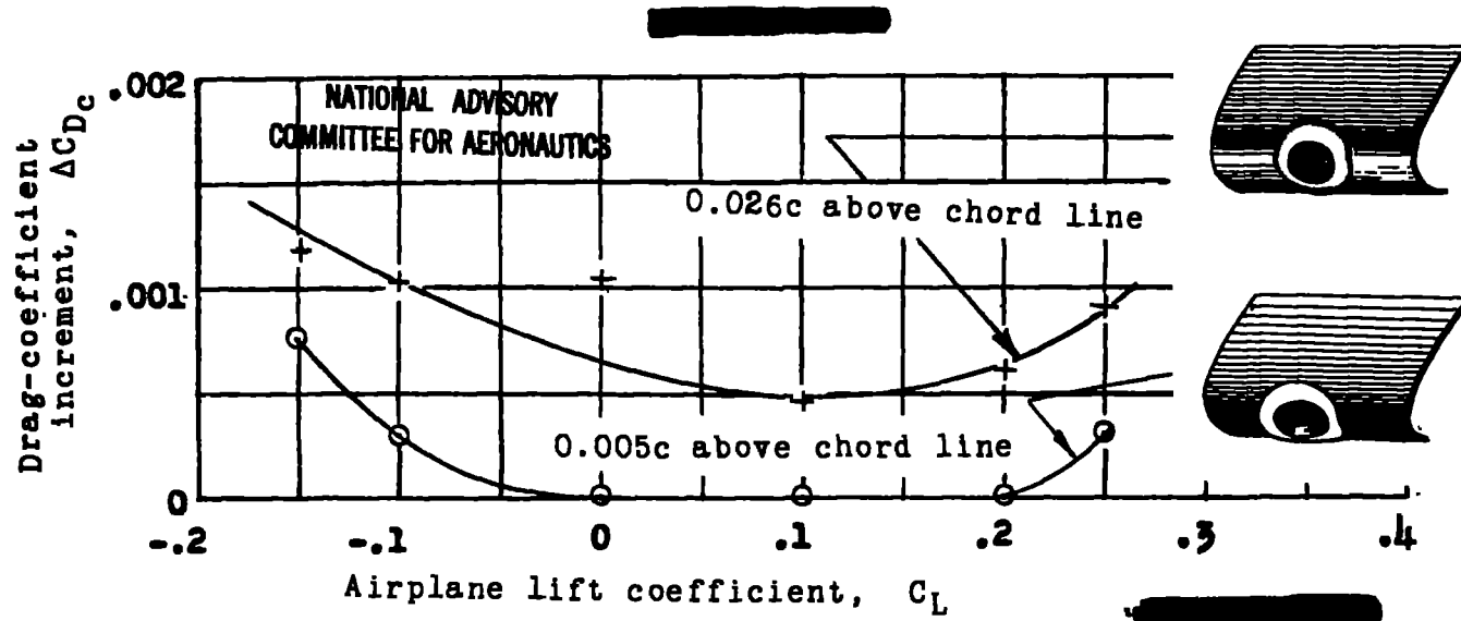
Figure 11.- Drag increments of gun ports on wing of XF2A-2 airplane in Langley full-scale tunnel. R = 5.5 \times 10^6 .
