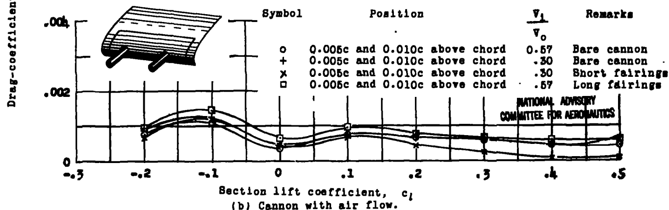
Figure 38.- Several cannon installations on model of wing of XA-41 airplane in Ames 7- by 10-foot tunnel. R = 6.35 \times 10^6 . Holes around cannon have 0.032c and 0.034c diameters.
