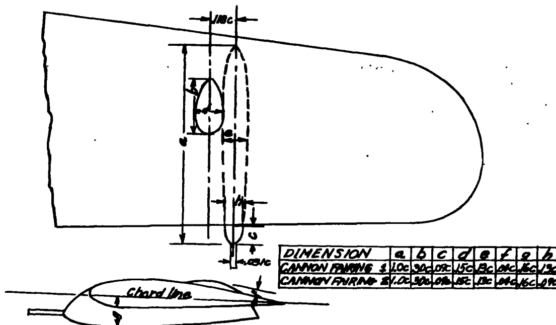
(a) Underslung cannon installation.
