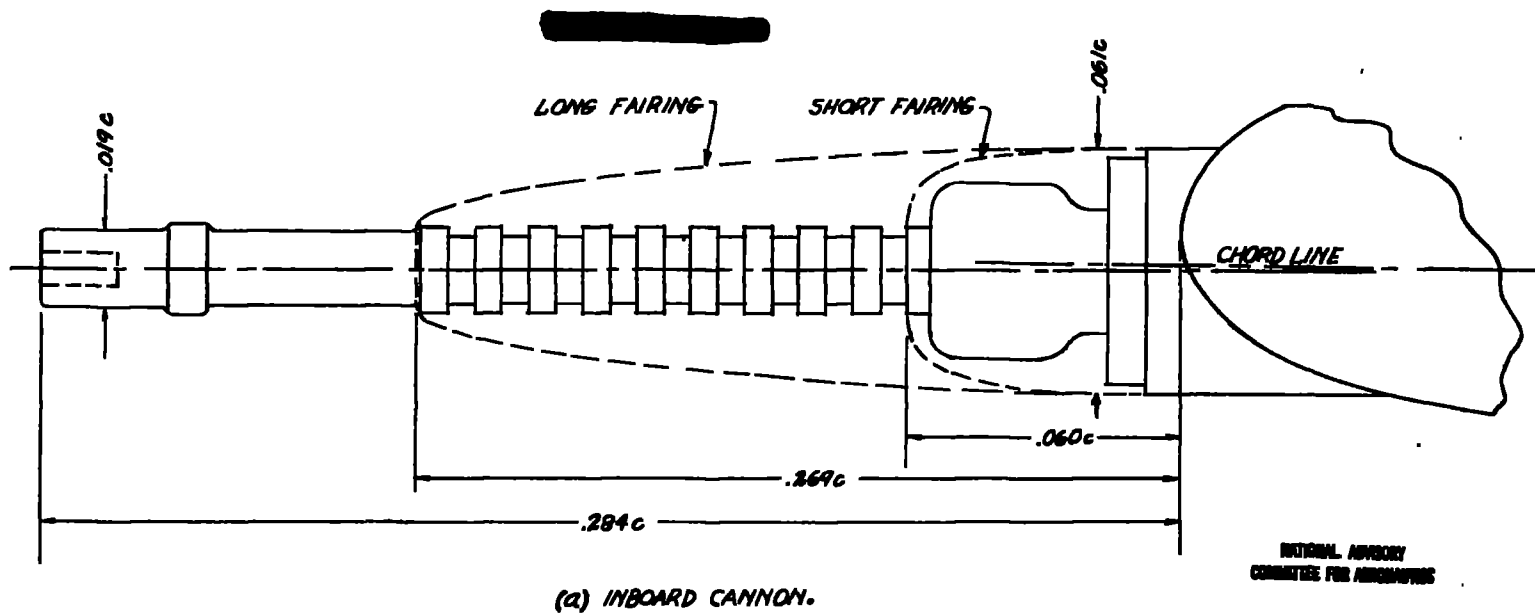
Figure 35.- Cannon installations on model of XP4U-1 airplanes.
