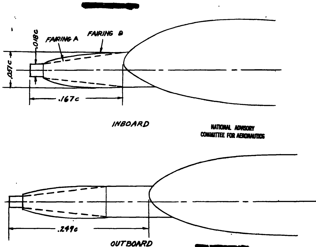
Figure 33.- Cannon installations on XF14C-2 airplanes.
