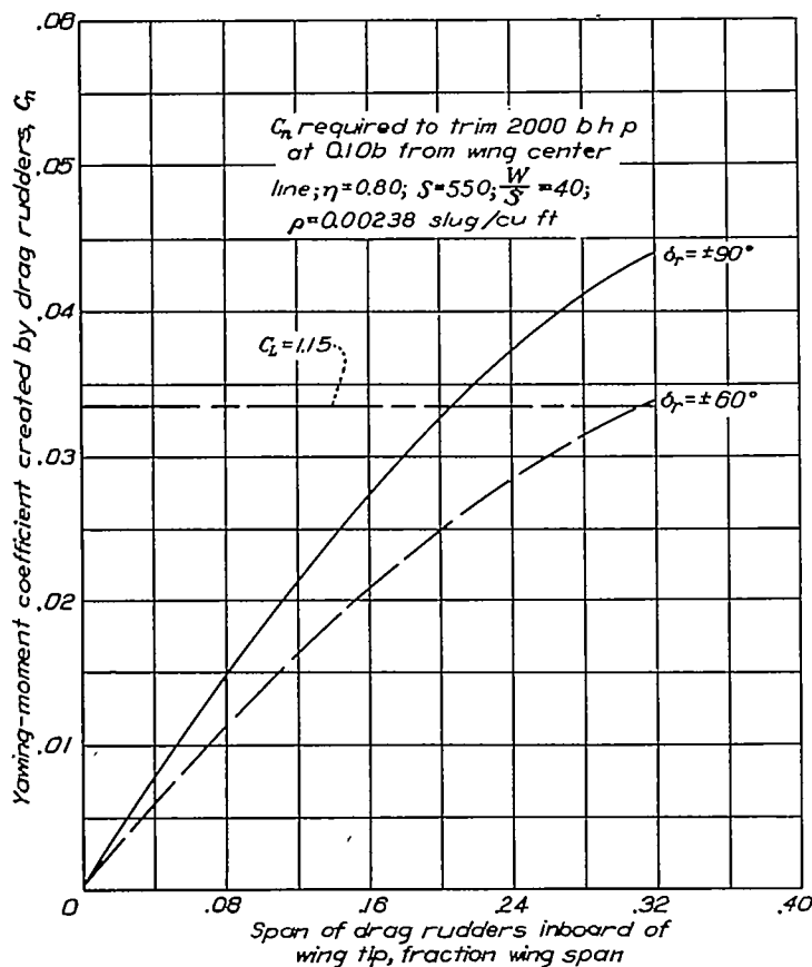
FIGURE 18.—Yawing moments created by double split perforated drag rudders mounted at wing tips. C_f=0.20 ; \eta , propulsive efficiency; \frac{W}{S} , wing loading, pounds per square foot.
