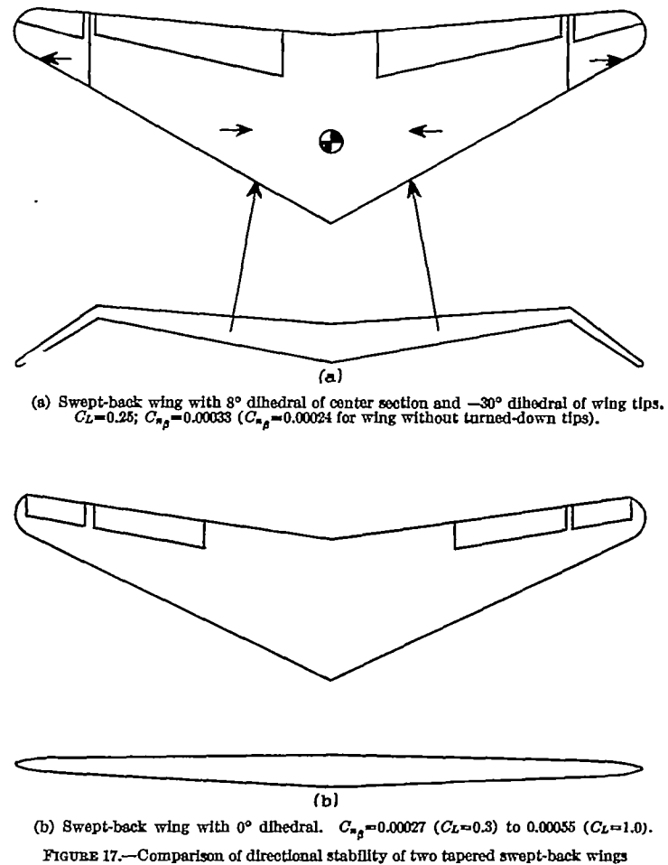
FIGURE 17.—Comparison of directional stability of two tapered swept-back wings
