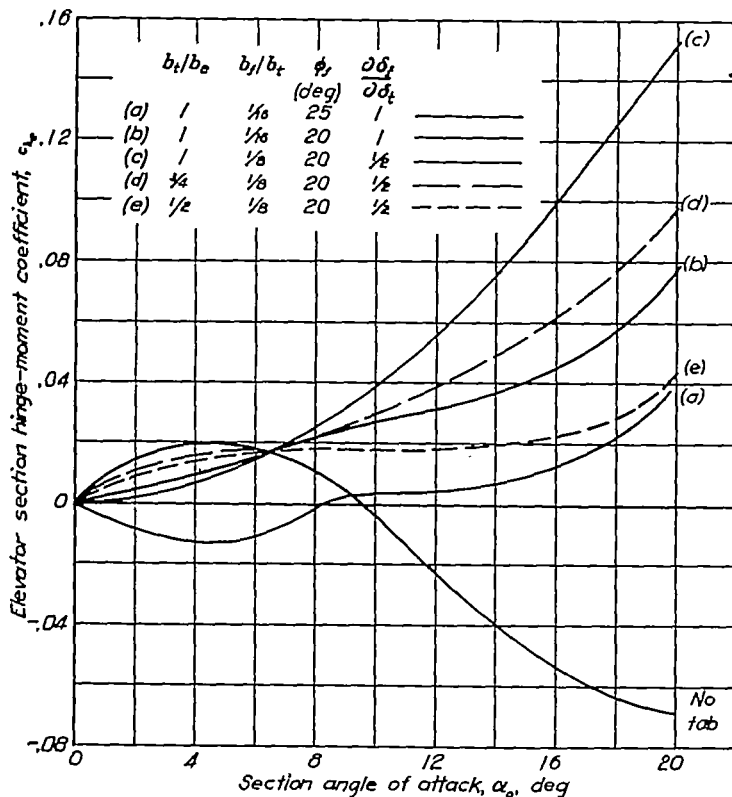
FIGURE 12.—Variation of c_h with \alpha_0 at \delta_0 = 0^\circ for various flipper-tab arrangements on a beveled elevator. Section data.
