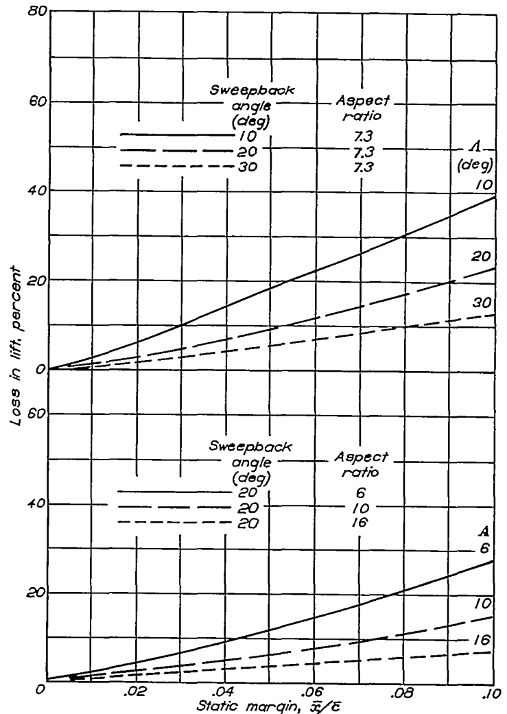
FIGURE 10.—Percent loss in lift caused by longitudinal control. c_{\theta}=0.30 ; \delta_a=21^\circ ; \frac{1}{\lambda}=4:1 . Control consists of extending elevator span inboard from tip until the resulting pitching moment about the center of gravity is zero.
