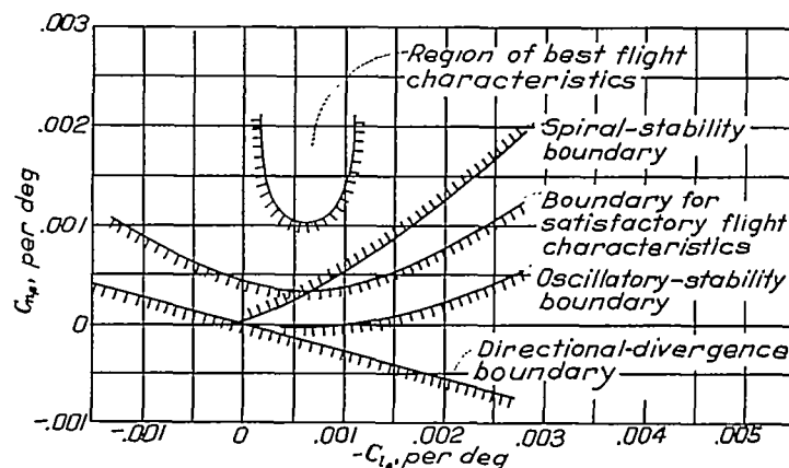
FIGURE 14.—Effect of directional stability C_{n\beta} and dihedral effect C_{l\beta} on flight characteristics as determined by tests of a model in Langley free-flight tunnel. C_L=1.0 .
