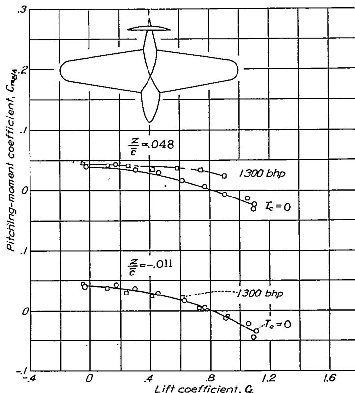
FIGURE 7.—Effect of power on the longitudinal stability of a pusher-type tailless airplane.
