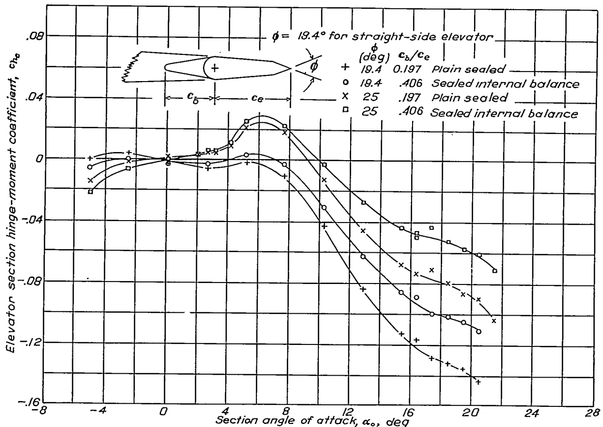
FIGURE 11.—Variation of section hinge-moment coefficient with angle of attack for 0.18c elevators on a modified NACA 65,3-018 airfoil. \delta_e = 0^\circ ; q = 59.4 pounds per square foot.
