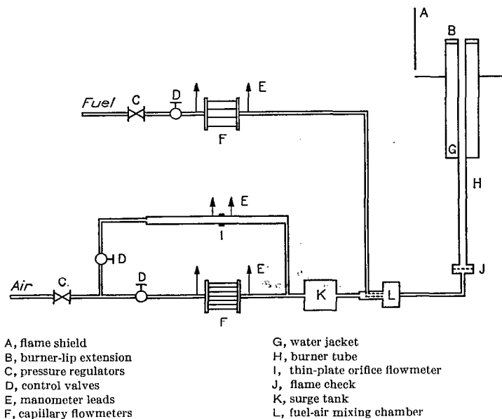
FIGURE 1.—Diagram of experimental apparatus.
