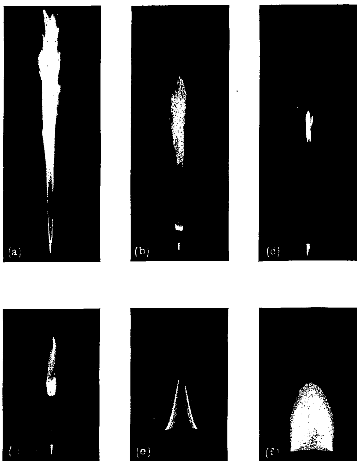
(a) Seated flame; turbulent flow; Reynolds number, 3770; fuel-air ratio, 0.183.
