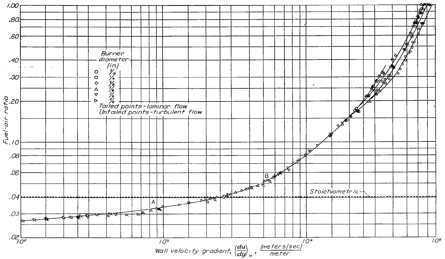
FIGURE 5.—Variation of fuel-air ratio with velocity gradient at tube wall for blow-off of seated propane-air flames.
