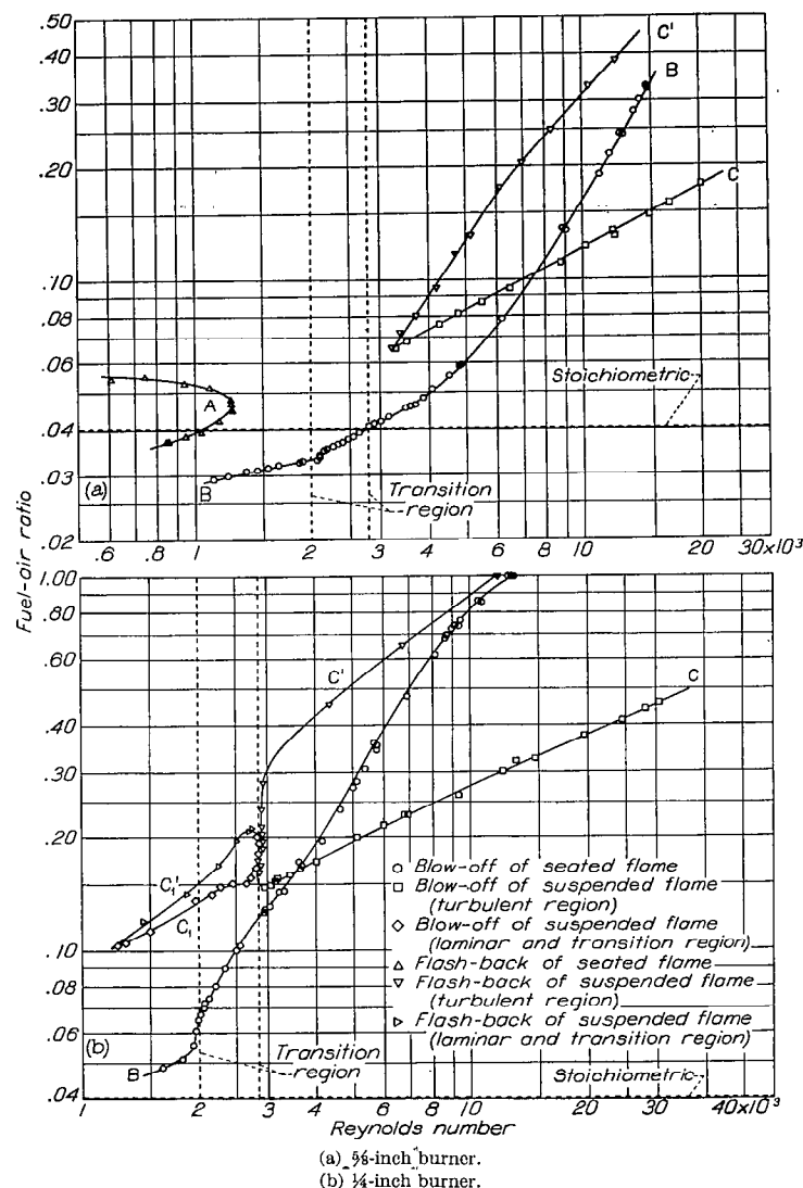
FIGURE 3.—Regions of stable burning for propane-air flames.
