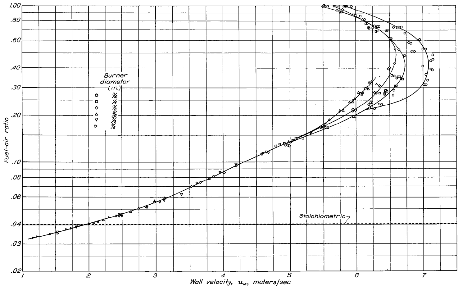
FIGURE 6.—Variation of fuel-air ratio with wall velocity for blow-off of turbulent seated propane-air flames.
