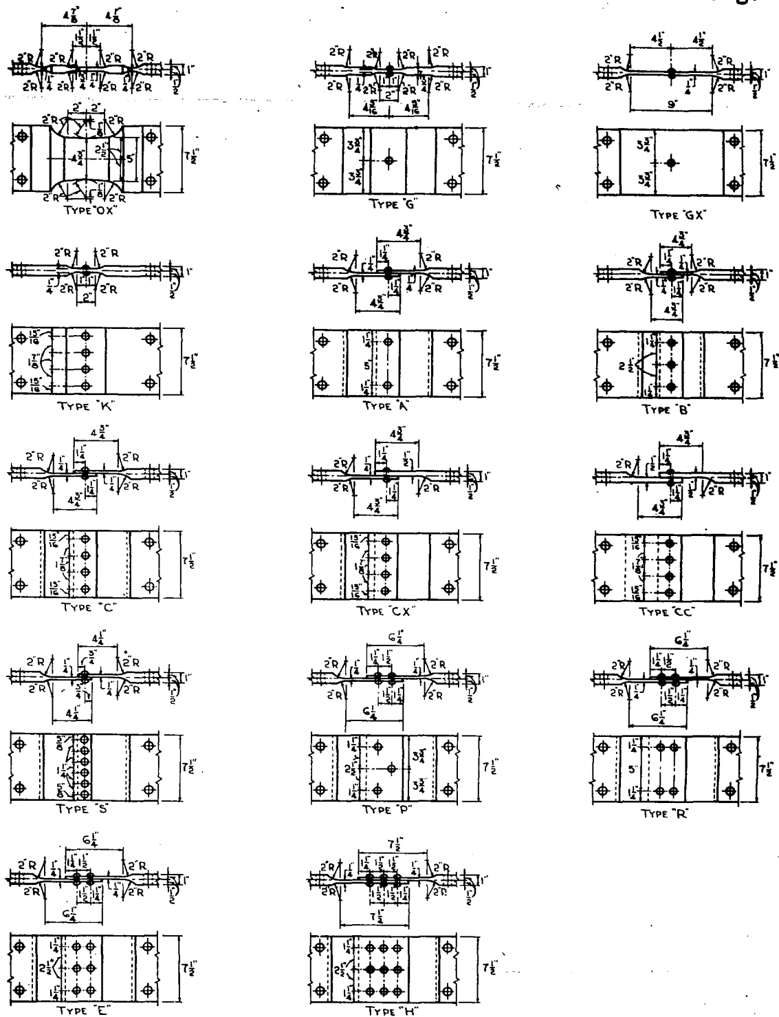
Figure 8.- Single plate and lap joint fatigue test specimens.
