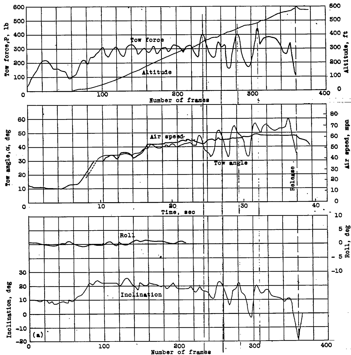
Figure 13(a to c).—Results of flight of Stiglmeier "Stick" glider launched by power winch.
