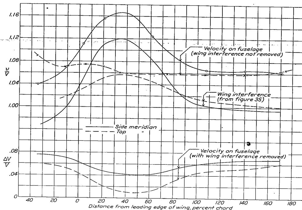
Figure 38.- Correction of velocity distribution on fuselage for wing interference. M , 0.194.
