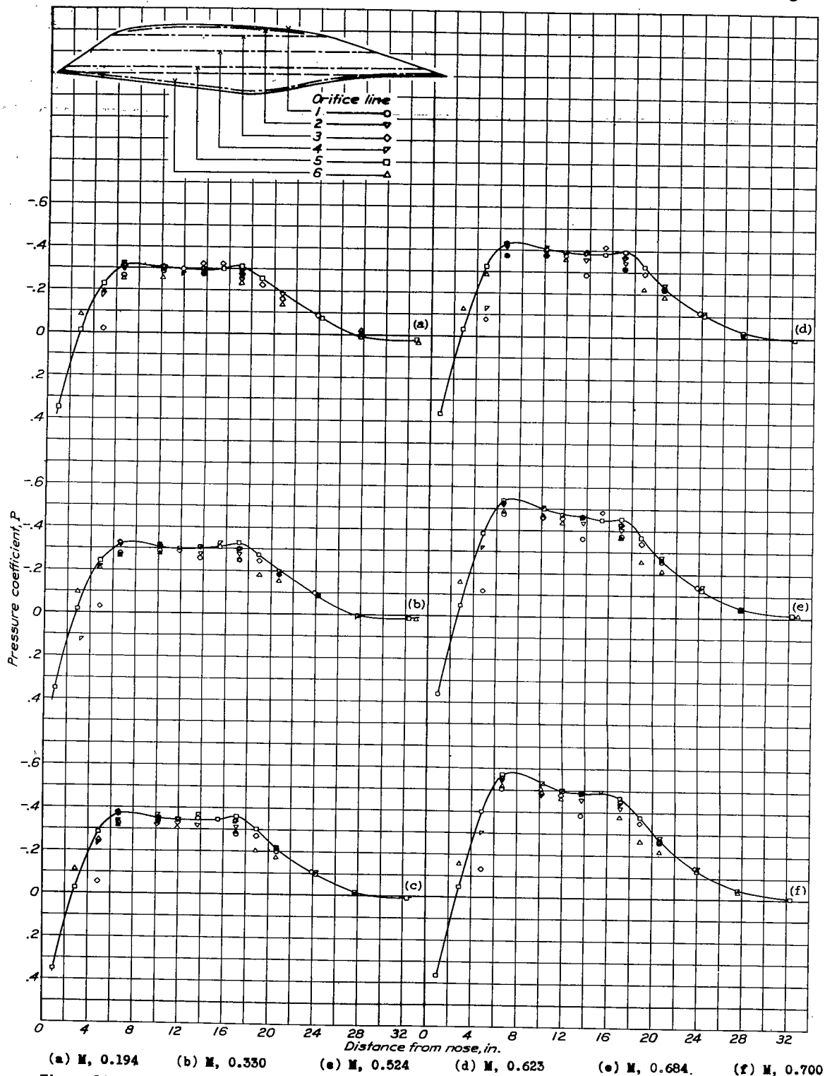
Figure 24.- Pressure distribution about the X-2 windshield for various Mach numbers. \alpha , -0.67^\circ .
