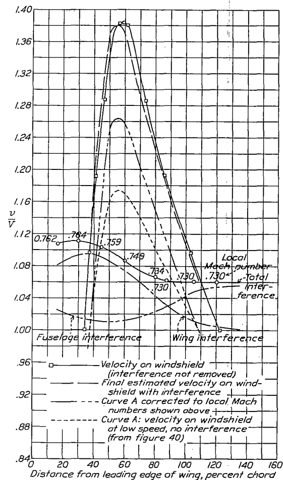
Figure 40.- Correction of velocity distribution on meridian 4 of X-1 windshield for interference. M , 0.688; \alpha , -0.67^\circ .
