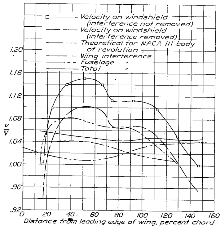
Figure 41.- Correction of velocity distribution on meridian 3 of 4-0-3 windshield for interference. M , 0.197. \alpha , -0.67^\circ .
