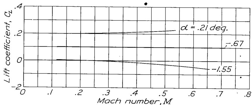
Figure 10.- Variation of model lift coefficient with Mach number.
