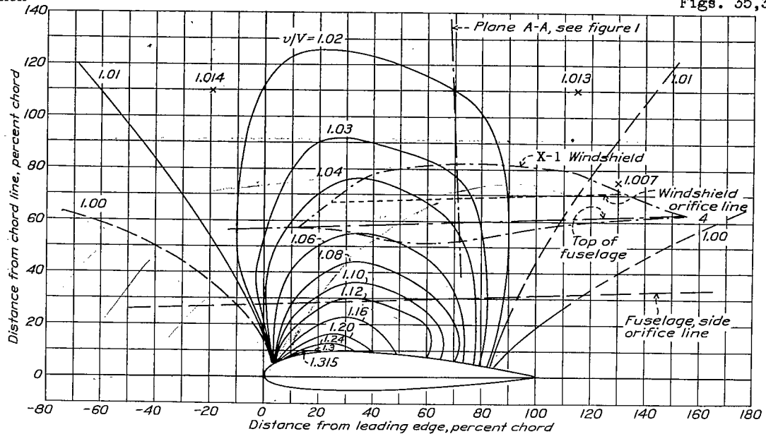
Figure 35.- Theoretical velocity contours for the NACA 2215 wing section. \alpha , -0.67^\circ .
