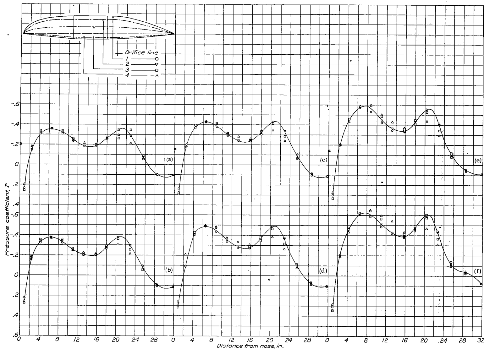
Figure 17.- Pressure distribution about the 3-1-2 windshield for various Mach numbers. \alpha , -0.67^\circ .
