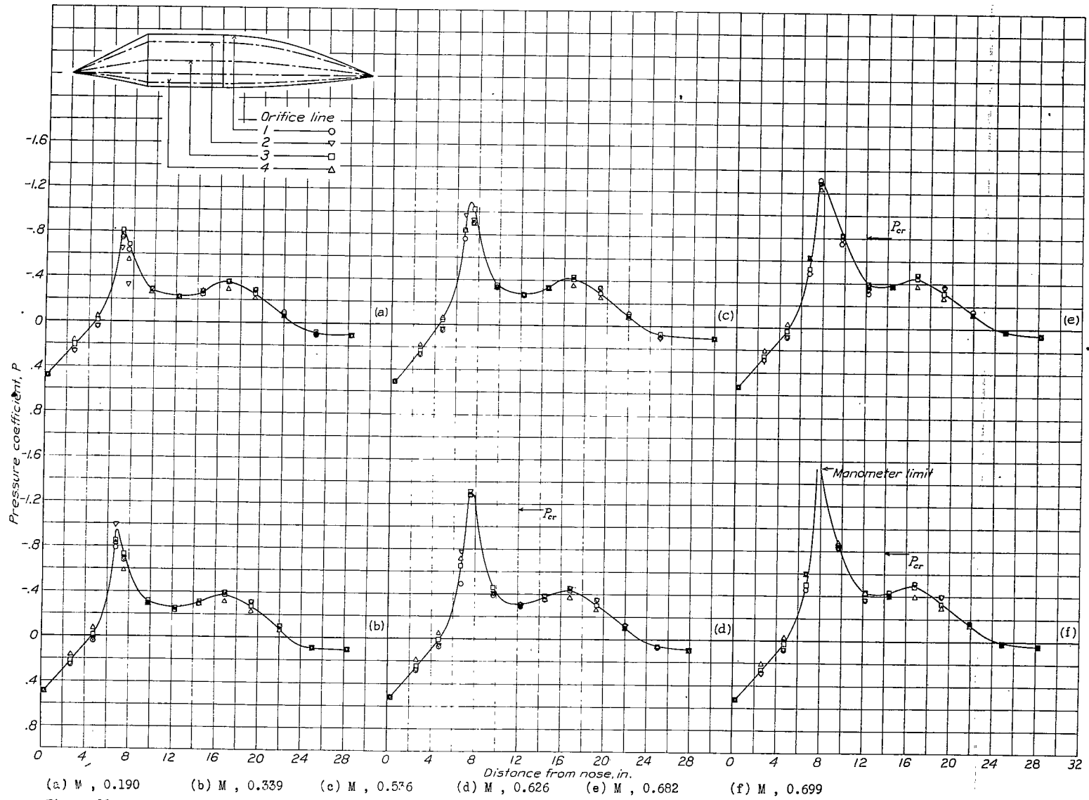
Figure 20.- Pressure distribution about the 10-1-2 windshield for various Mach numbers. \alpha , -0.67^\circ .
