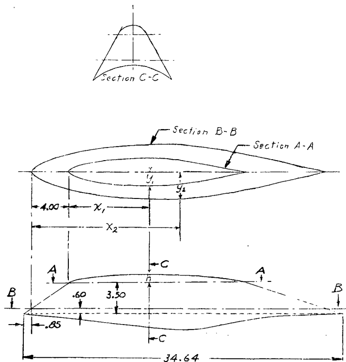
Figure 3.- The X-2 windshield.
