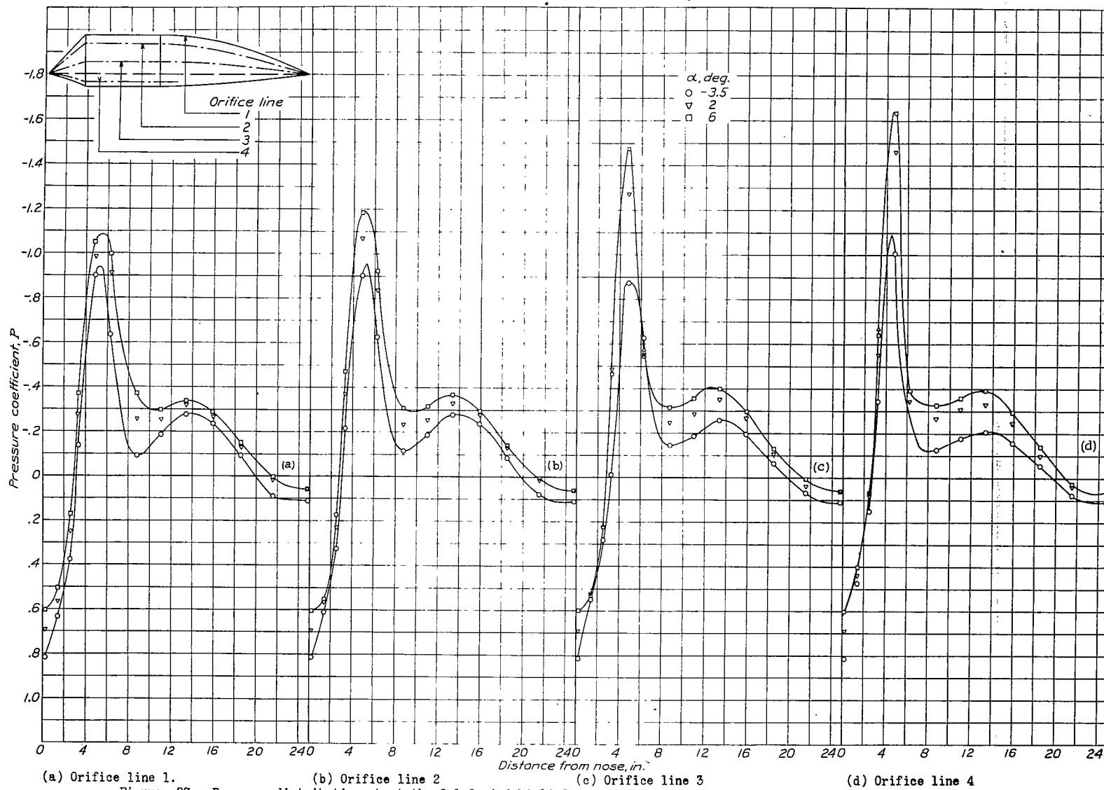
Figure 27.- Pressure distribution about the 9-1-2 windshield for various angles of attack. M , 0.196.
