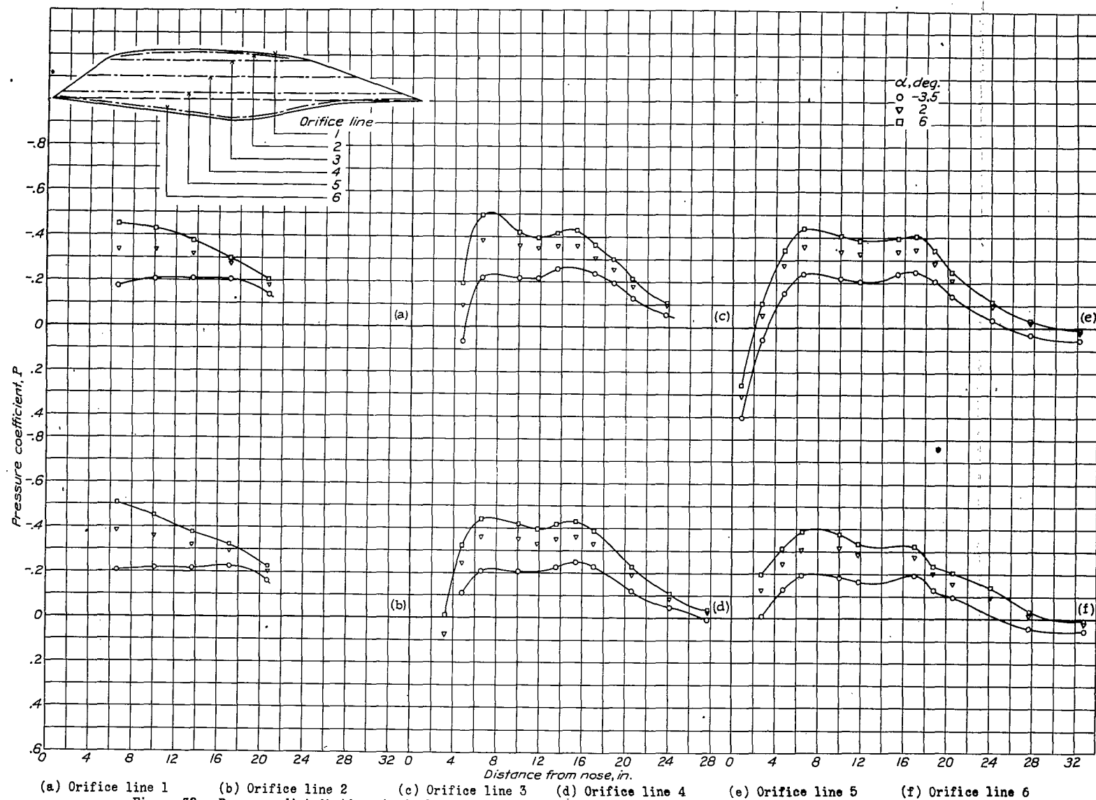
Figure 32.- Pressure distribution about the X-2 windshield for various angles of attack. M , 0.192.
