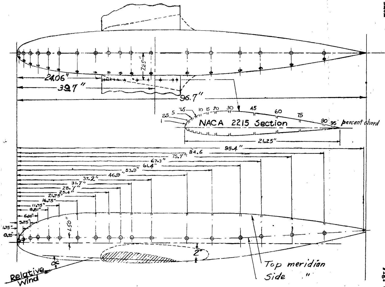
Figure 6. — Pressure-orifice locations on wing and fuselage
