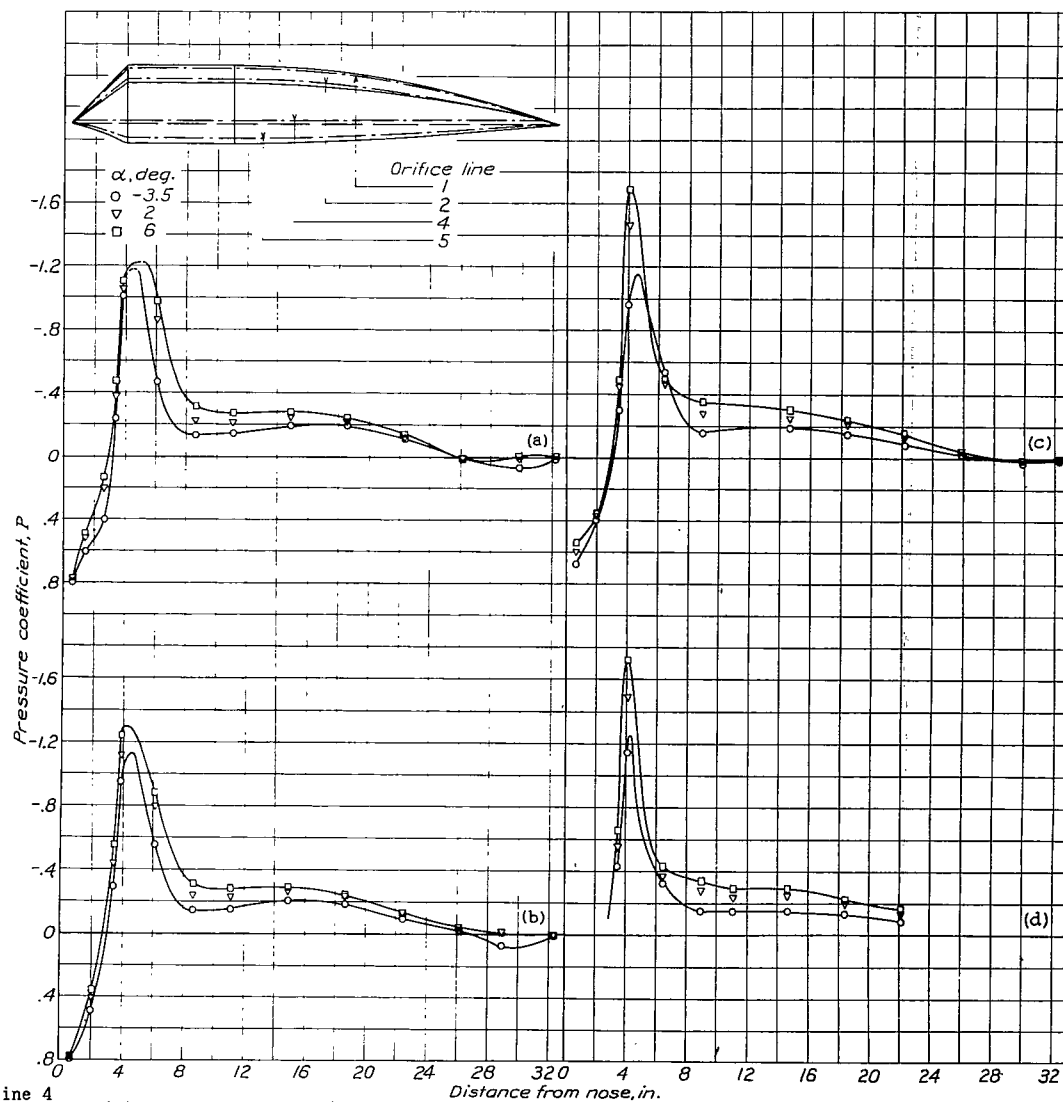
(a) Orifice line 1 (b) Orifice line 2 (c) Orifice line 4 (d) Orifice line 5 Figure 29.- Pressure distribution about the 7-3-4 windshield for various angles of attack. M , 0.192.
