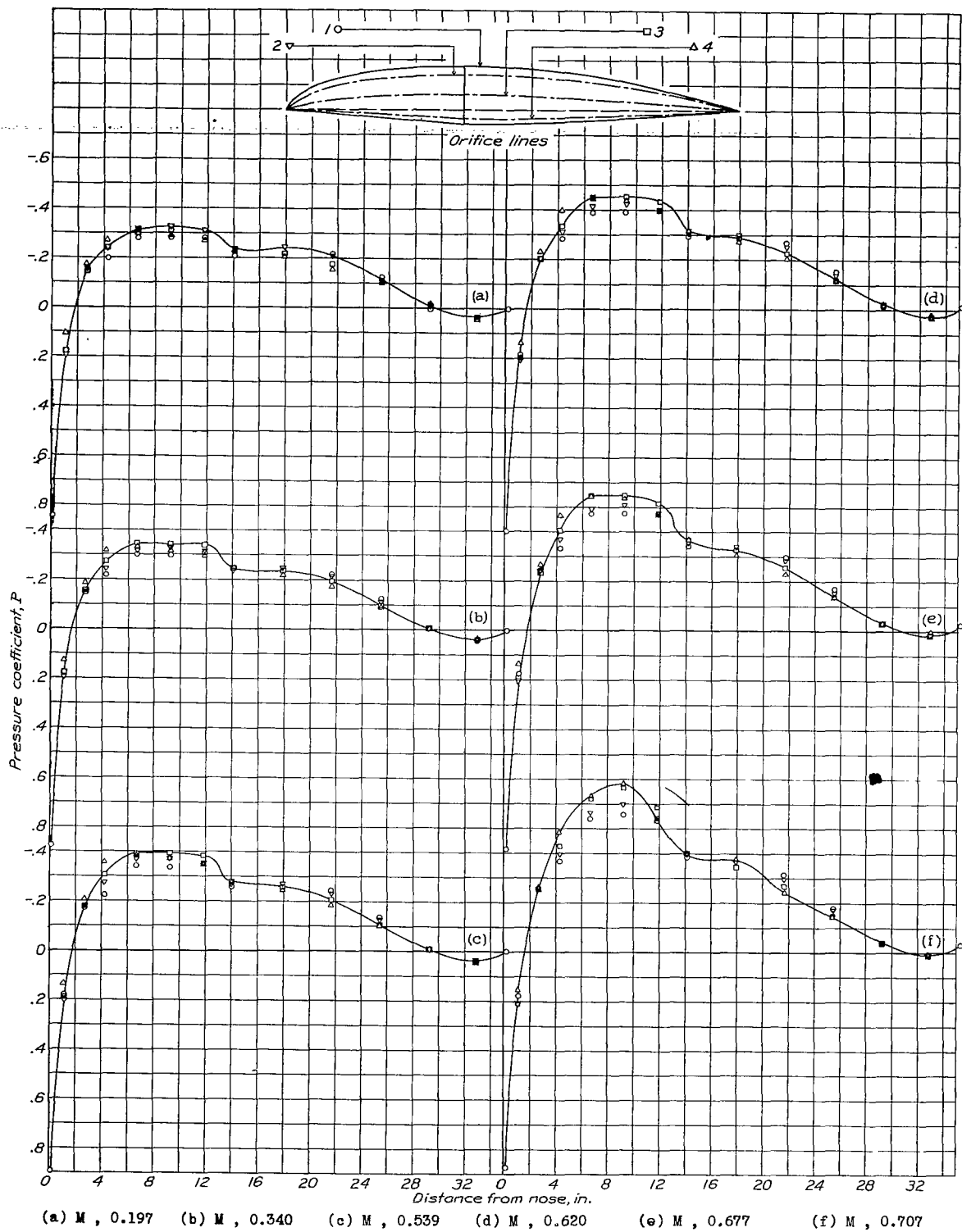
Figure 15.- Pressure distribution about the 4-0-3 windshield for various Mach numbers. \alpha , -0.67^\circ .
