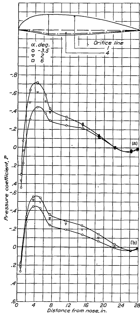
(a) Orifice line 1. (b) Orifice line 4 Figure 25.- Pressure distribution about the 2-0-3 windshield for various angles of attack. M , 0.199.
