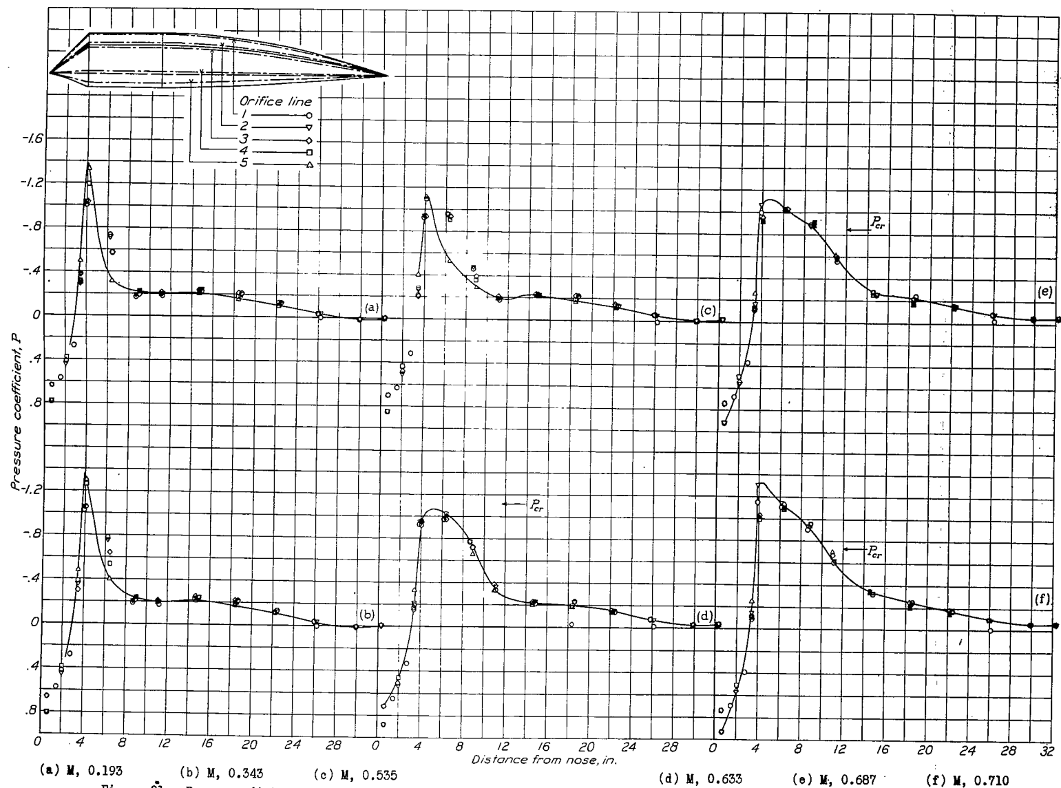
Figure 21.- Pressure distribution about the 7-3-4 windshield for various Mach numbers. \alpha , -0.67^\circ .
