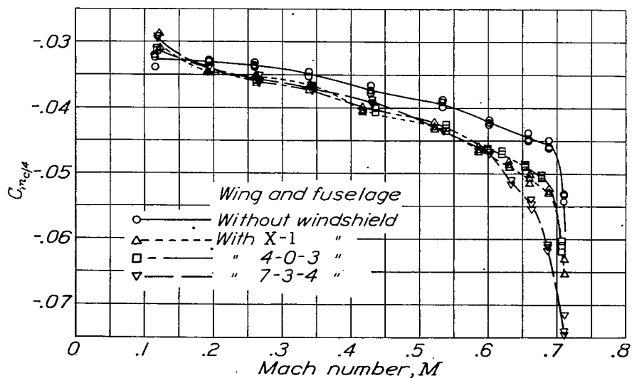
Figure 13.- Variation of model pitching-moment coefficient with Mach number. \alpha , -0.67^\circ .
