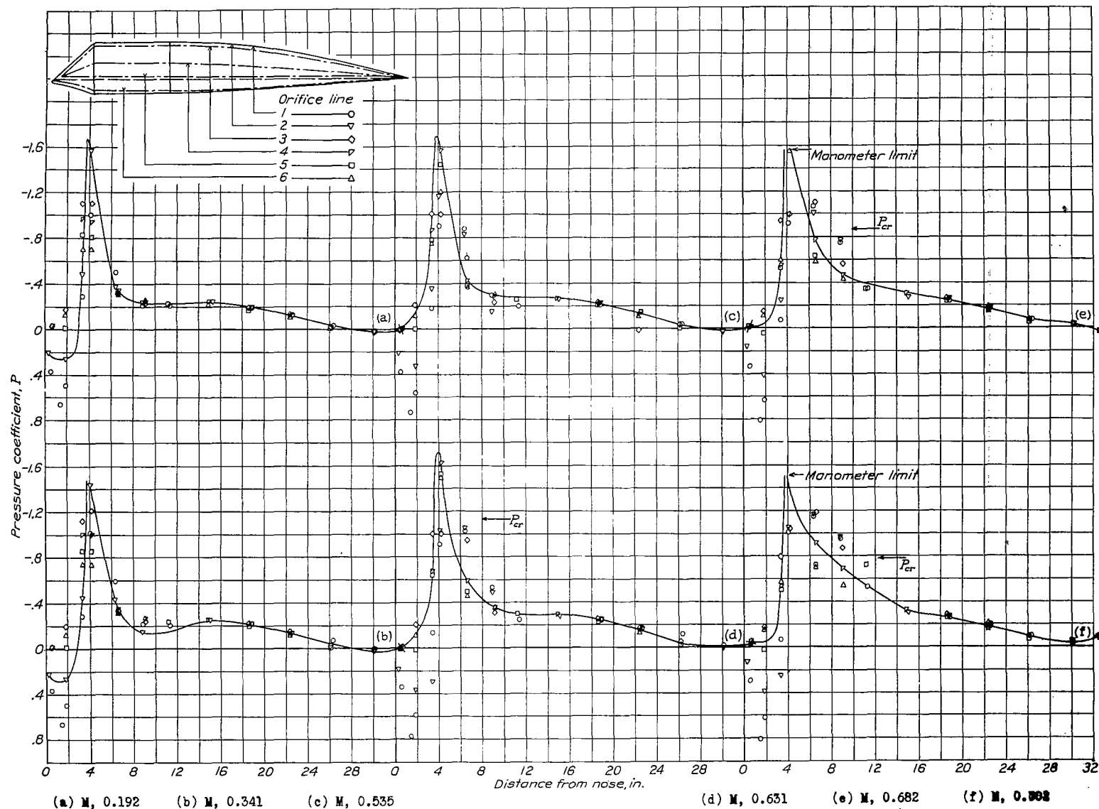
Figure 22.- Pressure distribution about the 8-4-5 windshield for various Mach numbers. \alpha, -0.67^\circ .
