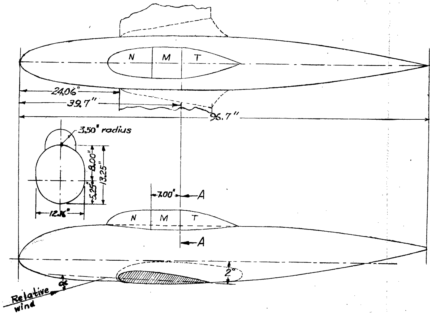
Figure 5.- Typical windshield installation.
