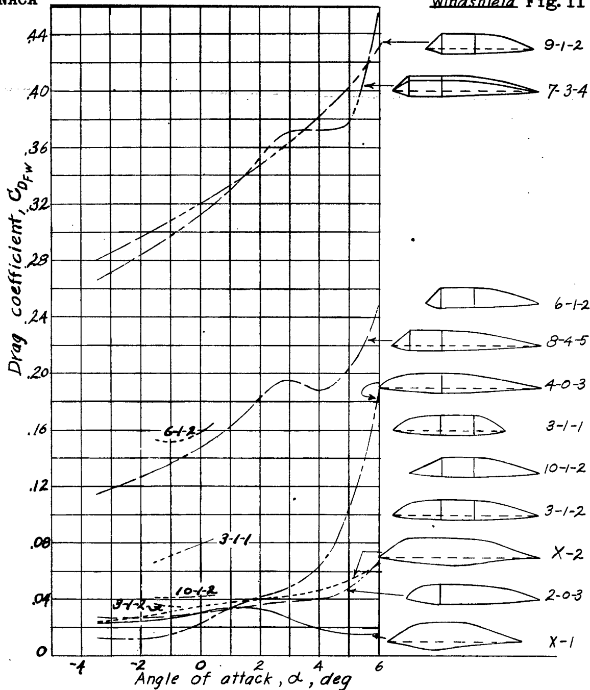
Figure 11.- Variation of windshield drag coefficient with angle of attack. M, 0.193 ; R, 1,980,000 .
