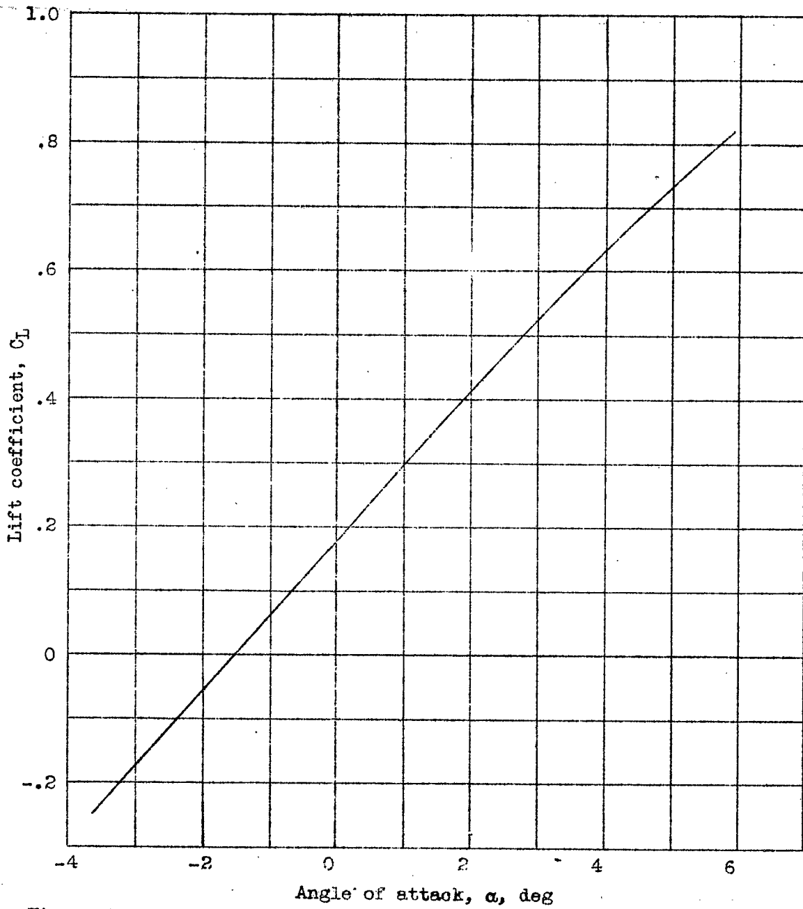
Figure 9.— Variation of model lift coefficient with angle of attack. M, 0.193; R, 1,980,000.
