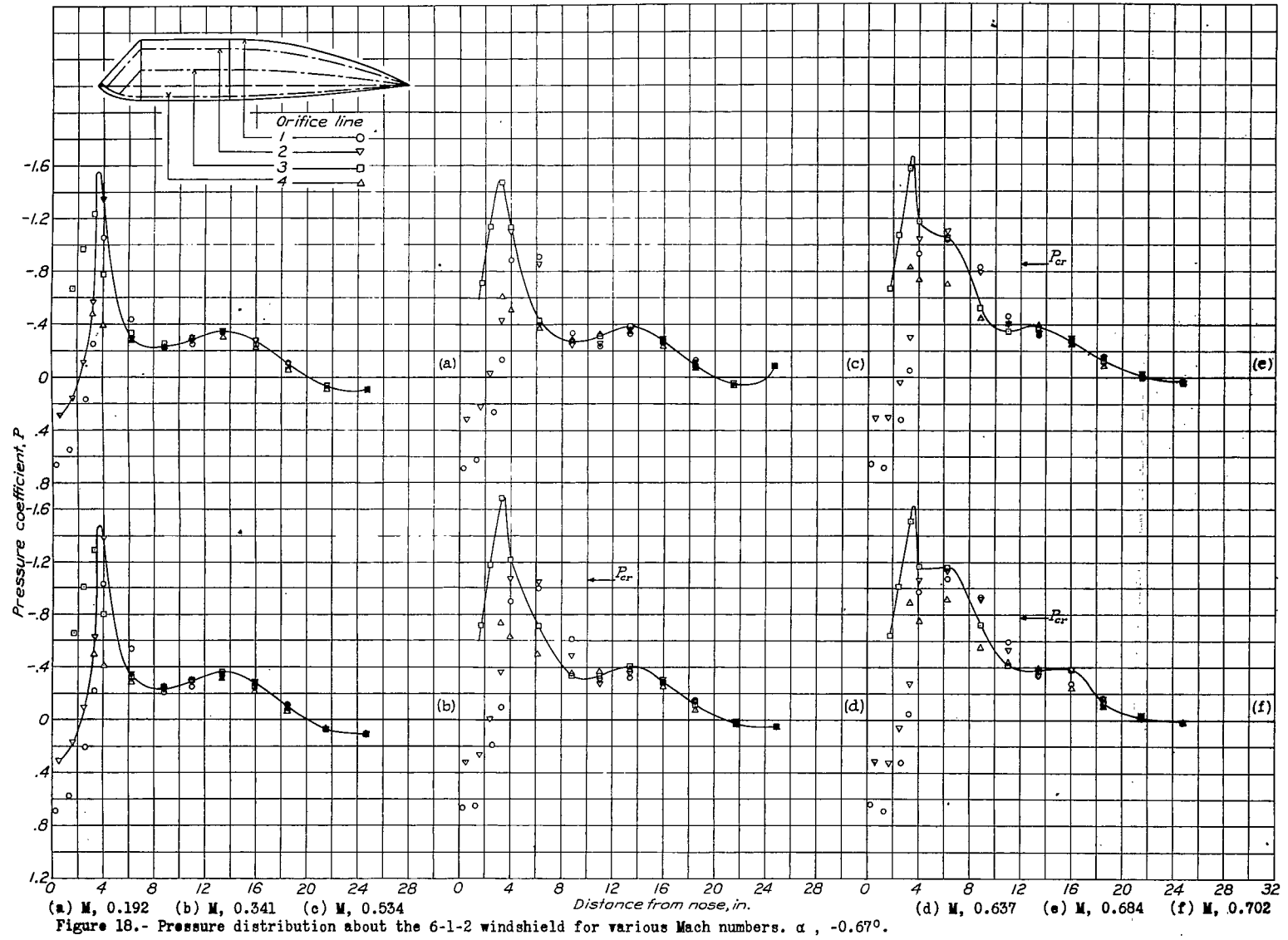
Figure 18.- Pressure distribution about the 6-1-2 windshield for various Mach numbers. \alpha, -0.67^\circ .
