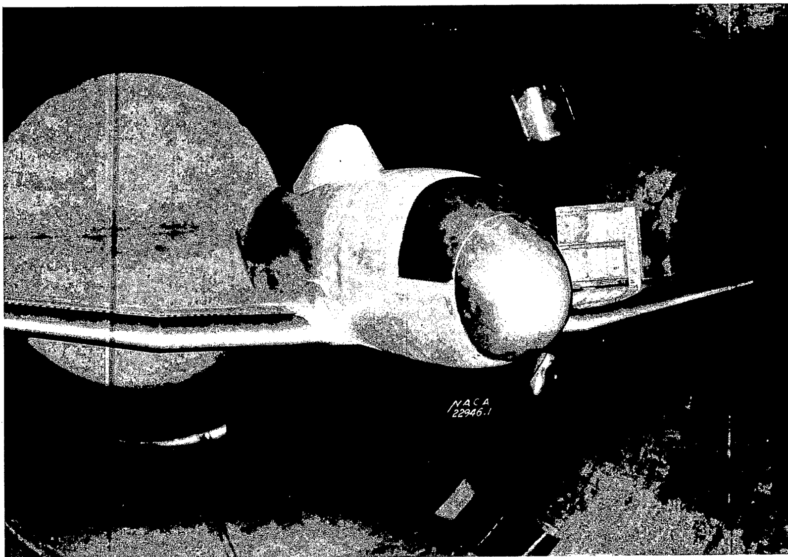
Figure 7.- Model installation in the tunnel showing the X-1 windshield.
