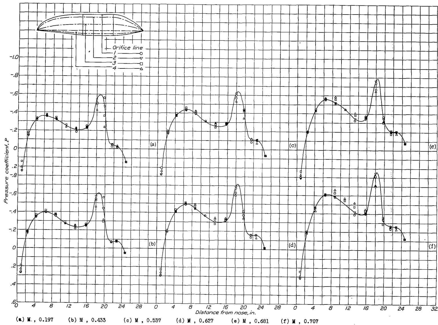
Figure 16.- Pressure distribution about the 3-1-1 windshield for various Mach numbers. \alpha , -0.67^\circ .
