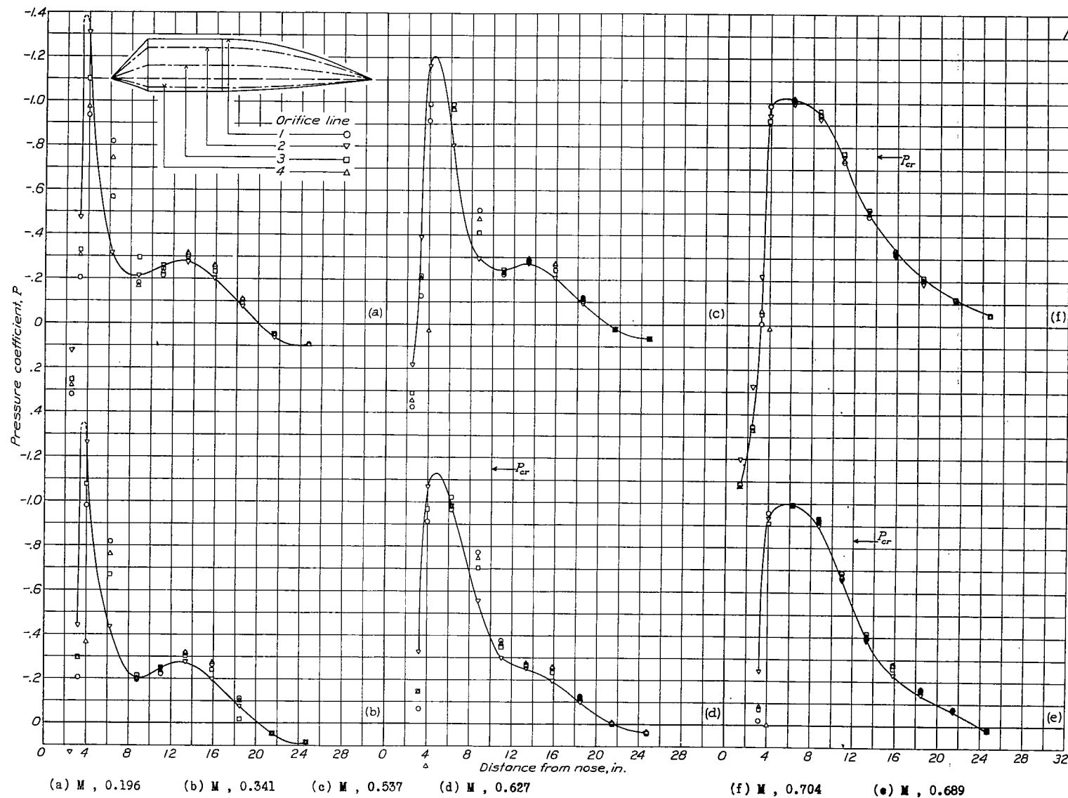
Figure 19.- Pressure distribution about the 9-1-2 windshield for various Mach numbers. \alpha , -0.67^\circ .
