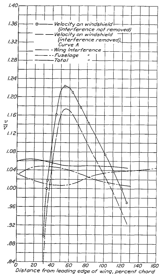
Figure 39.- Correction of velocity distribution on meridian 4 of X-1 windshield for interference. M , 0.191; \alpha , -0.67^\circ .
