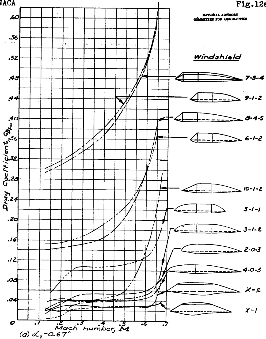
Figure 12(a,b).- Variation of windshield drag coefficient with Mach number.
