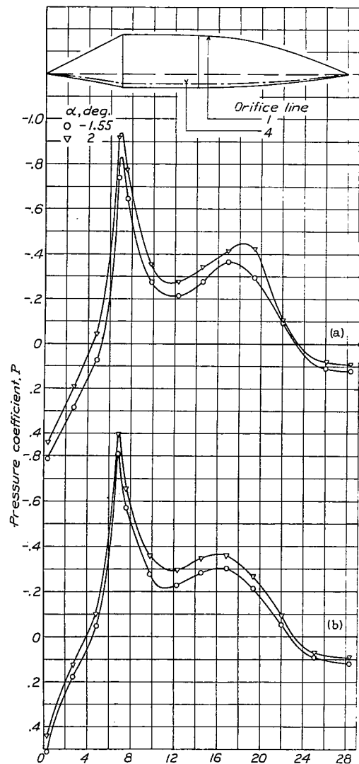
(a) Orifice line 1 Distance from nose, in. (b) Orifice line 4 Figure 28.- Pressure distribution about the 10-1-2 windshield for various angles of attack. M , 0.339.
