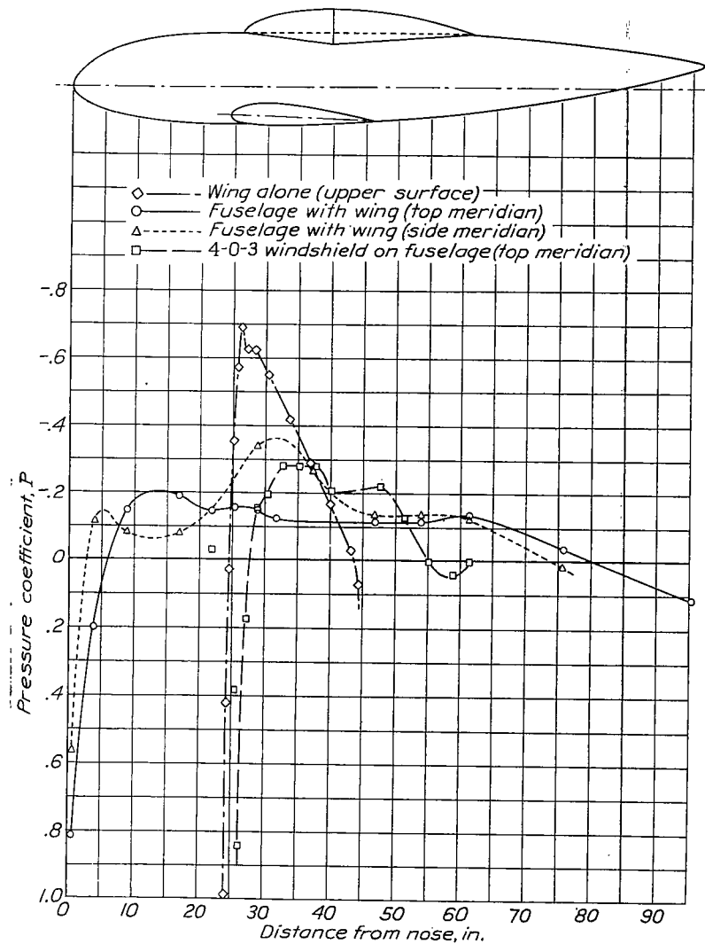
Figure 34.- Pressure distribution on wing, fuselage, and windshield. M, 0.194 ; \alpha, -0.67^\circ .
