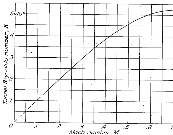
Figure 8.- Variation of test Reynolds number with Mach number.
