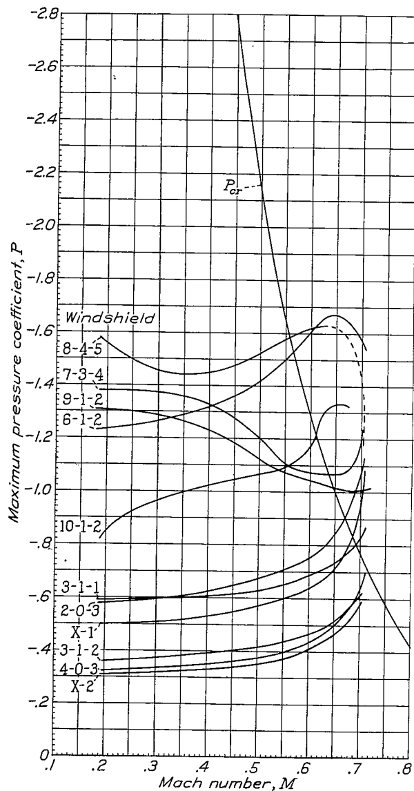
Figure 33.- Variation of the peak negative pressure coefficient with Mach number. \alpha, -0.67^\circ .
