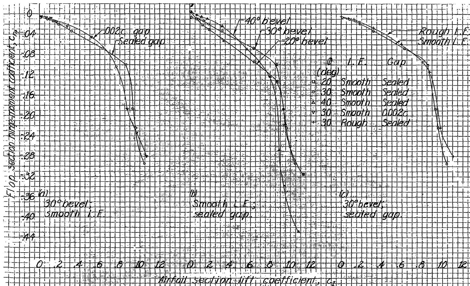
Figure 18-Variation of flap section hinge-moment coefficient with airfoil section lift coefficient for a 0.40c flap from \delta_f = 0^\circ to \delta_f = 30^\circ , \alpha_0 = 0^\circ .
