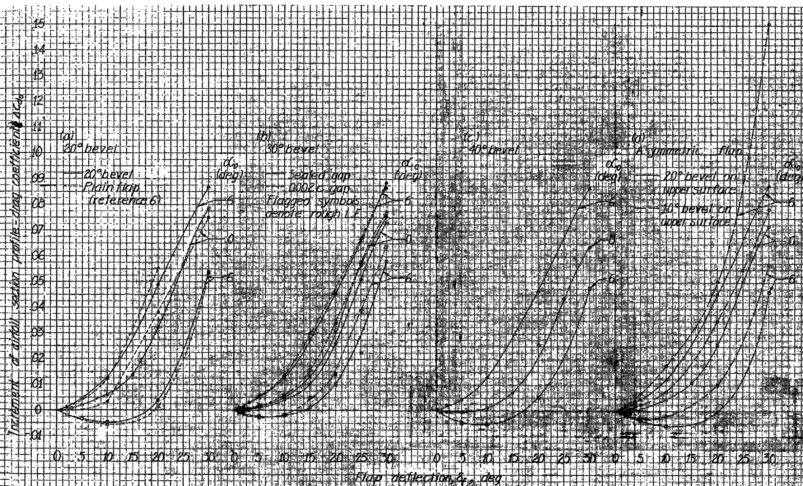
Figure 22. Increment of airfoil section profile-drag coefficient caused by deflection of a 0.30c flap with four beveled trailing edges. Smooth I.F. except as indicated.
