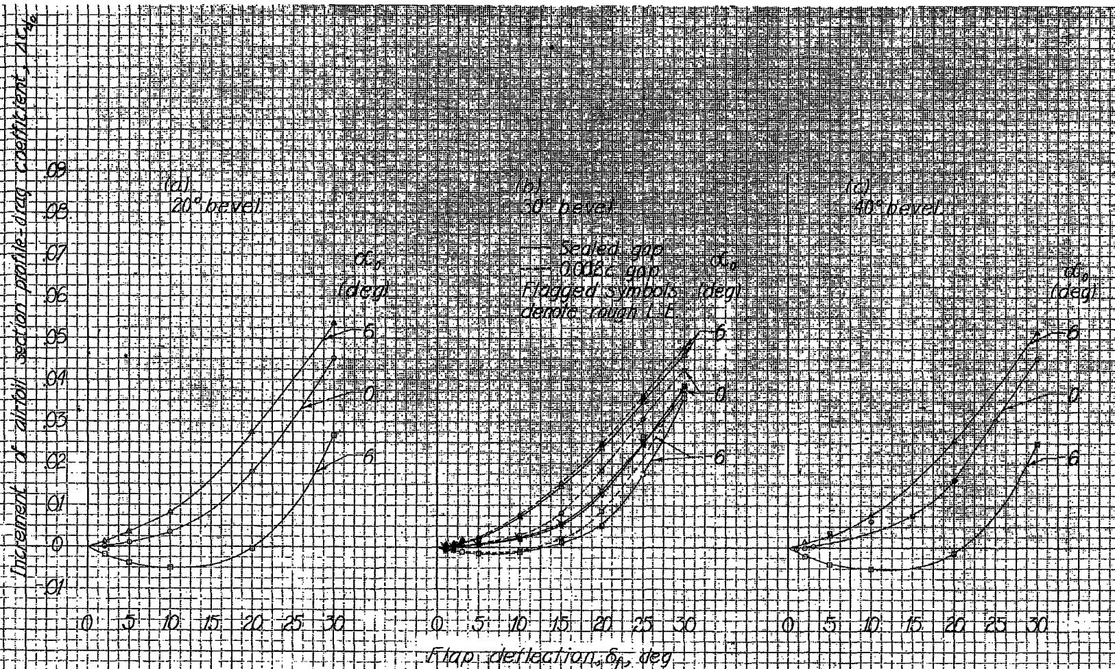
Figure 21 - Increment of airfoil section profile drag coefficient caused by deflection of a 0.80c flap with three beveled trailing edges. Smooth L.E. except as indicated.
