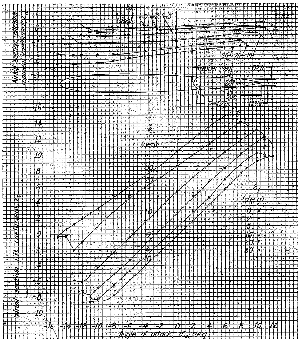
Figure 6 - Aerodynamic section characteristics of an NACA 0009 airfoil having 0.30c flap with 20° beveled trailing edge. Sealed gap, q = 11.25 pounds per square foot.
